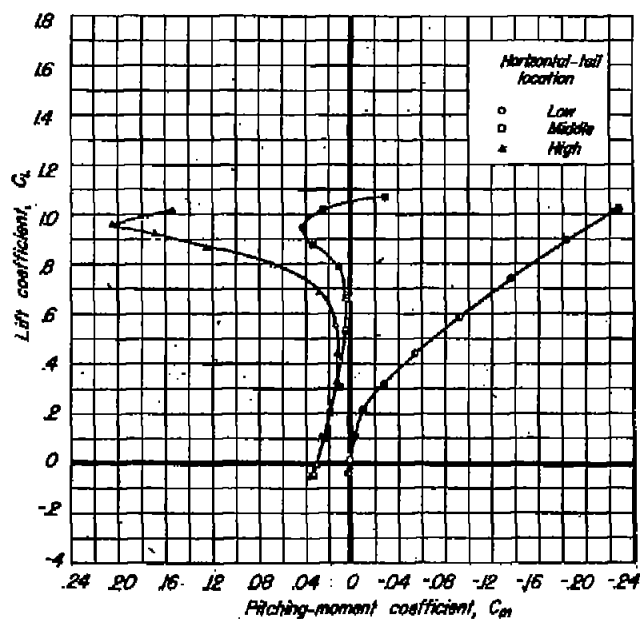
(a) \lambda, 0.33
