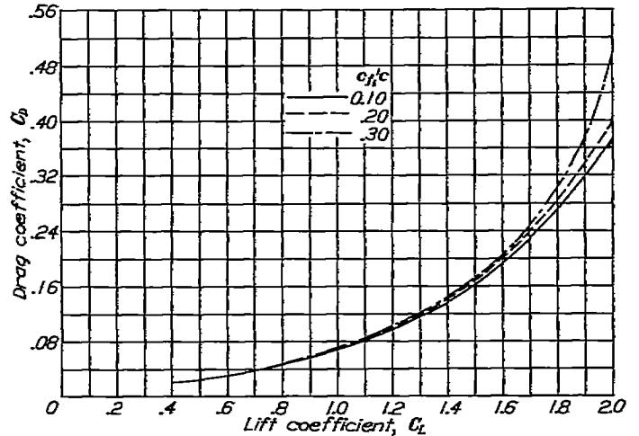
FIGURE 9.—Envelope drag polars for a Clark Y airfoil equipped with plain flaps of various sizes. R=0.609 \times 10^6 ; A=6 ; reference 10.
