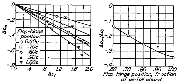
FIGURE 23.—Variation of increment of pitching-moment coefficient with increment of lift coefficient for various hinge positions of a 0.40c extensible split flap on a Clark Y airfoil. \alpha_0=0^\circ ; reference 18.
