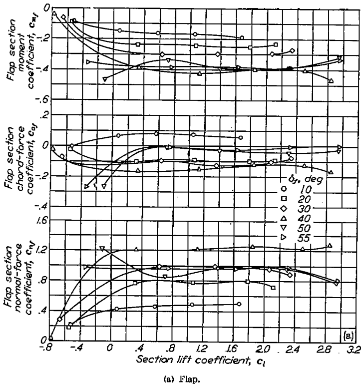
FIGURE 47.—Section force and moment characteristics for the double-slotted-flap arrangement on an NACA 83,4-421 (approx.) airfoil; partial slot-entry-skirt extension (see fig. 42 (b)). R=2.4 \times 10^6 .
