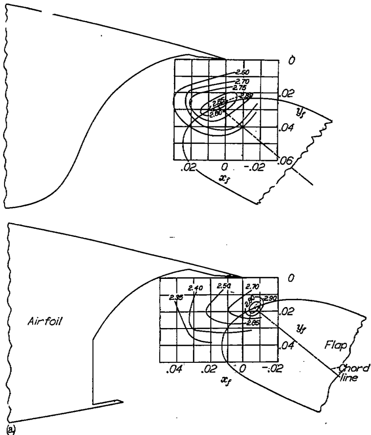
(a) NACA 66, 2-216, \alpha=0.6 airfoil with 0.25c slotted flap and two slot-entry configurations. R=5.1 \times 10^6 ; \delta_f=40^\circ ; reference 25.
