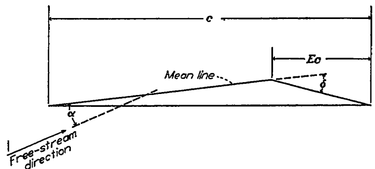
FIGURE 1.—Definition of parameters used in flap theory.
