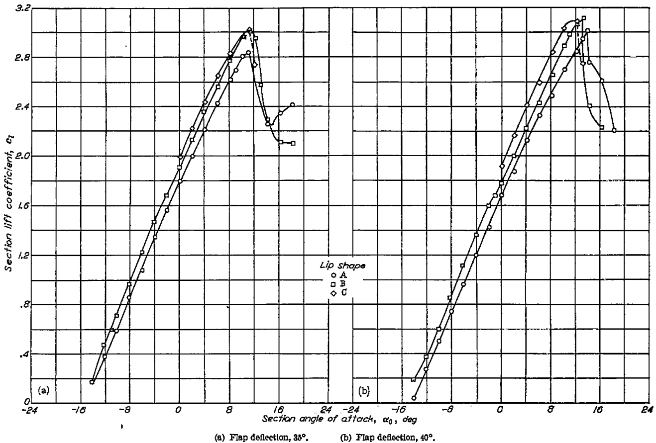
FIGURE 29.—Effect of slot-lip shape on section lift characteristics of an NACA 63,4-420 airfoil equipped with a 0.25c slotted flap. R=6.0 \times 10^6 .
