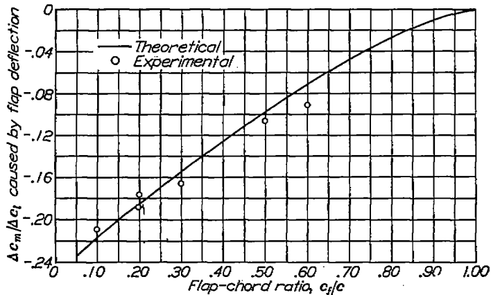
FIGURE 11.—Variation of ratio of pitching-moment coefficient to lift coefficient at constant angle of attack with flap-chord ratio.
