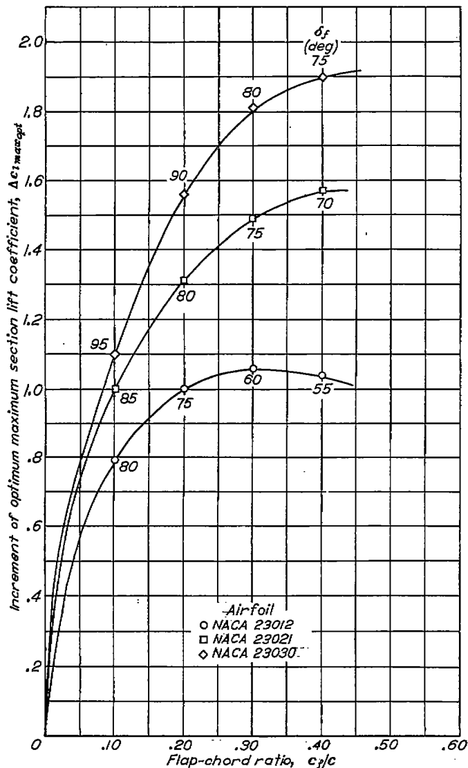
FIGURE 15.—Variation of increment of optimum maximum section lift coefficient with flap-chord ratio. NACA 230-series airfoils equipped with split flaps. R=2.5 \times 10^6 .
