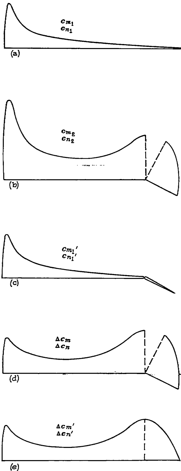
(a) Normal-force distribution for airfoil with flap neutral. (b) Normal-force distribution for airfoil with flap deflected. (c) Distribution shown in (a) with flap normal-force distribution plotted normal to flap-deflected chord. (d) Incremental normal-force distribution caused by flap deflection. (e) Distribution shown in (d) plotted normal to flap-neutral chord.
