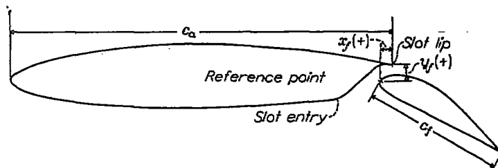
FIGURE 24.—Sketch of typical single-slotted-flap configuration. (All dimensions are given in fractions of airfoil chord.)
