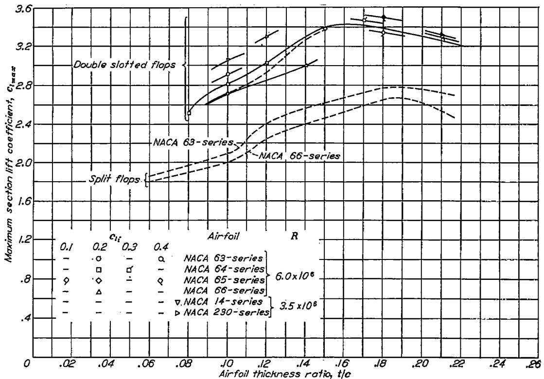
FIGURE 44.—Maximum section lift coefficients for several NACA airfoil sections with double slotted and split flaps.
