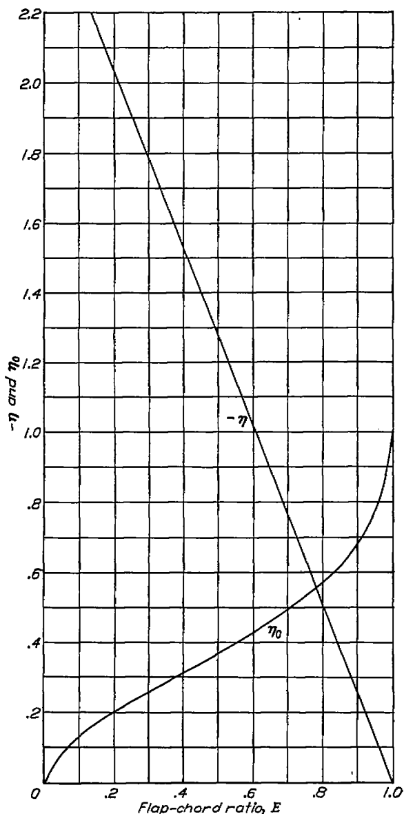
FIGURE 3.—Factors \eta and \eta_0 in equation for flap normal-force coefficients. Reference 4.
