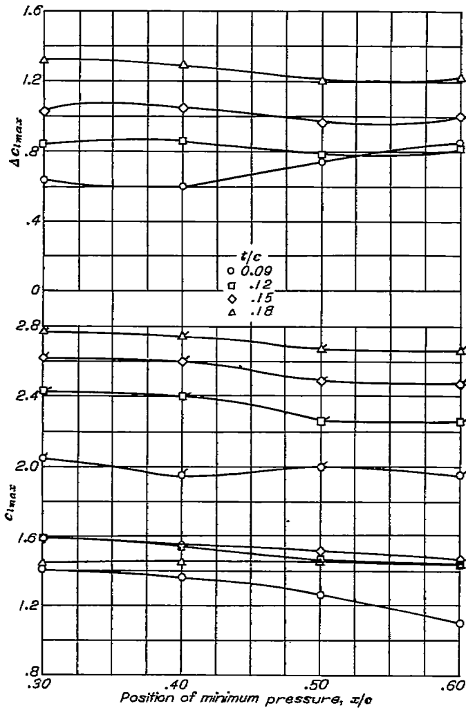
FIGURE 18.—Variation of maximum section lift coefficient with position of minimum pressure and airfoil thickness ratio for some NACA 6-series airfoil sections with and without split flaps. c_f=0.2 ; R=6.0 \times 10^6 . (Flagged symbols are for 60° simulated split flap.)
