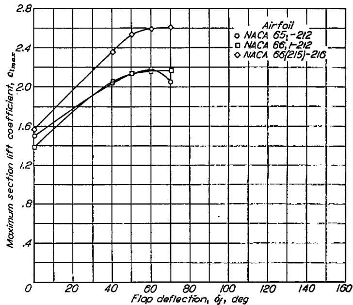
FIGURE 16.—Variation of maximum section lift coefficient with flap deflection for several NACA 6-series airfoil sections equipped with 0.20c split flaps. R=6.0 \times 10^6 ; reference 18.
