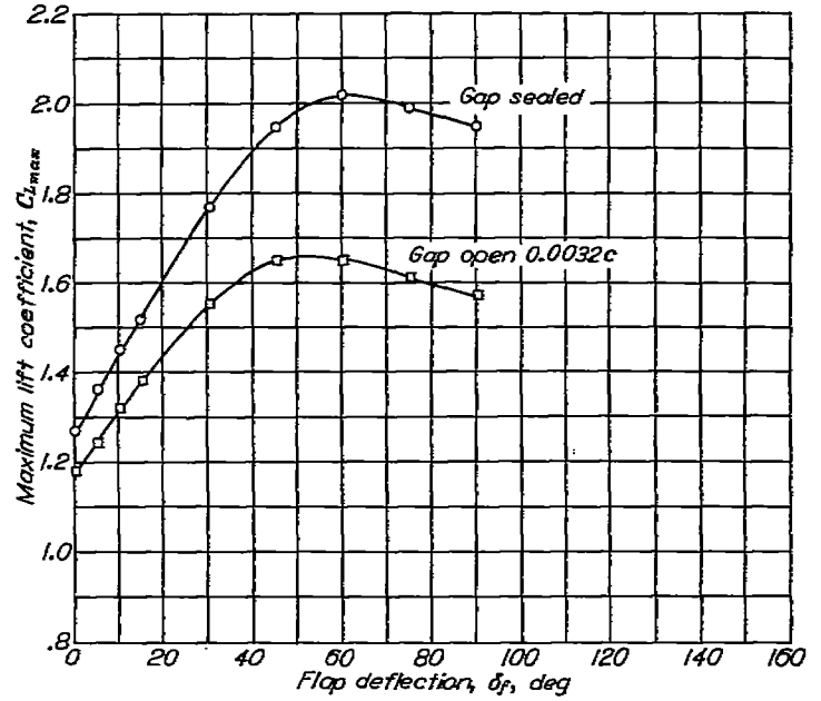
FIGURE 8.—Effect of gap seal on maximum lift coefficient of a rectangular Clark Y wing equipped with a full-span 0.20c plain flap. A=6 ; R=0.609 \times 10^6 ; reference 10.
