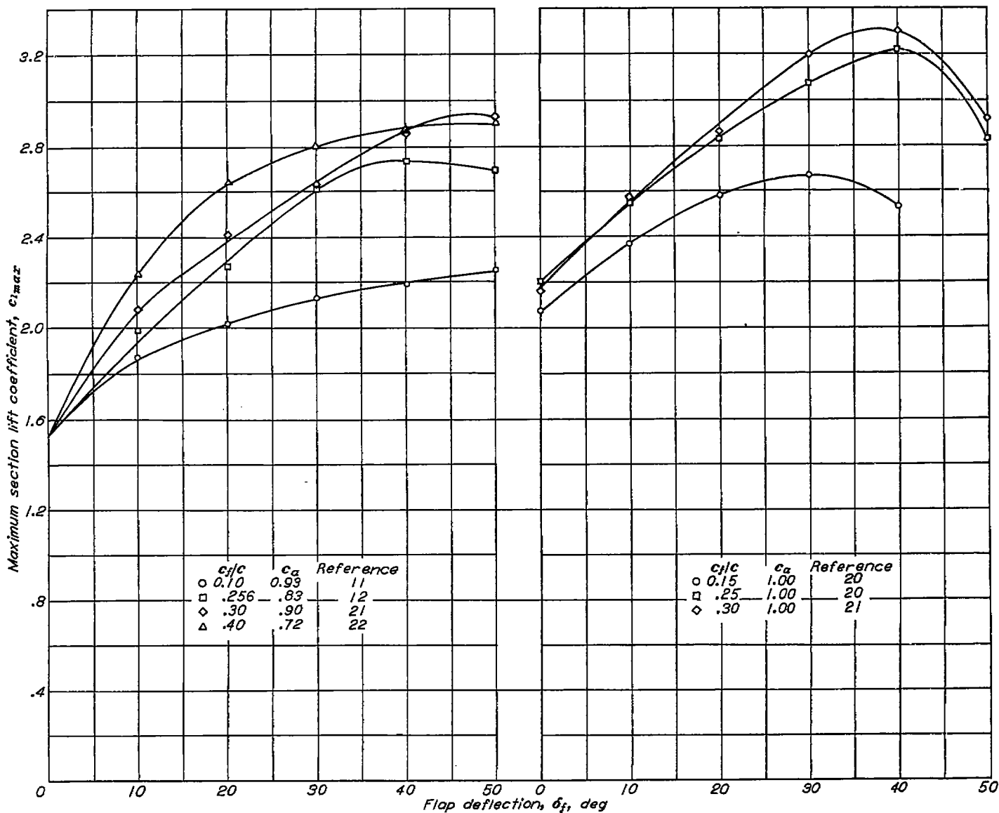
FIGURE 25.—Variation of maximum section lift coefficient with flap deflection for the NACA 23012 airfoil equipped with various slotted flaps. R=3.5 \times 10^4 .
