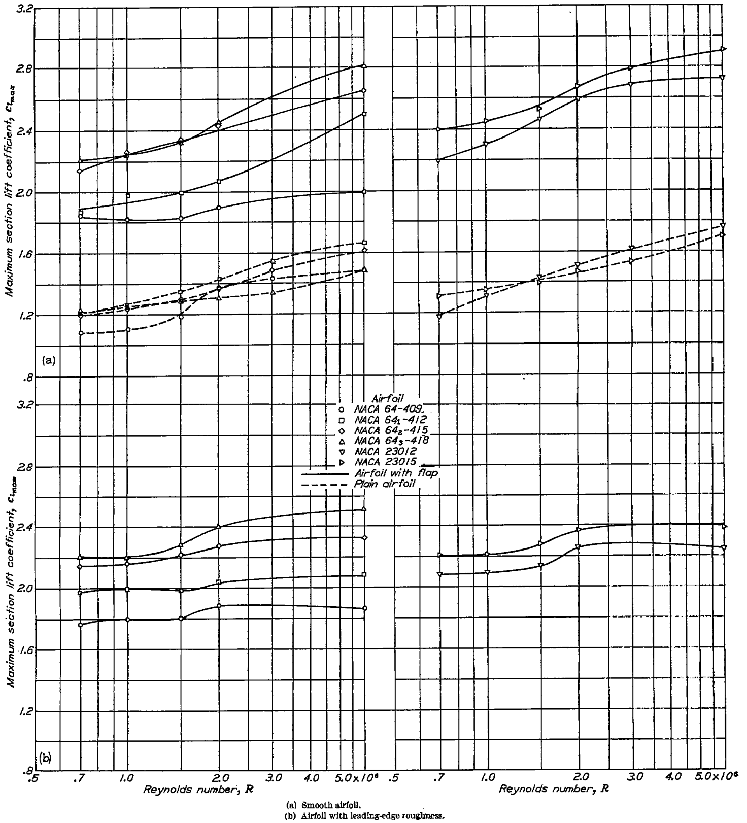
FIGURE 19.—Variation of maximum section lift coefficient with Reynolds number for several NACA airfoil sections with and without 0.20c split flaps deflected 60°.
