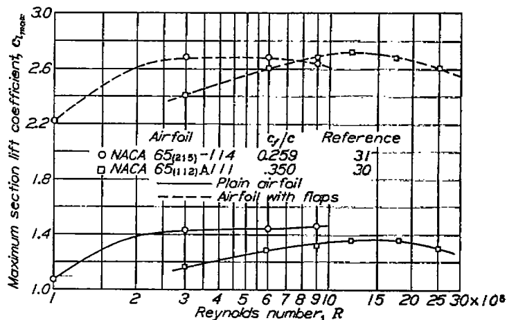
FIGURE 33.—Scale effect on maximum section lift coefficient for two low-drag airfoil sections equipped with slotted flaps.
