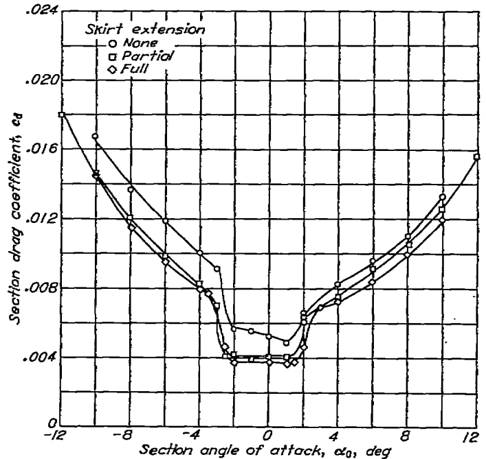
FIGURE 38.—Effect of slot-entry-skirt extension on section drag characteristics of an NACA 66,2-116, \alpha=0.6 airfoil equipped with a 0.25c slotted flap. \delta_f=0^\circ ; R=6.0 \times 10^6 ; reference 34. (Same airfoil-flap combination as fig. 28.)
