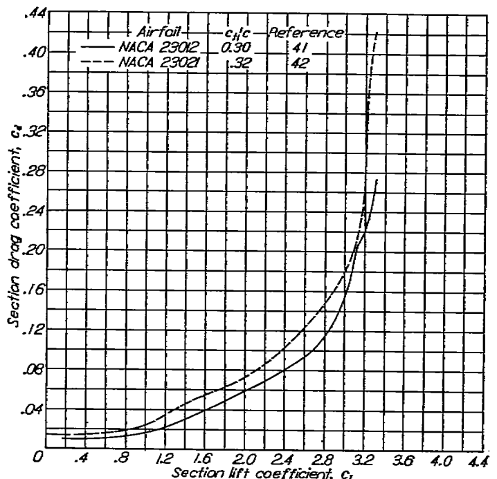
FIGURE 46.—Comparison of envelope polars for two airfoil sections equipped with double slotted flaps. R=3.5 \times 10^6 .
