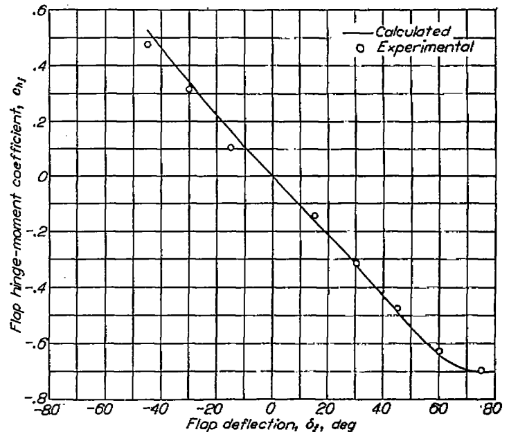
FIGURE 13.—Variation of flap hinge-moment coefficient with flap deflection. NACA 23012 airfoil; 0.20c plain flap; \alpha_i=0^\circ .
