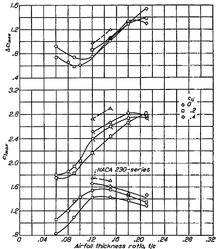
FIGURE 17.—Variation of maximum section lift coefficient with airfoil thickness ratio and camber for some NACA 64-series airfoil sections with and without simulated split flaps. R=6.0 \times 10^6 ; reference 7. (Flagged symbols are for 90° simulated split flaps.)
