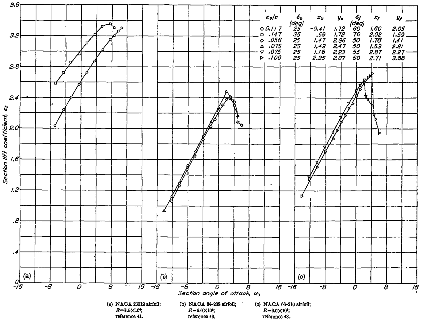
FIGURE 41.—Effect of vane size on lift characteristics of several airfoil sections with double slotted flaps.
