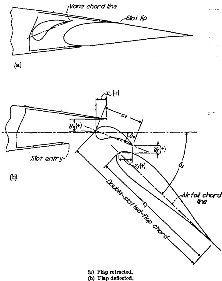
FIGURE 40.—Sketch of typical double-slotted-flap configuration. (All dimensions are given in fractions of airfoil chord.)
