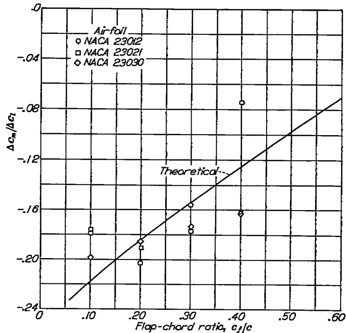
FIGURE 21.—Variation of ratio of increment of section pitching-moment coefficient to increment of section lift coefficient with flap-chord ratio for several airfoil sections equipped with split flaps. \alpha=0^\circ ; reference 15.
