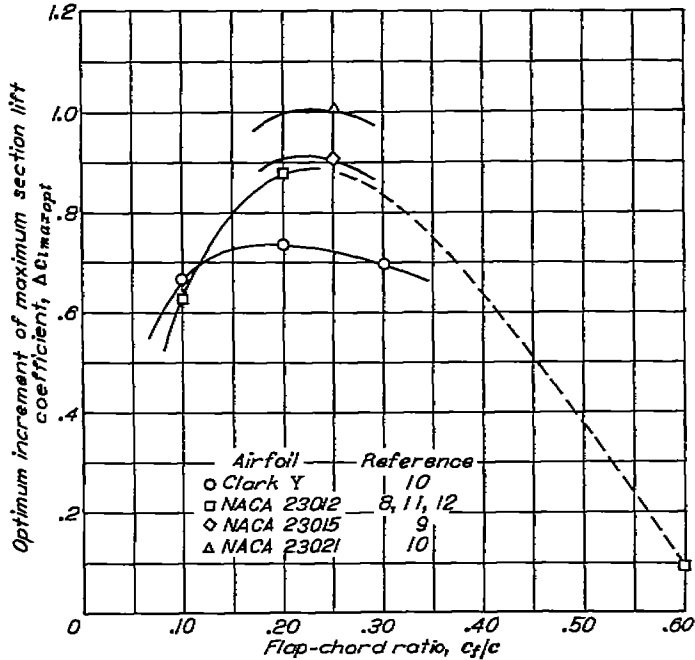
FIGURE 7.—Variation of optimum increment of maximum section lift coefficient with flap-chord ratio for several airfoil sections equipped with plain flaps.
