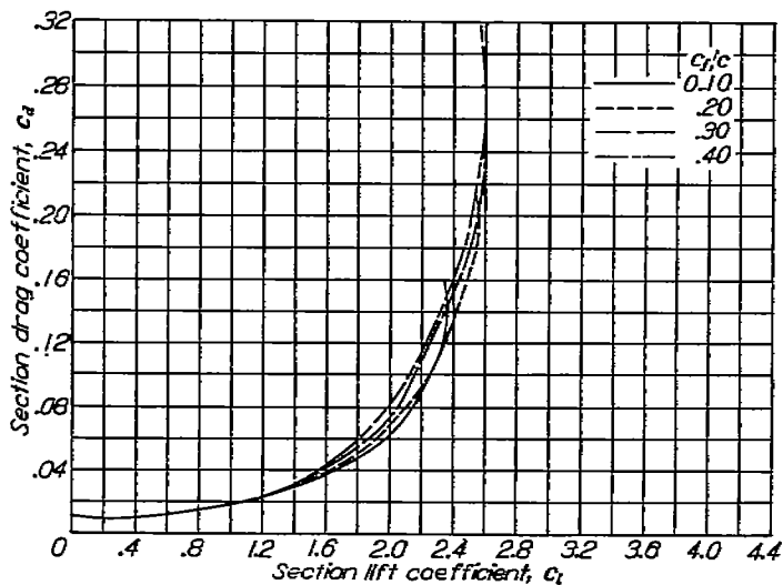
FIGURE 20.—Envelope drag polars for an NACA 23012 airfoil equipped with split flaps of various sizes. R=3.5 \times 10^6 ; reference 15.
