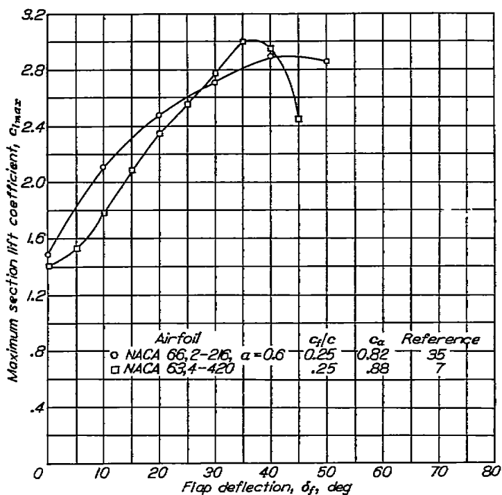
FIGURE 26.—Variation of maximum section lift coefficient with flap deflection for several NACA 6-series airfoil sections equipped with slotted flaps. R = 5.1 \times 10^6 for NACA 66-series airfoil and R = 6.0 \times 10^6 for NACA 63-series airfoil.
