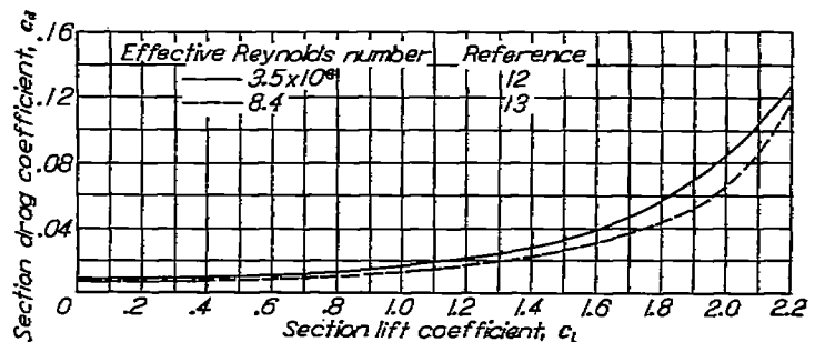
FIGURE 10.—Envelope drag polars for an NACA 23012 airfoil equipped with a 0.20c plain flap at two Reynolds numbers.
