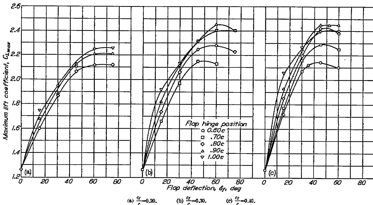
FIGURE 22.—Variation of maximum lift coefficient with flap deflection and hinge position for a Clark Y airfoil equipped with extensible split flaps of various sizes. R=0.6 \times 10^6 ; A=6 ; reference 18.
