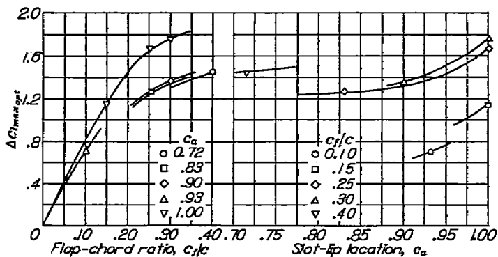
FIGURE 27.—Variation of optimum increment of section maximum lift coefficient with flap-chord ratio and with slot-lip location for the NACA 23012 airfoil section.
