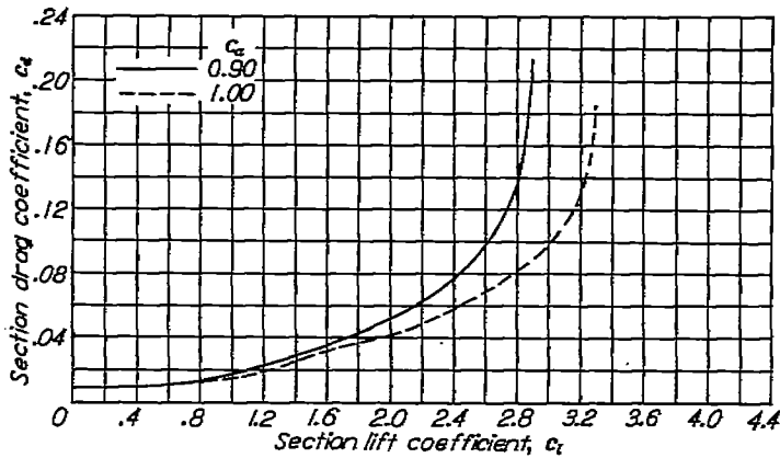
FIGURE 35.—Effect of slot-lip extension on envelope drag polars. NACA 23012 airfoil, \frac{c_f}{c}=0.30 ; R=3.5 \times 10^6 . Reference 21.
