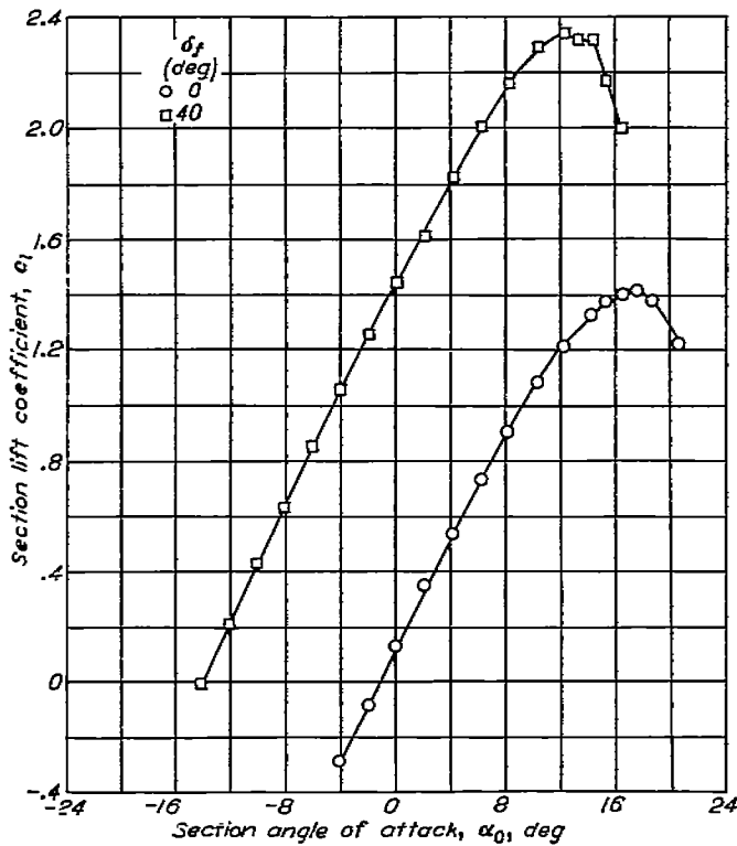
FIGURE 30.—Lift characteristics of an approximate NACA 66(218)-216 airfoil section equipped with a 0.25c slotted flap. R=6.0 \times 10^6 .
