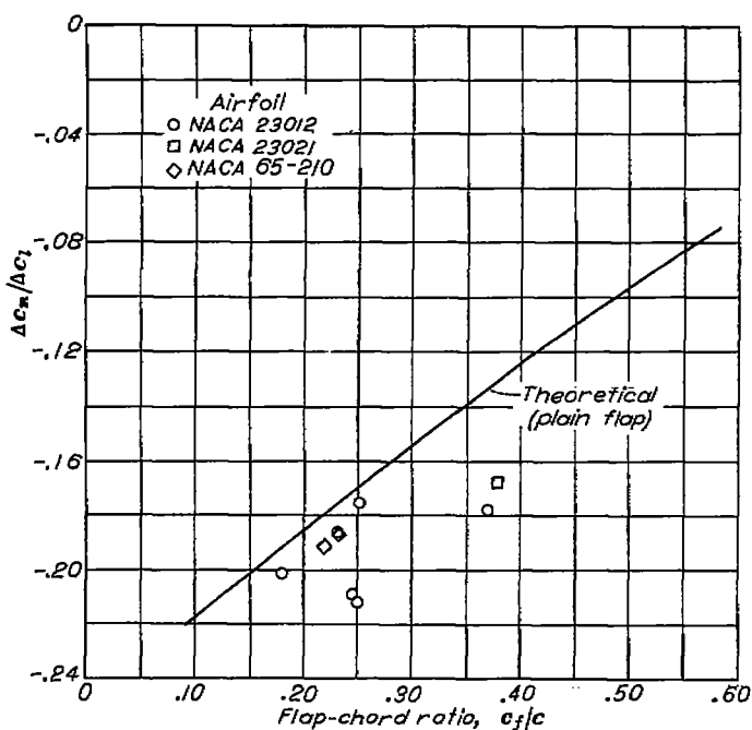
FIGURE 39.—Variation of ratio of increment of section pitching-moment coefficient to increment of section lift coefficient with flap-chord ratio for several airfoil sections with slotted flaps. \alpha_0=0^\circ . (All coefficients based on total chord with flap extended.)
