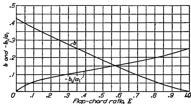
FIGURE 2.—Values of factors b and -b_1/a_1 in equation for hinge-moment coefficients. Reference 3.
