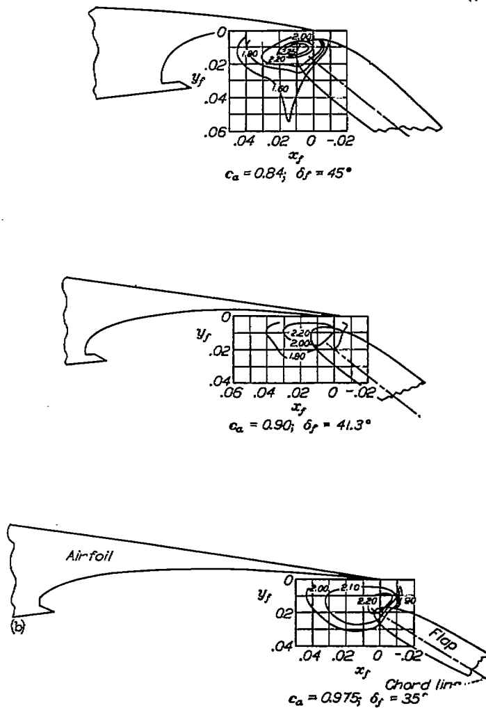
(b) NACA 65-210 airfoil with 0.25c slotted flap and three slot-lip locations. R=2.4 \times 10^6 ; reference 29.
