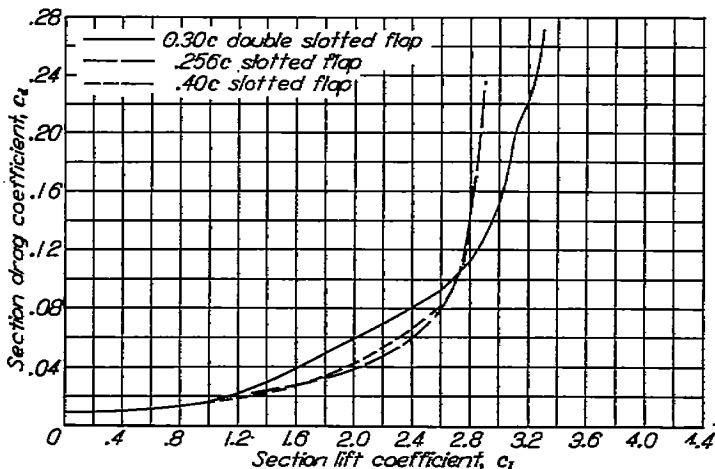
FIGURE 45.—Comparison of envelope polars for an NACA 23012 airfoil equipped with a double slotted flap and two sizes of single slotted flaps. R=3.5 \times 10^6 ; reference 41.
