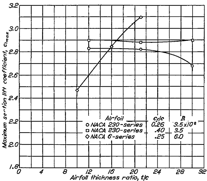
FIGURE 32.—Effect of airfoil thickness ratio on section maximum lift coefficients of airfoils equipped with single slotted flaps.
