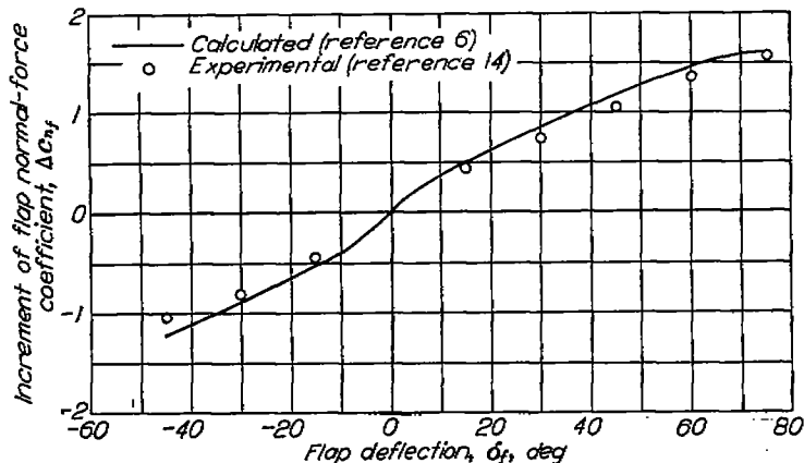
FIGURE 12.—Variation of flap normal-force coefficient with flap deflection. NACA 23012 airfoil; 0.20c plain flap; \alpha_i=0^\circ .
