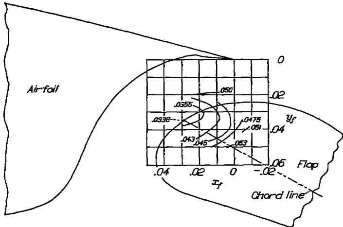
FIGURE 36.—Contours of flap position for various section drag coefficients for the NACA 66,2-216, \alpha=0.6 airfoil equipped with a 0.25c slotted flap. \delta_f=30^\circ ; c_f=2.6 ; R=5.1 \times 10^6 ; reference 35.
