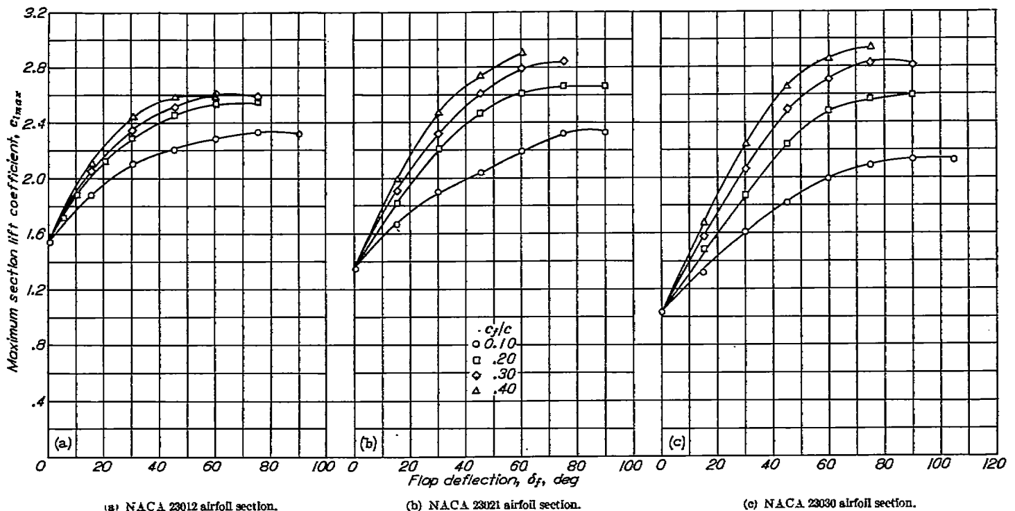
FIGURE 14.—Variation of maximum section lift coefficient with flap deflection for three NACA 230-series airfoils equipped with split flaps of various sizes. R=3.5 \times 10^6 ; reference 15.
