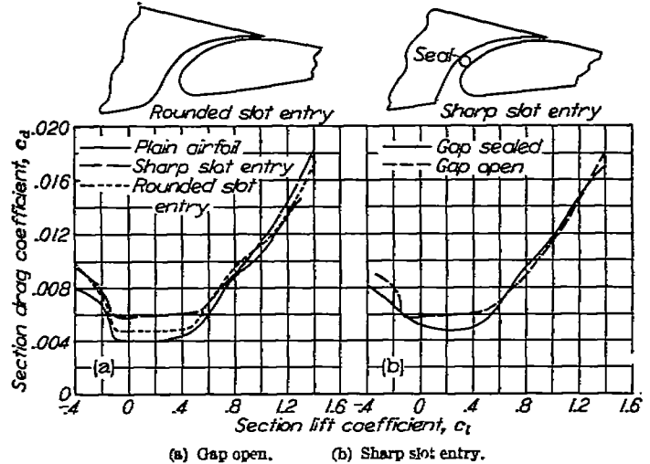
FIGURE 37.—Effect of slot opening and gap seal on drag coefficient of an NACA 65(216)-3(16.5) (approx.) airfoil equipped with a 0.25c slotted flap. R=6.0 \times 10^6
