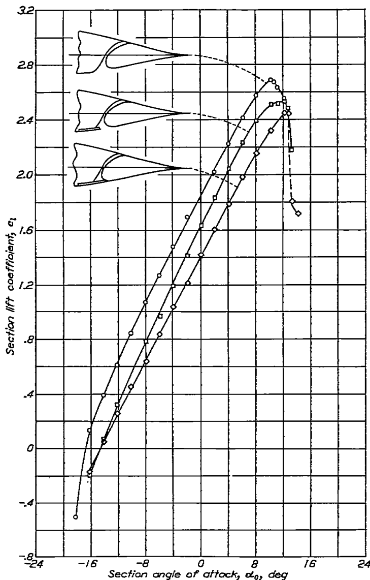
FIGURE 28.—Effect of slot-entry-skirt extension on section lift characteristics of an NACA 66,2-116, \alpha = 0.6 airfoil equipped with a 0.25c slotted flap deflected 45°. R = 6.0 \times 10^6 ; reference 34.
