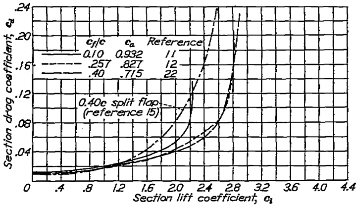
FIGURE 34.—Effect of flap size on envelope drag polars for an NACA 23012 airfoil equipped with single slotted flaps. R=3.5 \times 10^6 .
