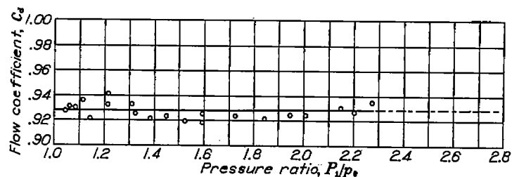
FIGURE 6.—Variation in flow coefficient with pressure ratio for discharge from straight pipes.
