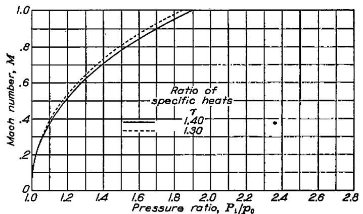
FIGURE 3.—Comparison of Mach number for two values of ratio of specific heats over range of pressure ratios. ( \gamma for model nozzles, approximately 1.40; \gamma for full-scale nozzles, 1.30 to 1.40.)
