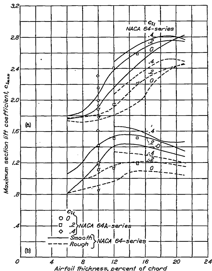
(a) Airfoil with simulated split flap deflected 60^\circ . (b) Plain airfoil.
