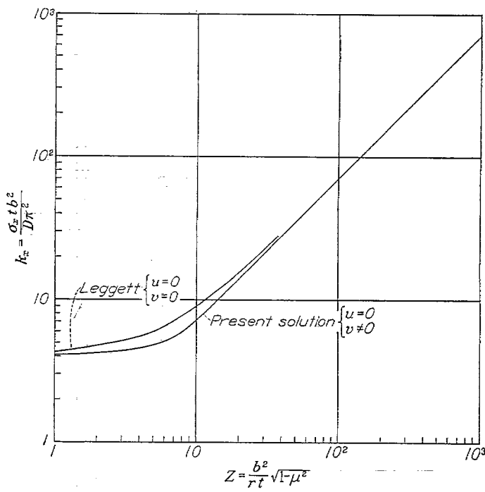
FIGURE 10.—Comparison of the present solution for the buckling under axial compression of a curved strip infinitely long in the axial direction, with solution found by Leggett (reference 8).
