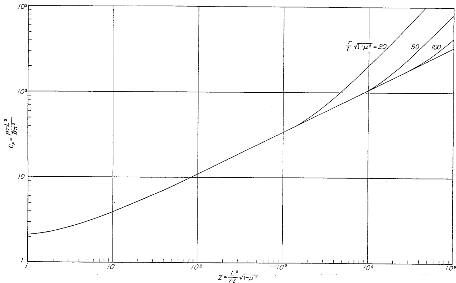
FIGURE 4.—Theoretical solution for hydrostatic pressure under which simply supported cylinders buckle.
