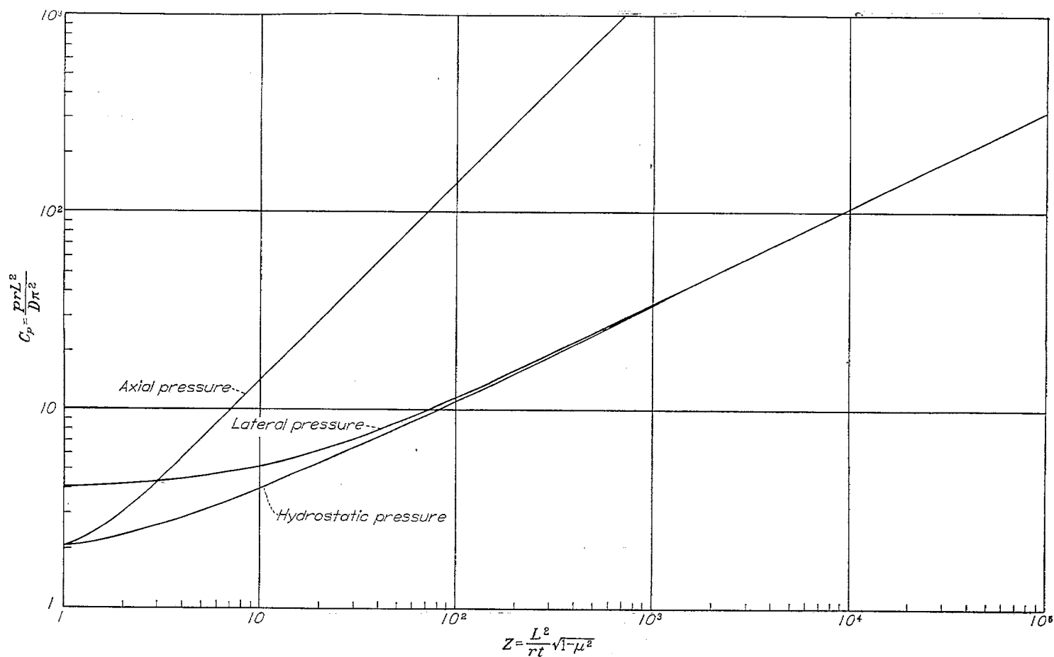
FIGURE 5.—Comparison of solution for buckling of simply supported cylinders under hydrostatic pressure with solutions for buckling under axial pressure alone and lateral pressure alone.
