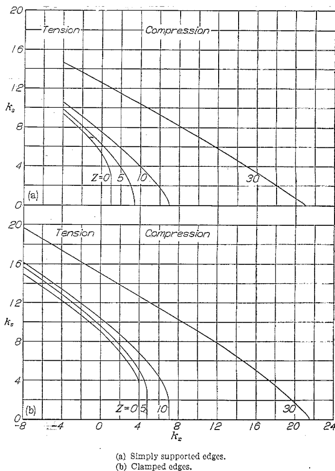
FIGURE 15.—Critical combinations of shear-stress and direct-axial-stress coefficients for cylinders. (Fig. 1 of reference 23.)
