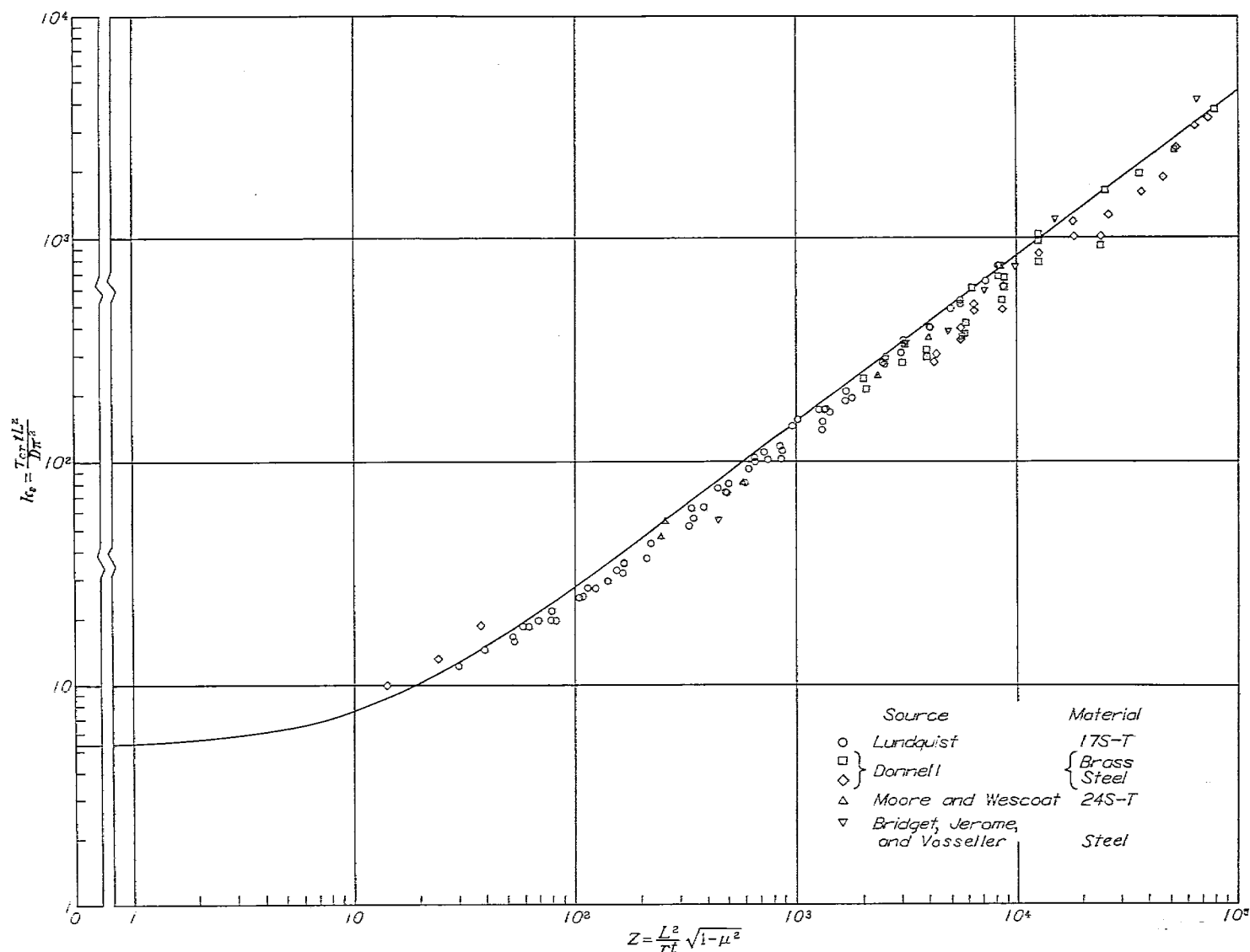
FIGURE 8.—Comparison of theoretical solution for critical shear stress of simply supported cylinders in torsion with experimental ultimate stresses. (Lundquist's data are from reference 10, Donnell's data are from reference 4, Moore and Wescoat's data are from reference 16, and Bridget, Jerome, and Vosseller's data are from reference 17.)
