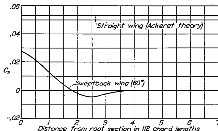
FIGURE 11.—Variation of drag coefficient with distance from root section for wings of biconvex section. M=1.4 ; \xi=10 percent.
