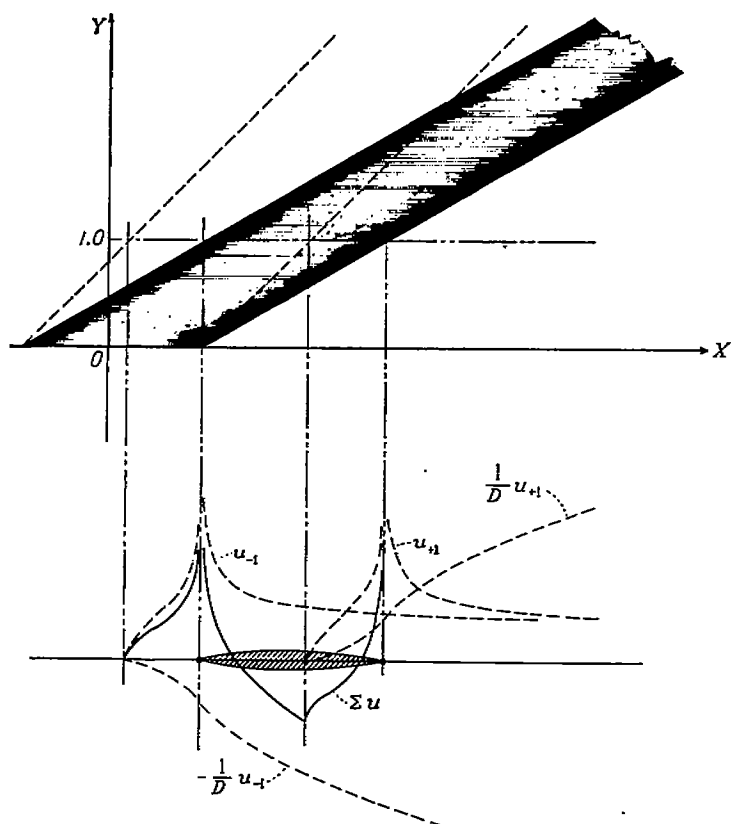
FIGURE 9.—Pressure distribution over wing of biconvex section. \frac{\Delta p}{q} = \frac{2\pi u}{\gamma} .
