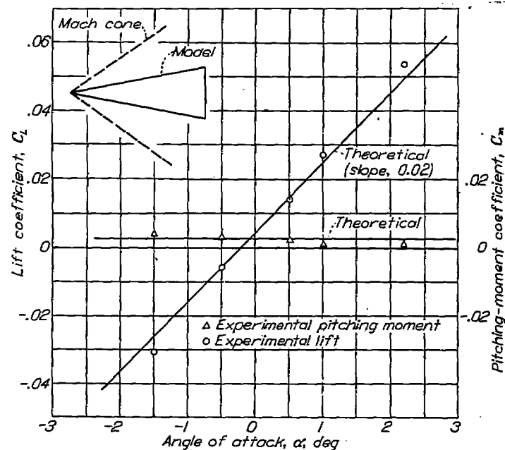
FIGURE 10.—Test of triangular airfoil in Langley model supersonic tunnel. Mach number, 1.75; Reynolds number, 1,600,000.
