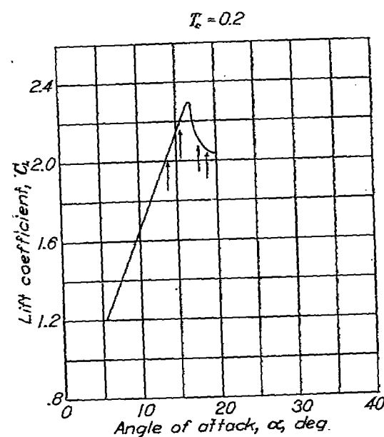
FIGURE 8.—Effect of propeller slipstream on the stalling characteristics of airplane 6. Airplane in service condition; \beta = 50^\circ ; approximate test velocity, 60 miles per hour.
