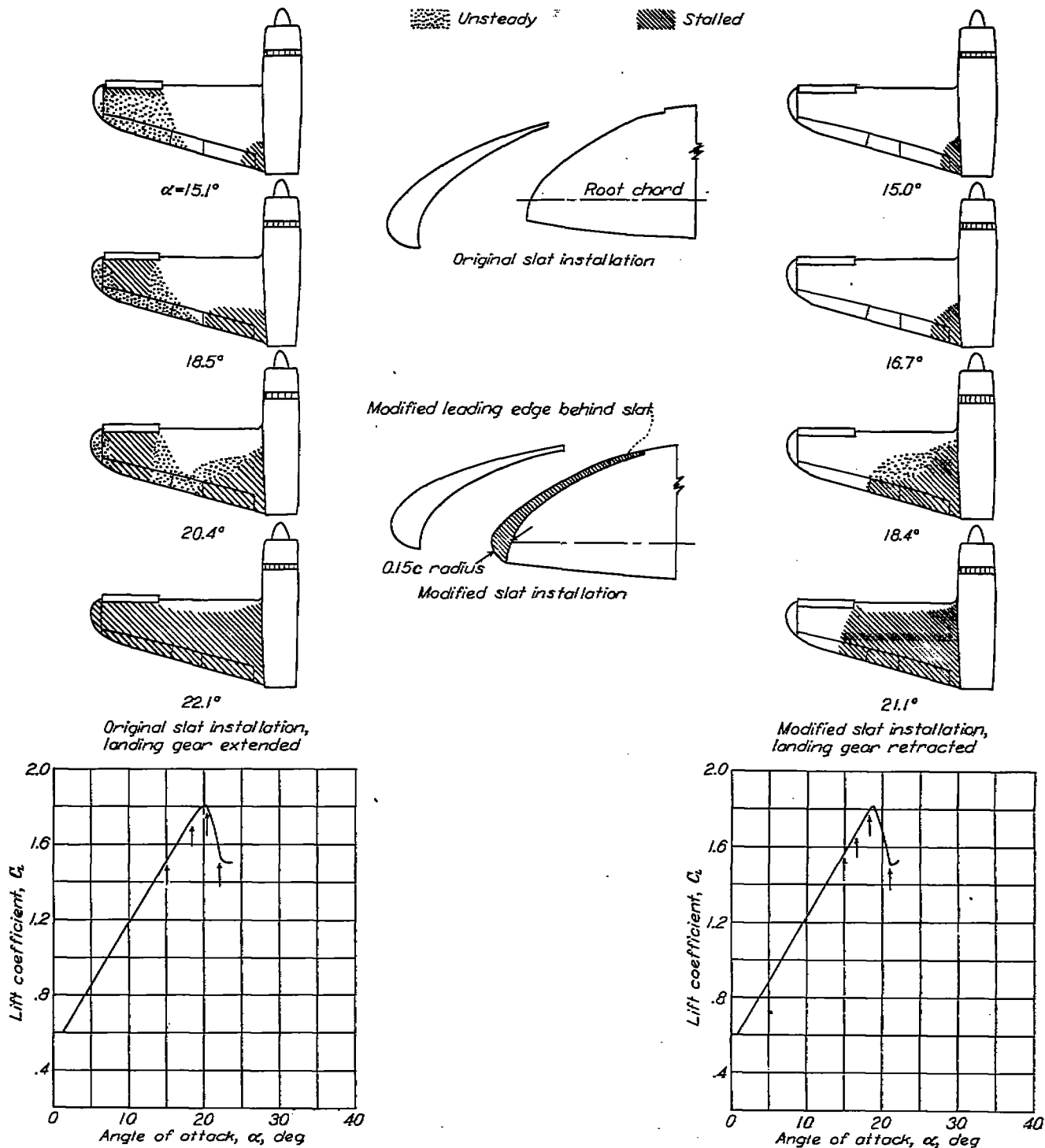
FIGURE 30.—Effect of slat installation on the stalling characteristics of airplane 7. Propeller and tail surfaces removed; \beta_r = 60^\circ ; approximate test velocity, 60 miles per hour.
