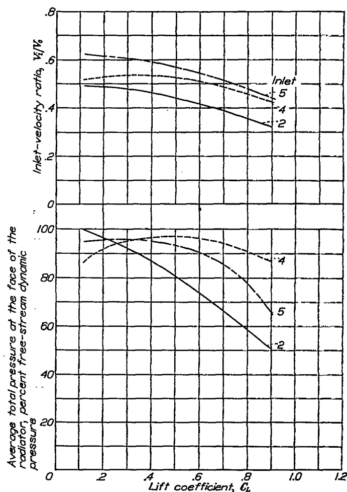
FIGURE 35.—Effect of lift coefficient on the average total pressure at the front of the radiator behind inlets 2, 4, and 5. Propeller removed; \delta_f = 0^\circ ; bottom outlet; airplane 16.
