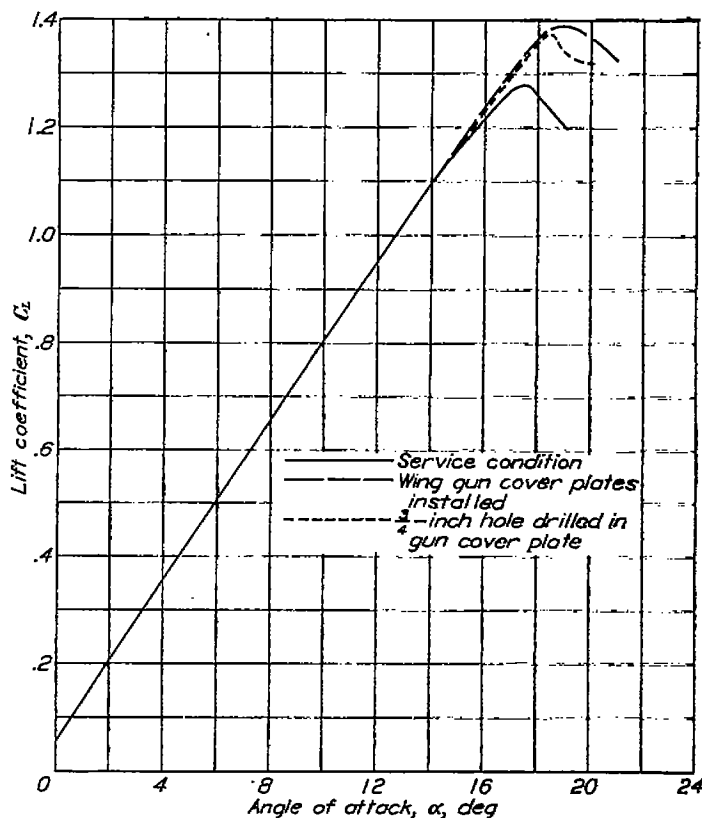
FIGURE 29.—Effect of wing gun ports on the C_{L_{max}} of airplane 1. \delta_T = 0^\circ .
