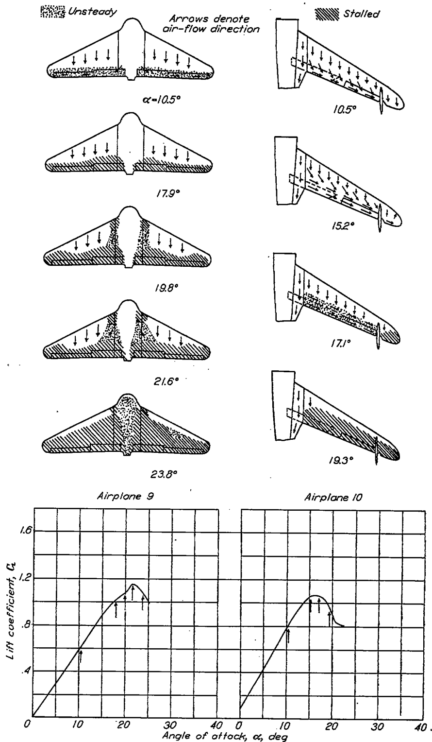
FIGURE 5.—Stall progressions for airplanes with sweptback wings. Propeller removed; \delta_1 = 0^\circ ; approximate test velocity, 60 miles per hour.
