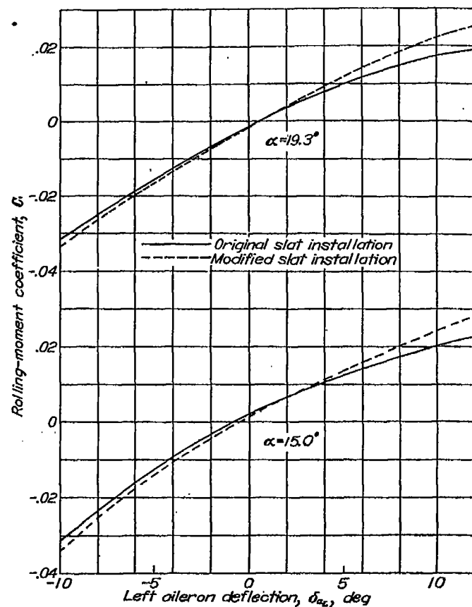
FIGURE 31.—Effect of slat installation on the aileron control characteristics of airplane 7. Both ailerons deflected; \delta_l = 60^\circ .
