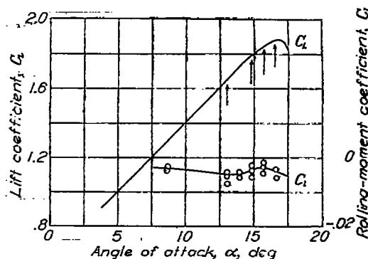
FIGURE 10.—Effect on the stalling characteristics and rolling moments of installing a sharp leading edge on the right wing of airplane 6. Propeller operating; T_o = 0.2 ; \delta_r = 50^\circ ; approximate test velocity, 60 miles per hour.
