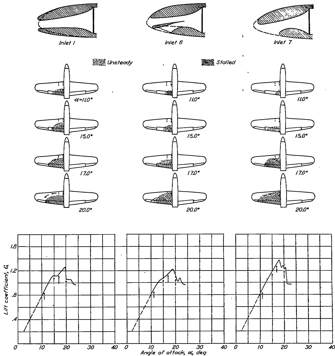
FIGURE 36.—Effect of wing-duct-inlet shape on the stalling characteristics of airplane 16. Inlet and tufts on left wing only. Propeller removed; \delta_f = 0^\circ ; approximate test velocity, 80 miles per hour. Outlet at bottom of wing
