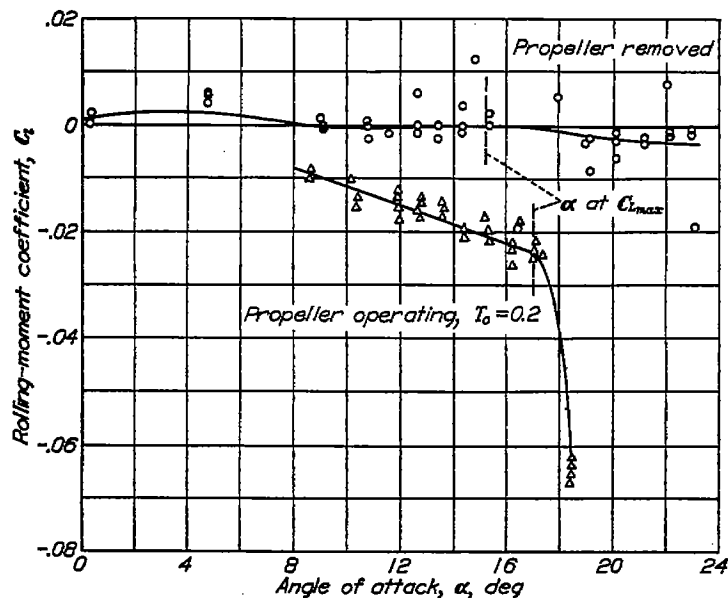
FIGURE 9.—Effect of propeller operation on the rolling moments of airplane 6. Airplane in service condition; \delta_r = 50^\circ ; approximate test velocity, 60 miles per hour.
