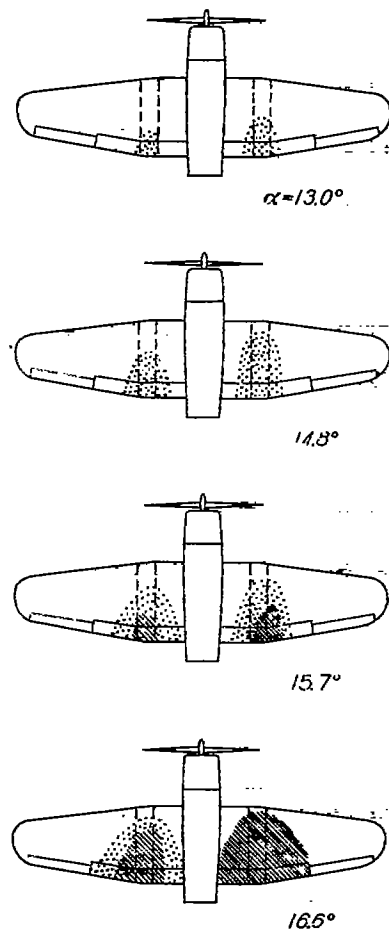
FIGURE 10.—Effect on the stalling characteristics and rolling moments of installing a sharp leading edge on the right wing of airplane 6. Propeller operating; T_o = 0.2 ; \delta_r = 50^\circ ; approximate test velocity, 60 miles per hour.
