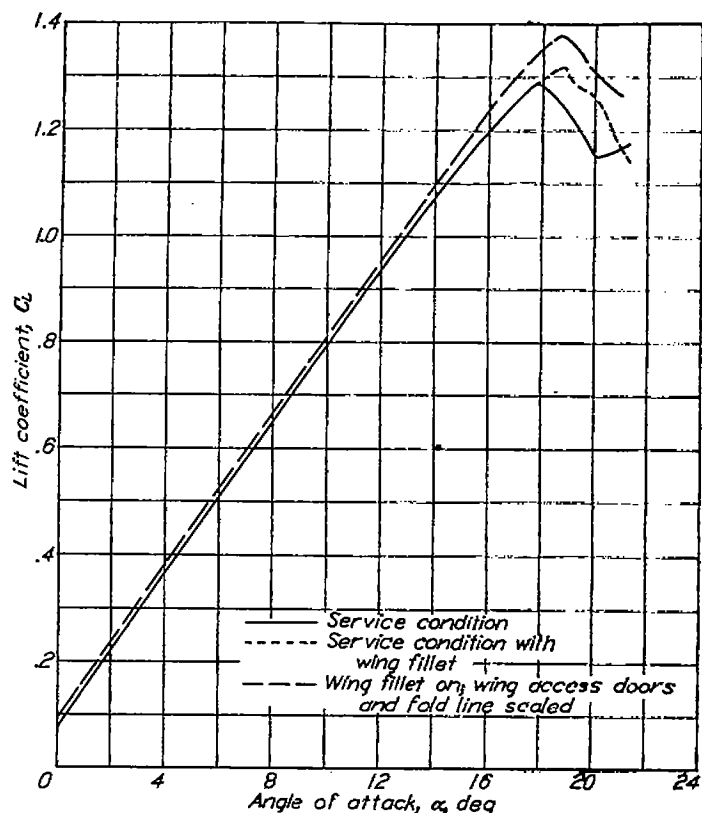
FIGURE 15.—Effect of wing surface roughness on the C_{L_{max}} of airplane 5. Propeller removed; \delta_f = 0^\circ ; approximate test velocity, 60 miles per hour.
