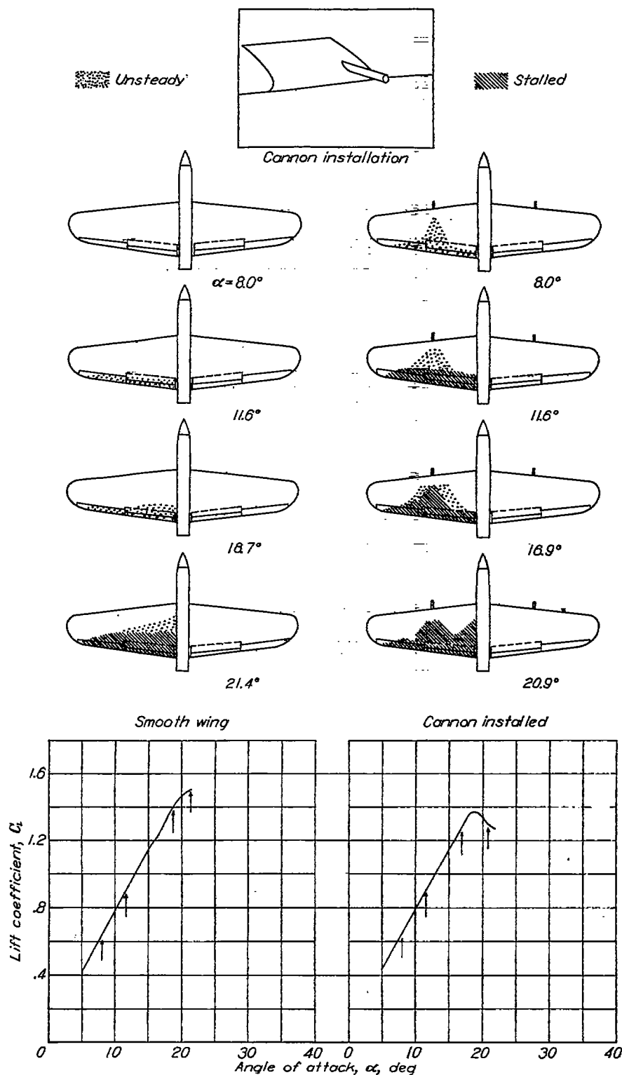
FIGURE 26.—Effect on stall and maximum lift of installing a 27-millimeter-cannon mock-up on the leading edge of the wing of airplane 4. \delta_f = 0^\circ ; approximate test, velocity 80 miles per hour. Tufts on left wing only.
