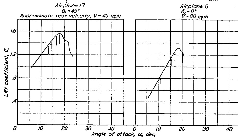
FIGURE 38.—Effect of airspeed-head location on stalling characteristics. Propellers removed.
