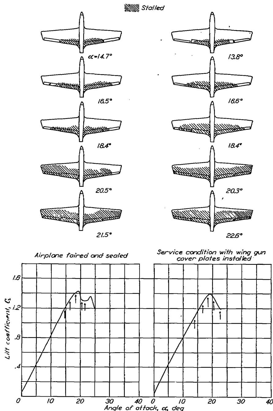
FIGURE 16.—Effect of wing surface roughness on the stalling characteristics of airplane 1. Propeller removed; \delta_r=0^\circ ; approximate test velocity, 60 miles per hour.
