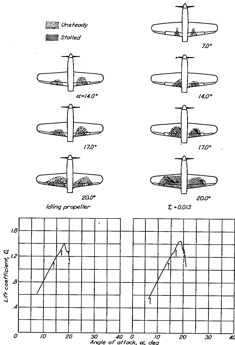
FIGURE 11.—Effect of propeller slipstream on the stalling characteristics of airplane 16. \beta_1=0^\circ ; approximate test velocity, 80 miles per hour.
