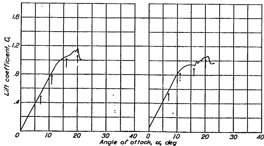
FIGURE 37.—Effect of wing-duct-outlet location on the stalling characteristics of airplane 18. Propeller removed; \delta_r = 0^\circ ; approximate test velocity, 60 miles per hour.
