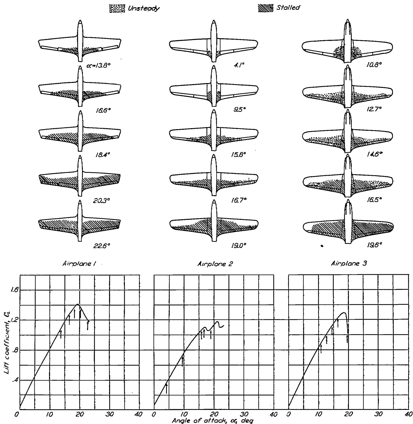
FIGURE 4.—Stall progressions for three present-day airplanes having low-drag wings. Complete airplanes less propellers; \beta = 0^\circ ; approximate test velocity, 60 miles per hour.
