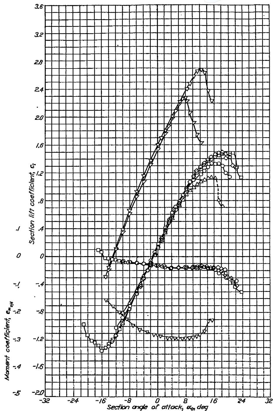
Aerodynamic characteristics of the NACA 653-218 airfoil section, 24-inch chord.
