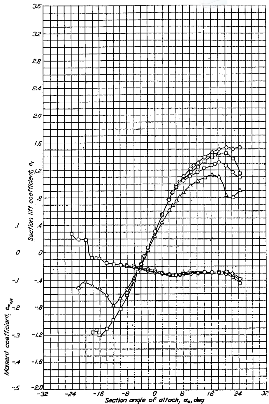
Aerodynamic characteristics of the NACA 65(421)-420 airfoil section, 24-inch chord.
