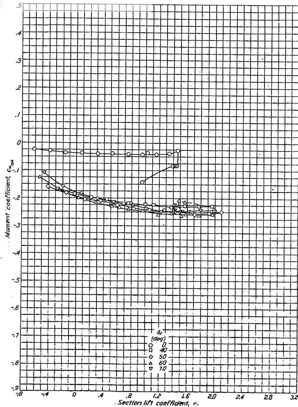
Lift and moment characteristics of the NACA 65-212 airfoil section with 0.20c split flap. R=6 \times 10^6 .
