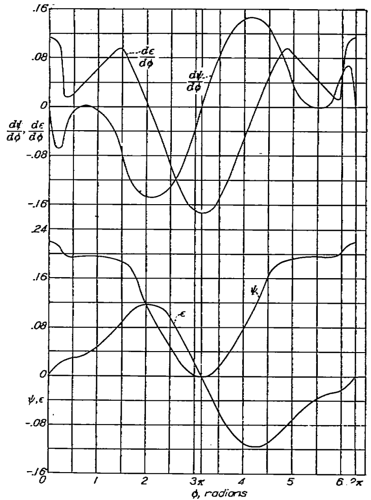
FIGURE 4.—Variation of airfoil parameters \psi , \epsilon , \frac{d\psi}{d\phi} , \frac{d\epsilon}{d\phi} with \phi for the NACA 64-018 airfoil section basic thickness form.
