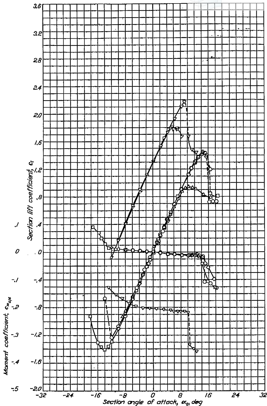
Aerodynamic characteristics of the NACA 64-012 airfoil section, 24-inch chord.
