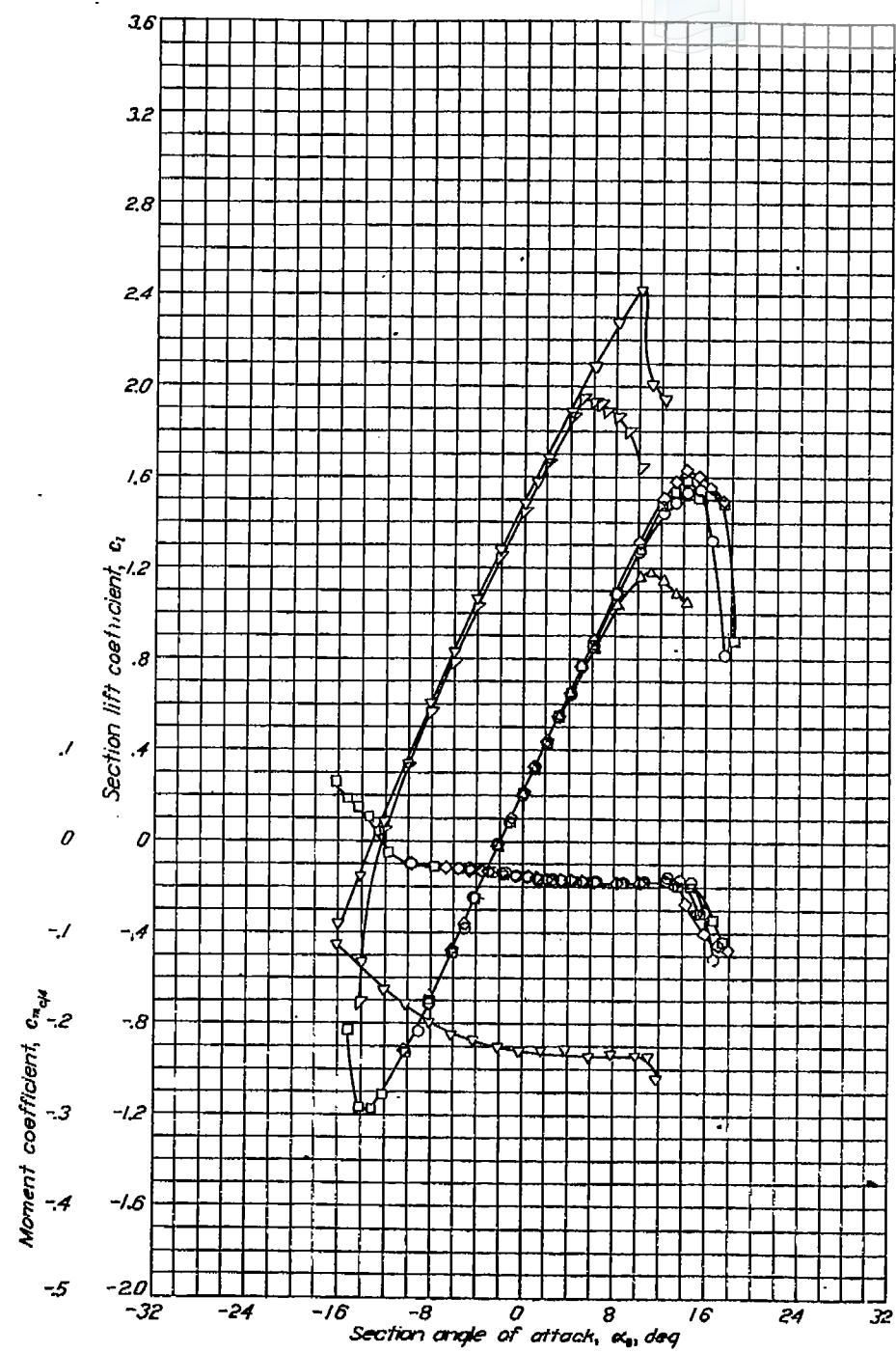
Aerodynamic characteristics of the NACA 631-212 airfoil section, 34-inch chord.
