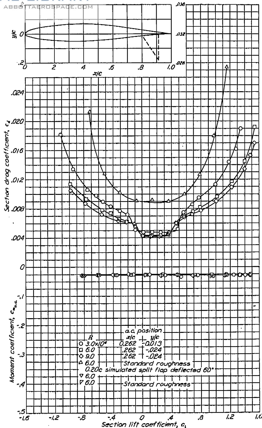
Aerodynamic characteristics of the NACA 64-212 airfoil section, 24-inch chord.
