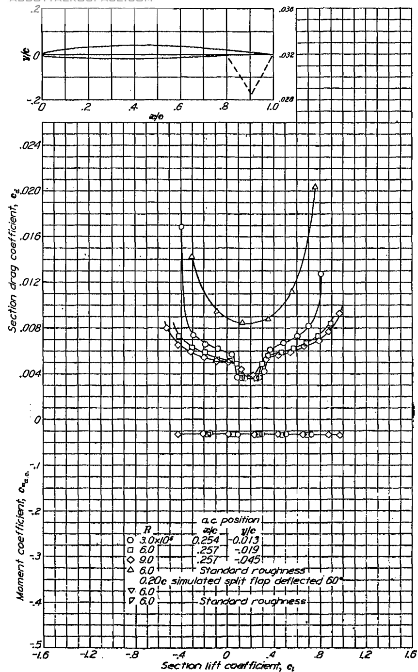
Aerodynamic characteristics of the NACA 65-206 airfoil section, 24-inch chord.
