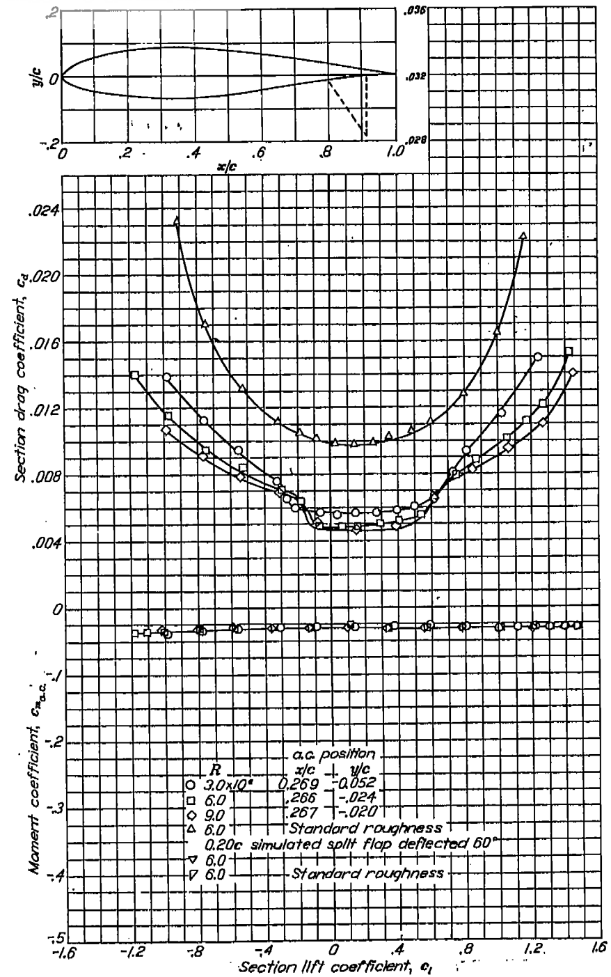
Aerodynamic characteristics of the NACA 63-215 airfoil section, 24-inch chord.
