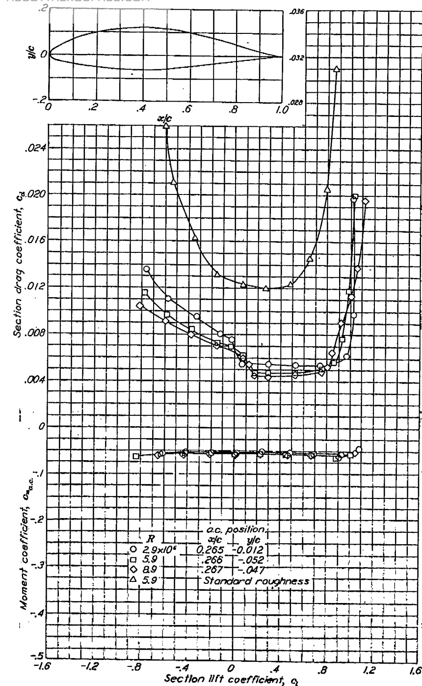
Aerodynamic characteristics of the NACA 65-118, \alpha=0.5 airfoil section, 24-inch chord.
