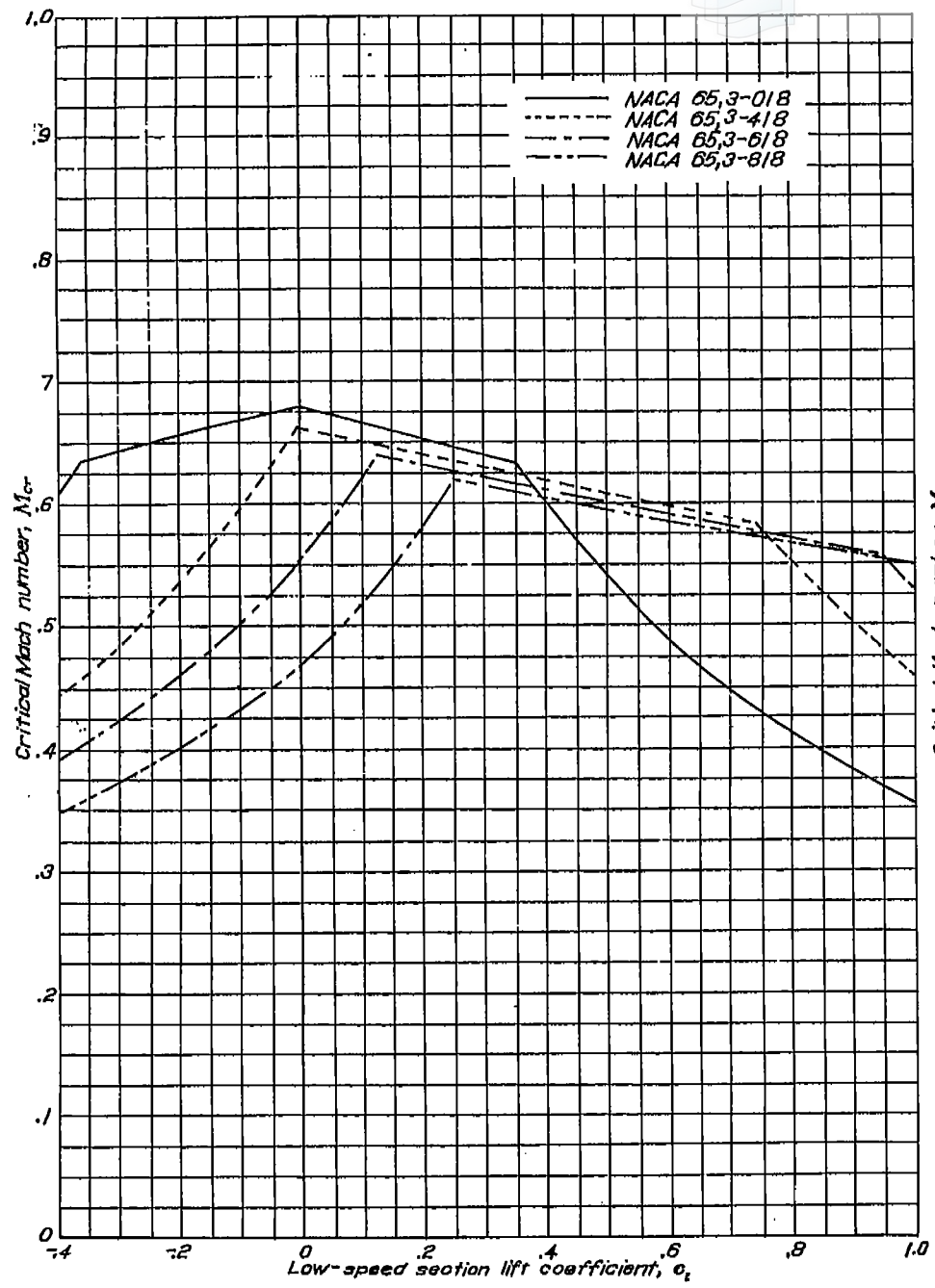
Variation of critical Mach number with low-speed section lift coefficient for several NACA 65-series airfoil sections with a thickness ratio of 0.18 and cambered for various design lift coefficients.
