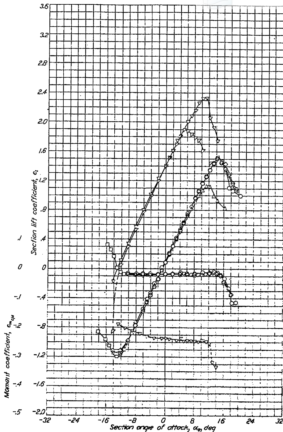
Aerodynamic characteristics of the NACA 1410 airfoil section, 24-inch chord.
