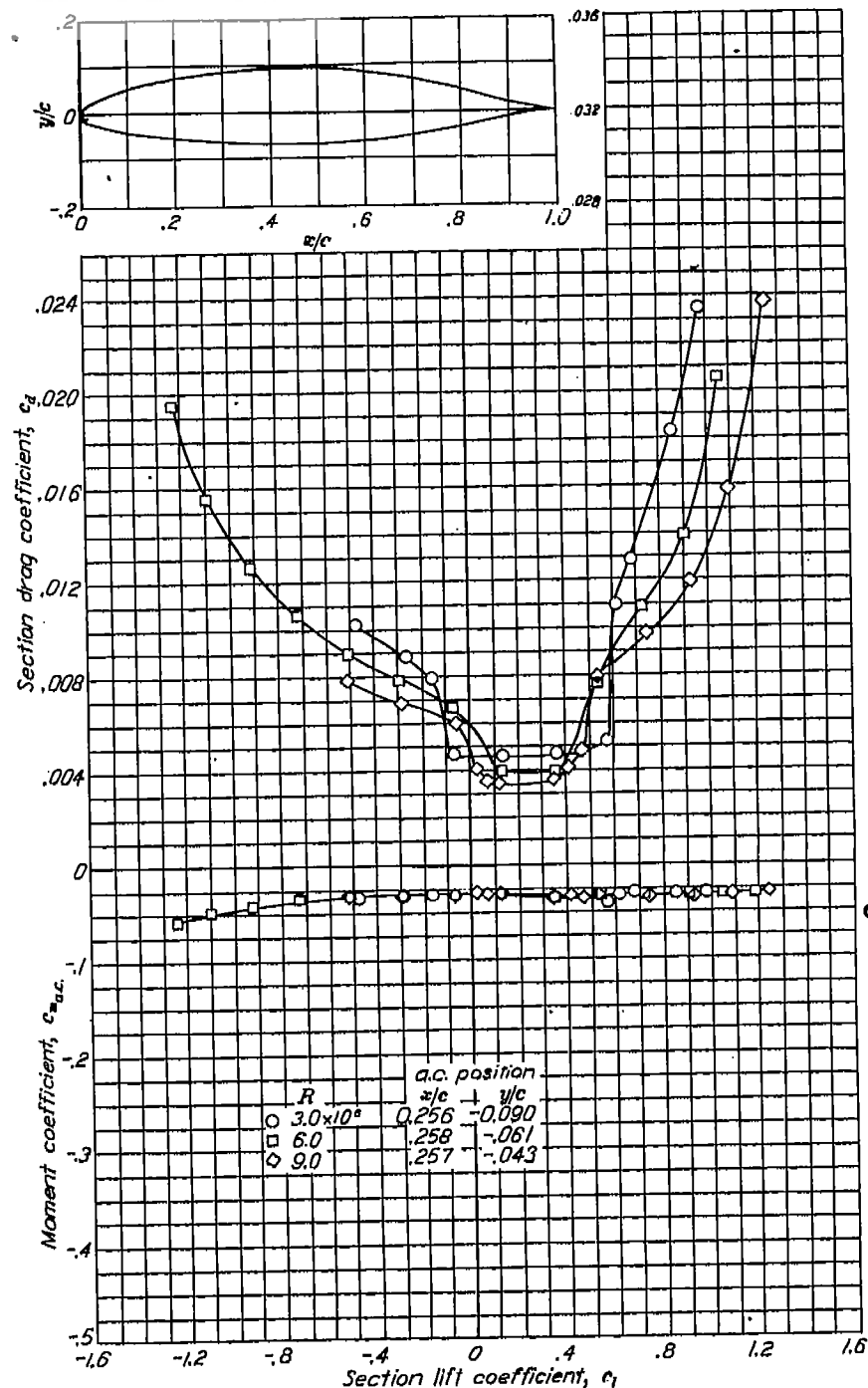
Aerodynamic characteristics of the NACA 66(215)-216, \alpha = 0.6 airfoil section, 24-inch chord.
