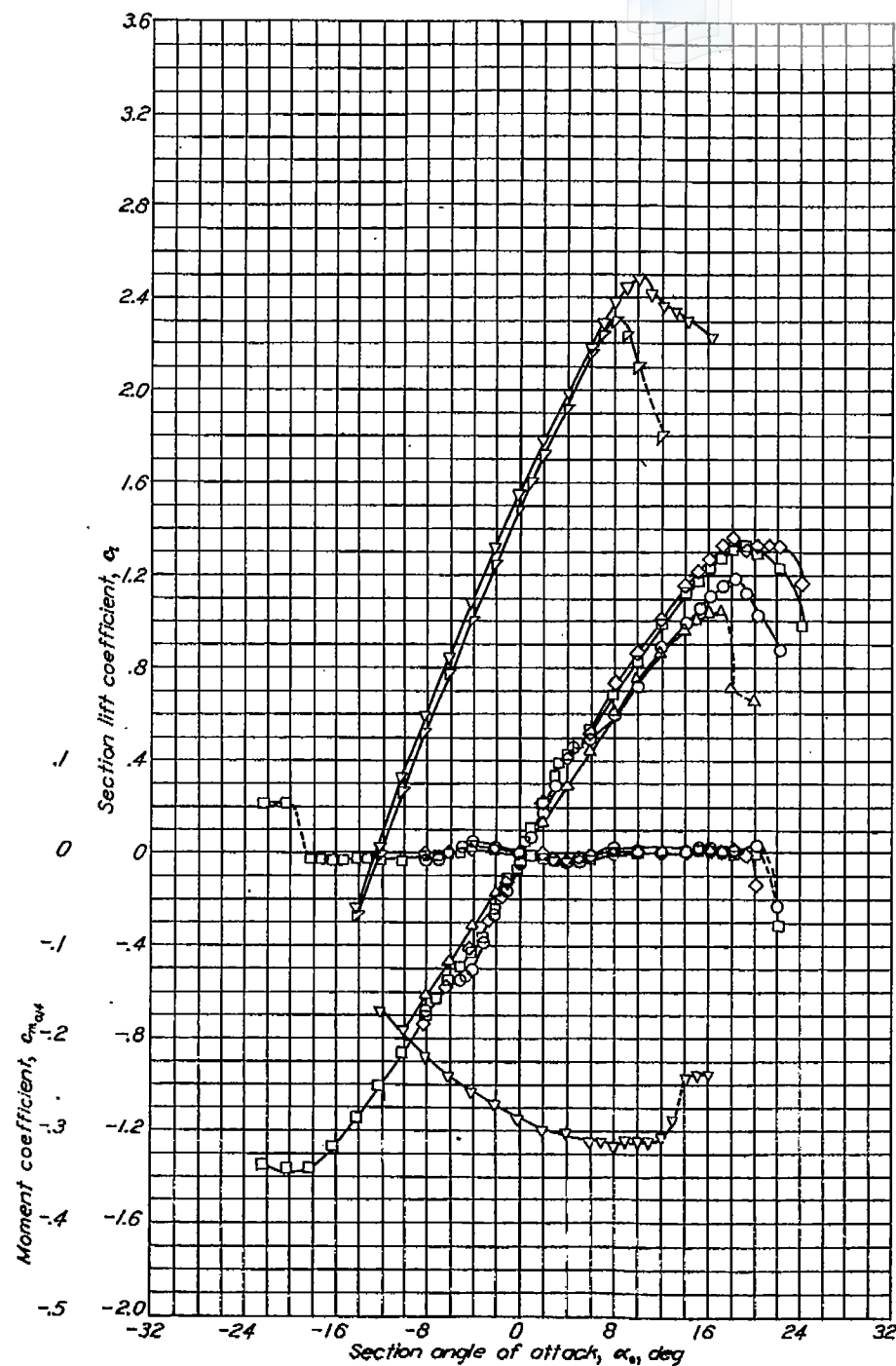
Aerodynamic characteristics of the NACA 66-021 airfoil section, 24-inch chord.
