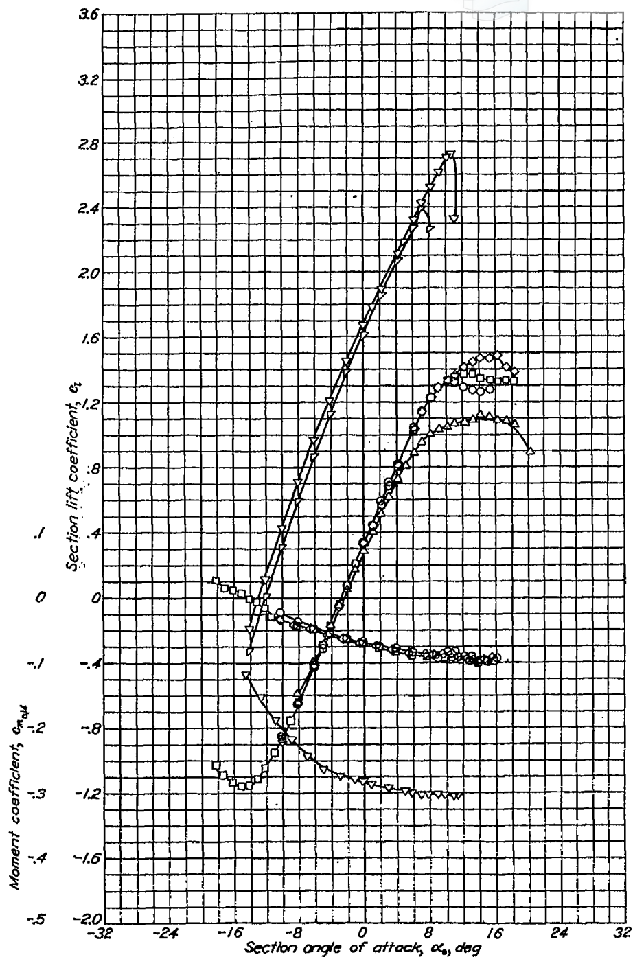
Aerodynamic characteristics of the NACA 634-421 airfoil section, 24-inch chord.
