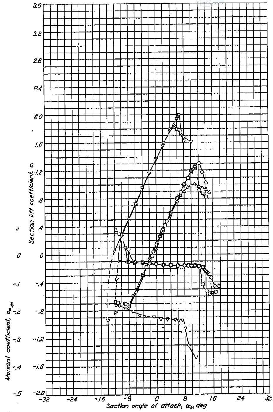
Aerodynamic characteristics of the NACA 65-209 airfoil section, 24-inch chord.
