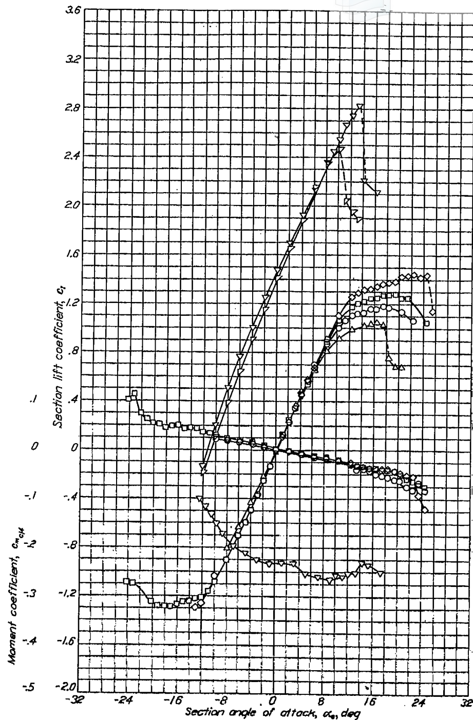
Aerodynamic characteristics of the NACA 64-021 airfoil section, 24-inch chord.
