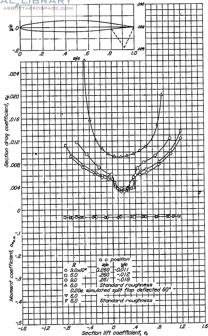
Aerodynamic characteristics of the NACA 66-210 airfoil section, 24-inch chord.
