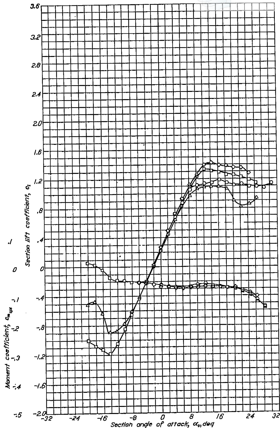
Aerodynamic characteristics of the NACA 63,4-420 airfoil section, 24-inch chord.
