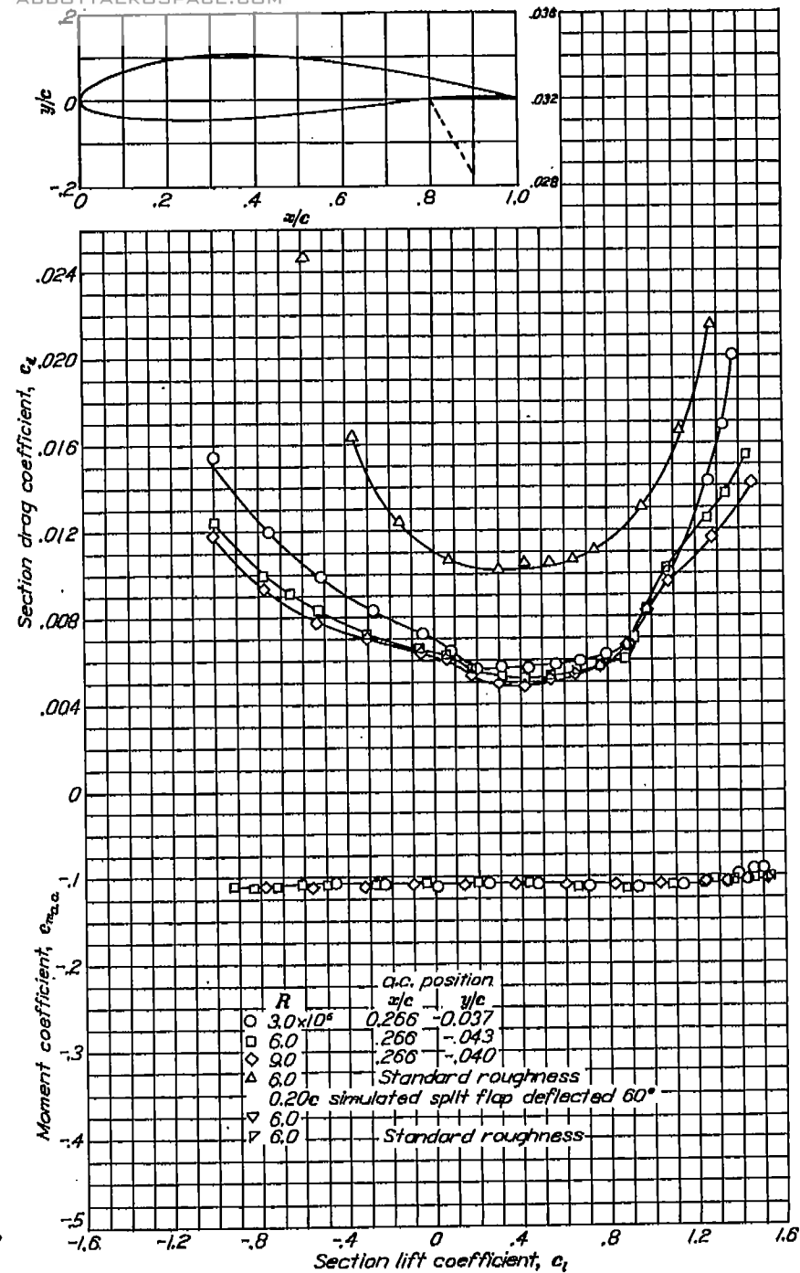
Aerodynamic characteristics of the NACA 63-615 airfoil section, 24-inch chord.
