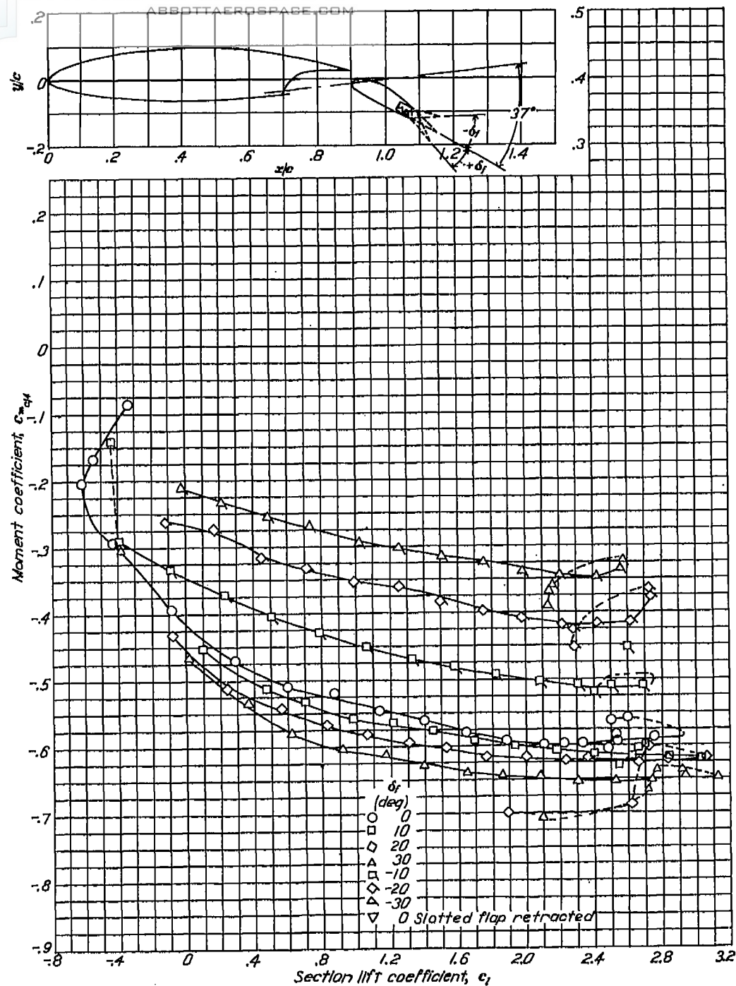
(g) Lift and moment characteristics. Slotted flap deflected 37^\circ ; R=6 \times 10^6 . NACA 66(215)-216, \alpha=0.6 airfoil section with 0.80c slotted and 0.10c plain flap.
