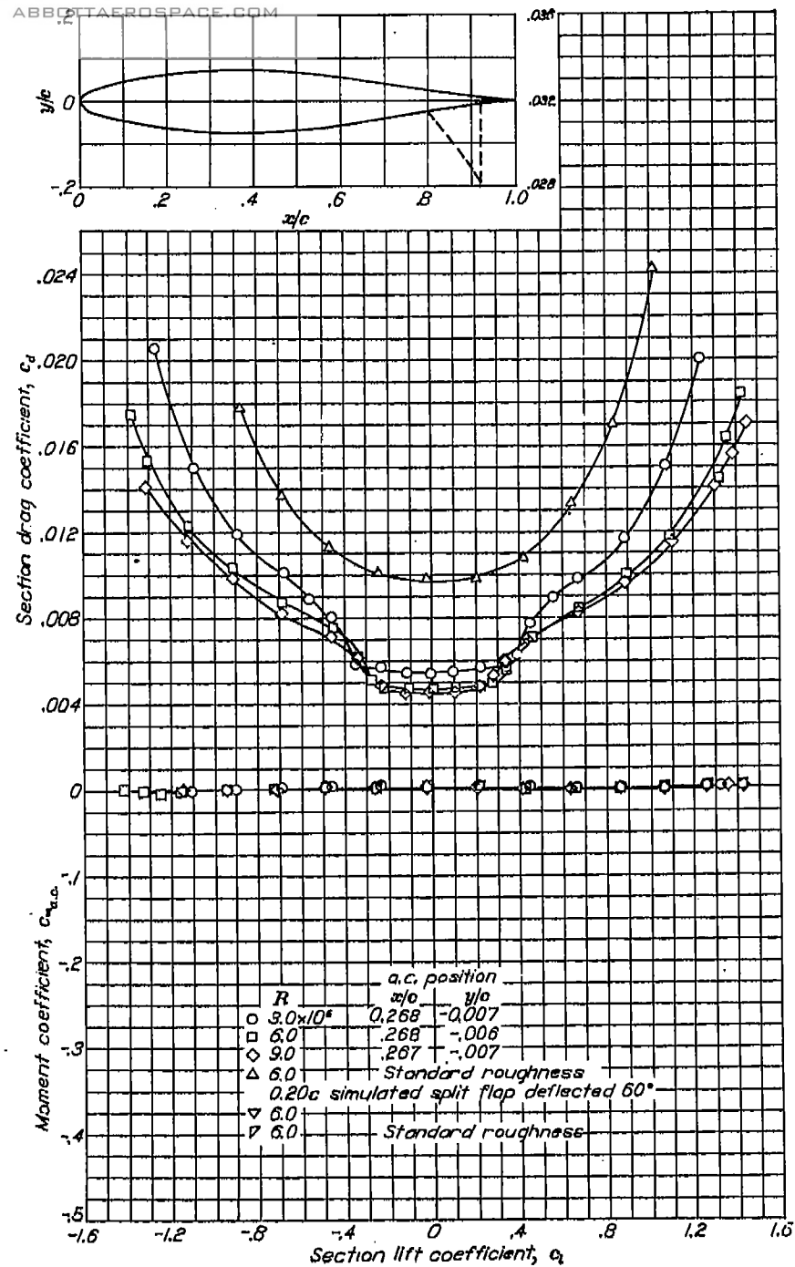
Aerodynamic characteristics of the NACA 64-015 airfoil section, 24-inch chord.
