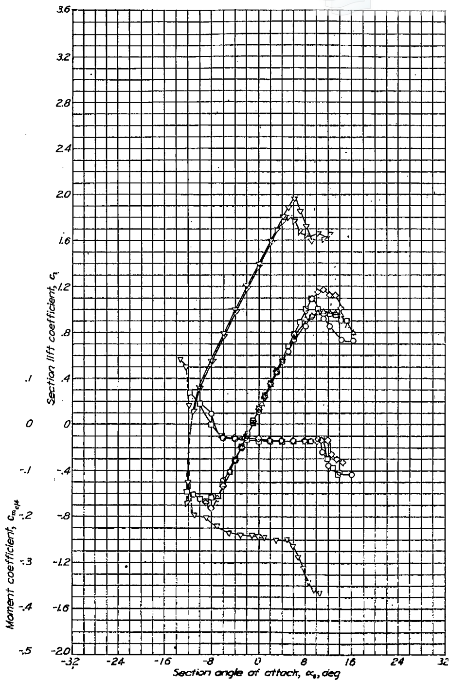
Aerodynamic characteristics of the NACA 66-209 airfoil section, 24-inch chord.
