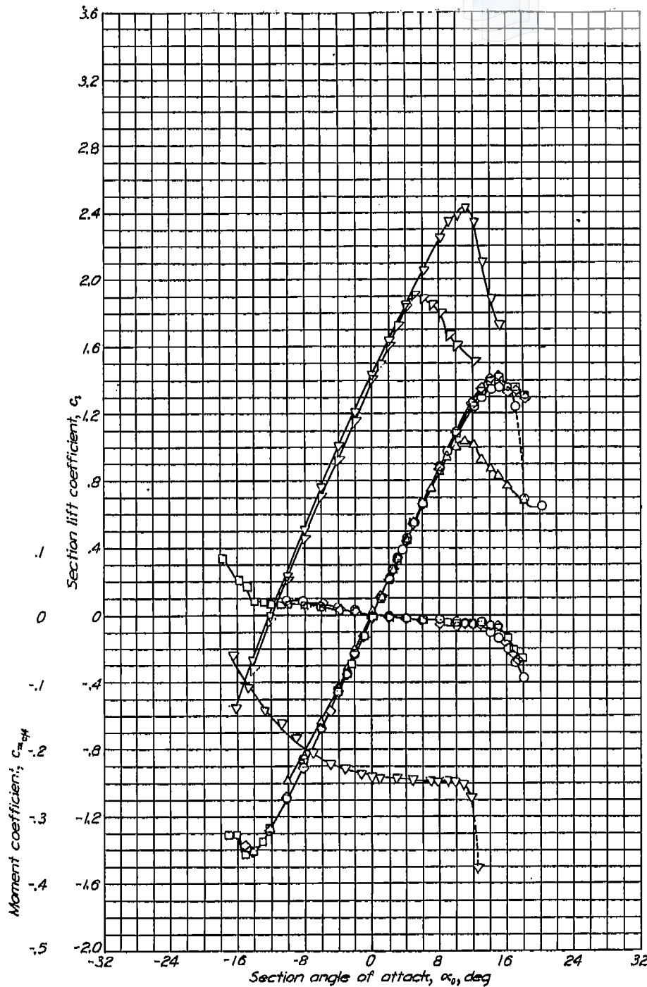
Aerodynamic characteristics of the NACA 65-015 airfoil section, 24-inch chord.
