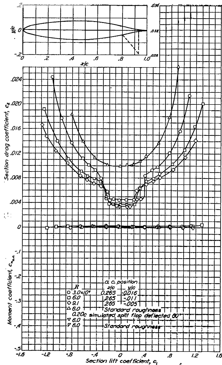
Aerodynamic characteristics of the NACA 662-015 airfoil section, 24-inch chord.
