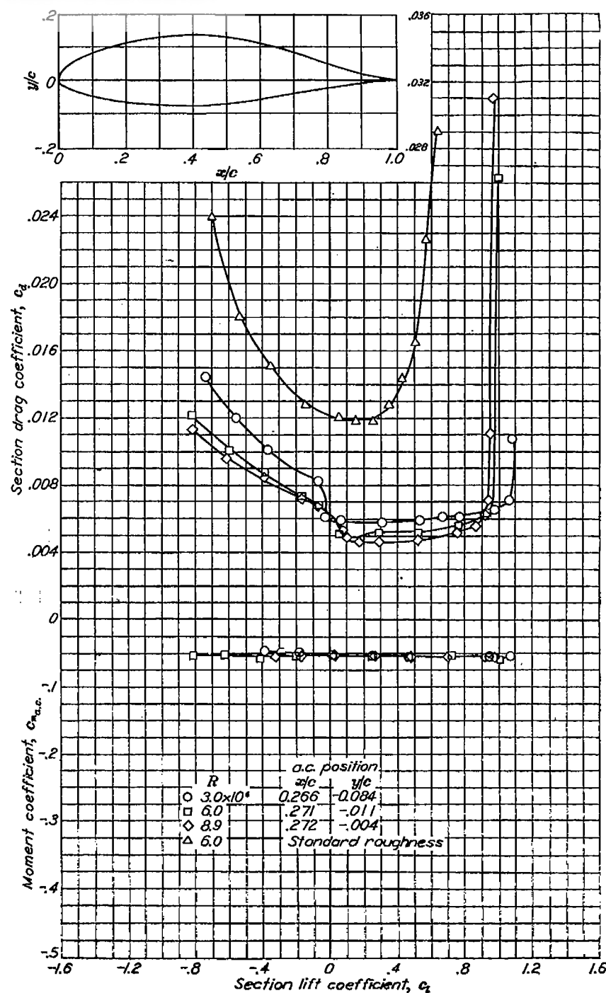
Aerodynamic characteristics of the NACA 65-121, \alpha=0.5 airfoil section, 24-inch chord.
