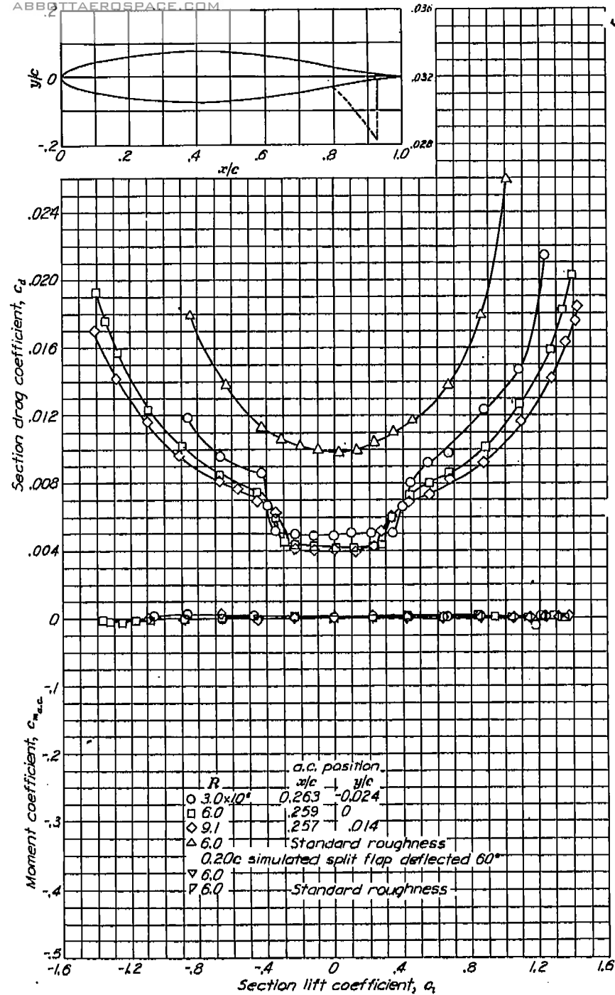
Aerodynamic characteristics of the NACA 65-015 airfoil section, 24-inch chord.
