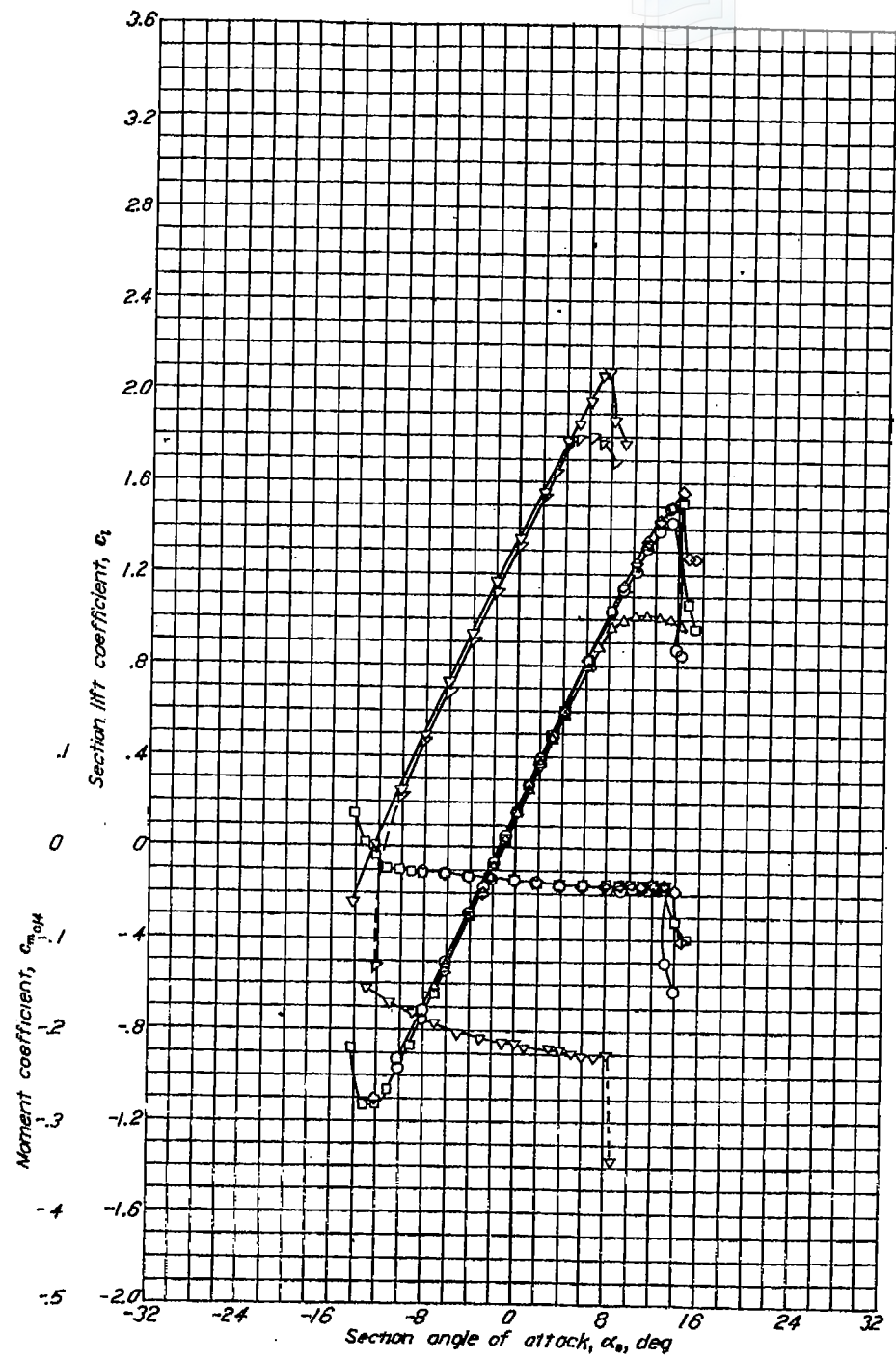
Aerodynamic characteristics of the NACA 63-210 airfoil section, 24-inch chord.
