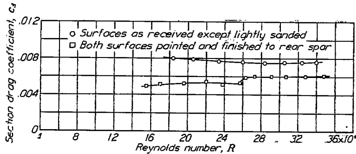
FIGURE 28.—Drag scale effect on 100-inch-chord practical-construction model of the NACA 65(216)-3(16.6) (approx.) airfoil section. c_l=0.2 (approx.).
