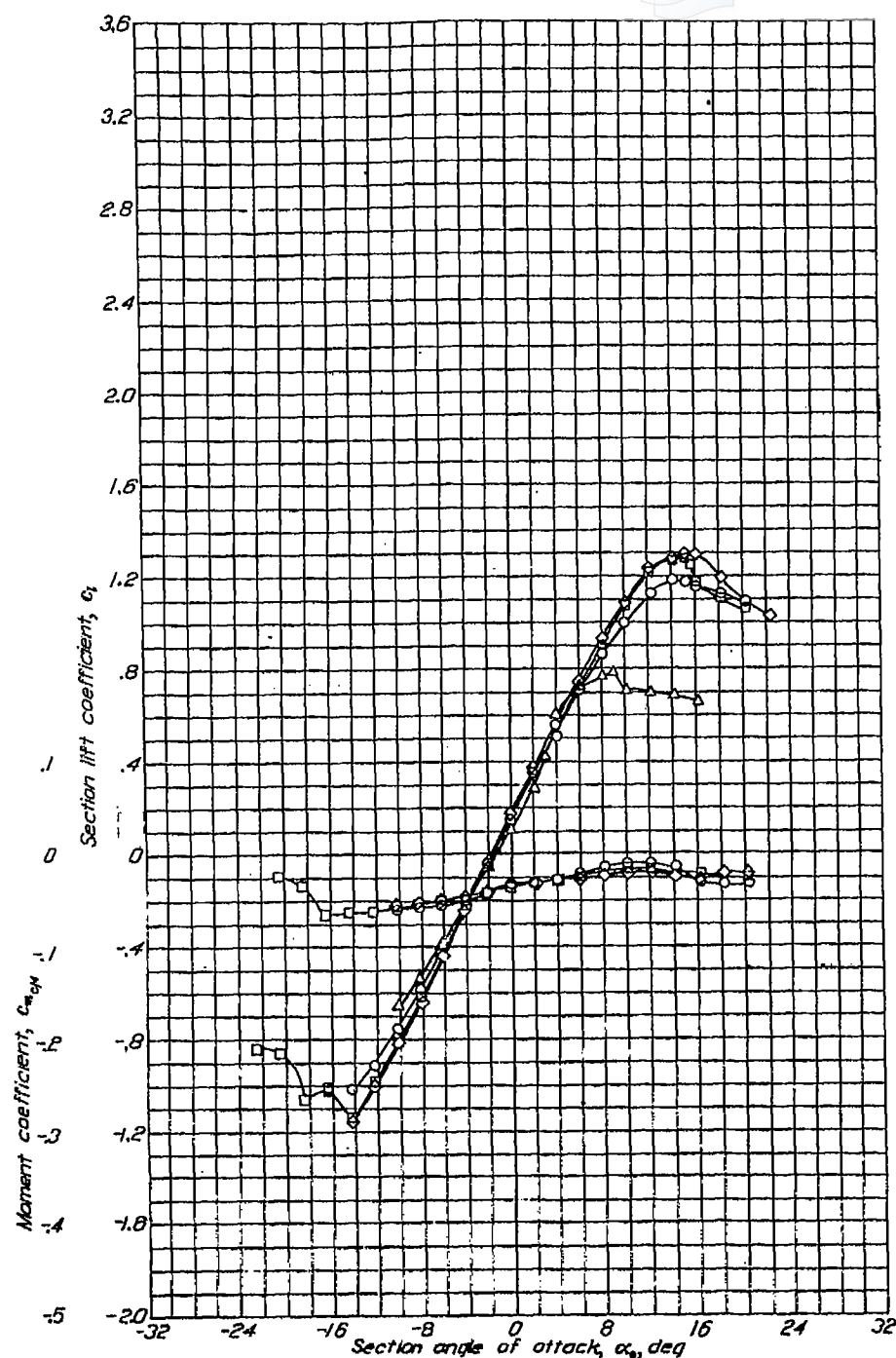
Aerodynamic characteristics of the NACA 2424 airfoil section, 24-inch chord.
