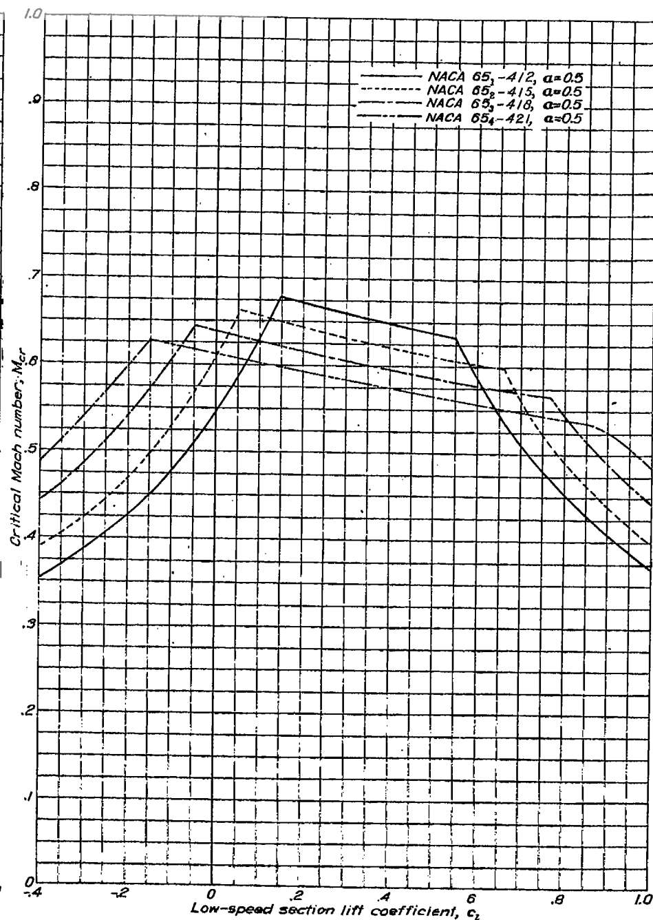
Variation of critical Mach number with low-speed section lift coefficient for several NACA 65-series airfoil sections with mean line of the type s=0.5 and cambered for a design lift coefficient of 0.4.
