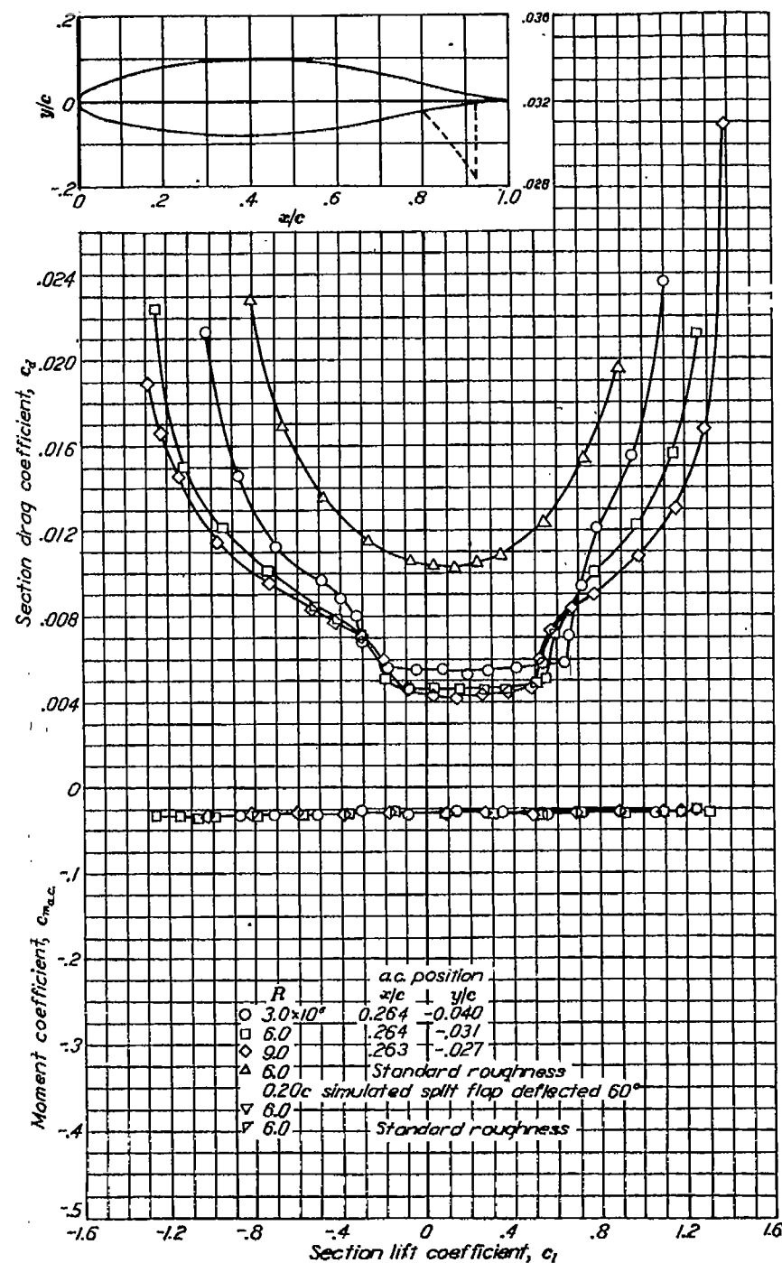
Aerodynamic characteristics of the NACA 653-218 airfoil section, 24-inch chord.
