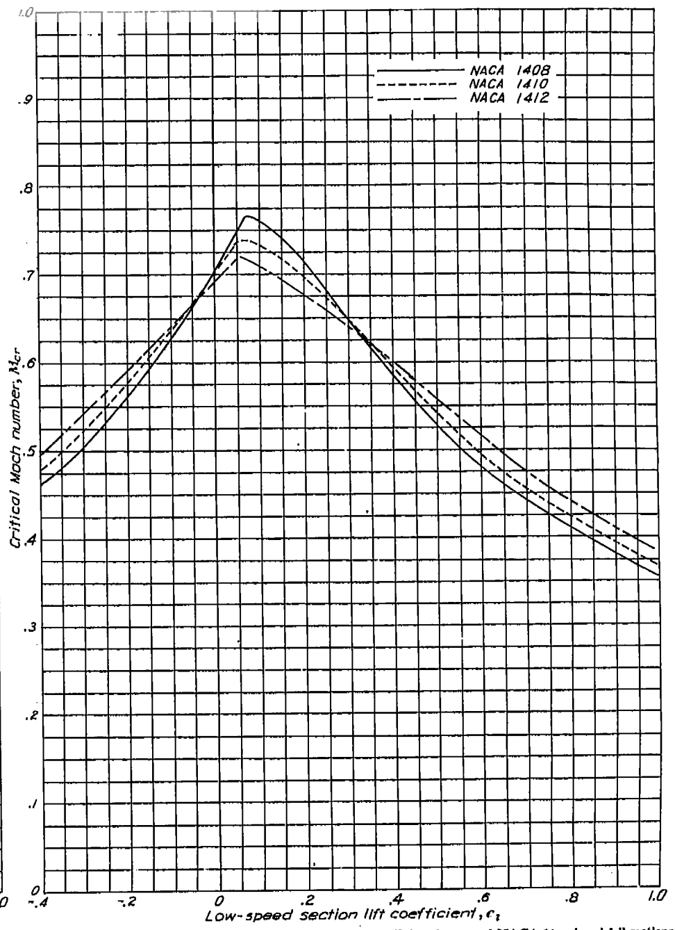
Variation of critical Mach number with low-speed section lift coefficient for several NACA 14-series airfoil sections of various thicknesses.
