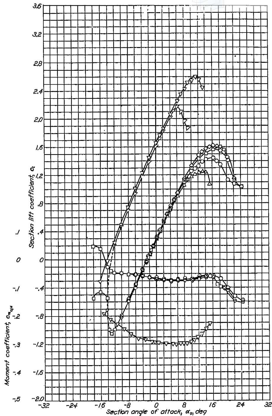
Aerodynamic characteristics of the NACA 65-415 airfoil section, 24-inch chord.
