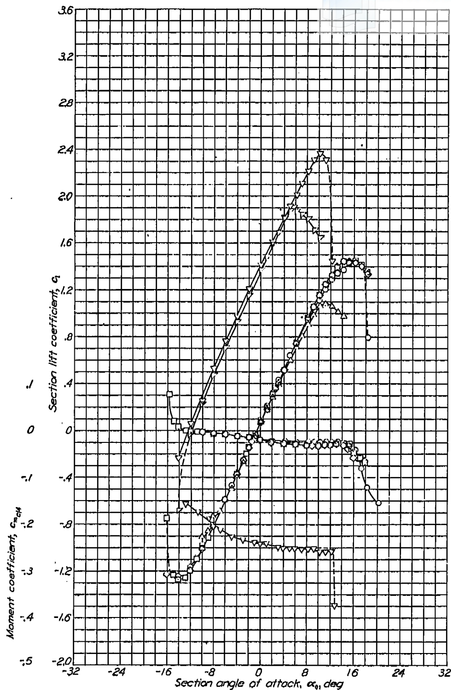
Aerodynamic characteristics of the NACA 65(11)-114 airfoil section, 24 inch chord.
