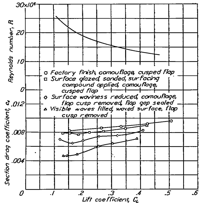
FIGURE 27.—Consolidated-Vultee flight measurements of the effect of wing surface condition on drag of an NACA 66(215)-1(14.5) wing section.
