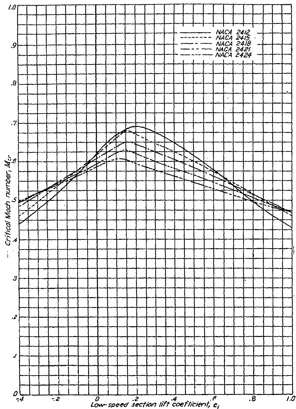
Variation of critical Mach number with low-speed section lift coefficient for several NACA 24-series airfoil sections of various thicknesses.
