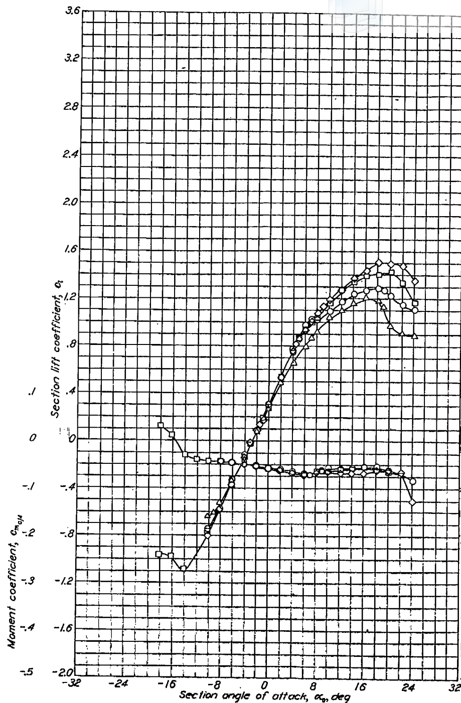
Aerodynamic characteristics of the NACA 65-118, \alpha=0.5 airfoil section, 24-inch chord.
