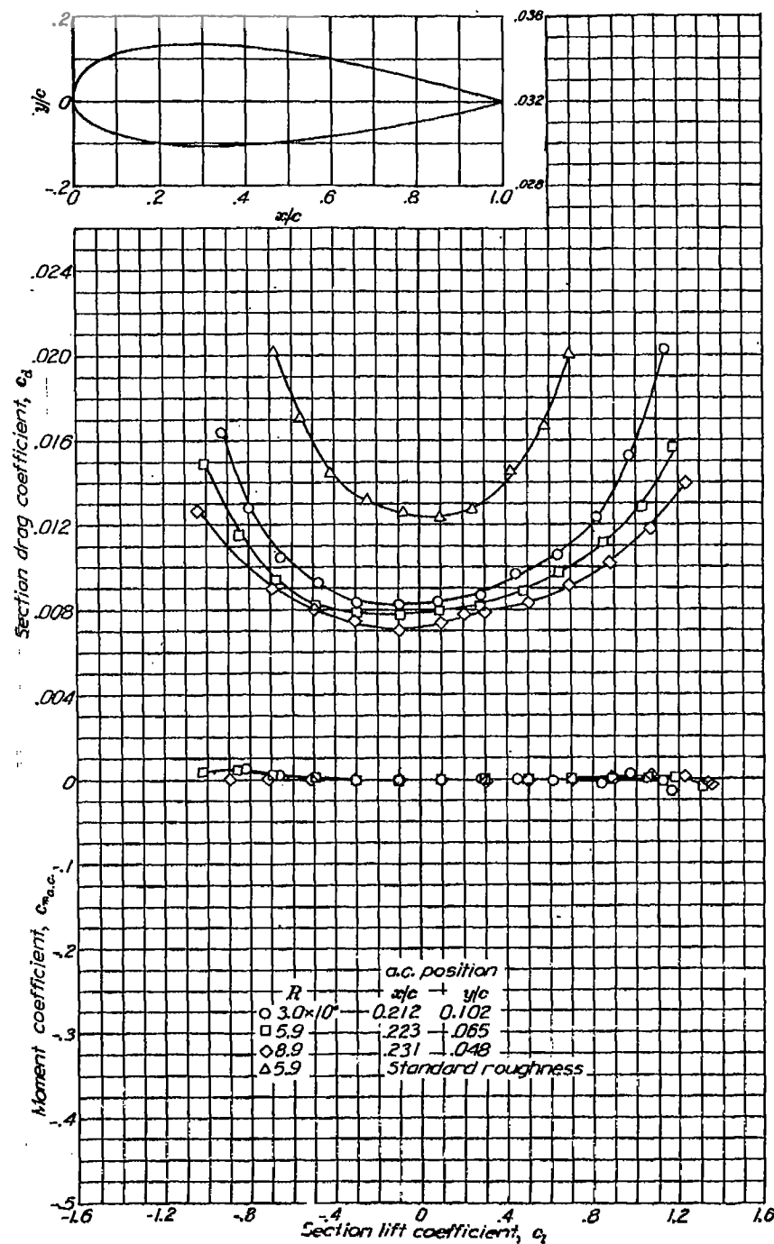
Aerodynamic characteristics of the NACA 23024 airfoil section, 24-inch chord.
