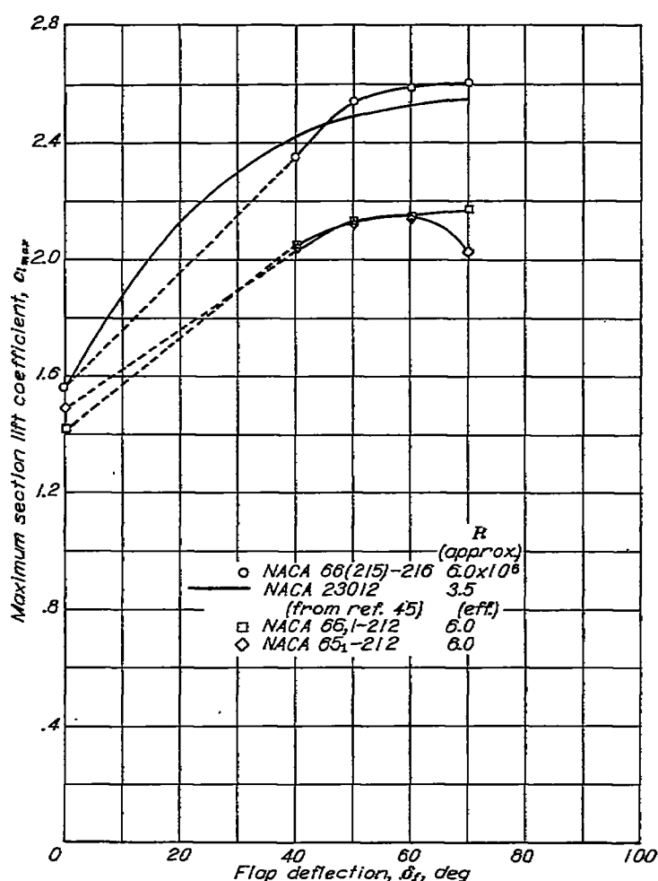
FIGURE 54.—Maximum lift coefficients for some NACA airfoils fitted with 0.20-airfoil-chord split flaps.
