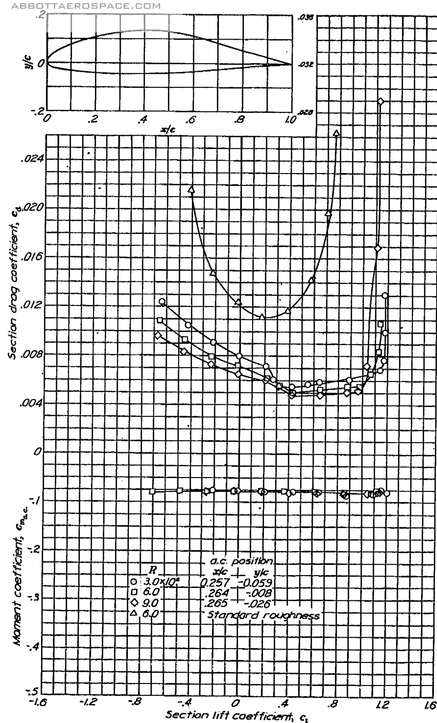
Aerodynamic characteristics of the NACA 653-618, \alpha = 0.5 airfoil section, 24-inch chord.
