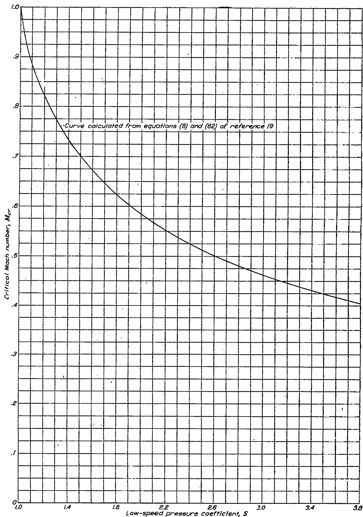
Critical Mach number chart.
