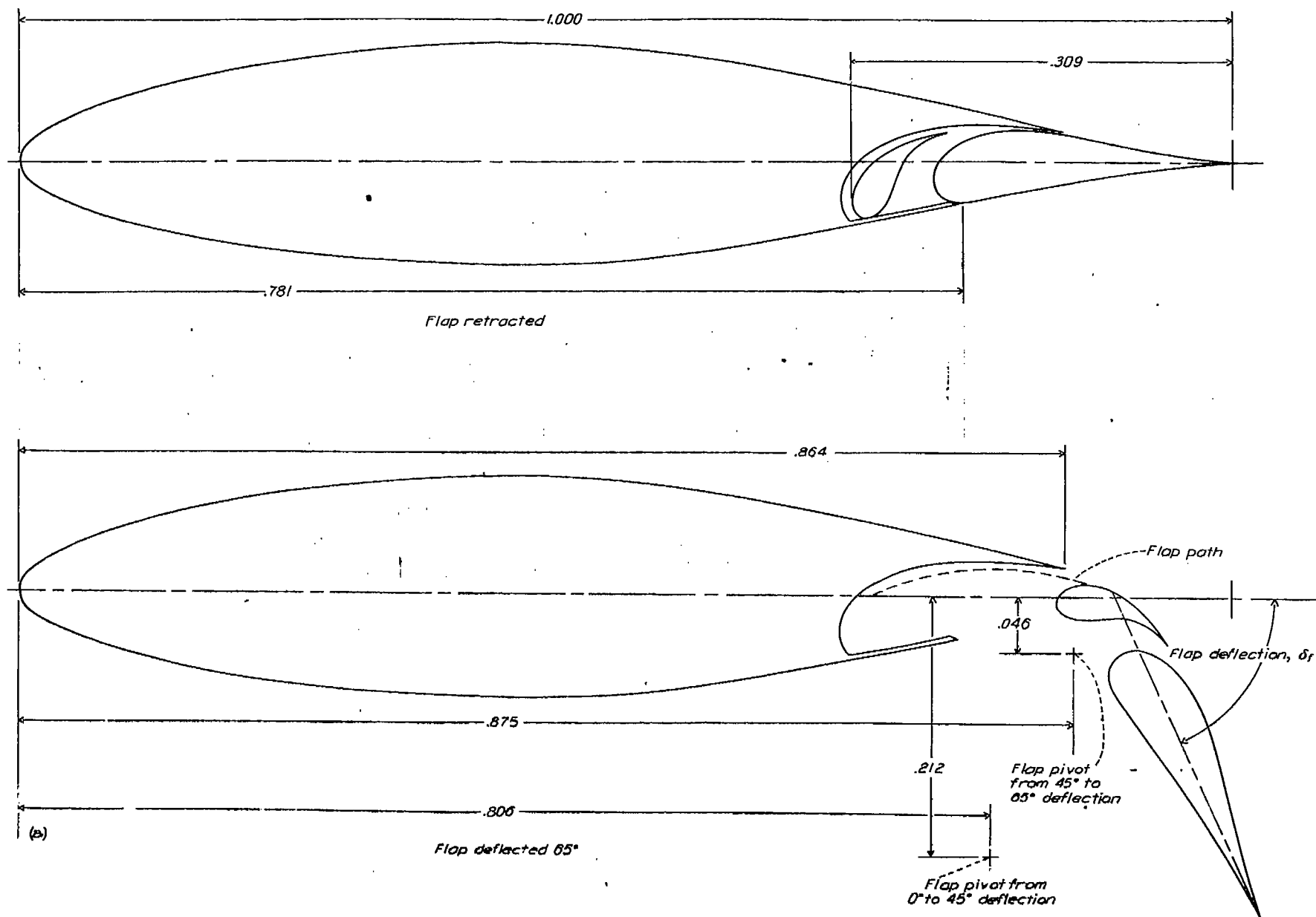
(a) Configuration. NACA 653-118 airfoil section with 0.309 double slotted flap.
