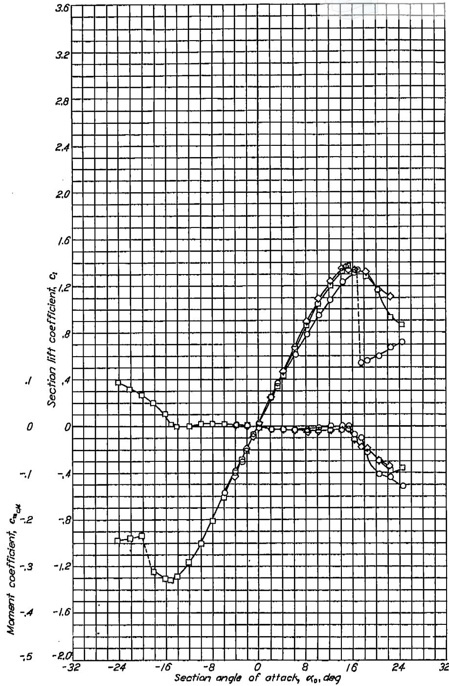
Aerodynamic characteristics of the NACA 66(215)-016 airfoil section, 24-inch chord.
