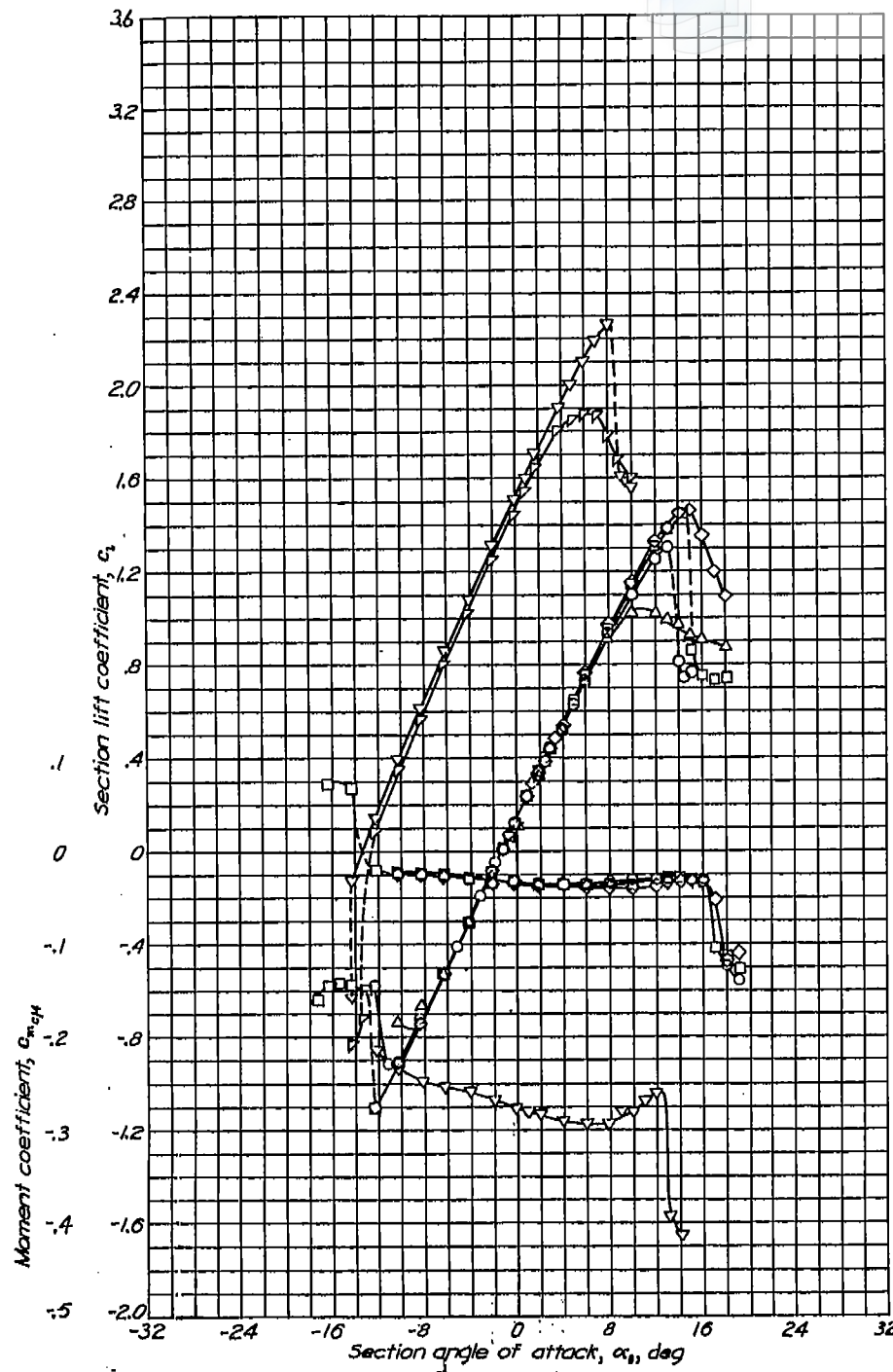
Aerodynamic characteristics of the NACA 661-212 airfoil section, 24-inch chord.
