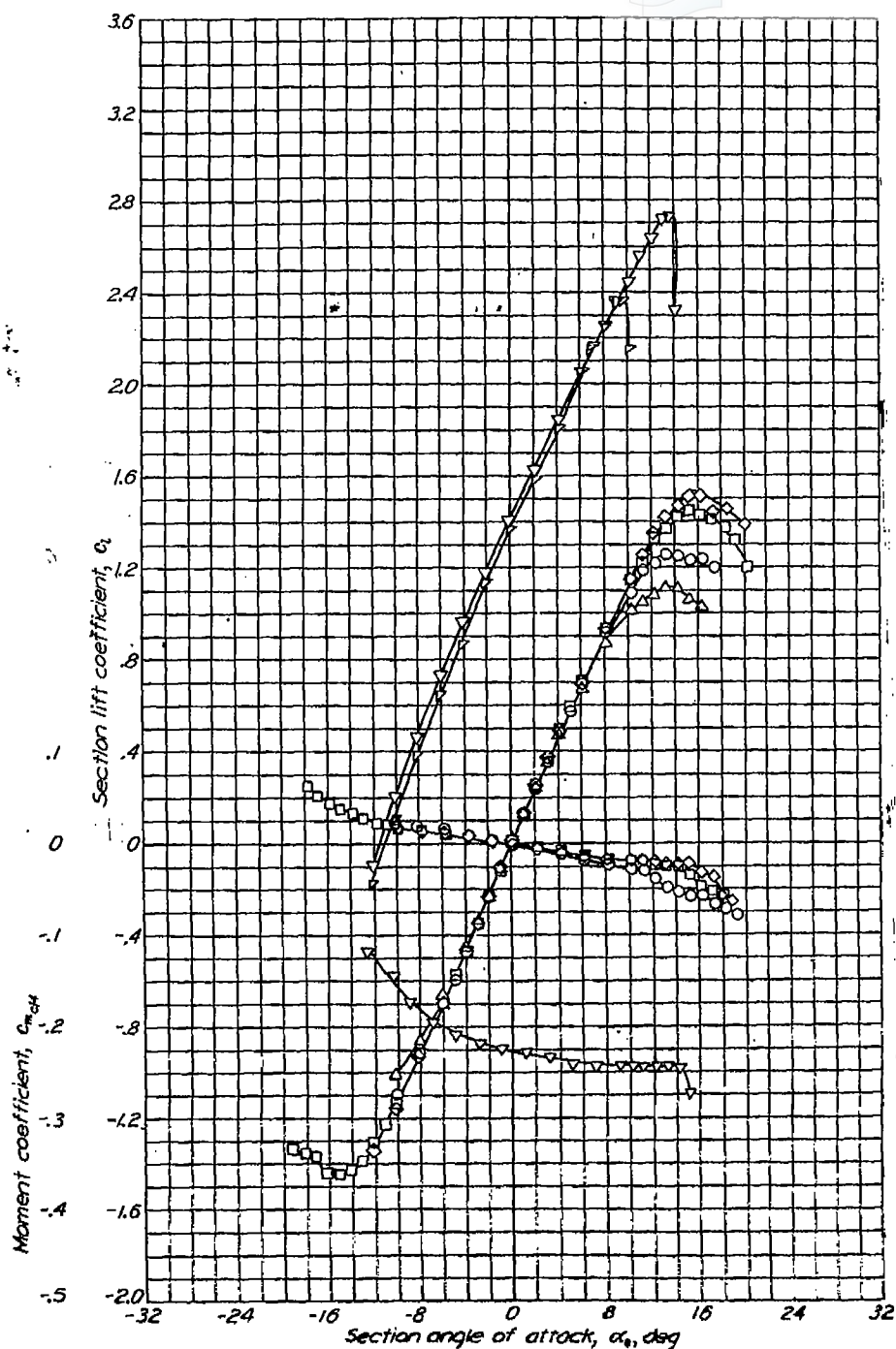
Aerodynamic characteristics of the NACA 633-018 airfoil section, 24-inch chord.
