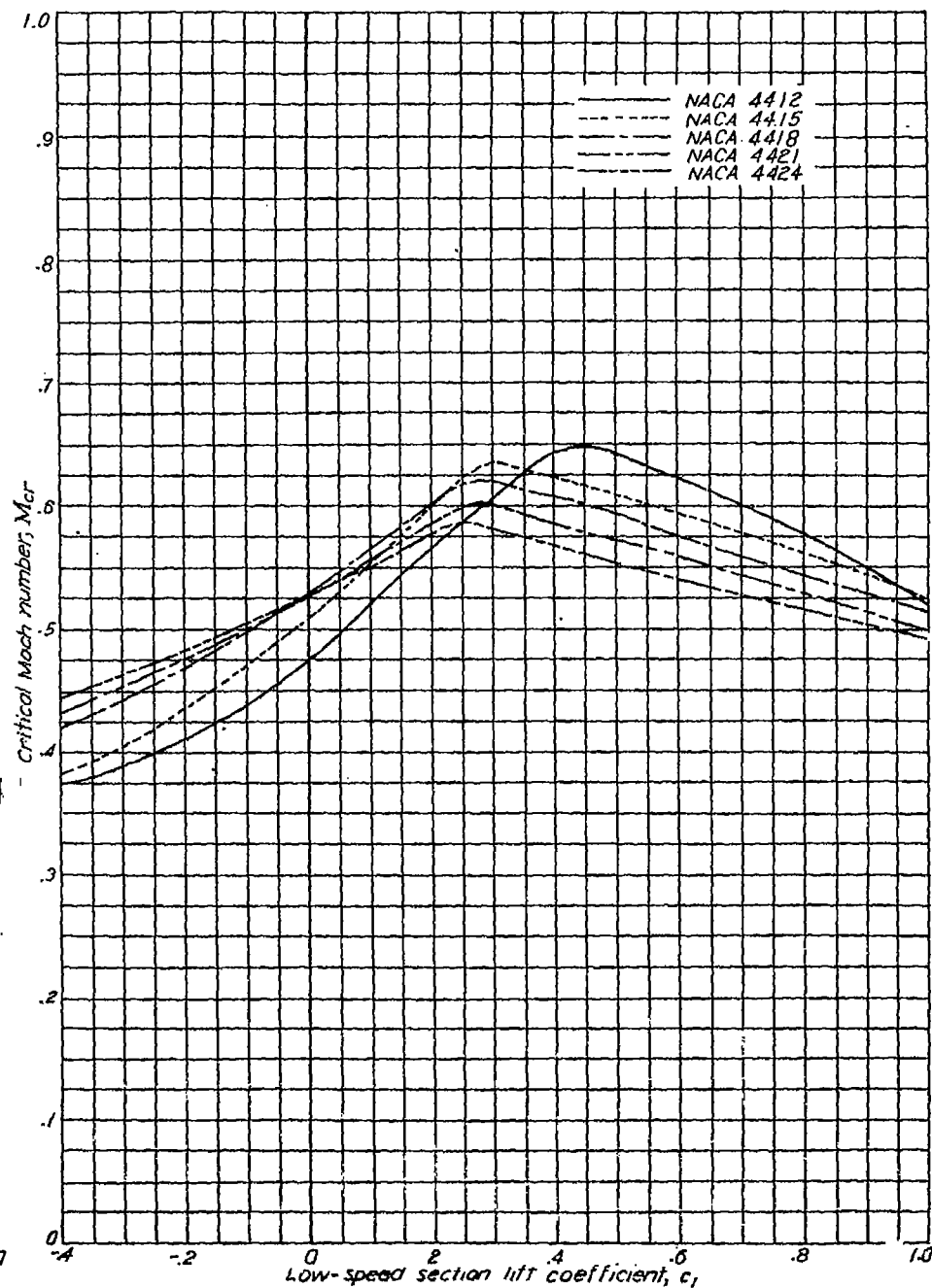
Variation of critical Mach number with low-speed section lift coefficient for several NACA 44-series airfoil sections of various thicknesses.
