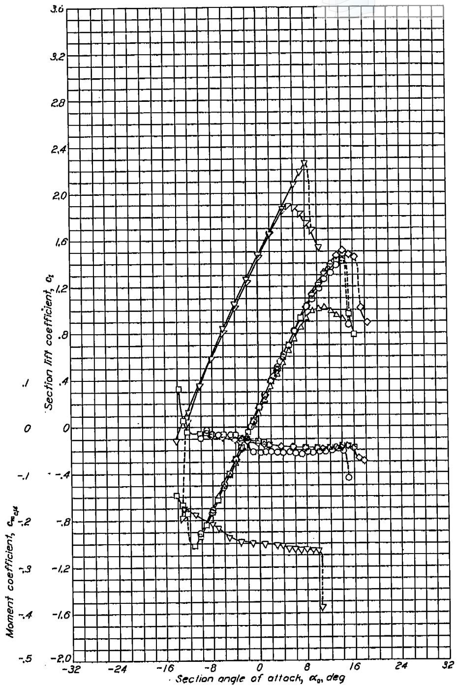
Aerodynamic characteristics of the NACA 65-212, \alpha=0.6 airfoil section, 24-inch chord.
