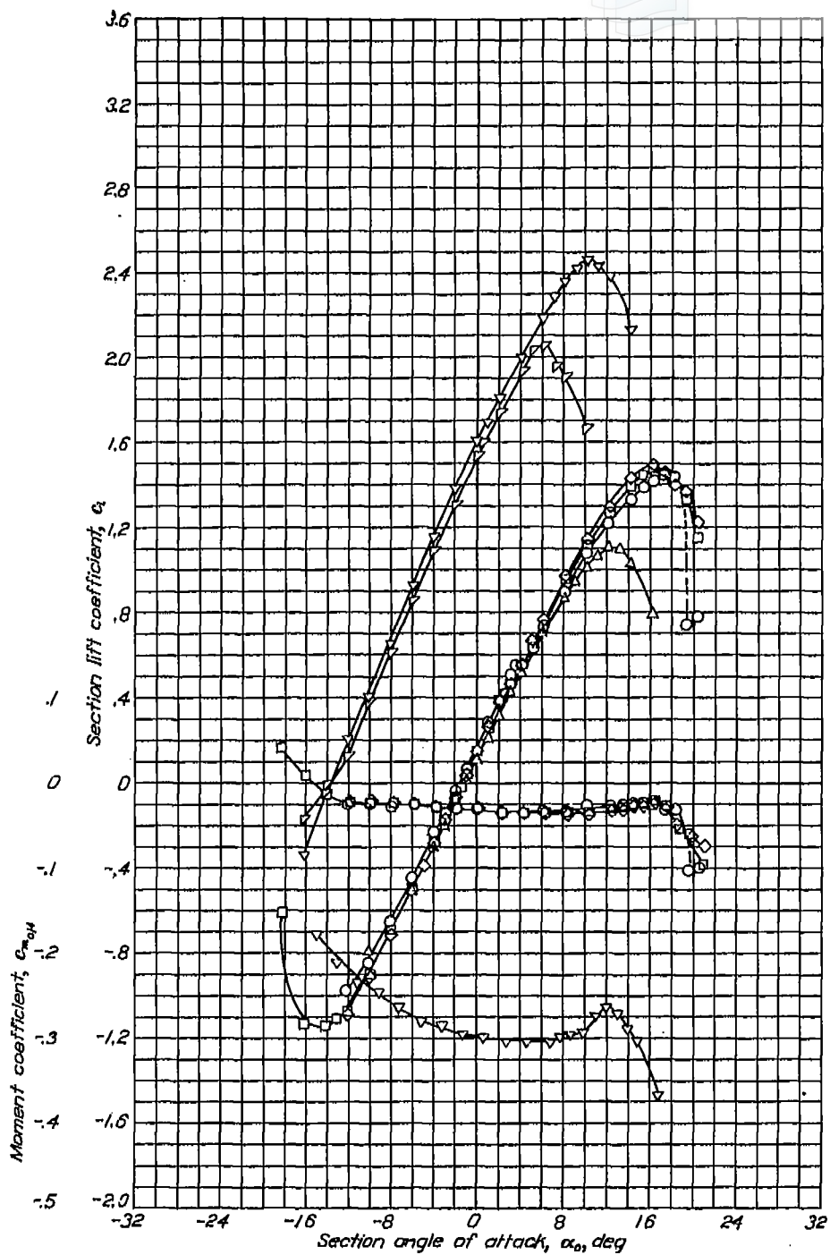
Aerodynamic characteristics of the NACA 66-215 airfoil section, 24-inch chord.
