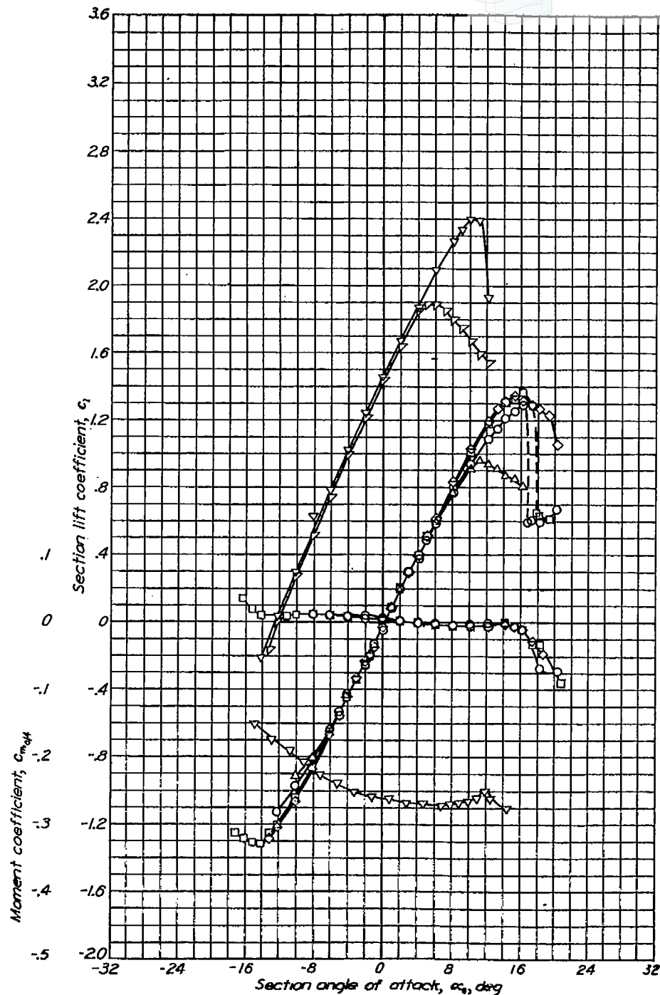
Aerodynamic characteristics of the NACA 662-015 airfoil section, 24-inch chord.
