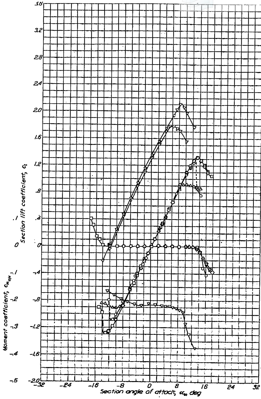
Aerodynamic characteristics of the NACA 0009 airfoil section, 24-inch chord.
