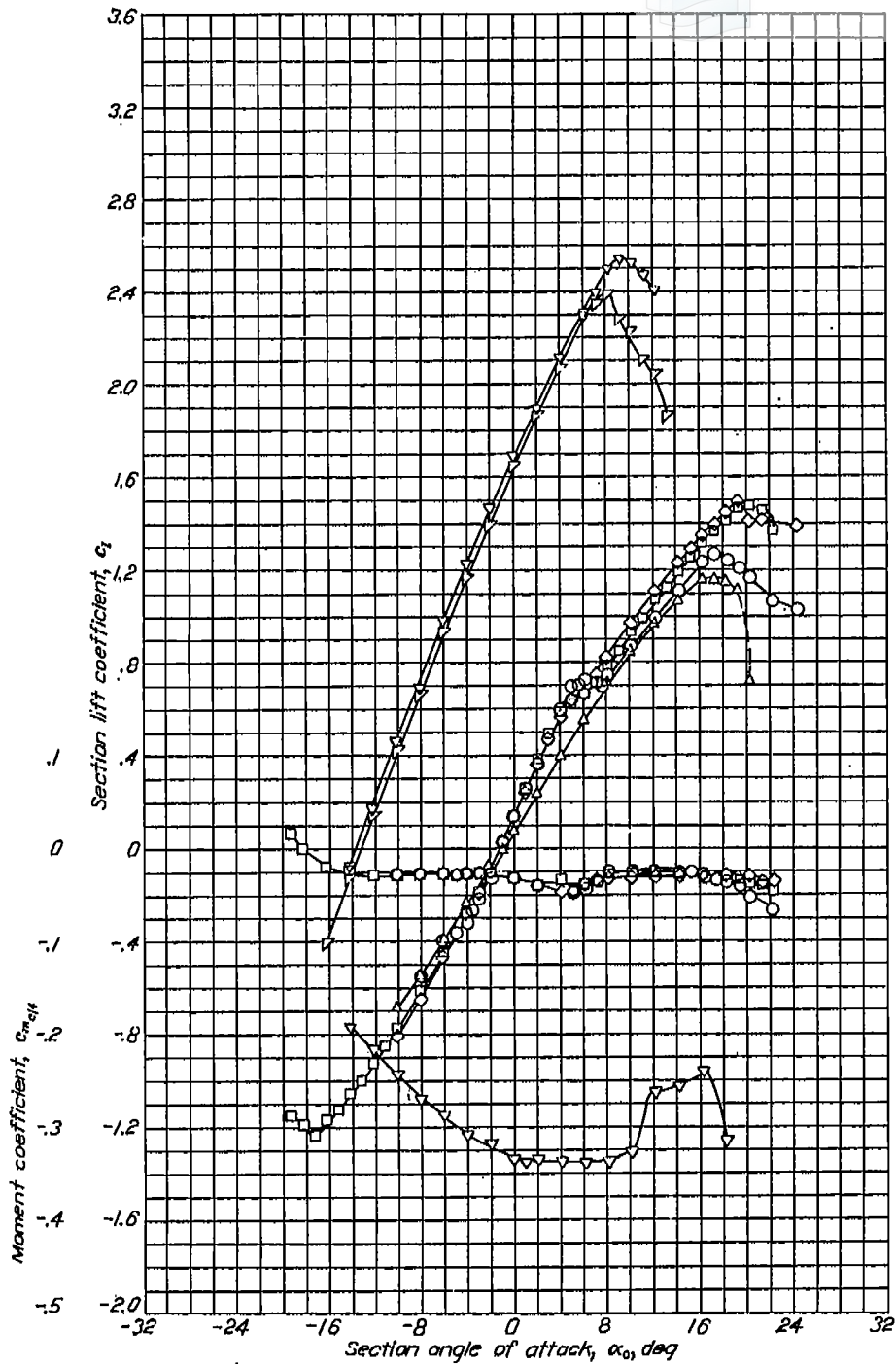
Aerodynamic characteristics of the NACA 66-221 airfoil section, 24-inch chord.
