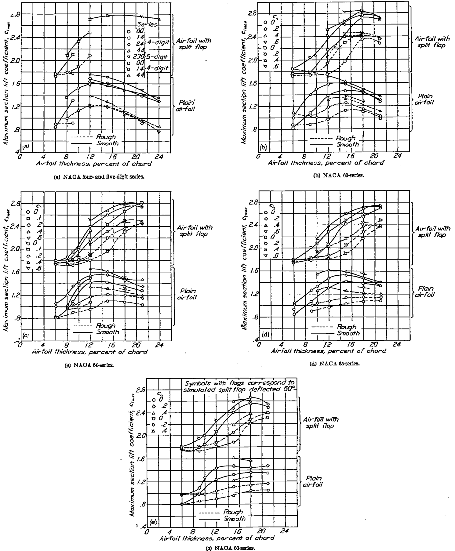
FIGURE 39.—Variation of maximum section lift coefficient with airfoil thickness ratio and camber for several NACA airfoil sections with and without simulated split flaps and standard roughness. R=6 \times 10^6 .
