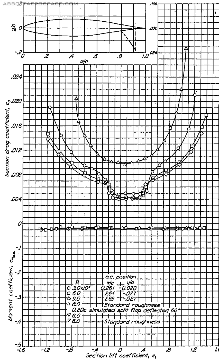
Aerodynamic characteristics of the NACA 65(11)-114 airfoil section, 24 inch chord.
