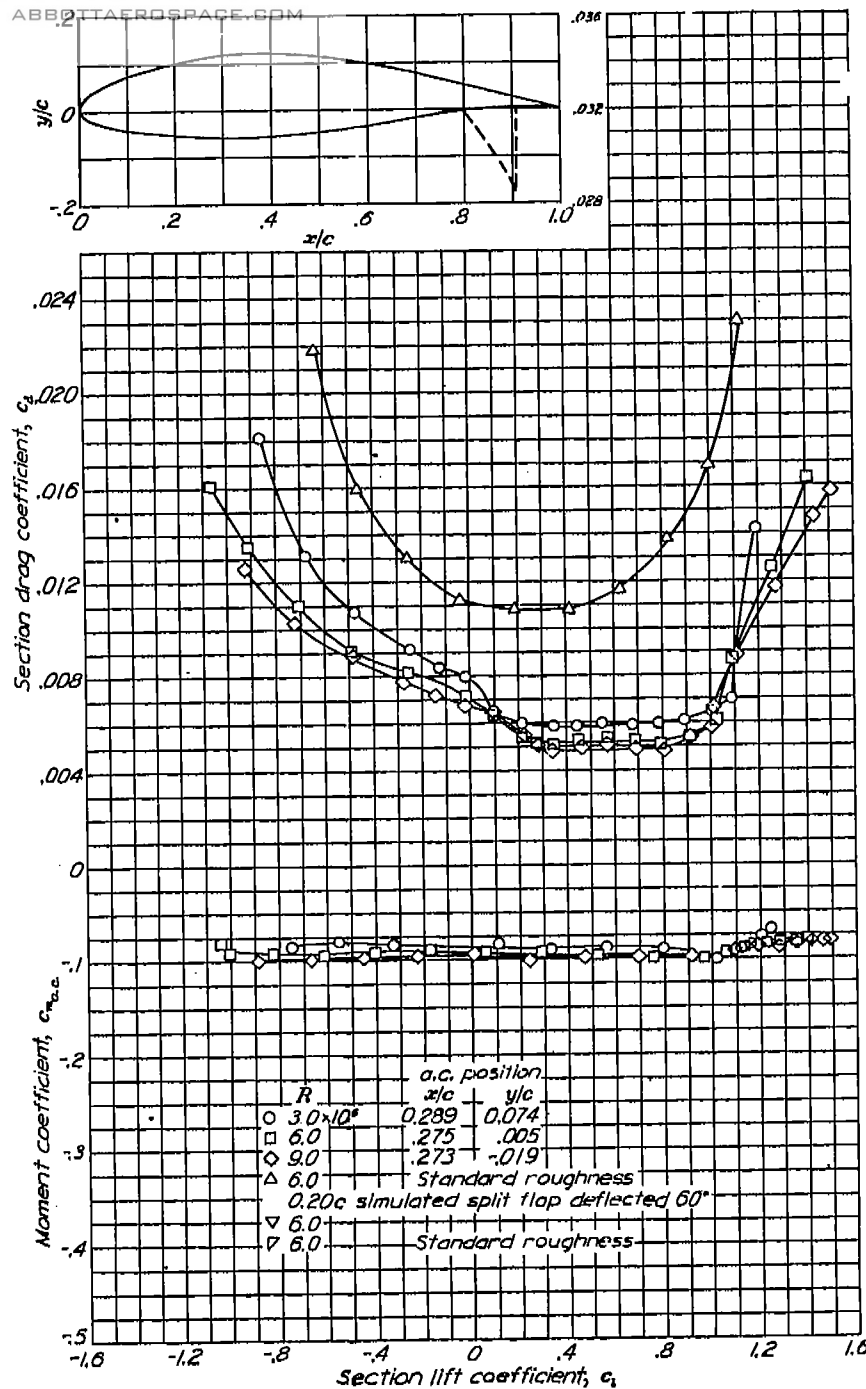
Aerodynamic characteristics of the NACA 643-618 airfoil section, 24-inch chord.
