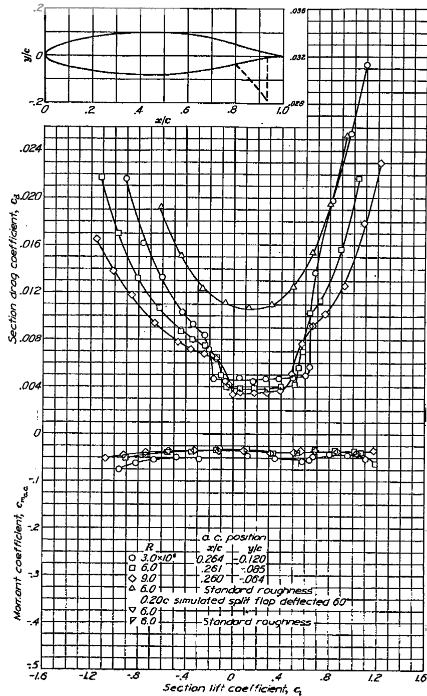
Aerodynamic characteristics of the NACA 66-218 airfoil section, 24-inch chord.
