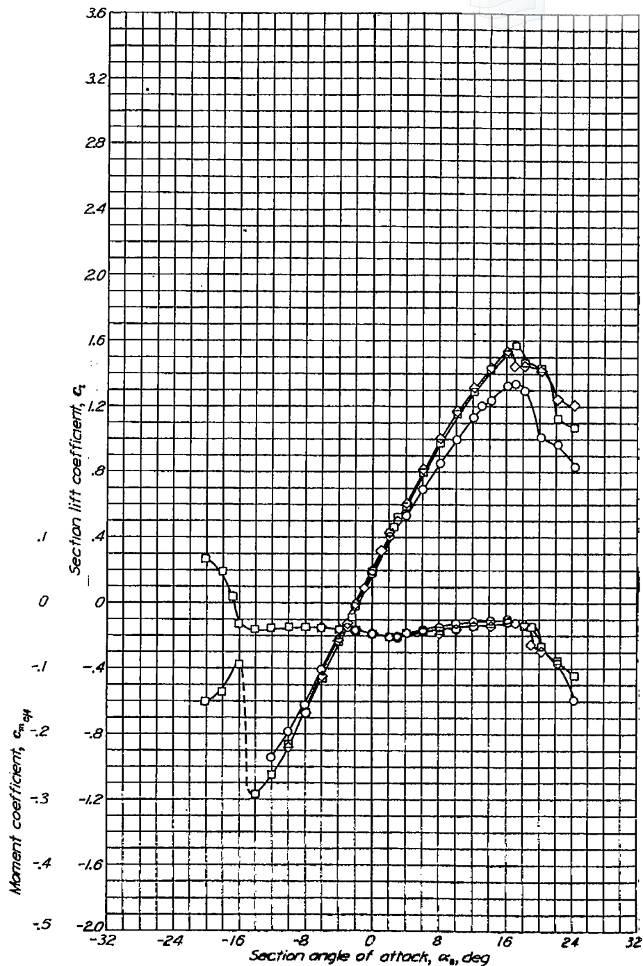
Aerodynamic characteristics of the NACA 66(215)-216 airfoil section, 24-inch chord.
