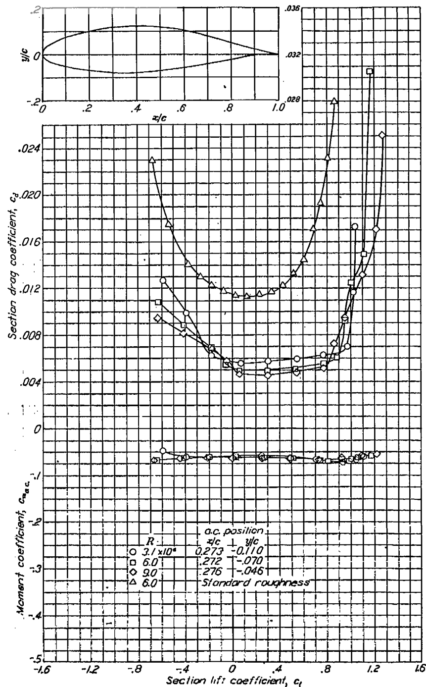
Aerodynamic characteristics of the NACA 65(421)-420 airfoil section, 24-inch chord.
