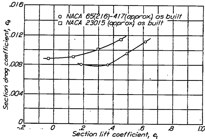
FIGURE 30.—Drag characteristics of the NACA 65(216)-417 (approx.) and NACA 23015 (approx.) airfoil sections built by practical-construction methods by the same manufacturer. R=10.28 \times 10^6 .
