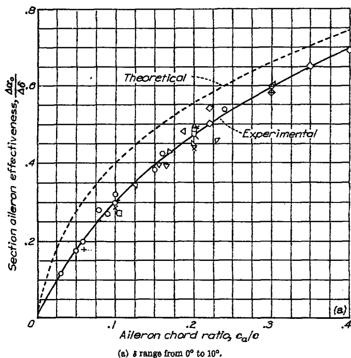
FIGURE 59.—Variation of section aileron effectiveness with aileron chord ratio for true-airfoil-contour ailerons without exposed overhang balance on a number of airfoil sections. Gaps sealed; \alpha_1=0 .
