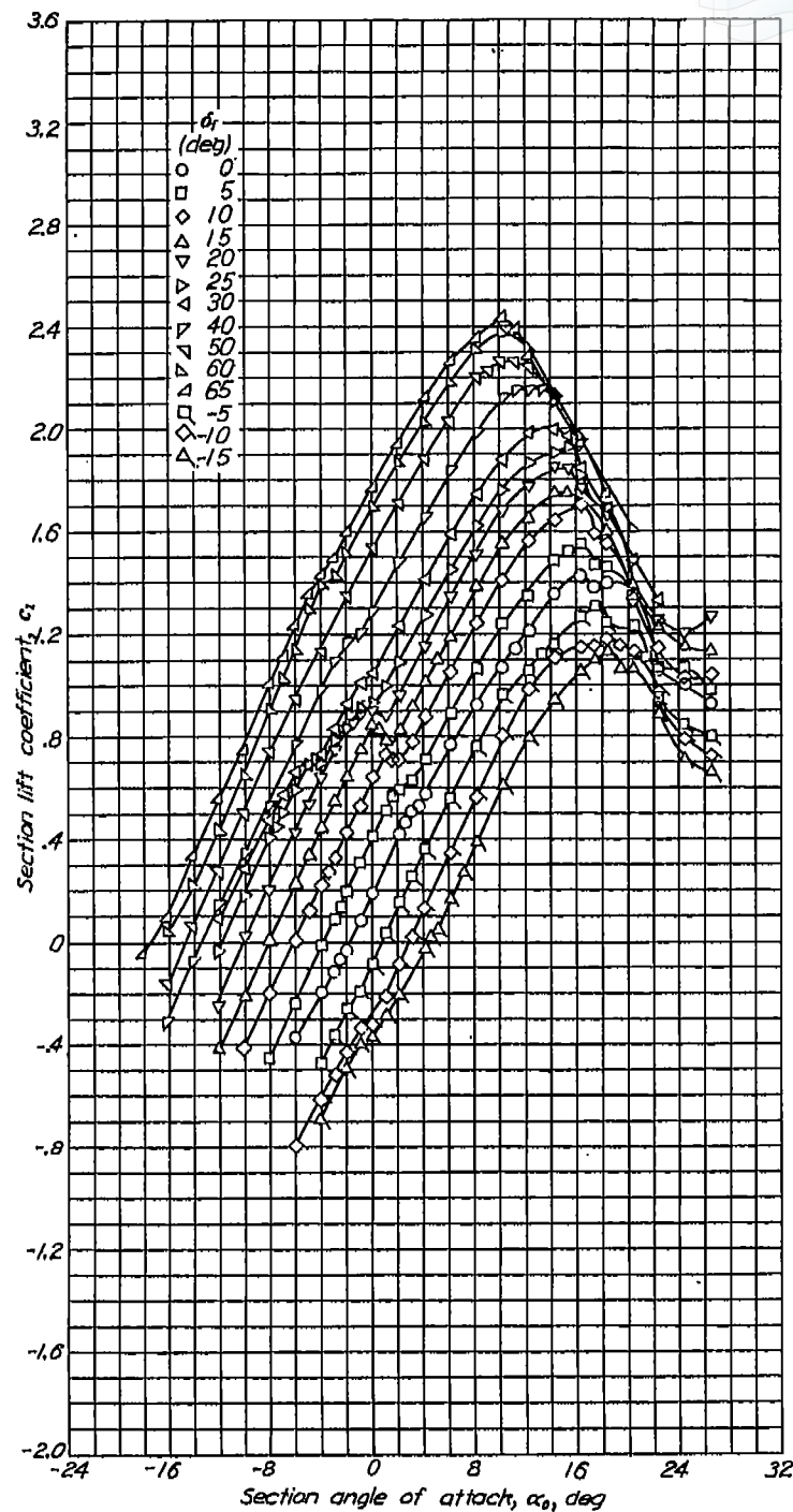
Aerodynamic characteristics of the NACA 66(215)-216 airfoil section with 0.20s sealed plain flap. R=6 \times 10^4 .
