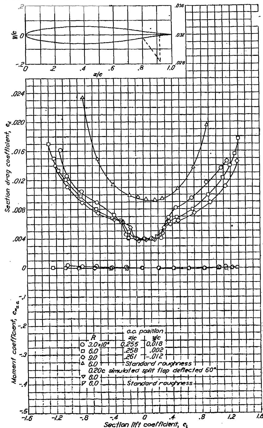
Aerodynamic characteristics of the NACA 651-012 airfoil section, 24-inch chord.
