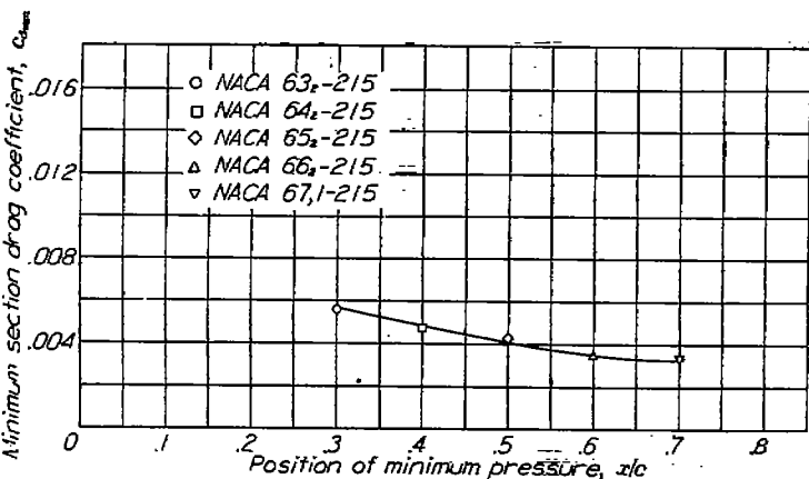
FIGURE 9.—Variation of minimum drag coefficient with position of minimum pressure for some NACA 6-series airfoils of the same camber and thickness. R = 6 \times 10^6 .
