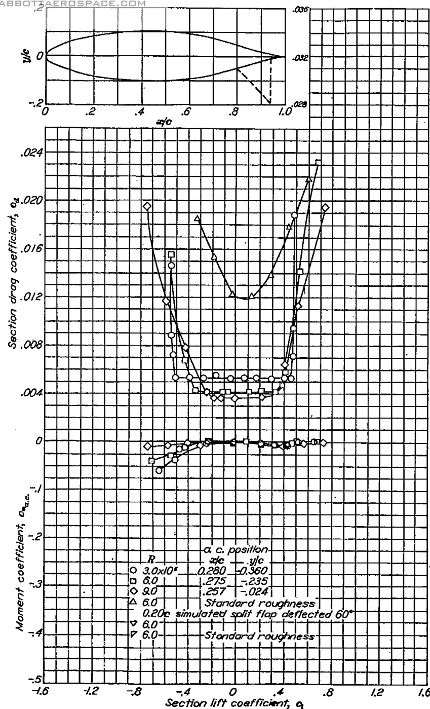
Aerodynamic characteristics of the NACA 66-021 airfoil section, 24-inch chord.
