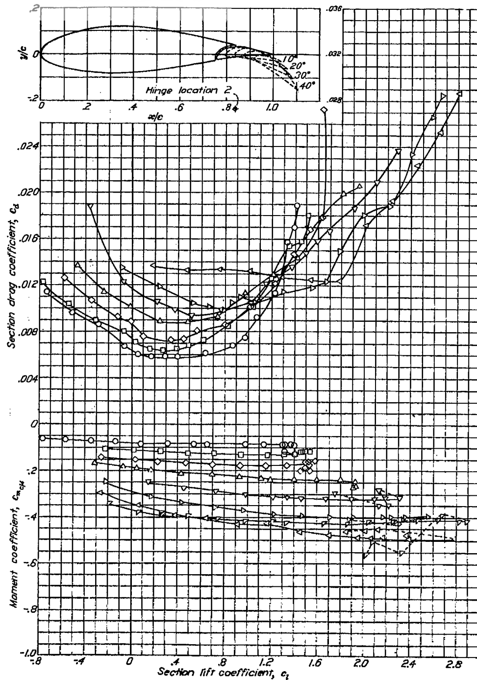
(c) Aerodynamic characteristics with hinge location 2. R = 5 \times 10^6 . NACA 63,4-420 airfoil section with 0.26c slotted flap.
