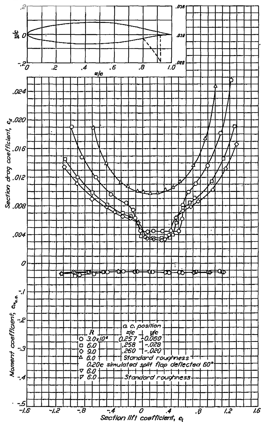
Aerodynamic characteristics of the NACA 66-215 airfoil section, 24-inch chord.
