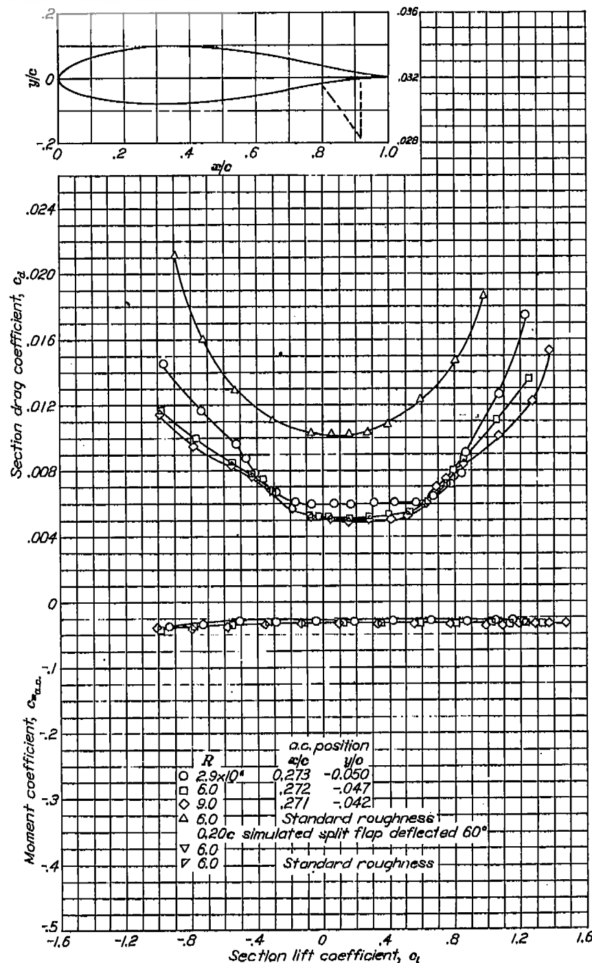
Aerodynamic characteristics of the NACA 63-218 airfoil section, 24-inch chord.
