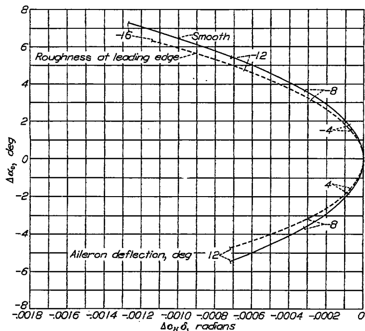
FIGURE 62.—Variation of the hinge-moment parameter \Delta\alpha_0\delta with the equivalent change in section angle of attack required to maintain a constant section lift coefficient for deflection of the aileron on the NACA 64,2-(1.4)(13.5) airfoil section, smooth and with roughness at the leading edge of the airfoil. (For description of aileron, see fig. 60.)
