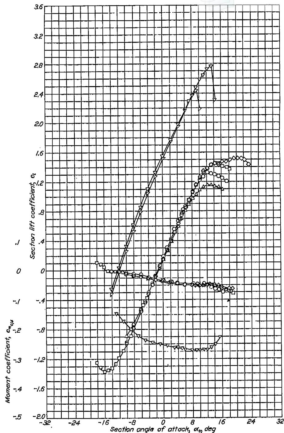
Aerodynamic characteristics of the NACA 63-218 airfoil section, 24-inch chord.
