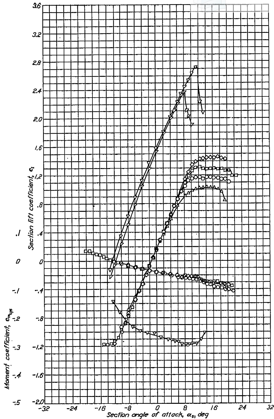
Aerodynamic characteristics of the NACA 634-221 airfoil section, 24-inch chord,
