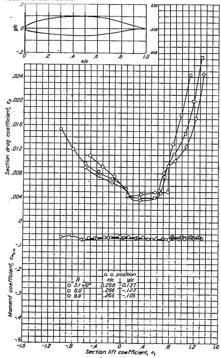
Aerodynamic characteristics of the NACA 66(215)-416 airfoil section, 24-inch chord.
