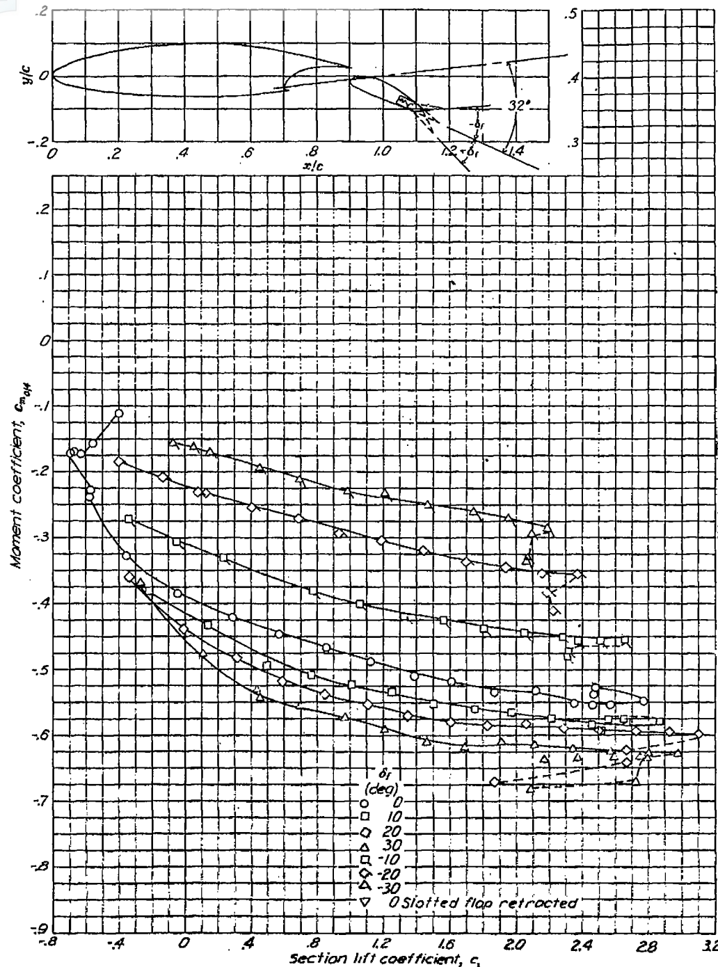
(f) Lift and moment characteristics. Slotted flap deflected 32^\circ ; R=6 \times 10^6 . NACA 66(215)-216, \alpha=0.6 airfoil section with 0.30c slotted and 0.10c plain flap.
