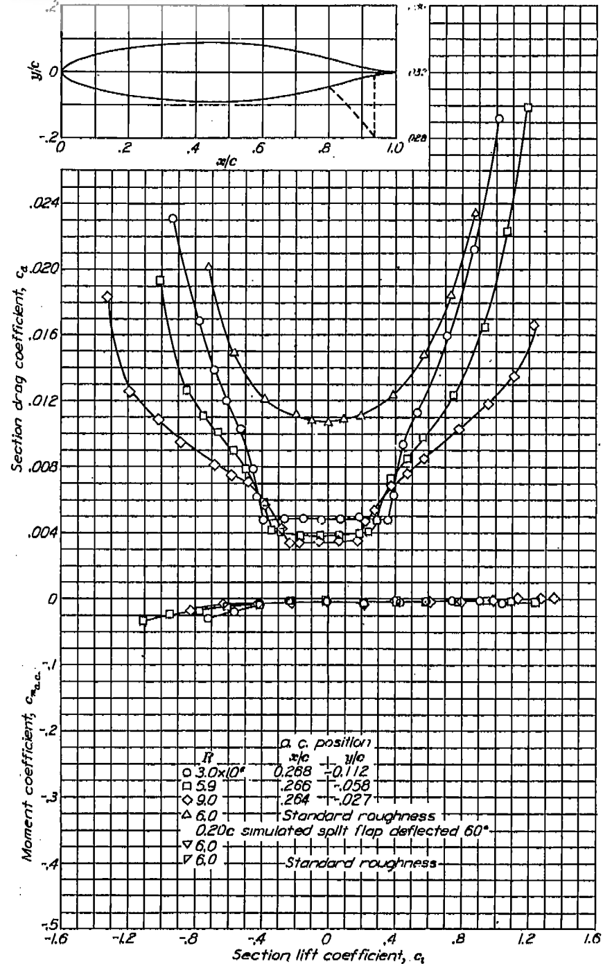
Aerodynamic characteristics of the NACA 66-018 airfoil section, 24-inch chord.
