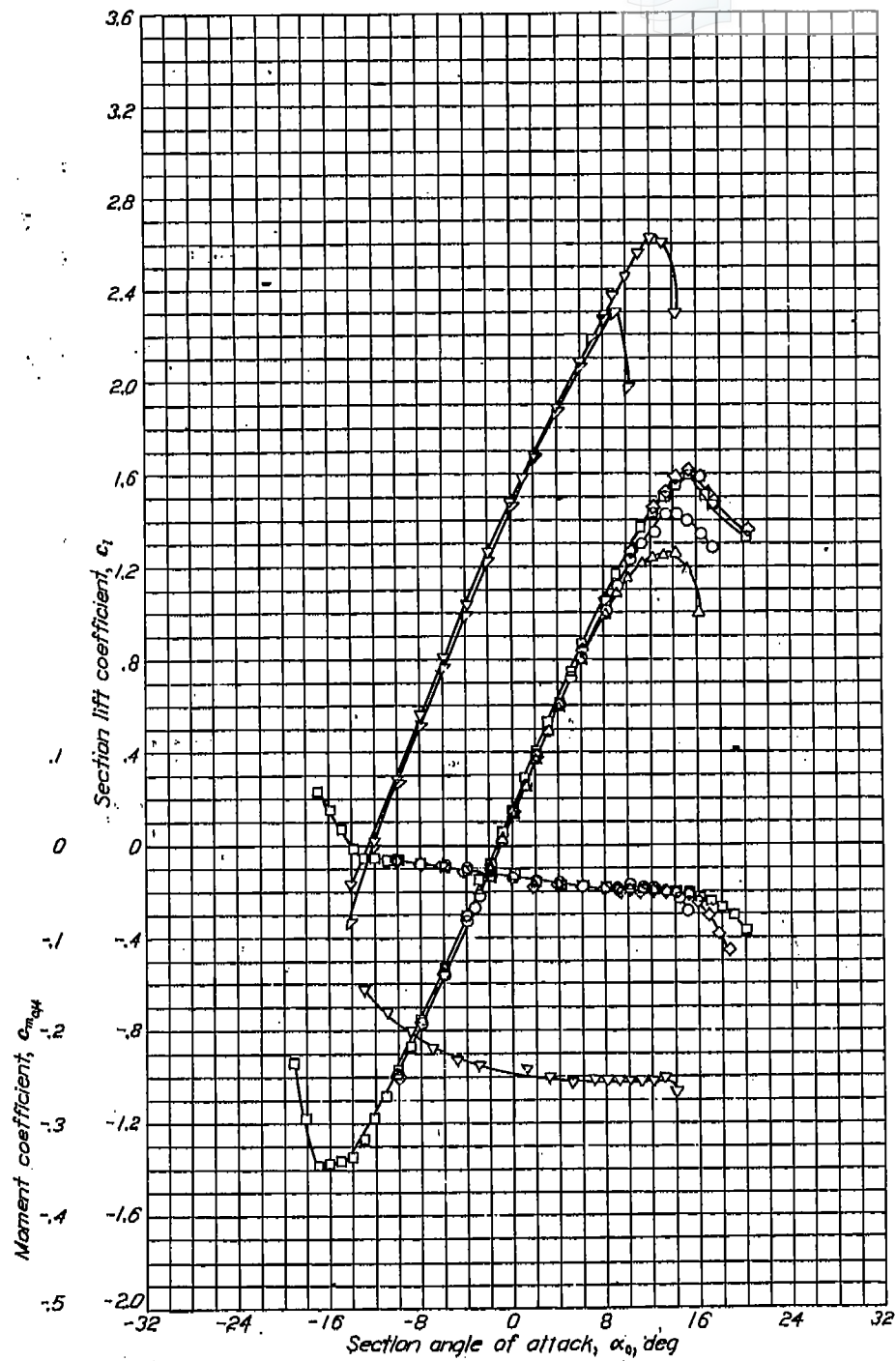
Aerodynamic characteristics of the NACA 63-215 airfoil section, 24-inch chord.
