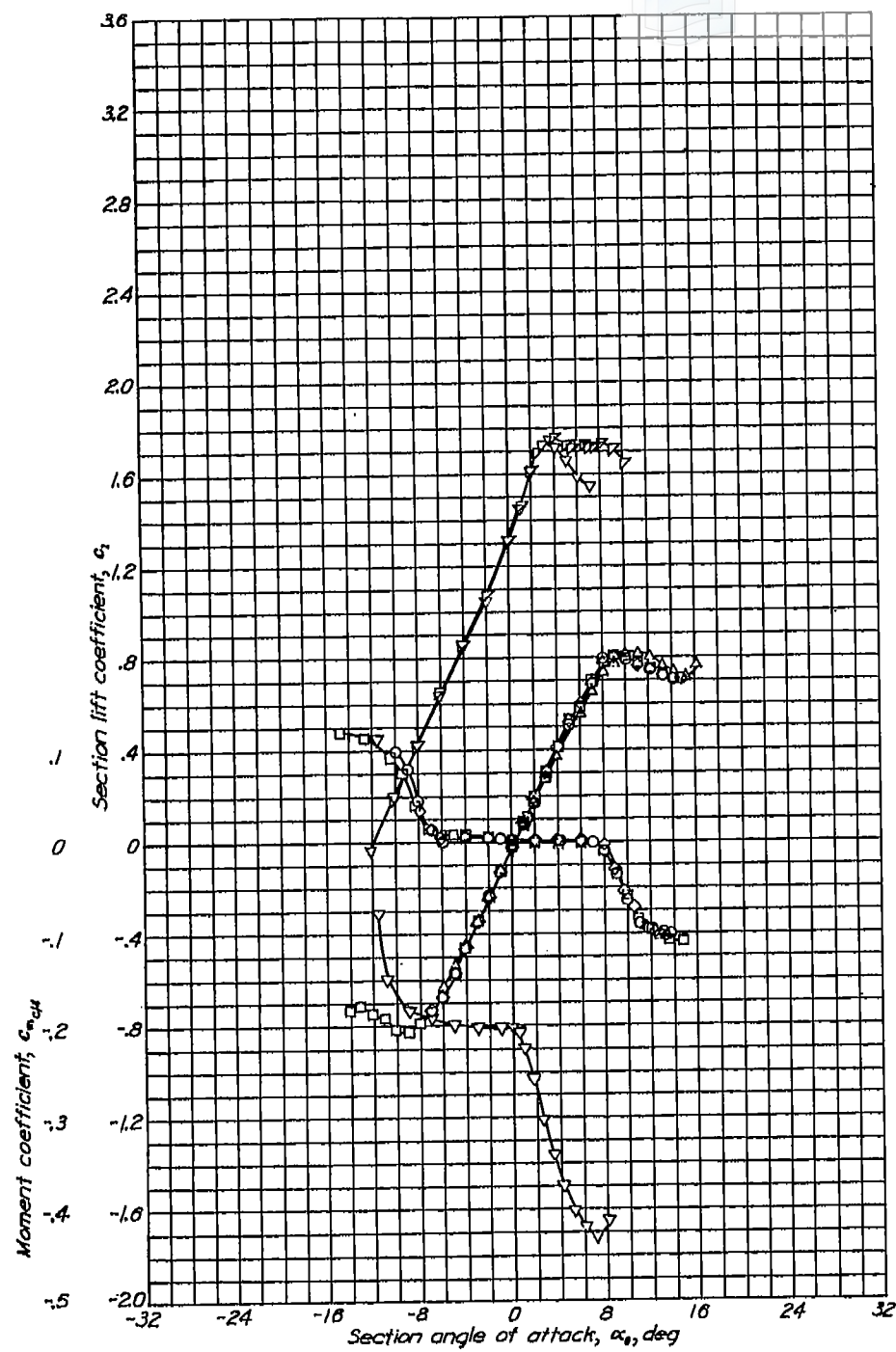
Aerodynamic characteristics of the NACA 66-006 airfoil section, 24-inch chord.
