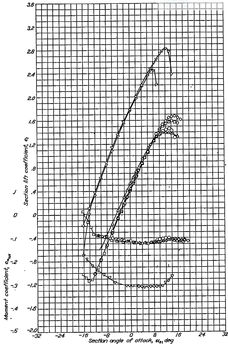
Aerodynamic characteristics of the NACA 63-615 airfoil section, 24-inch chord.
