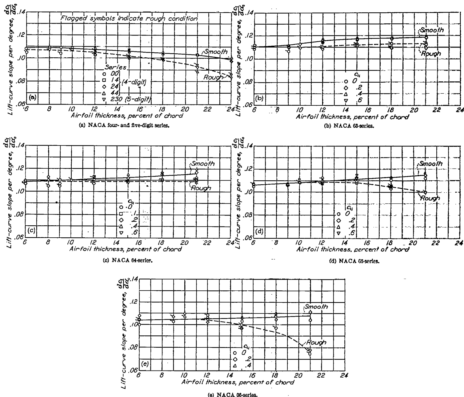
FIGURE 38.—Variation of lift-curve slope with airfoil thickness ratio and camber for a number of NACA airfoil sections in both the smooth and rough conditions. R=0 \times 10^6 .
