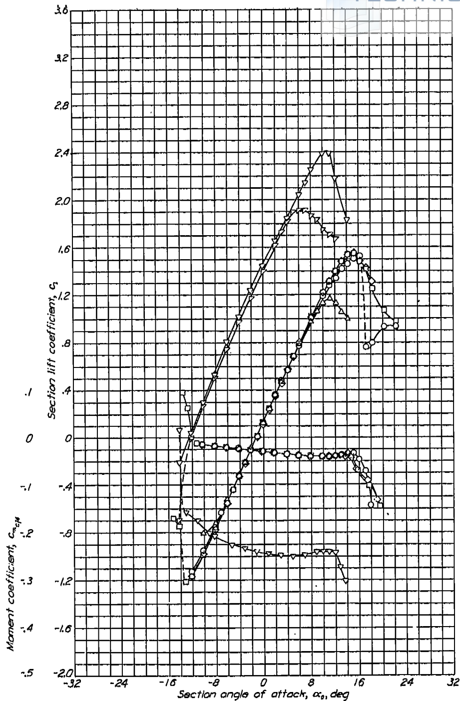
Aerodynamic characteristics of the NACA 64-212 airfoil section, 24-inch chord.
