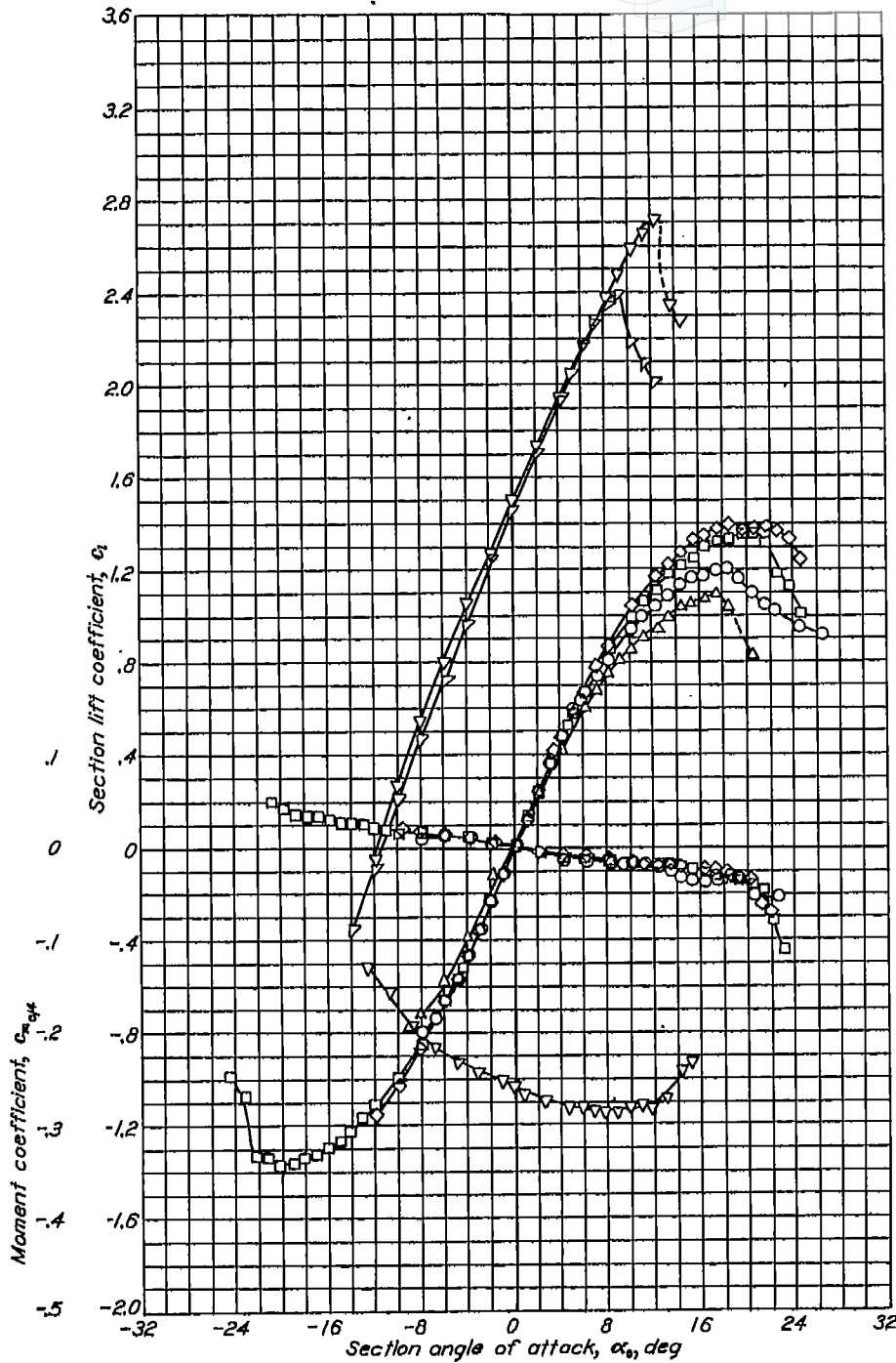
Aerodynamic characteristics of the NACA 654-021 airfoil section, 24-inch chord.
