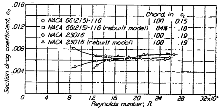
FIGURE 31.—Scale effect on drag of the NACA 66(215)-116 and NACA 23016 airfoil sections built by practical-construction methods by the same manufacturer and tested as received.
