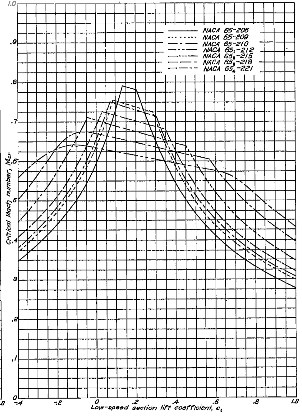
Variation of critical Mach number with low-speed section lift coefficient for several NACA 65-series airfoil sections of various thicknesses, cambered for a design lift coefficient of 0.2.
