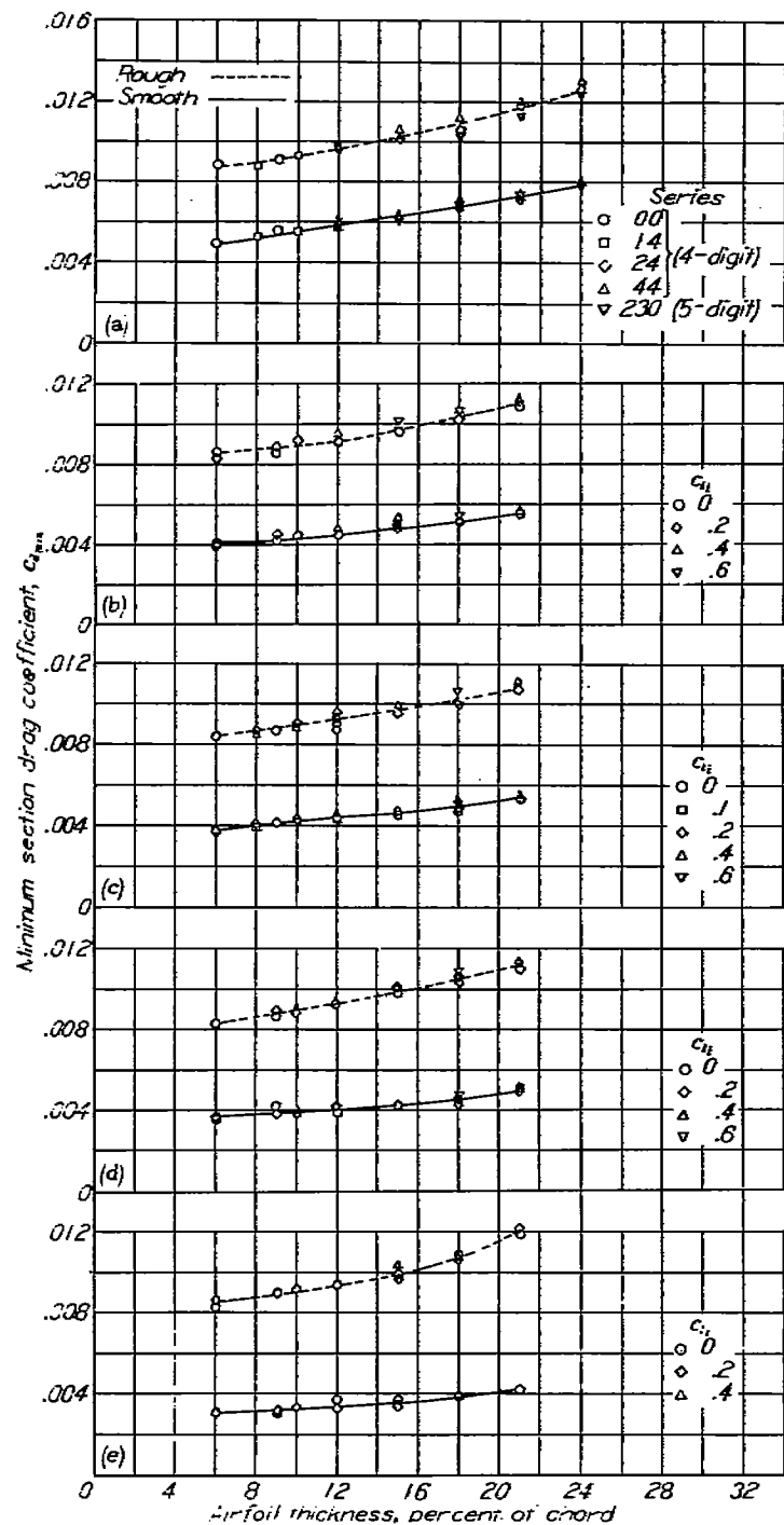
(a) NACA four- and five-digit series. (b) NACA 63-series. (c) NACA 64-series. (d) NACA 65-series. (e) NACA 66-series.
