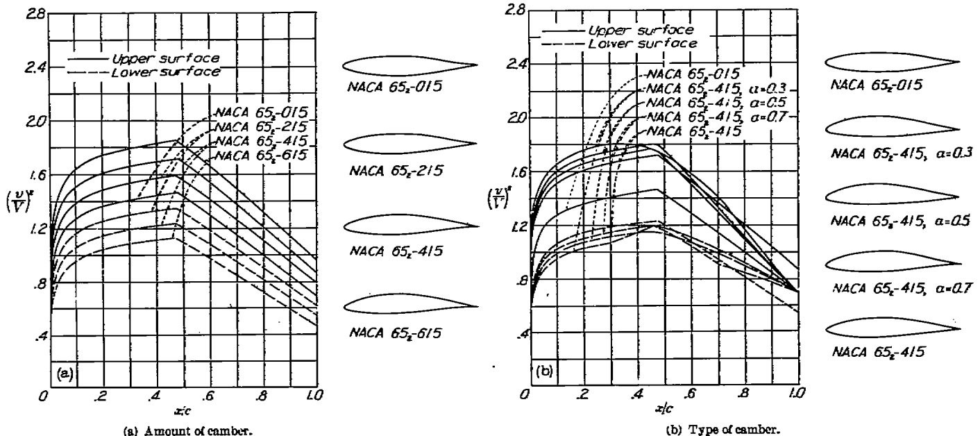
FIGURE 3.—Effect of amount and type of camber on pressure distribution at design lift.
