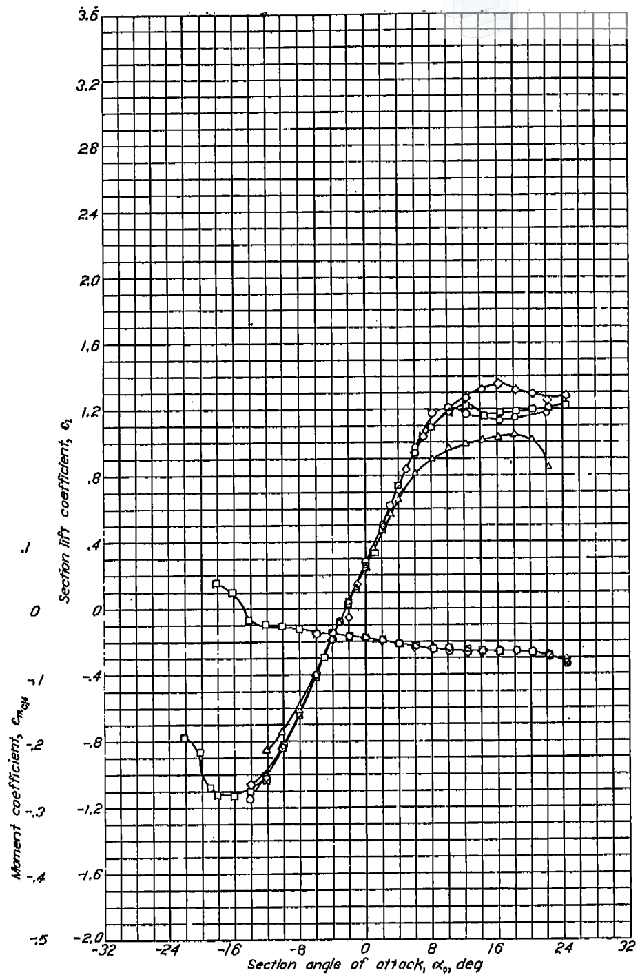
Aerodynamic characteristics of the NACA 63,4-420, \alpha = 0.3 airfoil section, 24-inch chord.
