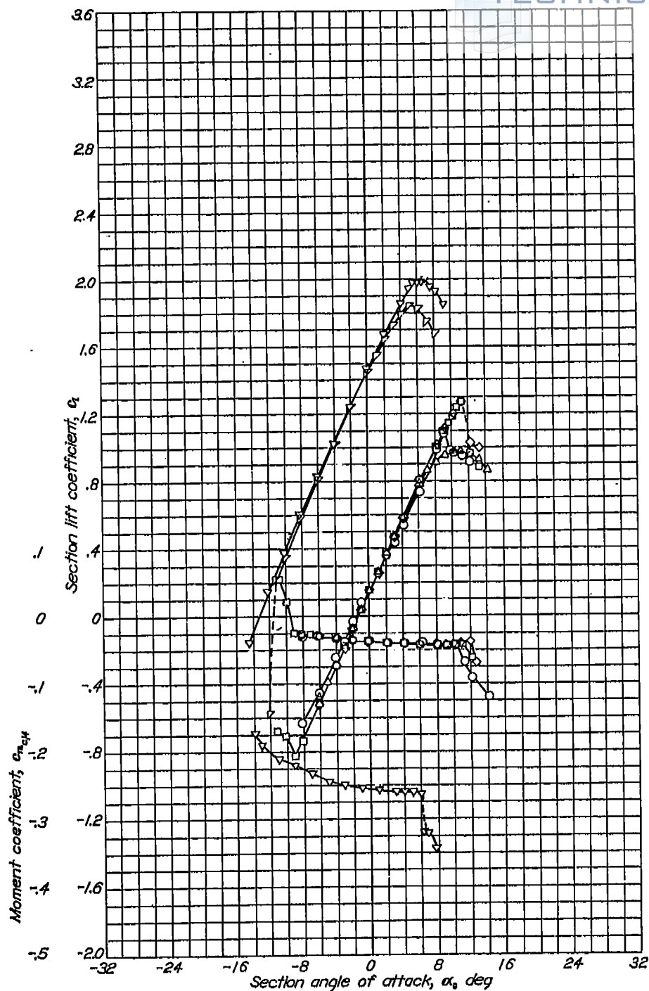
Aerodynamic characteristics of the NACA 66-210 airfoil section, 24-inch chord.
