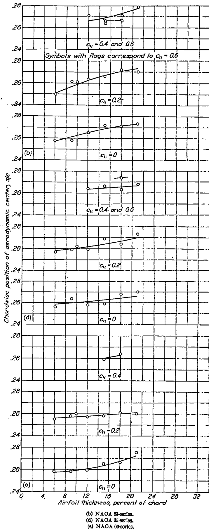
FIGURE 52.—Variation of section chordwise position of the aerodynamic center with airfoil thickness ratio for several NACA airfoil sections of different cambers. R=6 \times 10^6 .
