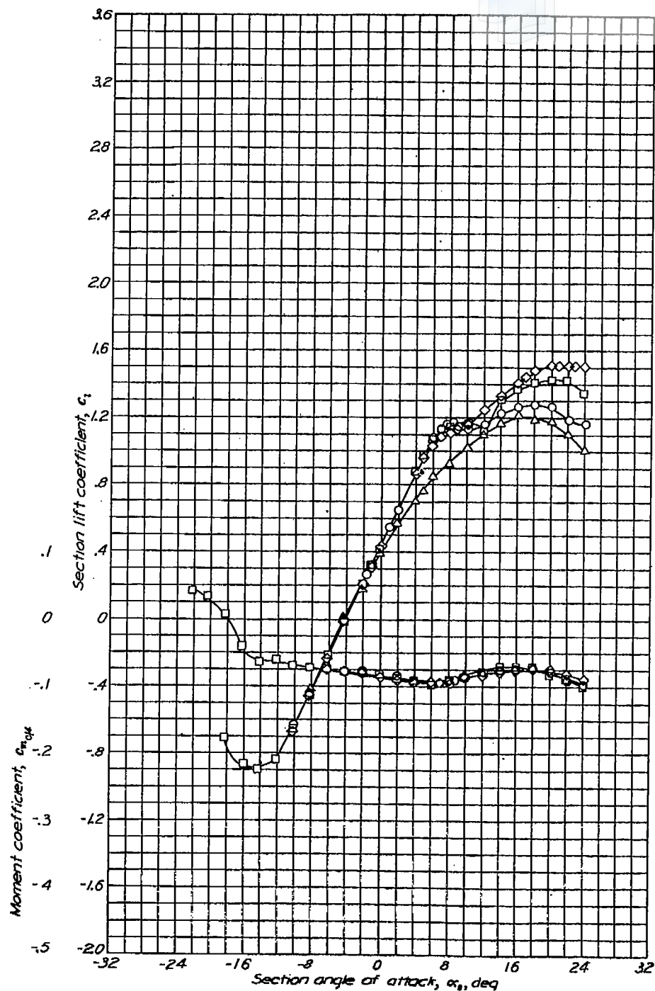
Aerodynamic characteristics of the NACA 653-618, \alpha = 0.5 airfoil section, 24-inch chord.
