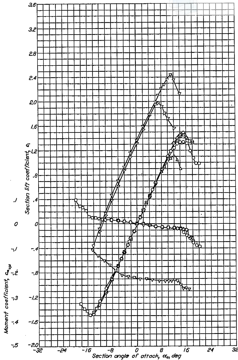
Aerodynamic characteristics of the NACA 64-015 airfoil section, 24-inch chord.
