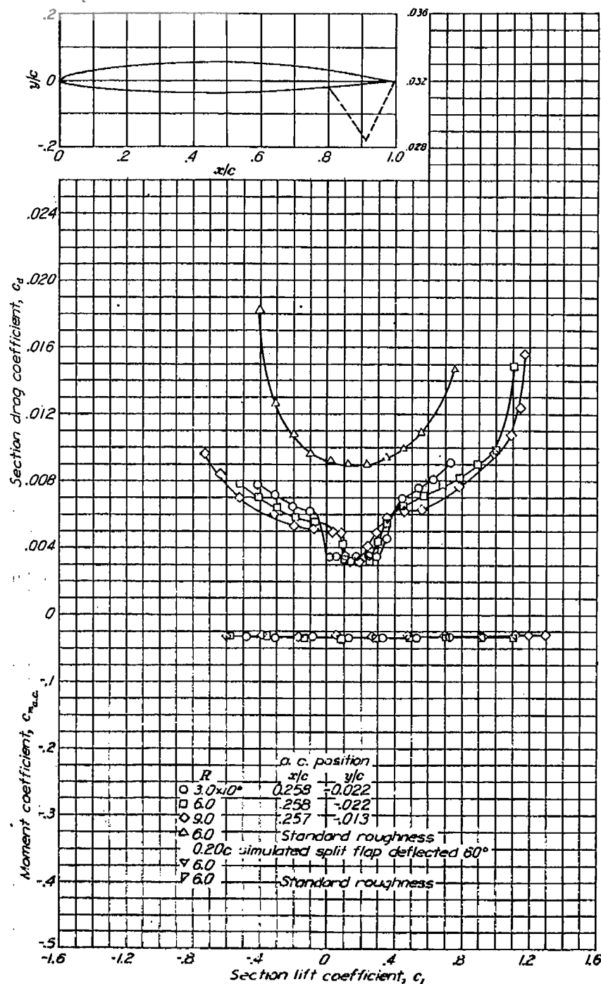
Aerodynamic characteristics of the NACA 66-209 airfoil section, 24-inch chord.
