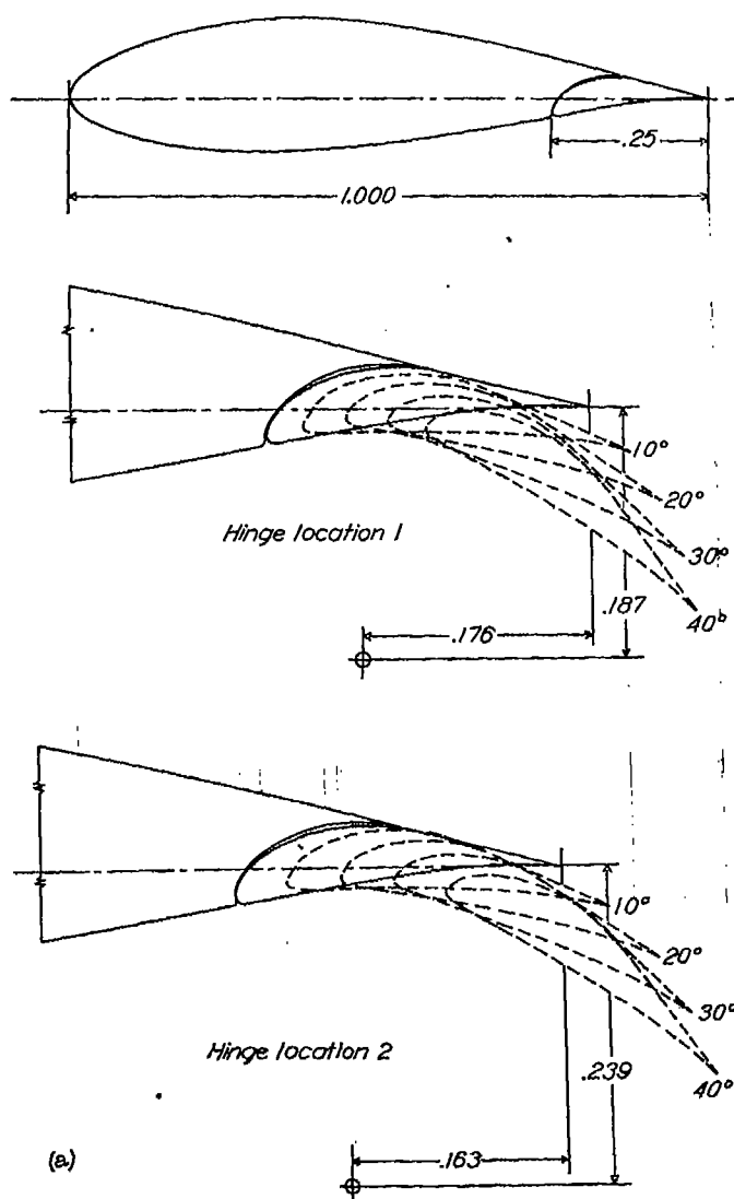
FIGURE 55.—Flap configuration and maximum lift coefficients for the NACA 63,4-420 airfoil with a 0.25-airfoil-chord hinged slotted flap. R=6 \times 10^6
