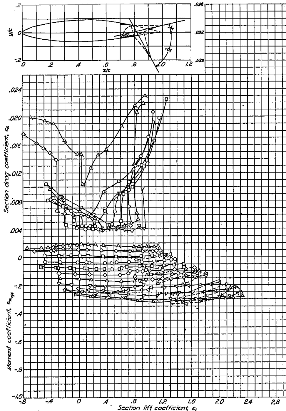
Aerodynamic characteristics of the NACA 66(215)-216 airfoil section with 0.20s sealed plain flap. R=6 \times 10^4 .
