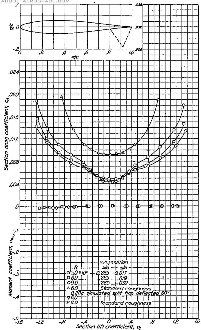
Aerodynamic characteristics of the NACA 63-012 airfoil section, 24-inch chord.
