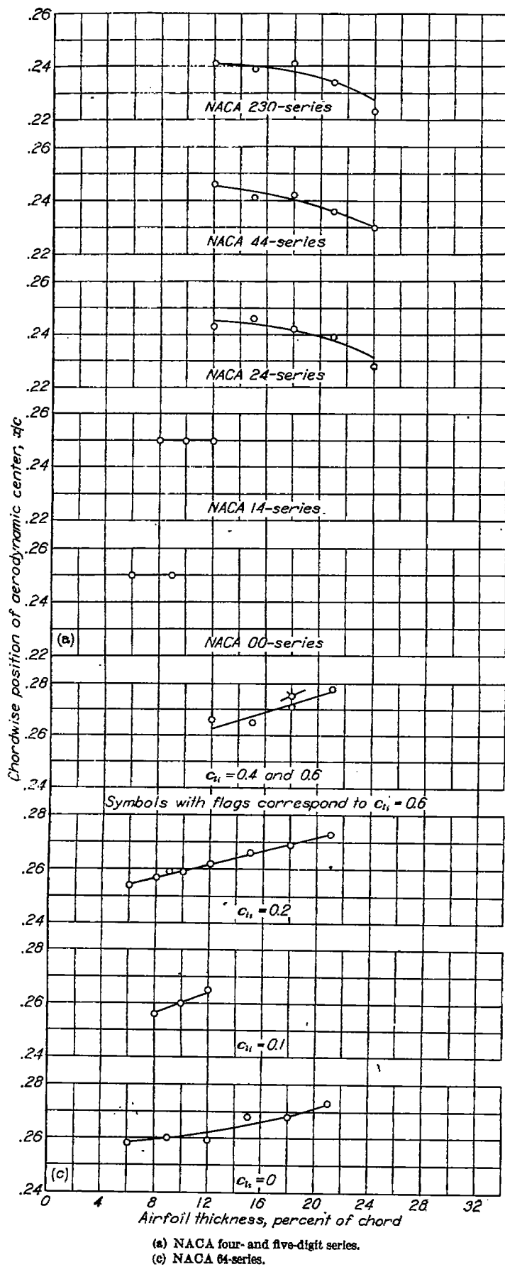
FIGURE 52.—Variation of section chordwise position of the aerodynamic center with airfoil thickness ratio for several NACA airfoil sections of different cambers. R=6 \times 10^6 .
