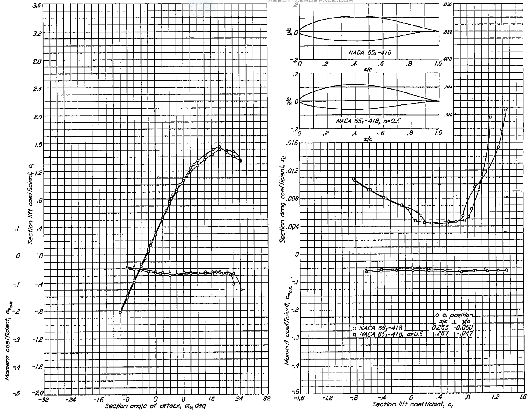
FIGURE 16. —Comparison of the aerodynamic characteristics of the NACA 653-418 and NACA 653-418, a = 0.5 airfoils at a Reynolds number of 9 \times 10^6 . T.D.T. tests 814, 820, 406, and 411.
