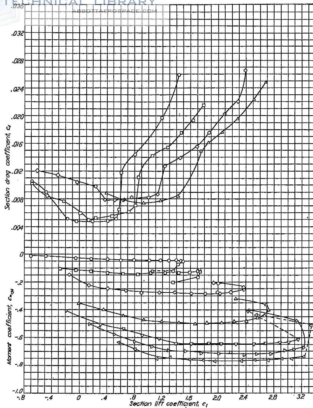
(b) Aerodynamic characteristics, R=6 \times 10^6 , NACA 65-118 airfoil section with 0.309c double slotted flap.
