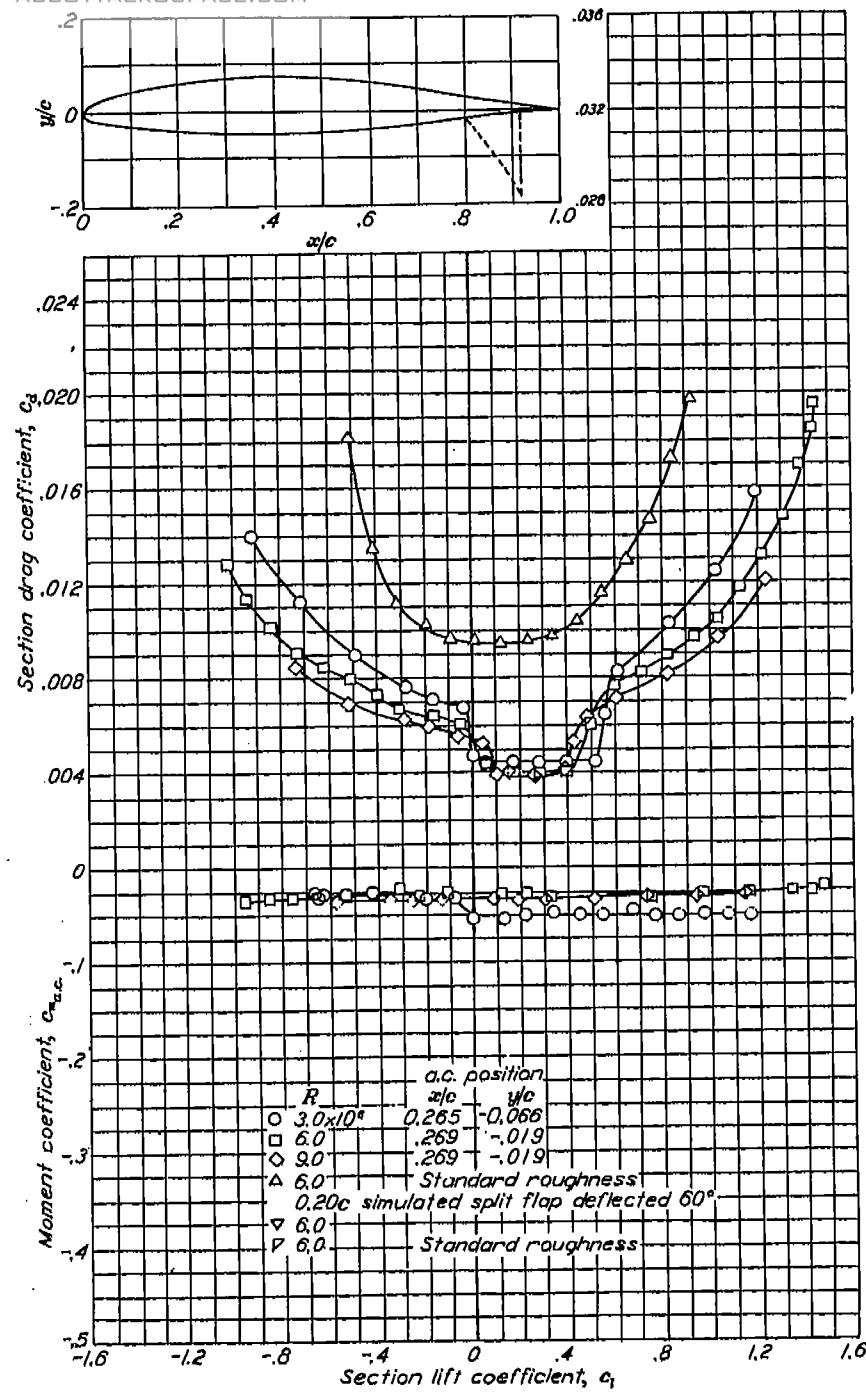
Aerodynamic characteristics of the NACA 65-212, \alpha=0.6 airfoil section, 24-inch chord.
