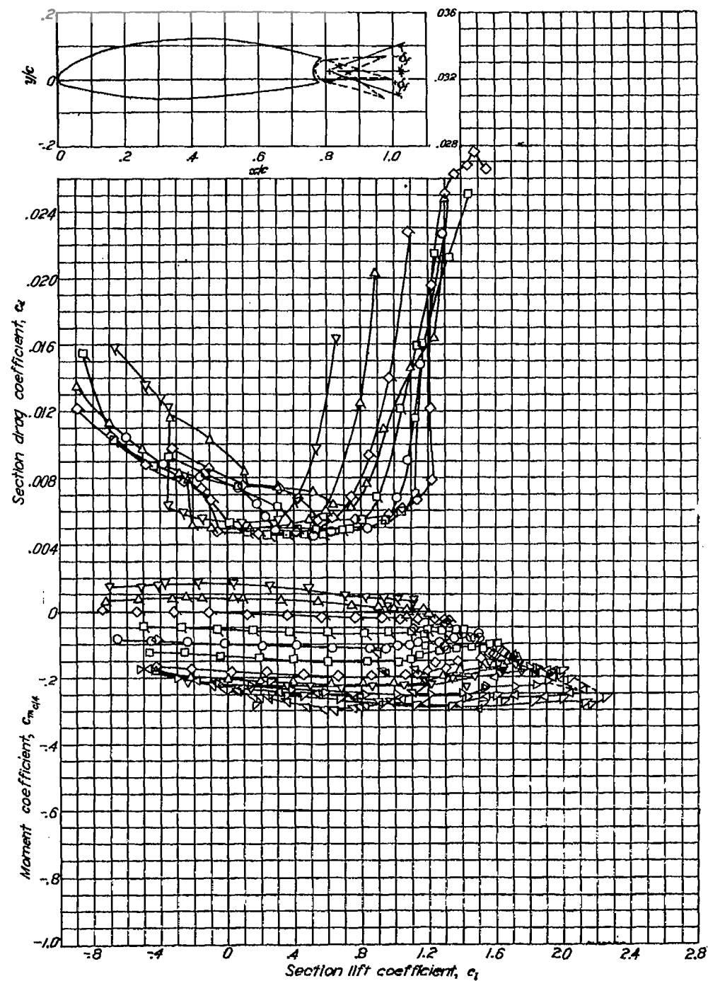
Aerodynamic characteristics of the NACA 65,3-618 airfoil section with 0.30c sealed plain flap. R=6 \times 10^6 .
