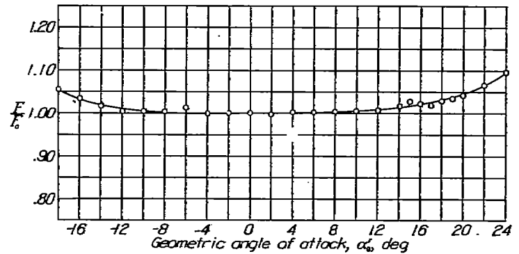
FIGURE 68.—Additional blocking factor at the tunnel walls plotted against angle of attack for the NACA 64-418 airfoil.
