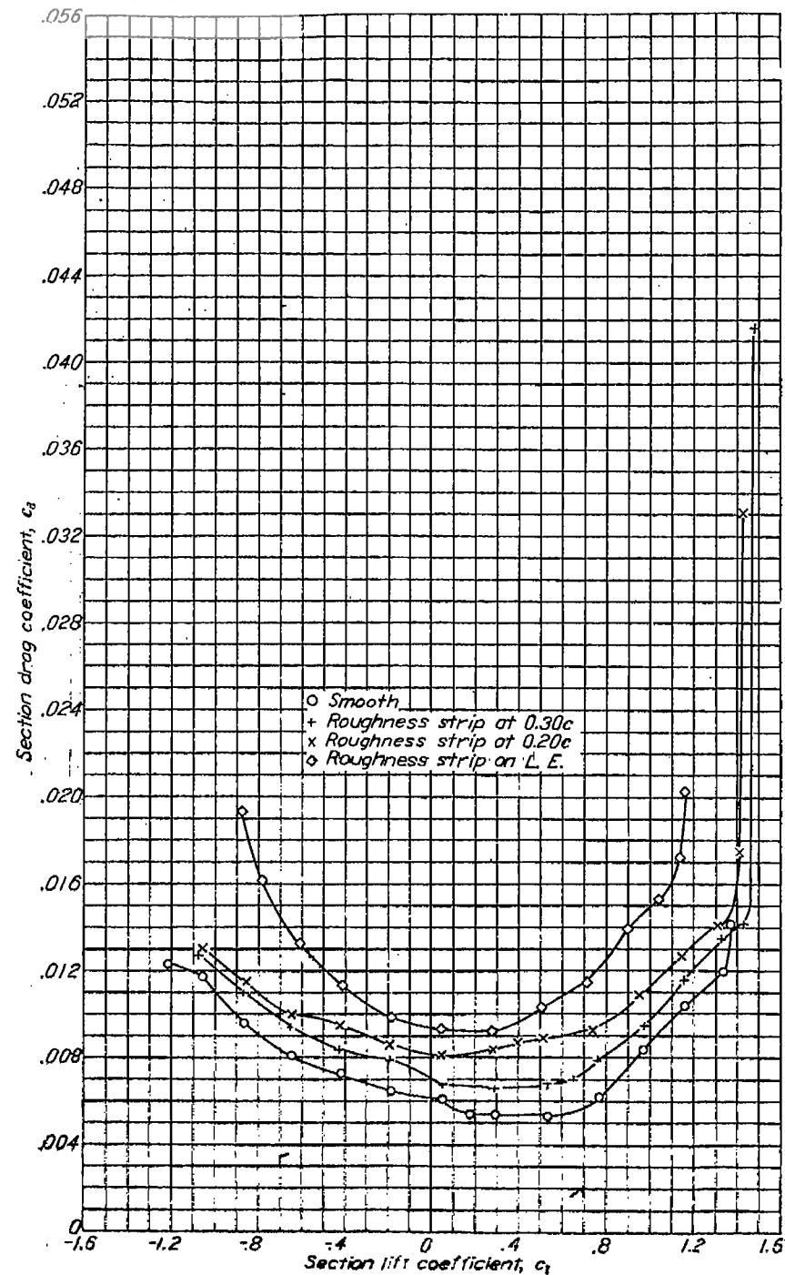
FIGURE 24.—Lift and drag characteristics of an NACA 63(420)-422 airfoil with 0.011-inch-grain roughness at various chordwise locations.
