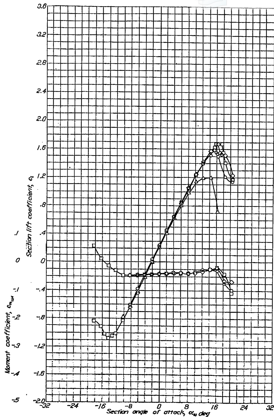
Aerodynamic characteristics of the NACA 2412 airfoil section, 24-inch chord.
