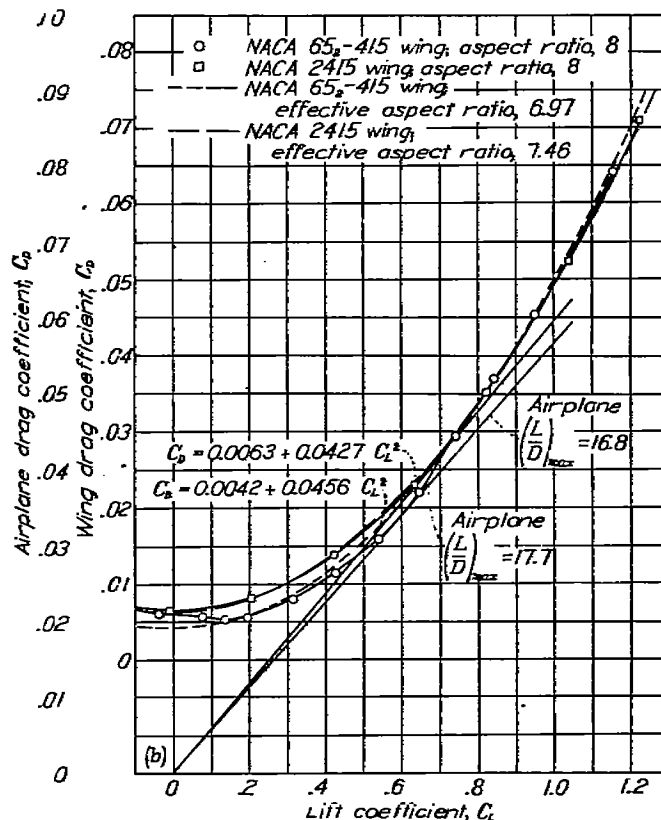
(b) NACA 65 3 -415 and 2415 wings of aspect ratio 8.
