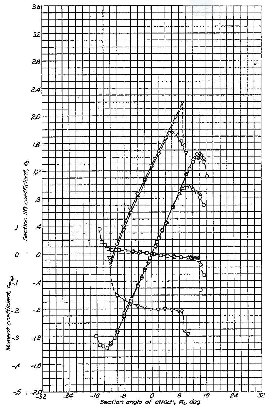
Aerodynamic characteristics of the NACA 63-012 airfoil section, 24-inch chord.
