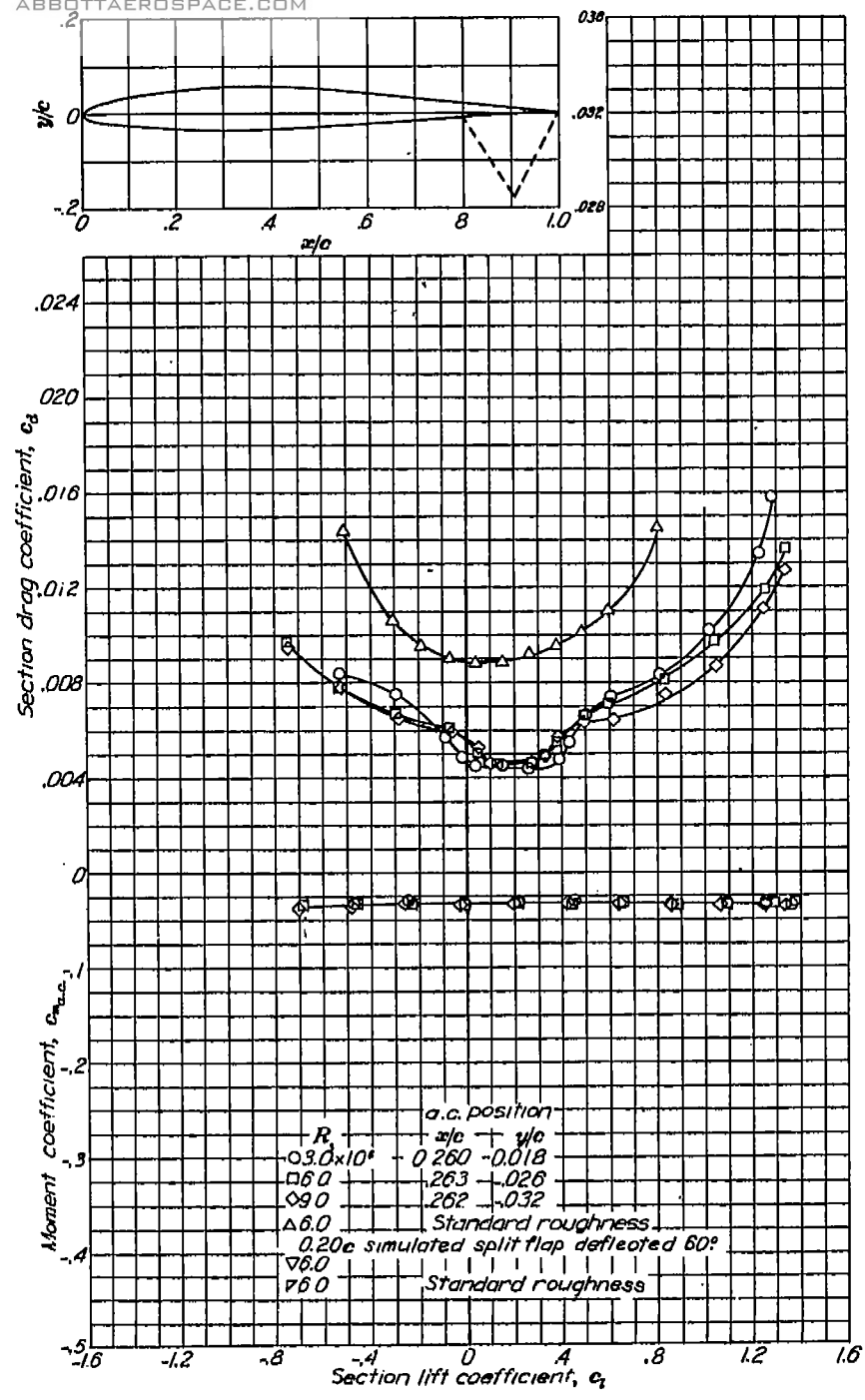
Aerodynamic characteristics of the NACA 63-209 airfoil section, 24-inch chord.
