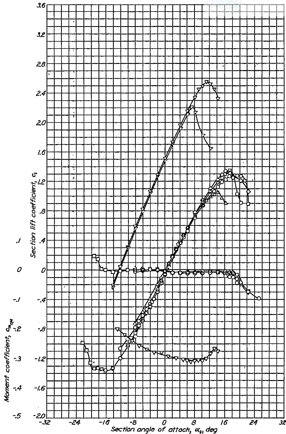
Aerodynamic characteristics of the NACA 66-018 airfoil section, 24-inch chord.
