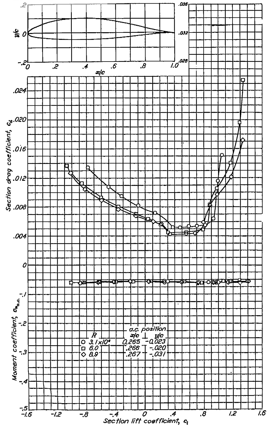
Aerodynamic characteristics of the NACA 65(216)-415, \alpha = 0.5 airfoil section, 24-inch chord.
