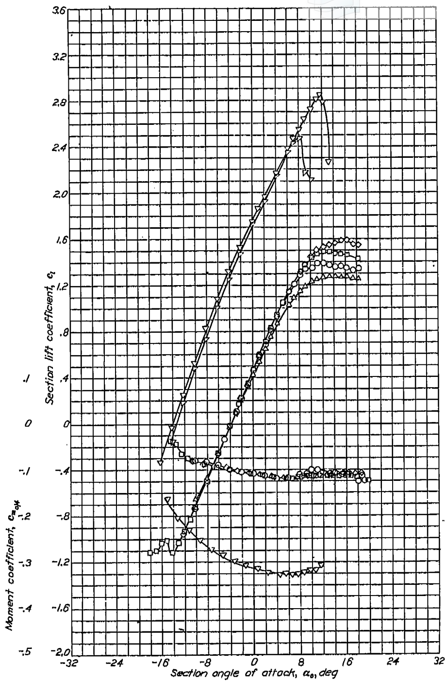
Aerodynamic characteristics of the NACA 63-618 airfoil section, 24-inch chord.
