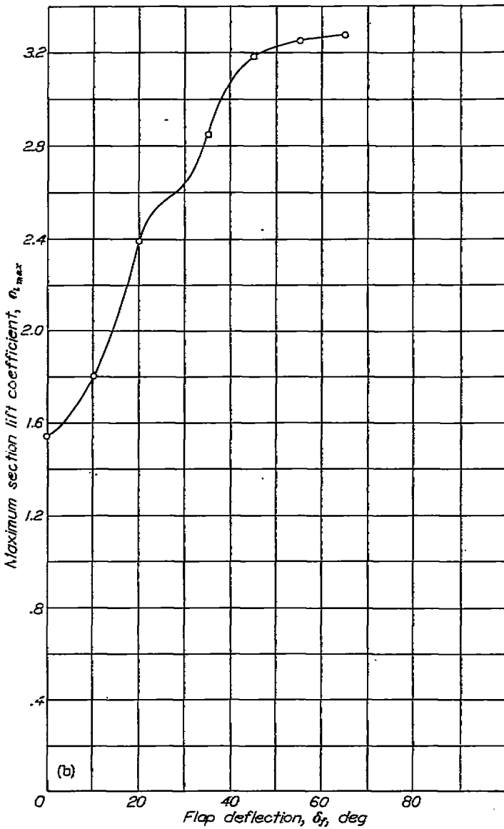
FIGURE 56.—Flap configuration and maximum lift coefficients for the NACA 65-118 airfoil with a double slotted flap. R=6 \times 10^6 .
