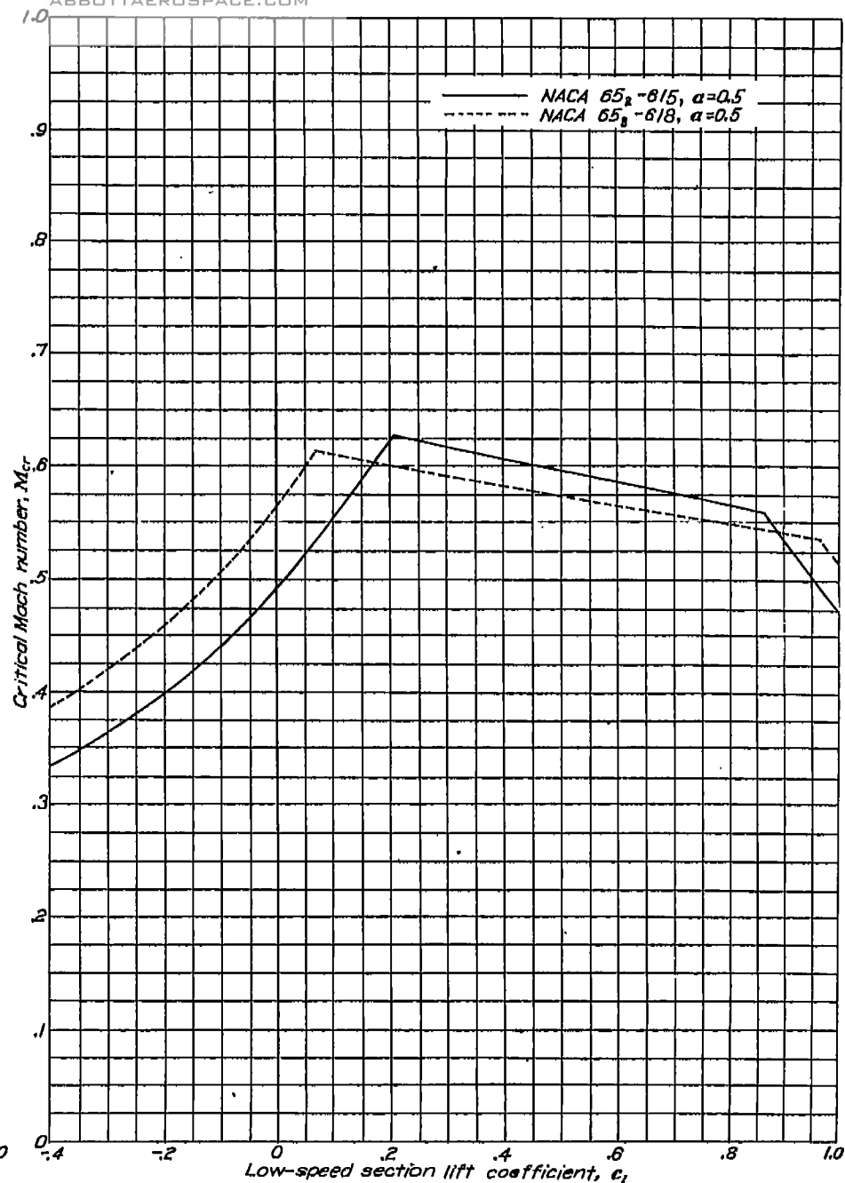
Variation of critical Mach number with low-speed section lift coefficient for two NACA 65-series airfoil sections with mean line of the type a=0.5 , with different thicknesses, and cambered for a design lift coefficient of 0.6.
