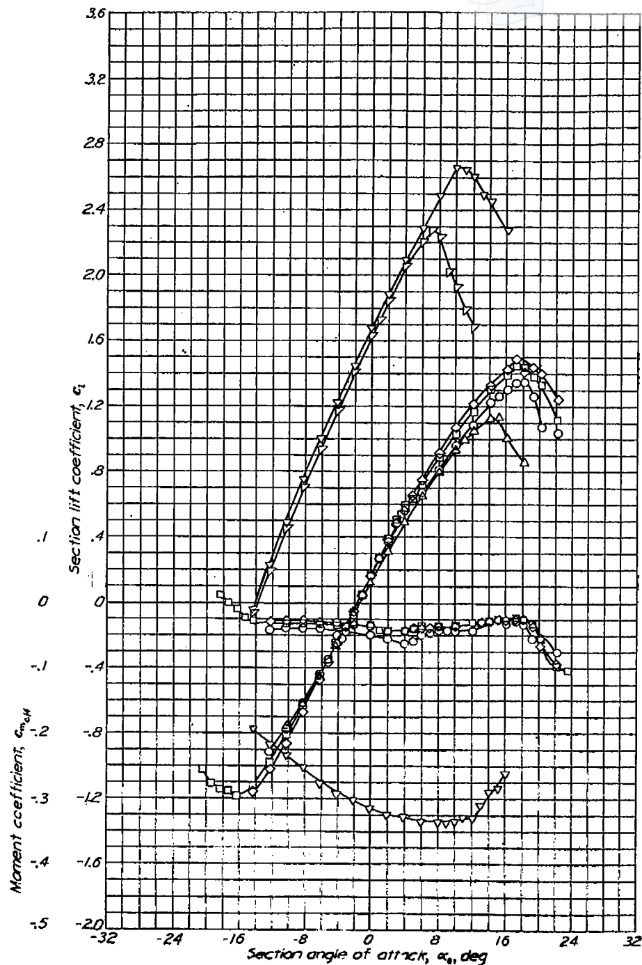
Aerodynamic characteristics of the NACA 66-218 airfoil section, 24-inch chord.
