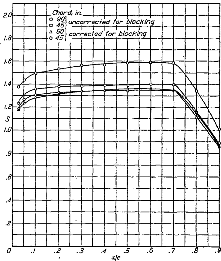
FIGURE 71.—Comparison between corrected and uncorrected pressure distributions for two chord sizes of a symmetrical NACA 6-series airfoil of 16-percent thickness. \alpha = 0^\circ
