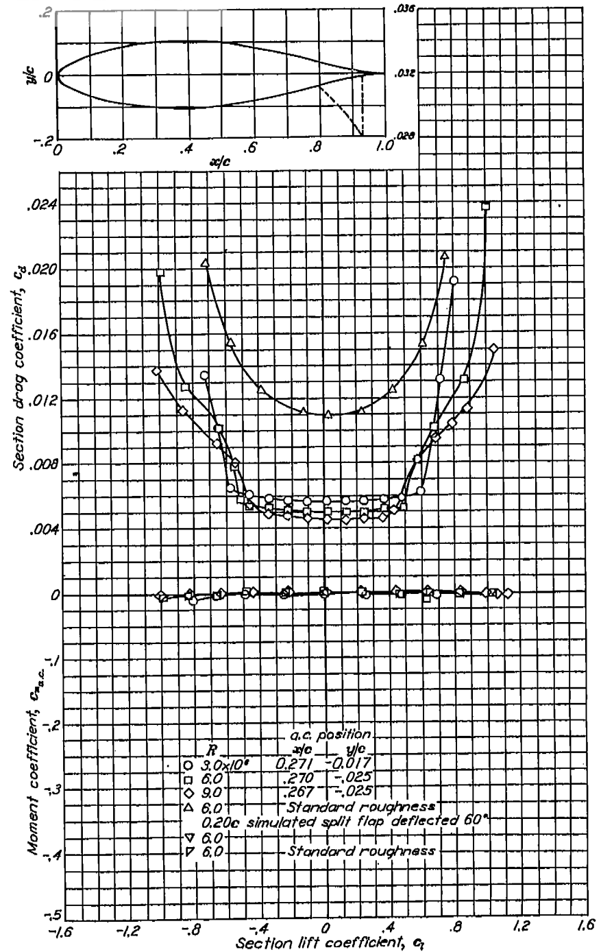
Aerodynamic characteristics of the NACA 654-021 airfoil section, 24-inch chord.
