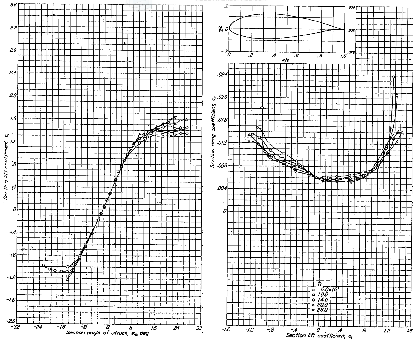
FIGURE 42.—Lift and drag characteristics of the NACA 63(420)-422 airfoil at high Reynolds number TDT tests 228 and 265.
