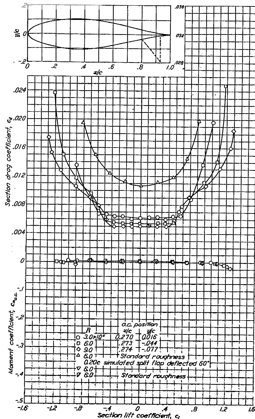
Aerodynamic characteristics of the NACA 64-021 airfoil section, 24-inch chord.
