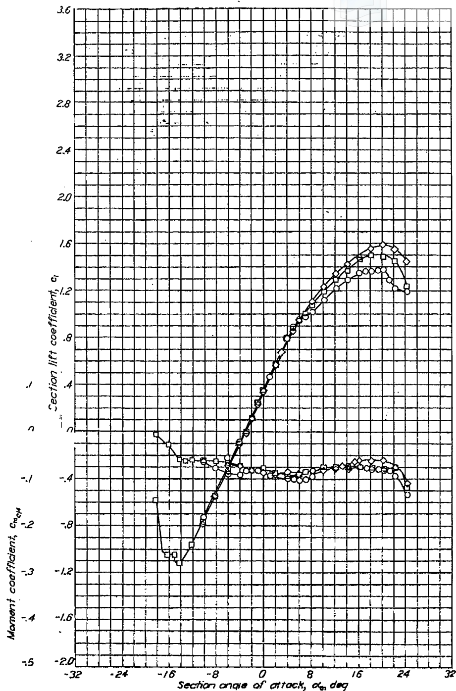
Aerodynamic characteristics of the NACA 65,3-418, \alpha = 0.8 airfoil section, 24-inch chord.
