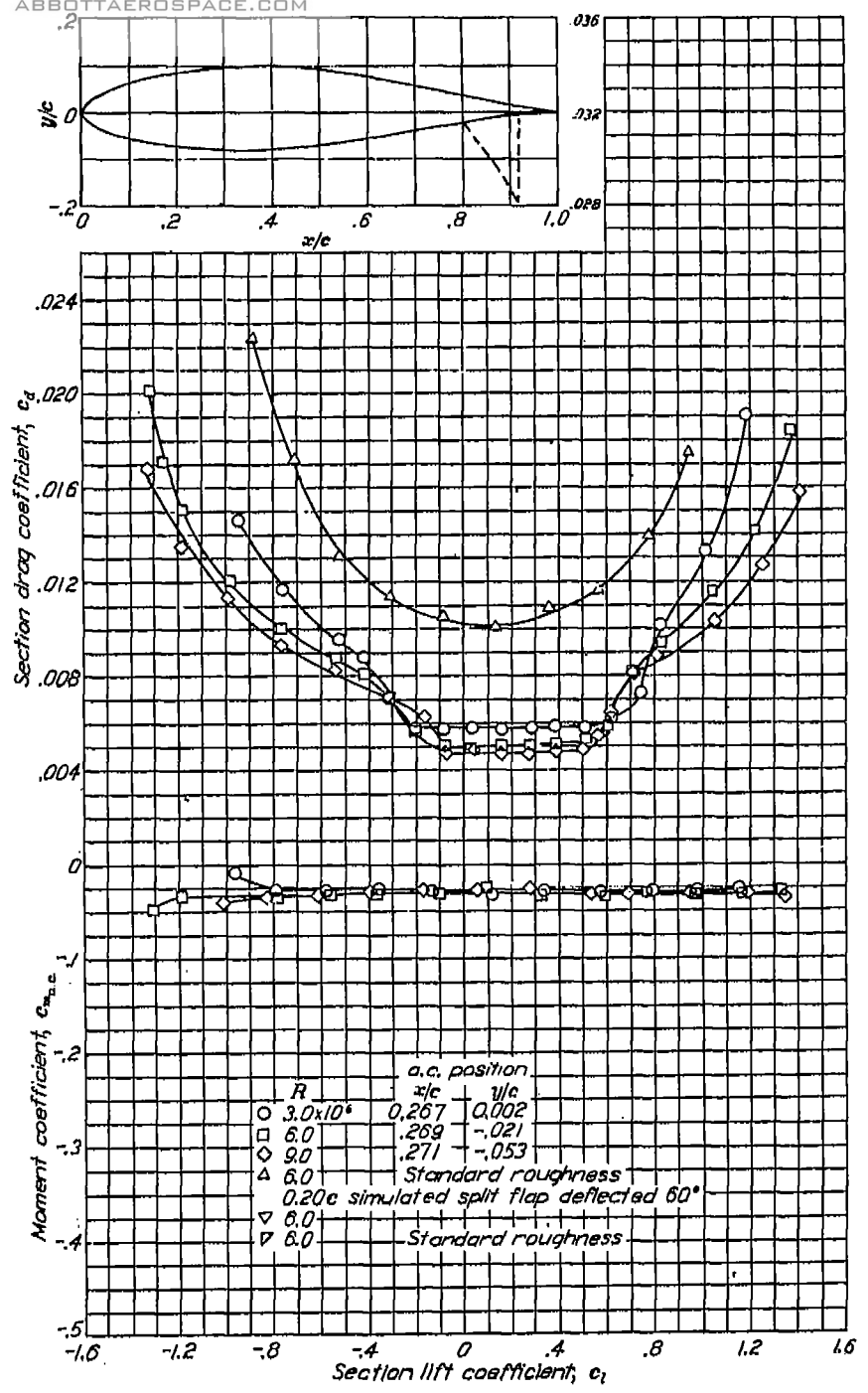
Aerodynamic characteristics of the NACA 64-218 airfoil section, 24-inch chord.
