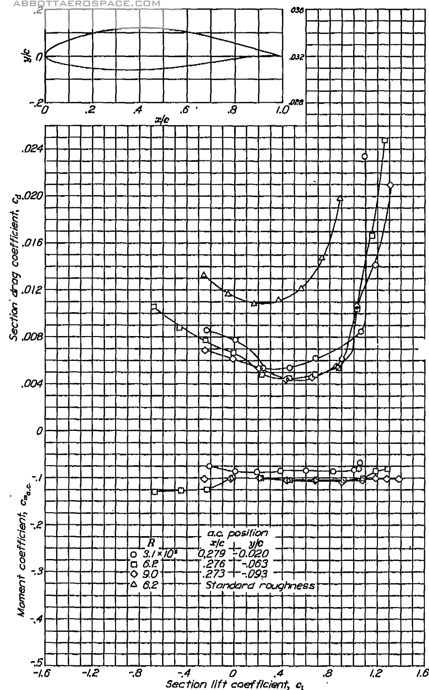
Aerodynamic characteristics of the NACA 65,3-618 airfoil section, 24-inch chord.
