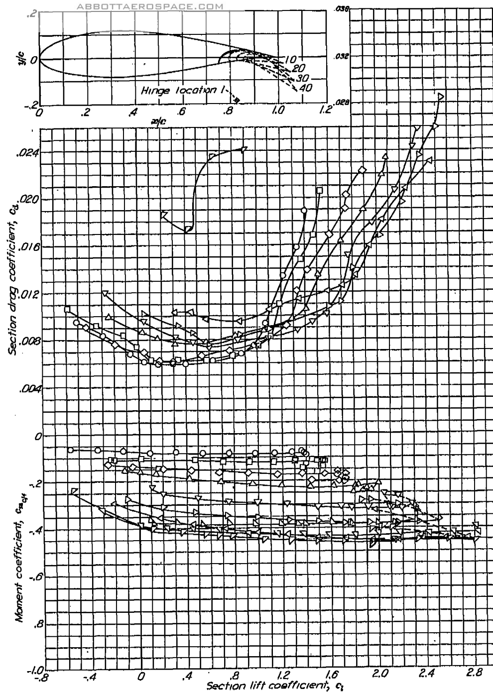
(b) Aerodynamic characteristics with hinge location 1, R = 6 \times 10^4 . NACA 63,4-420 airfoil section with 0.25c slotted flap.
