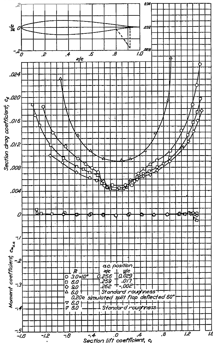
Aerodynamic characteristics of the NACA 64-012 airfoil section, 24-inch chord.
