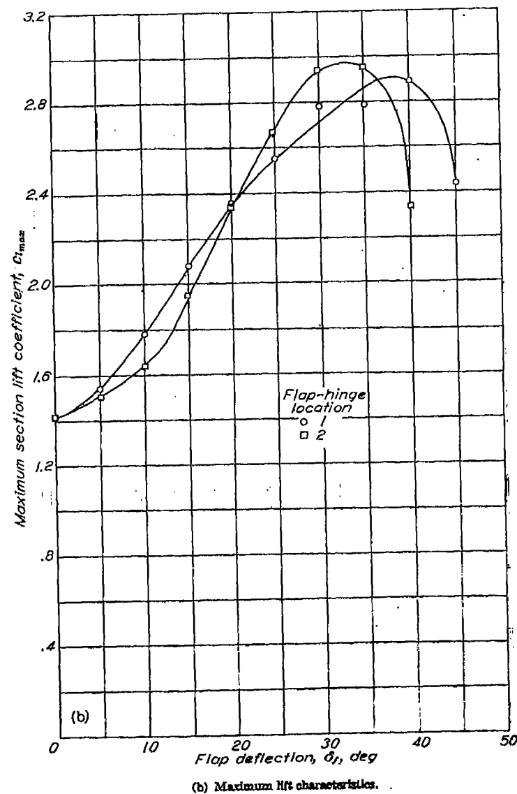
FIGURE 55.—Flap configuration and maximum lift coefficients for the NACA 63,4-420 airfoil with a 0.25-airfoil-chord hinged slotted flap. R=6 \times 10^6
