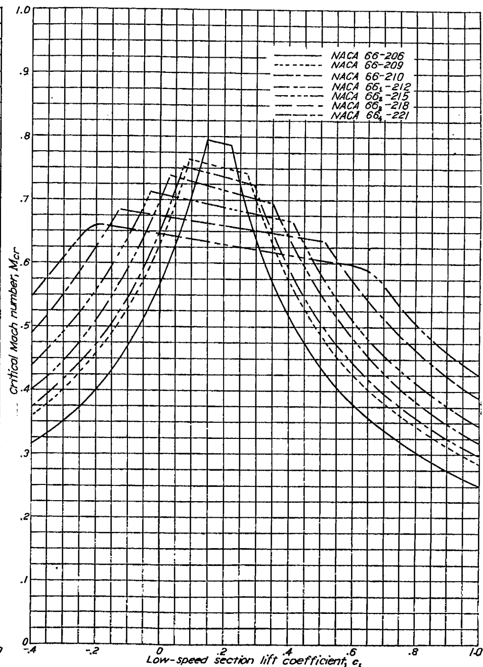
Variation of critical Mach number with low-speed section lift coefficient for several NACA 66-series airfoil sections of various thicknesses, cambered for a design lift coefficient of 0.2.
