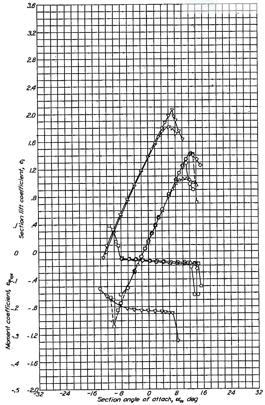
Aerodynamic characteristics of the NACA 63-209 airfoil section, 24-inch chord.
