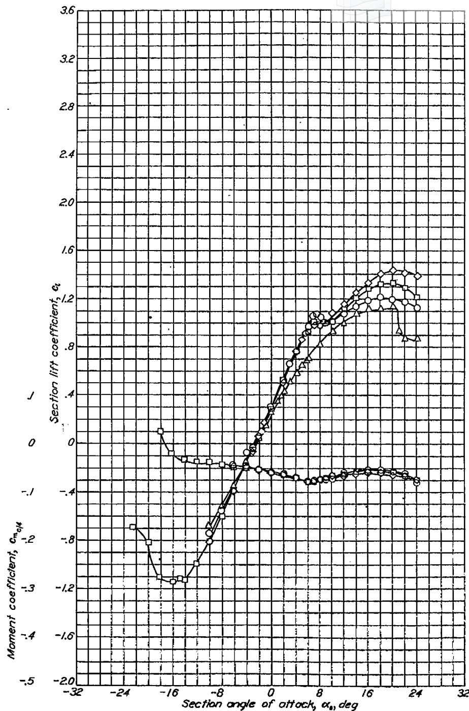
Aerodynamic characteristics of the NACA 65-121, \alpha=0.5 airfoil section, 24-inch chord.
