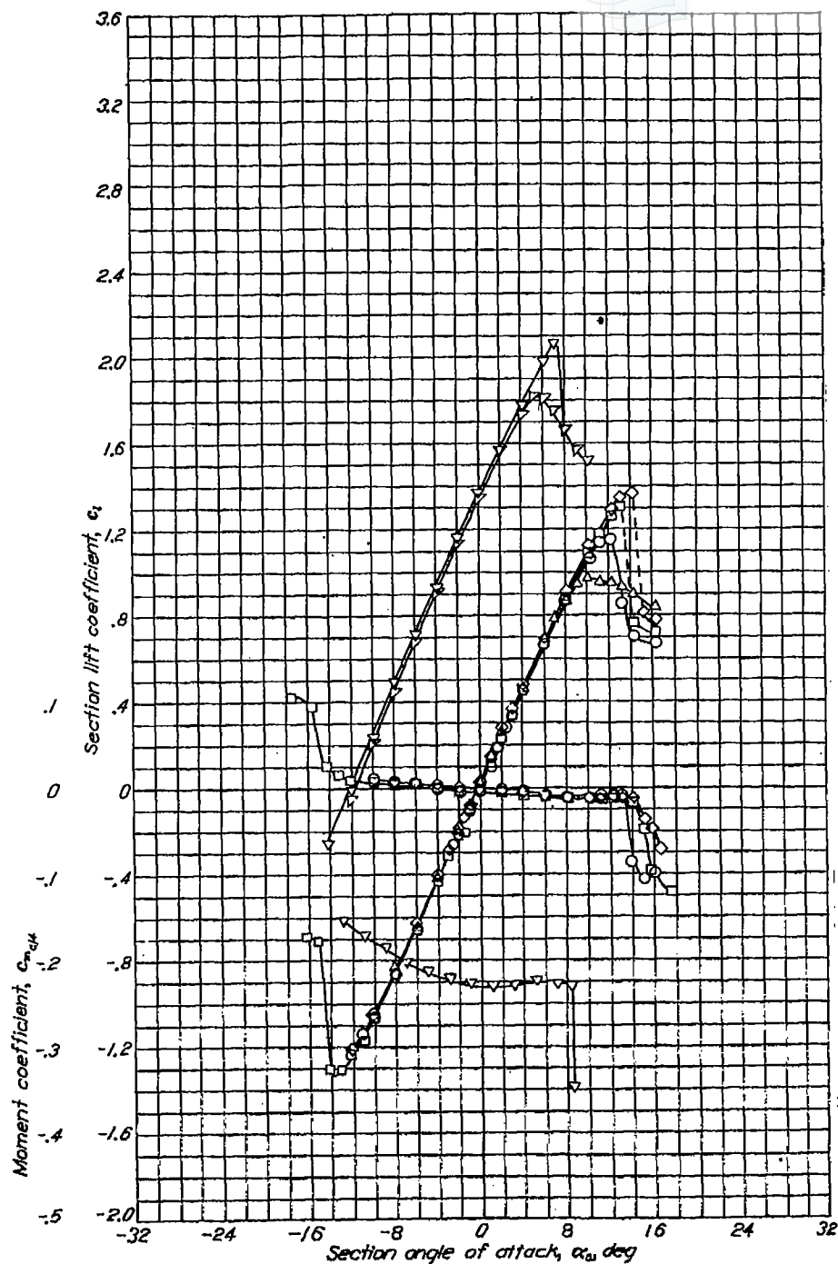
Aerodynamic characteristics of the NACA 651-012 airfoil section, 24-inch chord.
