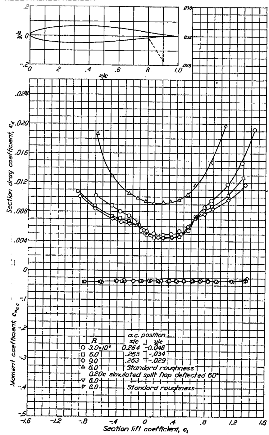
Aerodynamic characteristics of the NACA 631-212 airfoil section, 34-inch chord.
