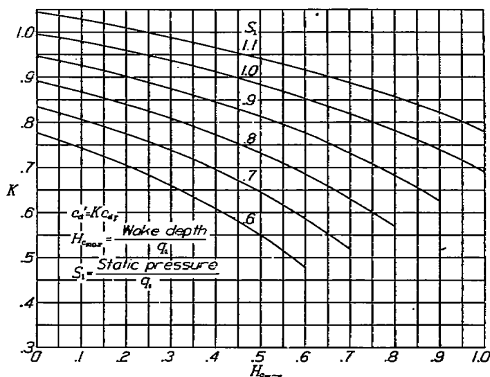
FIGURE 66.—Plot of K as a function of H_{c_{max}} with S_1 as a parameter.
