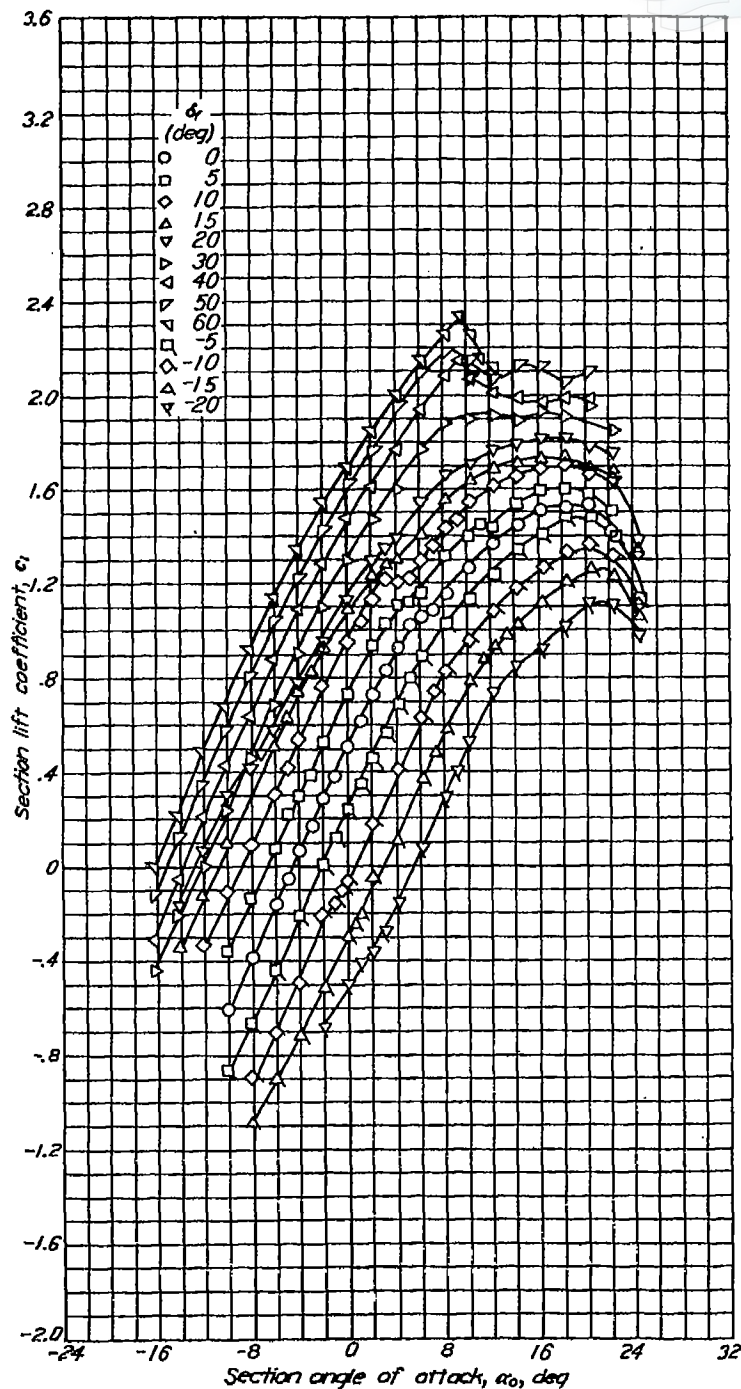
Aerodynamic characteristics of the NACA 65,3-618 airfoil section with 0.30c sealed plain flap. R=6 \times 10^6 .
