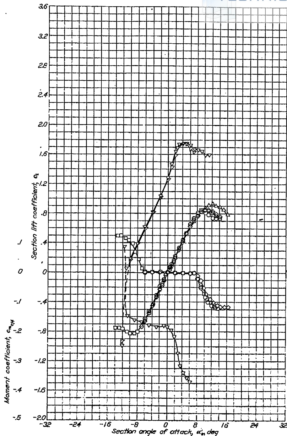
Aerodynamic characteristics of the NACA 65-006 airfoil section, 24-inch chord.
