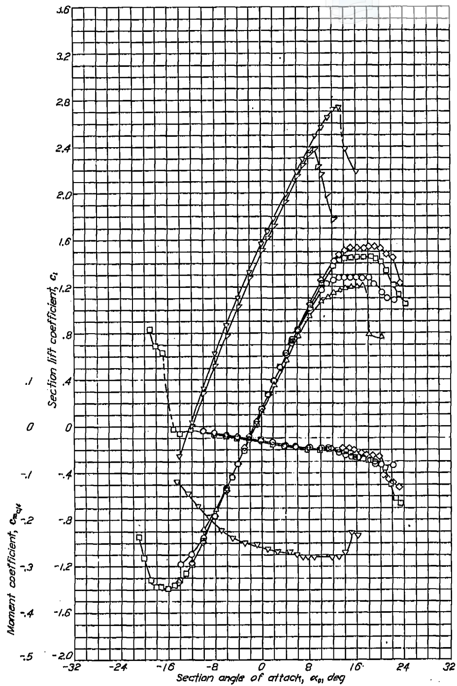
Aerodynamic characteristics of the NACA 64-218 airfoil section, 24-inch chord.
