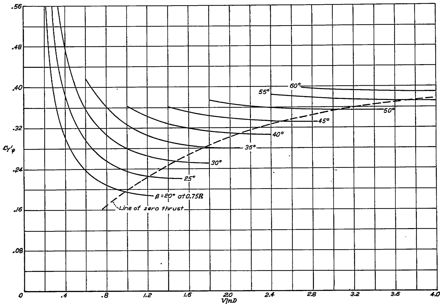
FIGURE 11.—Side-force derivative for single-rotating NACA propeller 10-3062-045 with spinner. Three blades; \sigma=0.124 .
