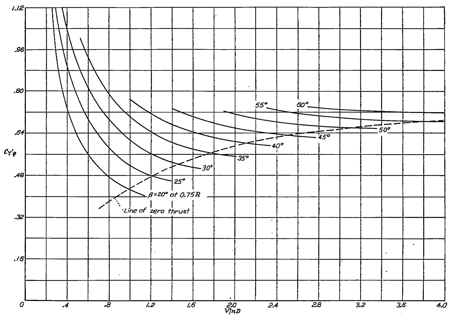
FIGURE 13.—Side-force derivative for dual-rotating NACA propeller 10-3062-045 with spinner. Six blades; \sigma = 0.247 .
