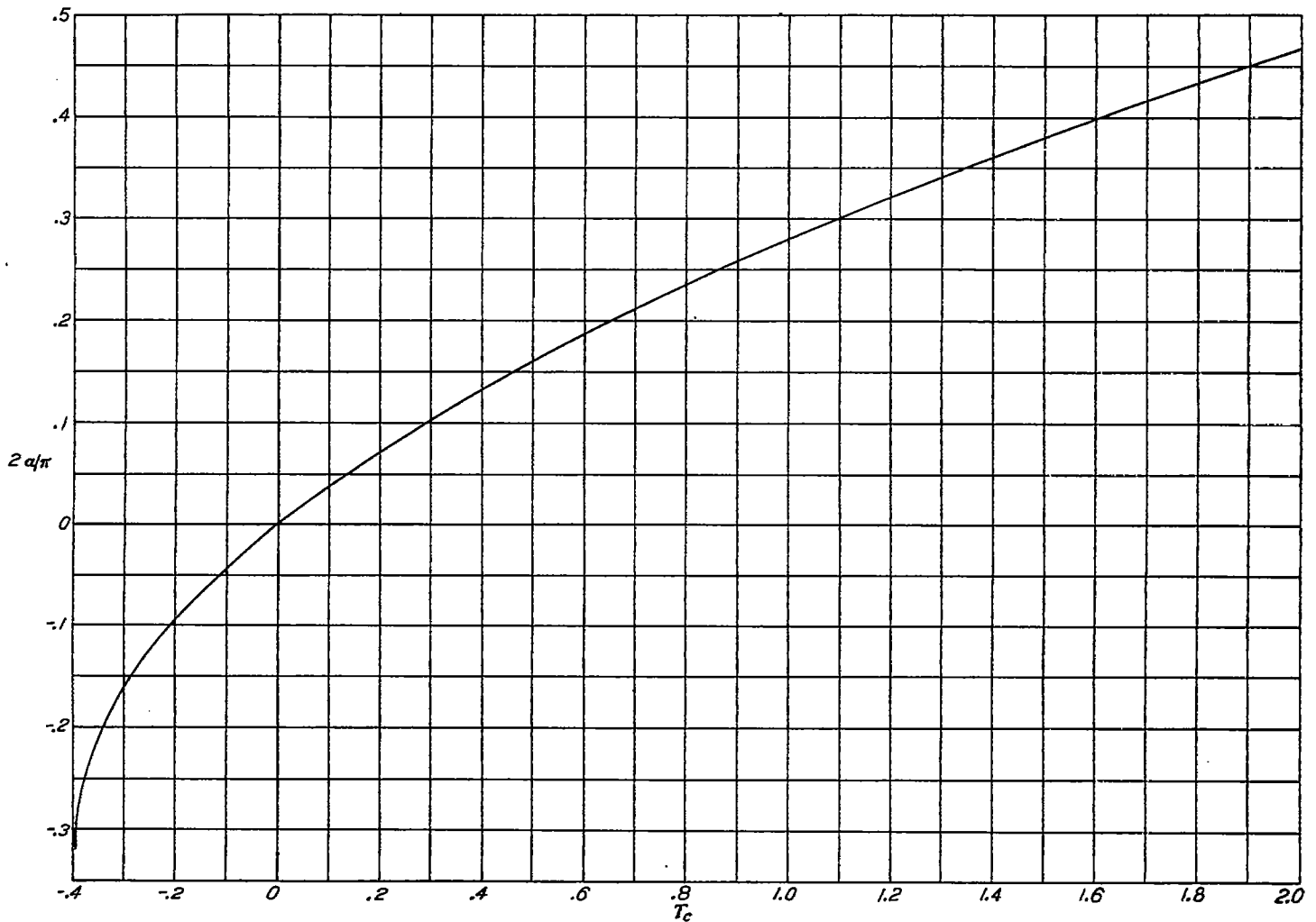
FIGURE 3.—Variation of 2a/\pi with T_c . T_c = \frac{C_T}{(V/nD)^2}
