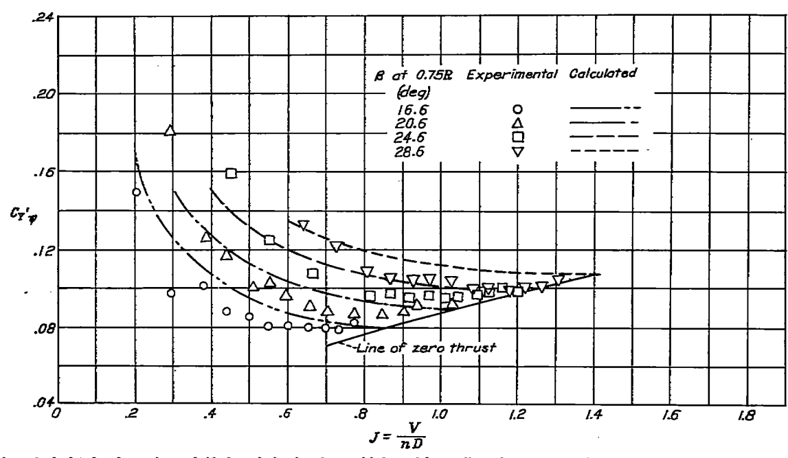
FIGURE 14.—Comparison of calculated and experimental side-force derivatives for two-blade model propeller. Curves are terminated, except for \beta = 16.6^\circ , at point where obvious stalling of blades occurs. Experimental data from reference 4.
