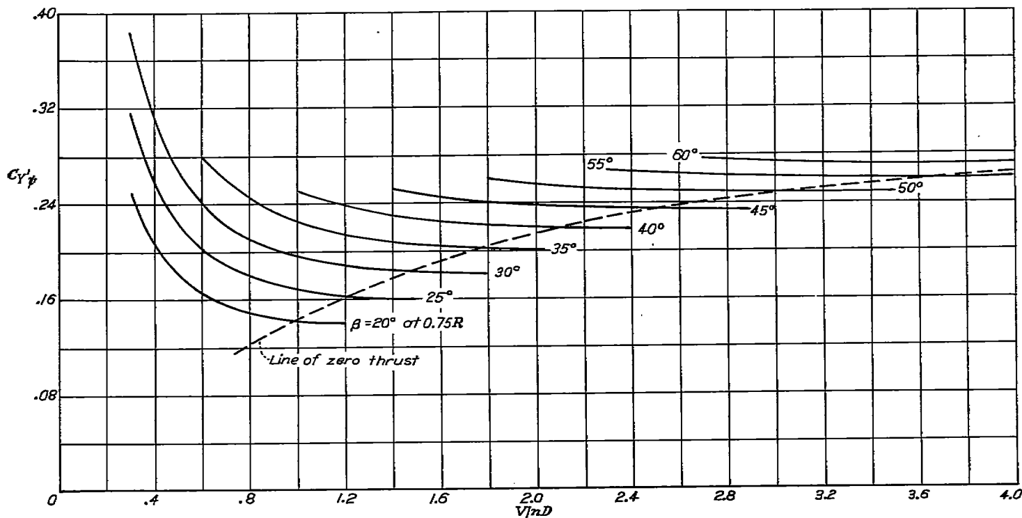
FIGURE 10.—Side-force derivative for single-rotating NACA propeller 10-3062-045 with spinner. Two blades; \sigma=0.0625 .
