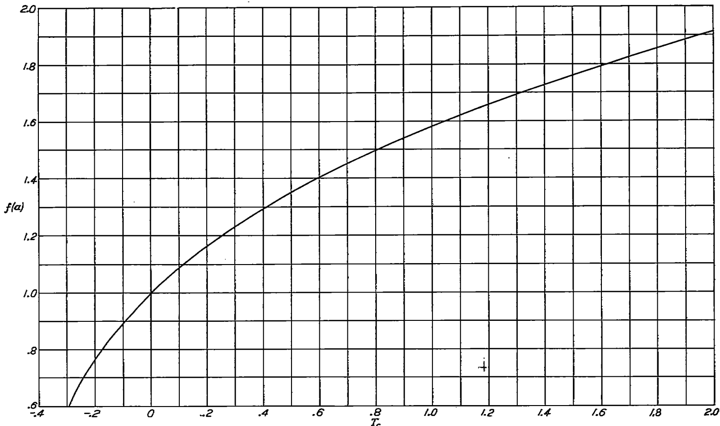
FIGURE 1.—Variation of q -factor f(a) with T_c . T_c = \frac{C_T}{(V/\pi D)^2}
