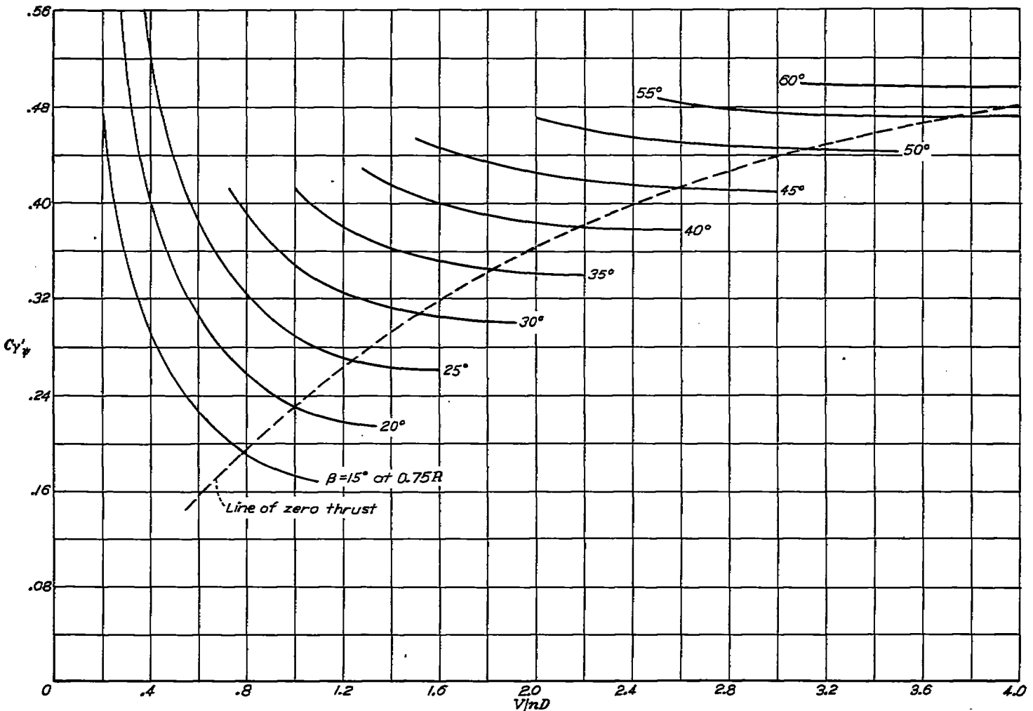
FIGURE 8.—Side-force derivative for single-rotating Hamilton Standard propeller 3155-6 with spinner. Six blades; \epsilon=0.182 .
