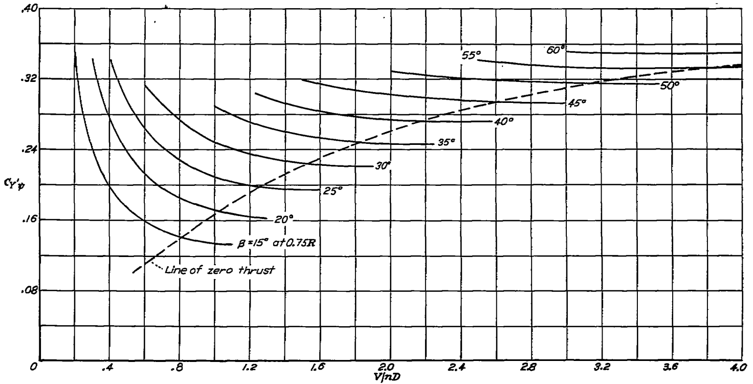
FIGURE 7.—Side-force derivative for single-rotating Hamilton Standard propeller 3155-6 with spinner. Four blades; \epsilon=0.121 .
