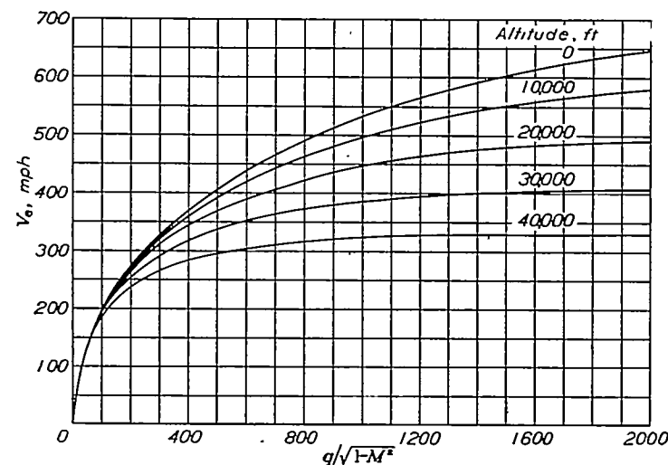
FIGURE 5.—Variation of equivalent airspeed with the factor q/\sqrt{1-M^2} .
