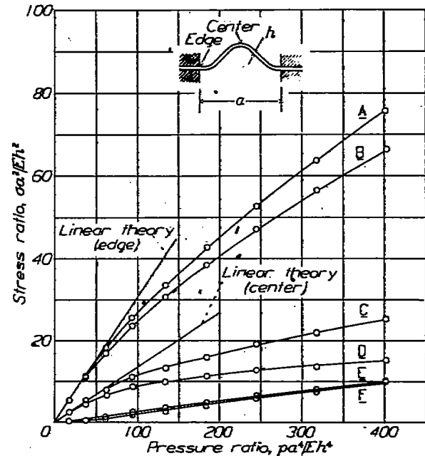
FIGURE 5.—Stresses perpendicular to edge at its midpoint and at the center of a clamped square plate in any direction. \mu , 0.316; \sigma''/Eh^2 , extreme-fiber bending stress ratio; \sigma'/Eh^2 , membrane stress ratio; \sigma''/Eh^2 , extreme-fiber stress ratio; pa^4/Eh^4 , pressure ratio.
