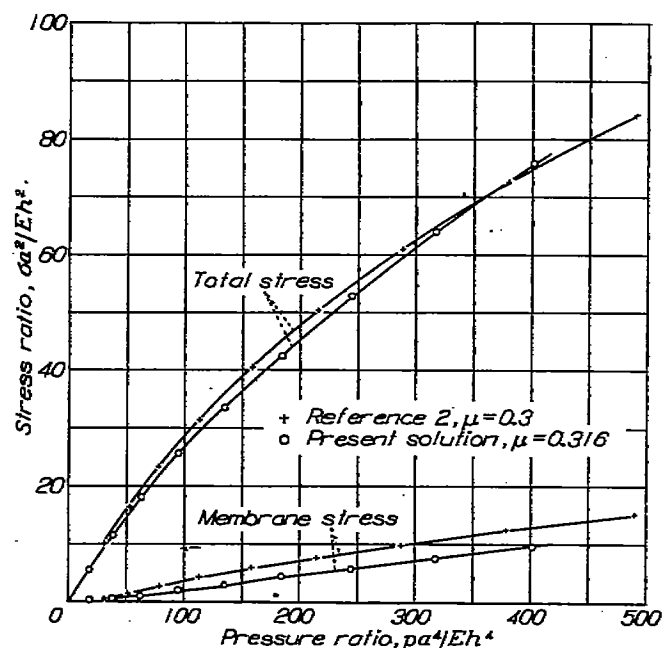
FIGURE 7.—Comparison of Way's solution (reference 2) using the Ritz energy method and the present solution for the total stress and the membrane stress perpendicular to the edge at its midpoint.
