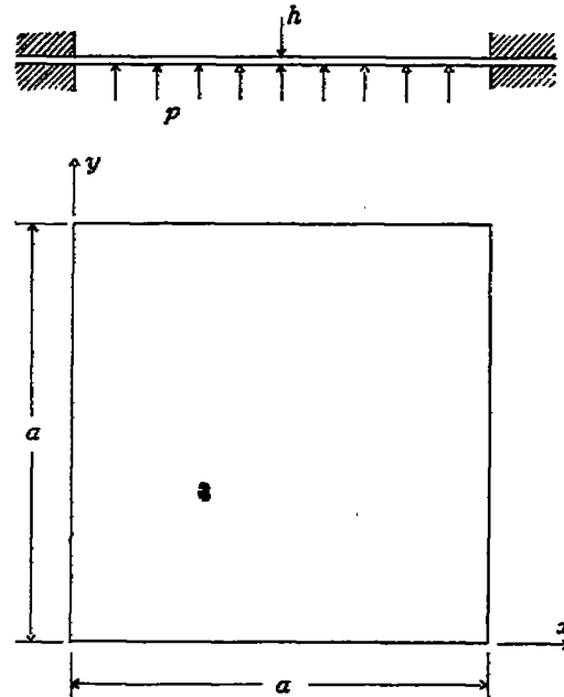
FIGURE 1.—Uniform normal pressure on a clamped square plate.
