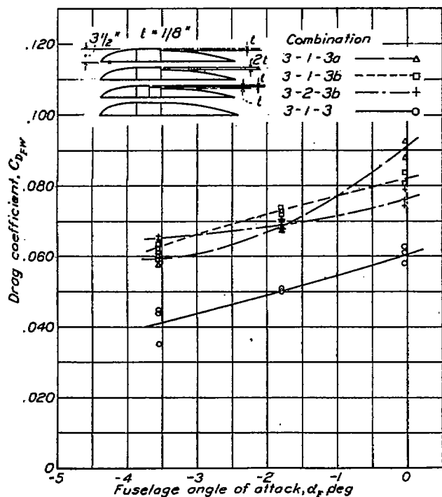
FIGURE 15.—Effect of steps for telescoping hoods. M , 0.34; V , 280 mph.
