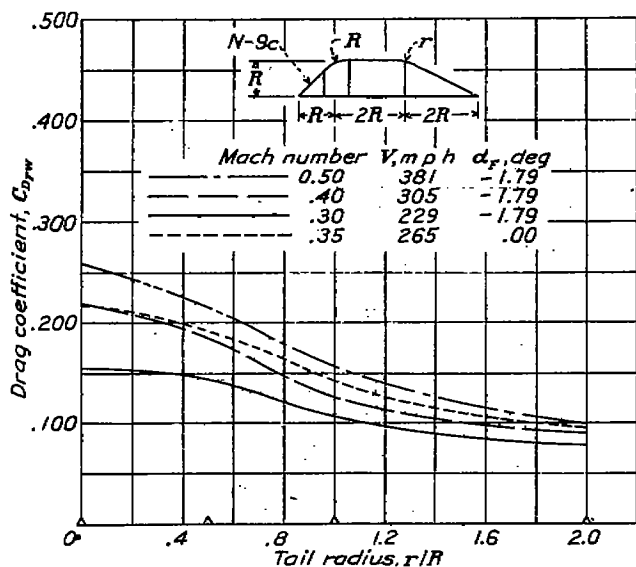
FIGURE 22.—Effect of radius at hood-tail juncture.
