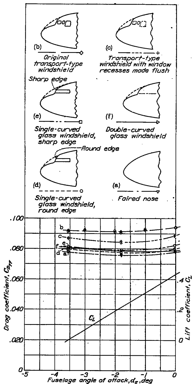
FIGURE 22.—Drag of fuselage with transport-type windshields. M , 0.35; V , 265 mph.
