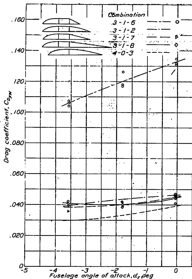
FIGURE 9.—Effect of tail length, conical shape. M, 0.34 ; V, 200 mph.
