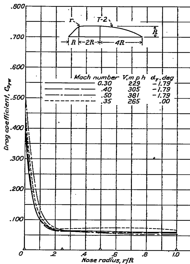
FIGURE 21.—Effect of radius at windshield-hood juncture.
