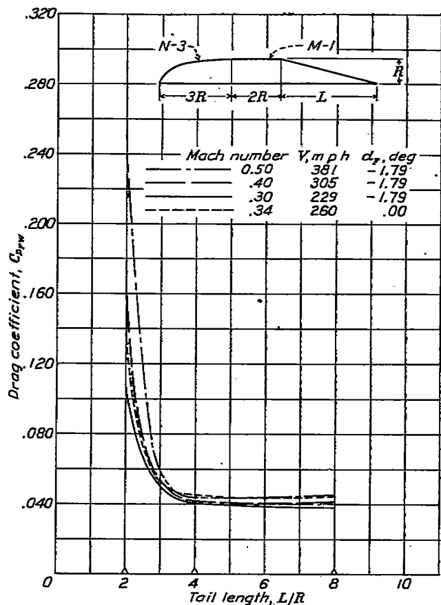
FIGURE 20.—Effect of tail length, conical shape.
