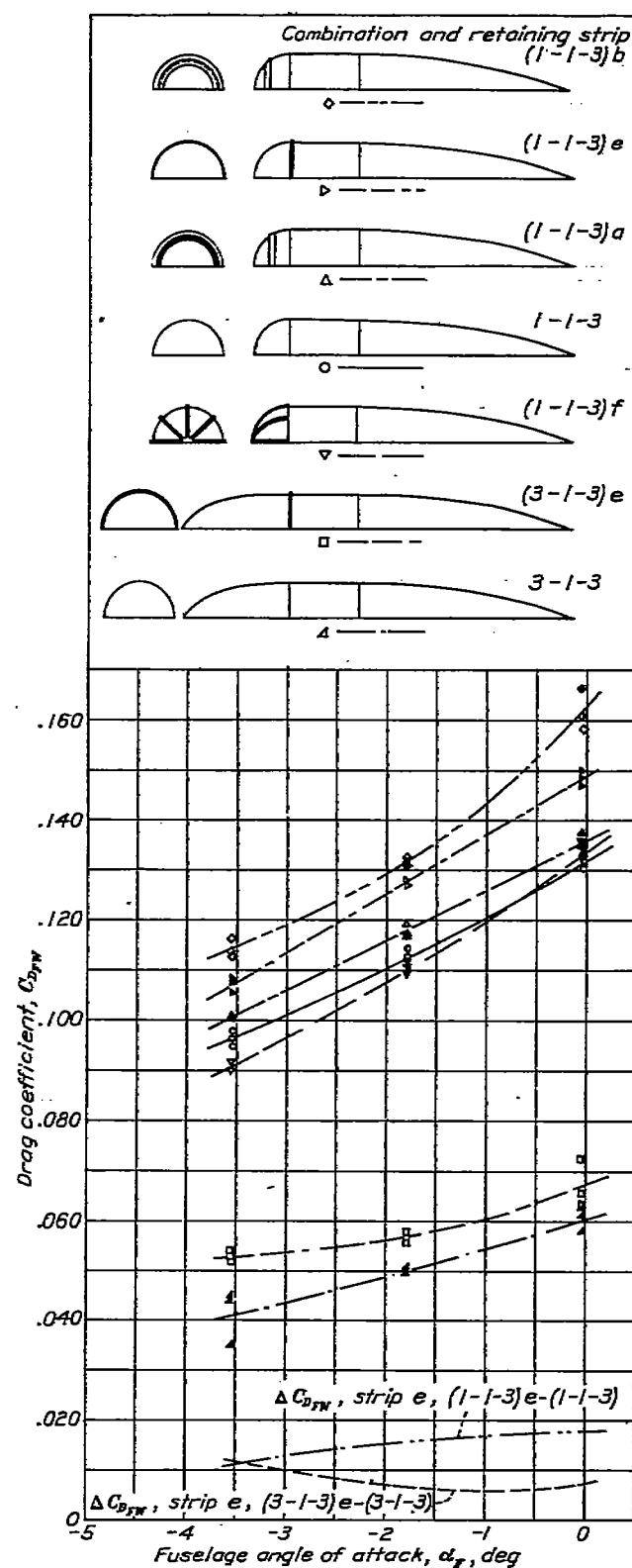
FIGURE 14.—Effect of retaining strips, combinations 1-1-3 and 3-1-3. M, 0.34 ; V, 260 mph.
