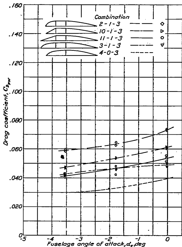
FIGURE 7.—Comparison between streamline and conical noses. M, 0.34 ; V, 260 mph.
