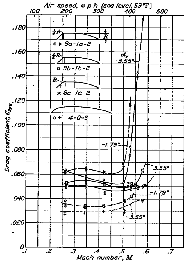
FIGURE 26.—Compressibility effect on windshields with various radii at nose-hood juncture.
