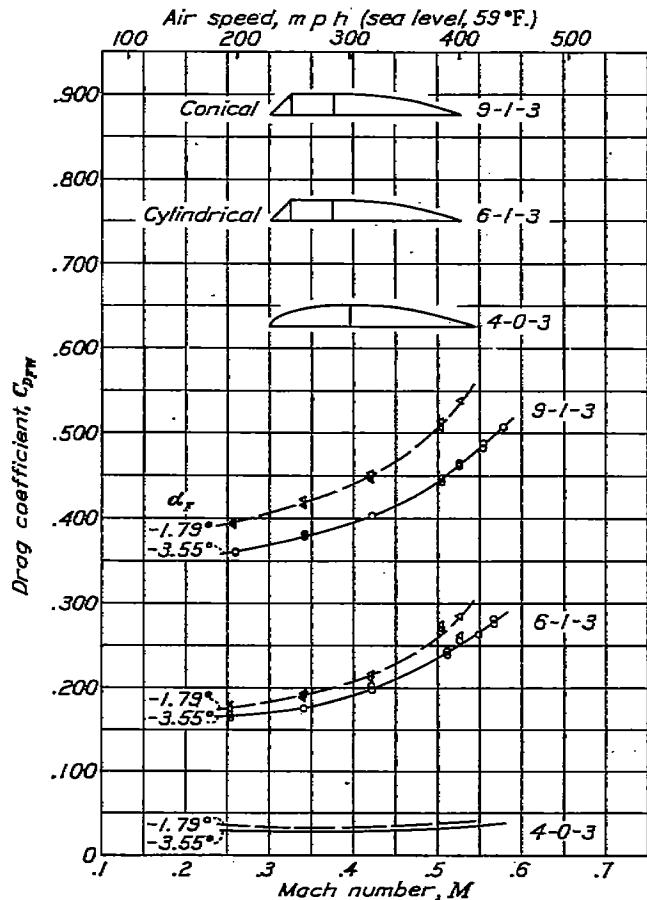
FIGURE 25.—Compressibility effect on windshield drag.
