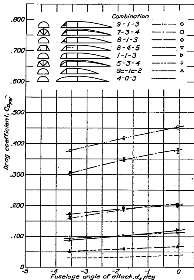
FIGURE 5.—Effect of nose shape of short length. M, 0.34 ; V, 260 mph.
