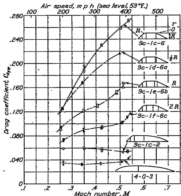
FIGURE 27.—Compressibility effect on windshields with various radii at hood-tail juncture. \alpha_r, -1.79^\circ .
