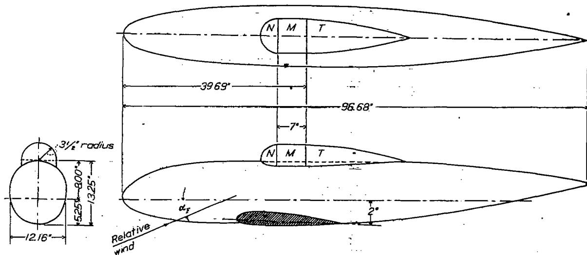
FIGURE 2.—Typical closed-cockpit windshield installation. Combination 1-1-3.
