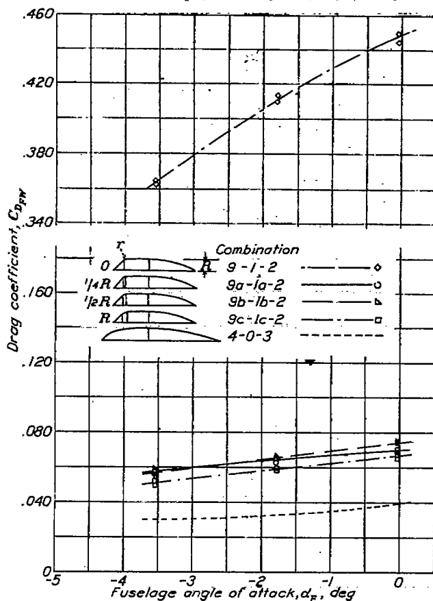
FIGURE 11.—Effect of radius at windshield-hood juncture. M, 0.35 ; V, 205 mph.
