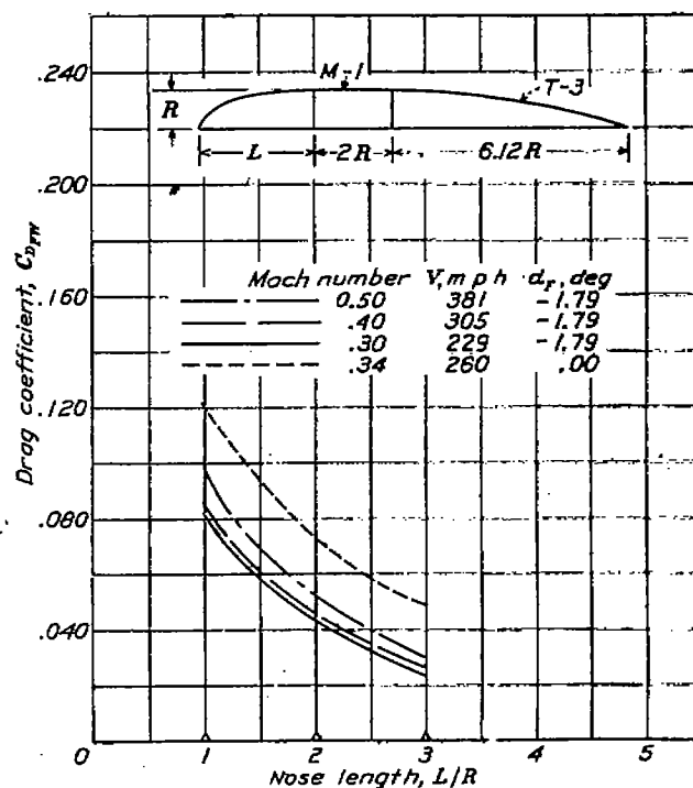
FIGURE 17.—Effect of nose length, streamline shape.
