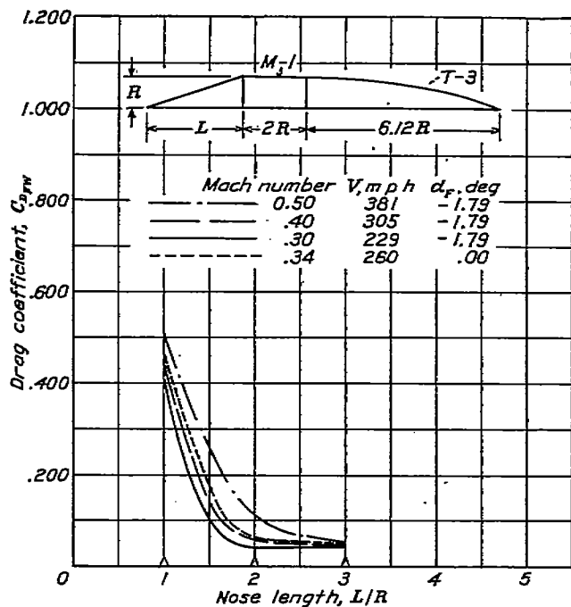
FIGURE 18.—Effect of nose length, conical shape.
