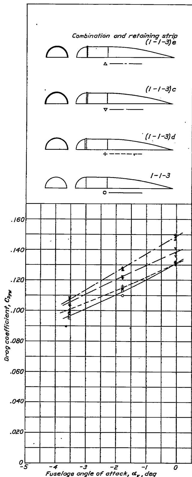
FIGURE 13.—Effect of retaining strips, combination 1-1-3. M, 0.34 ; V, 260 mph.
