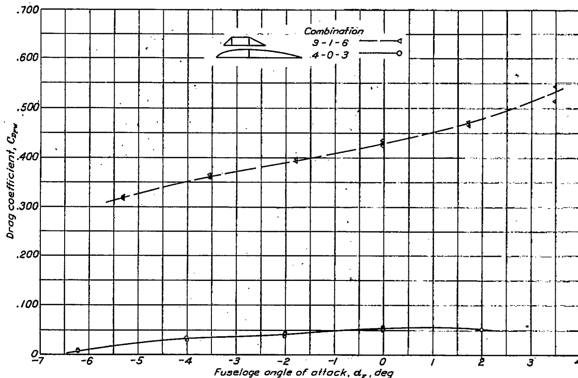
FIGURE 16.—Variation of drag with angle of attack. M , 0.18; V , 137 mph.
