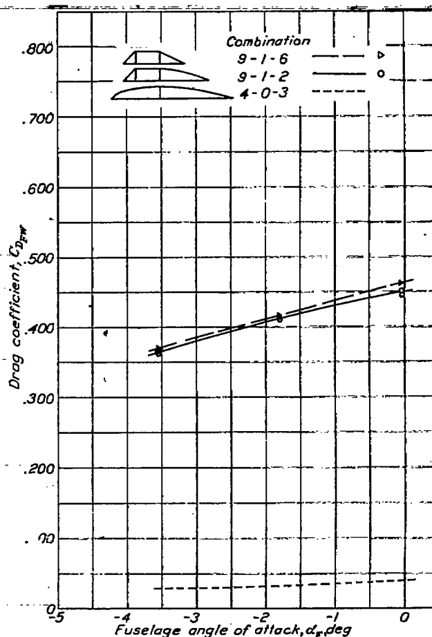
FIGURE 10.—Effect of tail length. M, 0.34 ; V, 200 mph.
