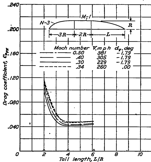
FIGURE 19.—Effect of tail length, streamline shape.
