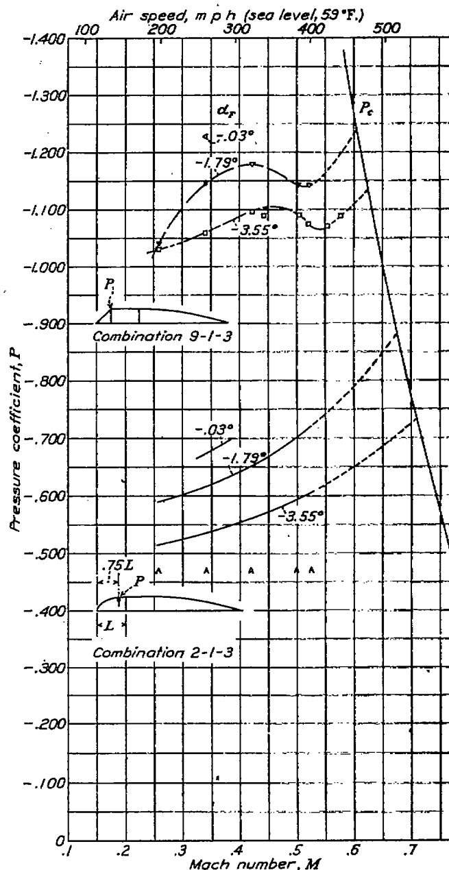
FIGURE 24.—Variation of peak negative pressure with speed for two windshields.
