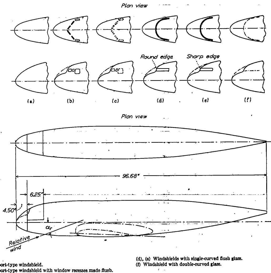
FIGURE 4.—Transport-type windshields.
