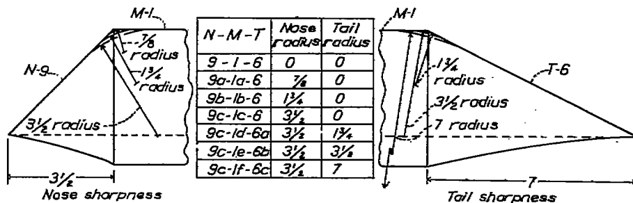
FIGURE 3.—Component parts of the closed-cockpit windshield combinations.
