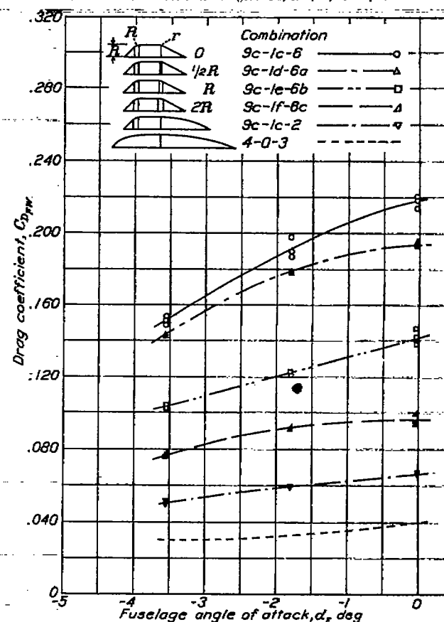
FIGURE 12.—Effect of radius at hood-tail juncture. M, 0.35 ; V, 205 mph.
