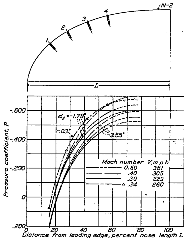
FIGURE 23.—Pressure distribution over streamline nose, medium length.
