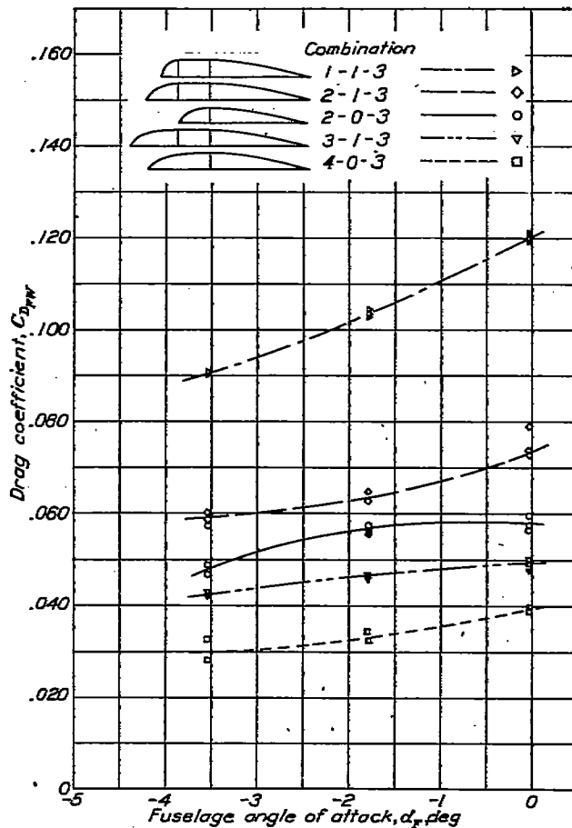
FIGURE 6.—Effect of nose length, streamline shape. M, 0.34 ; V, 260 mph.
