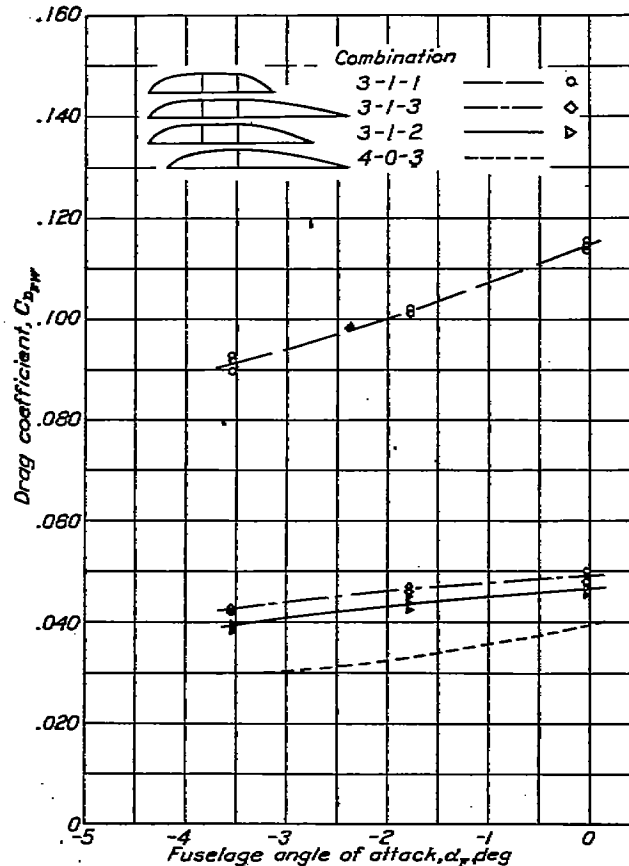
FIGURE 8.—Effect of tail length, streamline shape. M, 0.34 ; V, 260 mph.
