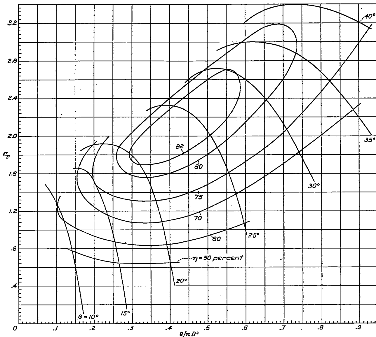
FIGURE 18.—Pressure coefficients showing lines of constant efficiency. \phi , 60°.
