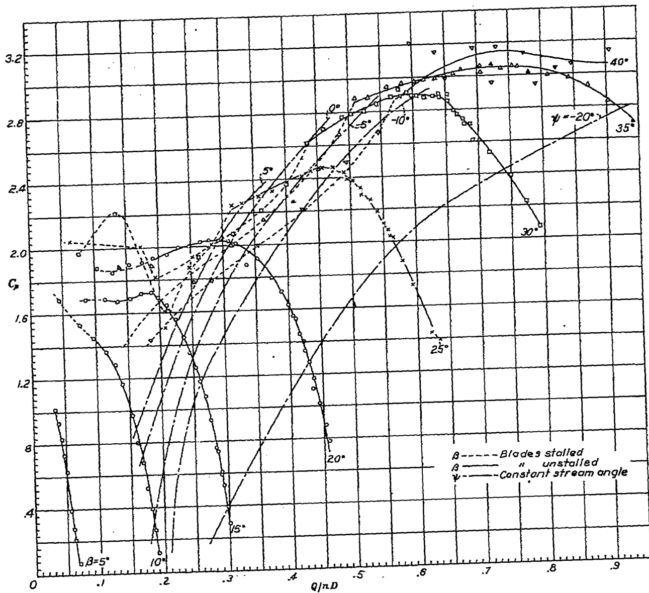
FIGURE 13.—Pressure coefficients. \phi, 50^\circ .
