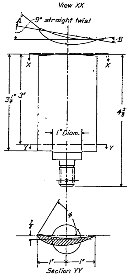
FIGURE 7.—Axial-fan contravane.
