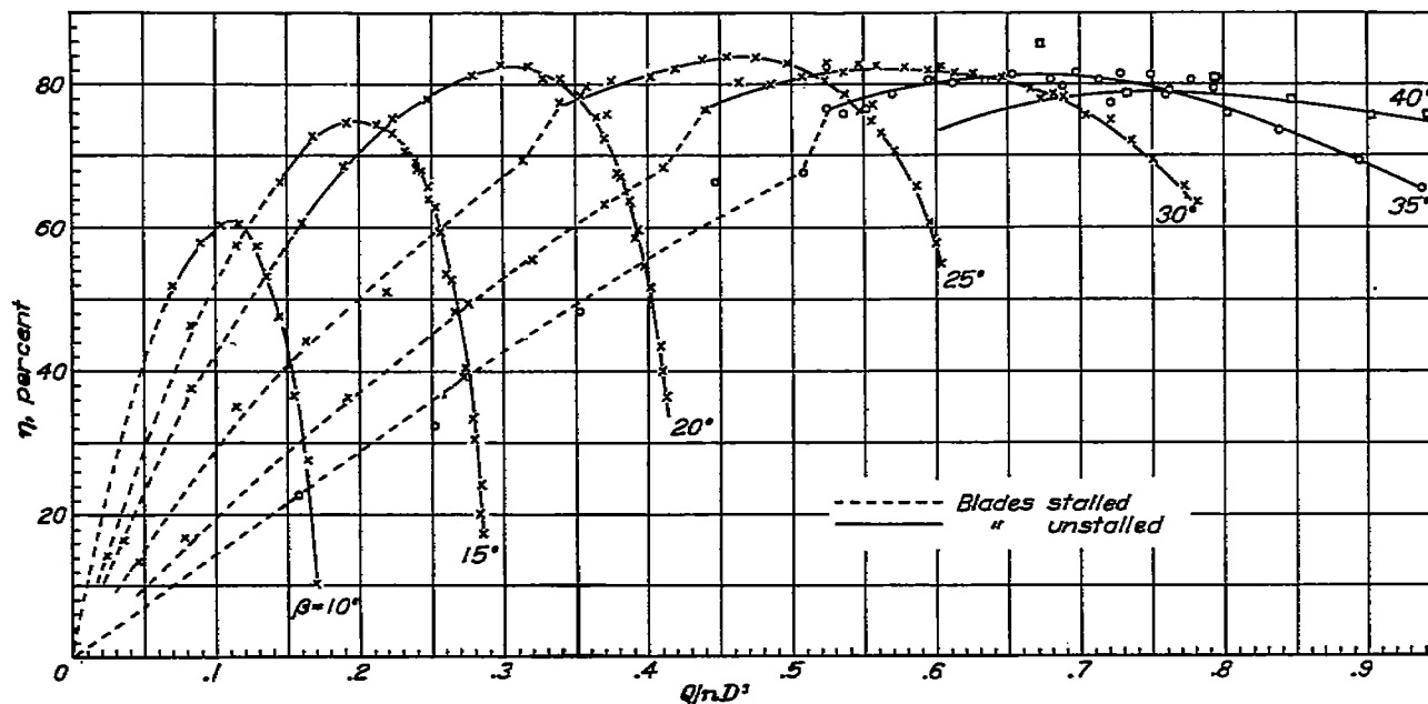
FIGURE 19.—Axial-fan efficiencies. \phi , 60°.
