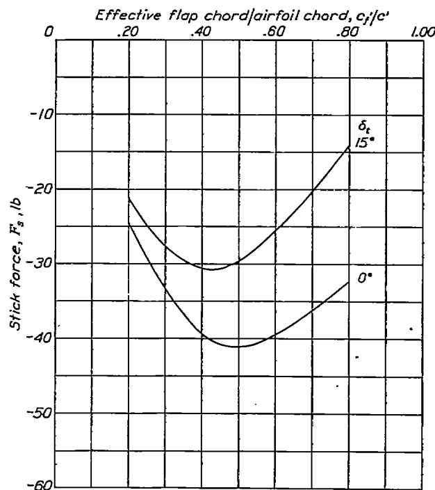
FIGURE 6.—Required stick force for tab neutral and deflected 15^\circ for landing with rectangular tails for various values of c_f'/c' . A_s', 4.5 ; \alpha_s', 14.0^\circ ; c_t'/c', 0.06 .
