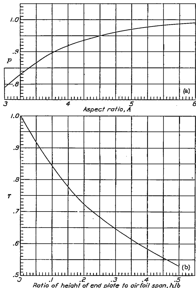
(a) Variation of parameter p with A for airfoils without end plates. (b) Variation of parameter r with h/b . For horizontal surfaces with end plates, p=1 . For horizontal surfaces with single vertical surfaces, r=1 . Values of r taken from reference 4.
