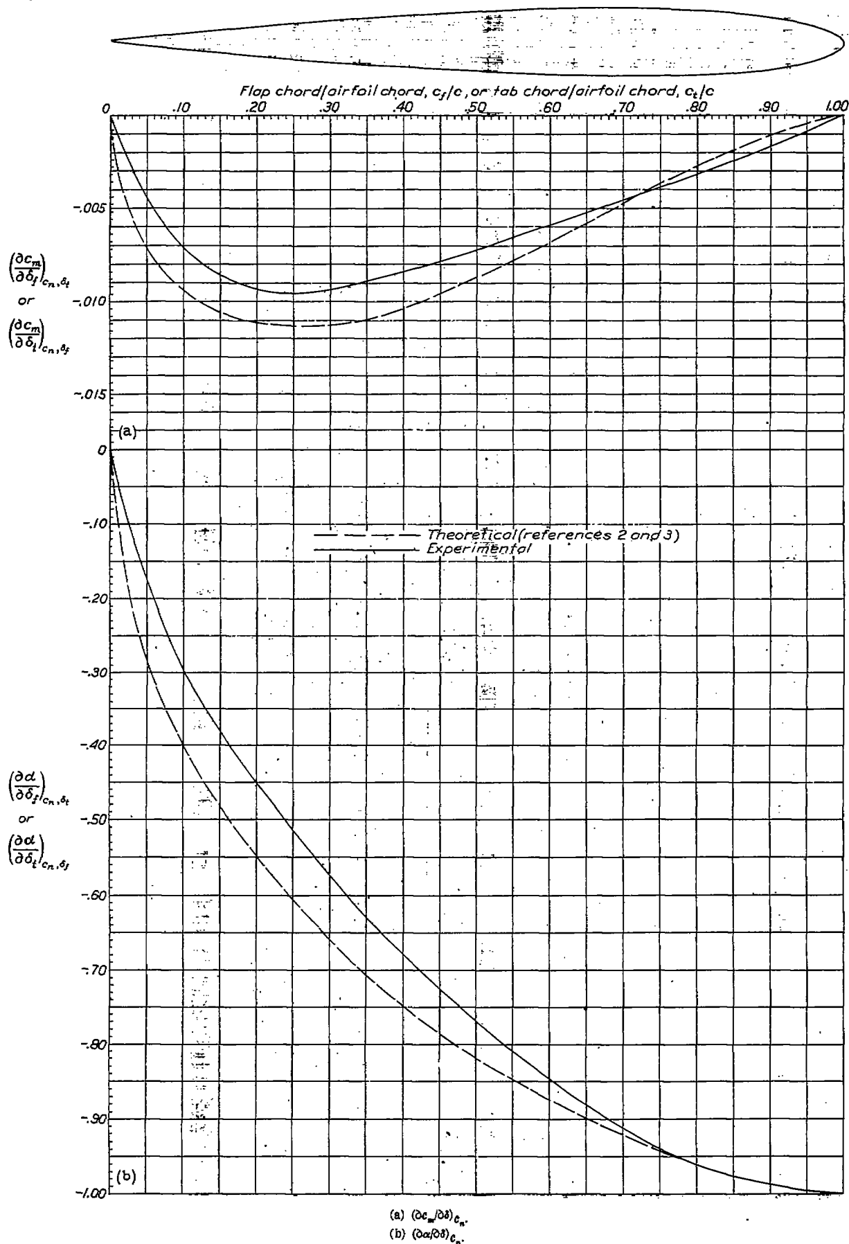
FIGURE 1.—Variation of (\partial c_m / \partial \delta) c_n and (\partial \alpha / \partial \delta) c_n with c_f/c or c_t/c for the NACA 0000 airfoil.
