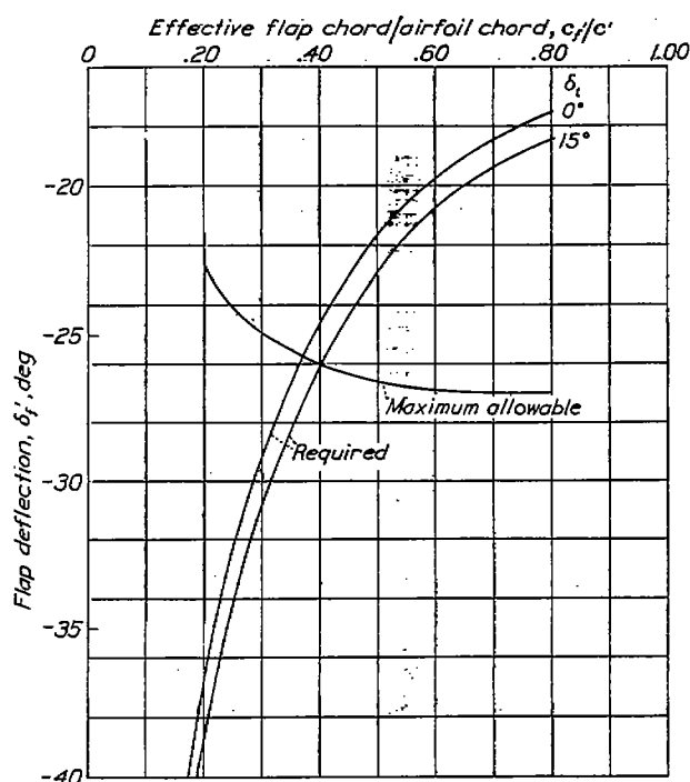
FIGURE 5.—Required flap deflections for tab neutral and deflected 15^\circ and maximum allowable flap deflections for various values of c_f'/c' . A_c, 4.5 ; \alpha_c, 14.0^\circ ; c_l'/c', 0.06 .
