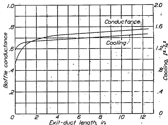
FIGURE 3.—Effect of exit-duct length on cooling and baffle conductance at 150° from front of cylinder at optimum exit-duct opening. Baffle exit opening, 1.50 inches; cylinder diameter, 4.66 inches; fin space, \frac{1}{16} inch; fin width, \frac{3}{16} inch. (Data from reference 8.)
