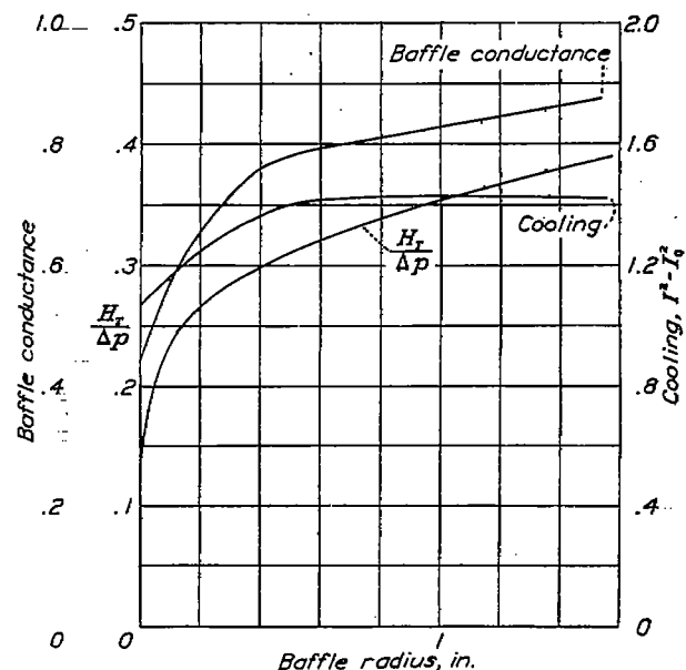
FIGURE 2.—Effect of baffle radius on H_r/\Delta p , baffle conductance, and cooling at 150° from front of cylinder at optimum exit-duct opening. Baffle exit opening, 1.0 inch; exit-duct length, 7.00 inches; cylinder diameter, 4.66 inches; fin space, \frac{1}{16} inch; fin width, \frac{3}{16} inch. (Reproduced from reference 8.)
