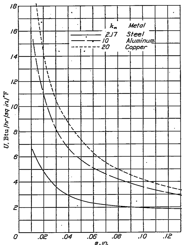
FIGURE 8.—Variation of over-all heat-transfer coefficient with spacing for three thermal conductivities, at 100 miles per hour and optimum fin thickness. u , 1 inch.
