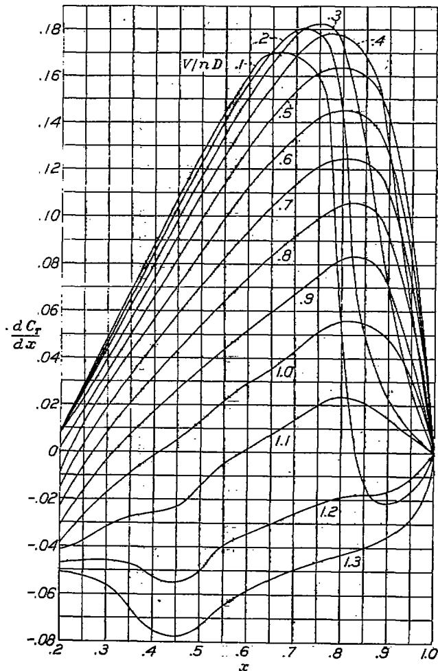
FIGURE 14.—Curves for dC_r/dx against x for propeller-hub body. \beta , 22^\circ .
