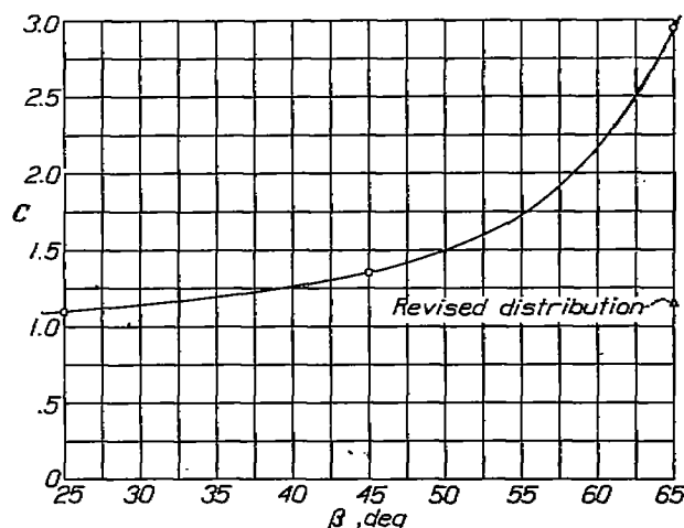
FIGURE 31.—Variation of \dot{C} with blade angle for propeller E.
