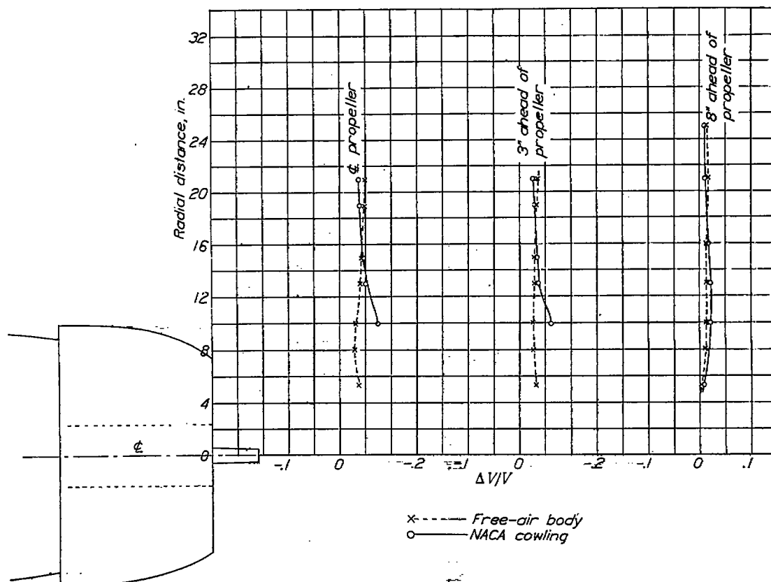
FIGURE 22.—Fractional increase in velocity due to propeller. \beta , 22°; V/nD , 0.895.
