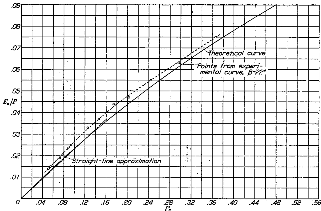
FIGURE 26.—Relationship between P_c and axial energy in the propeller wake.
