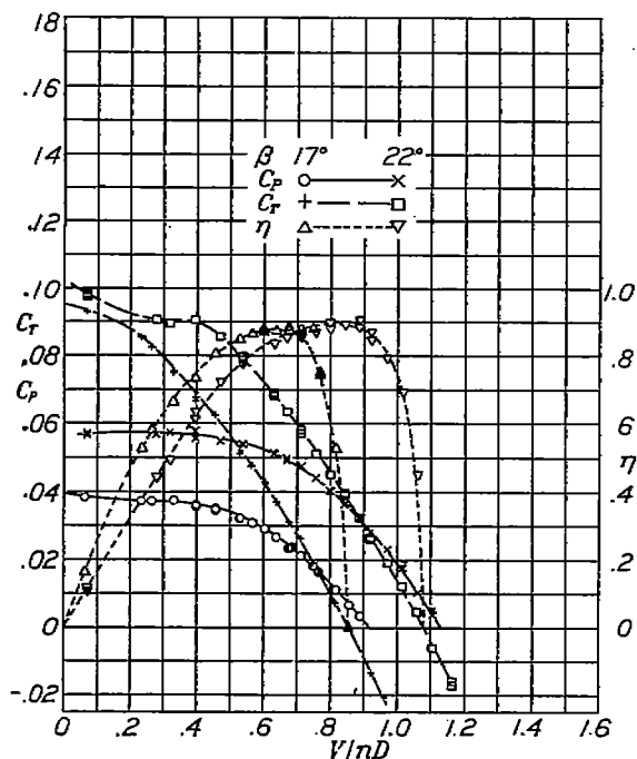
FIGURE 8.—Curves of C_T , C_P , and \eta against V/nD for propeller-hub body.
