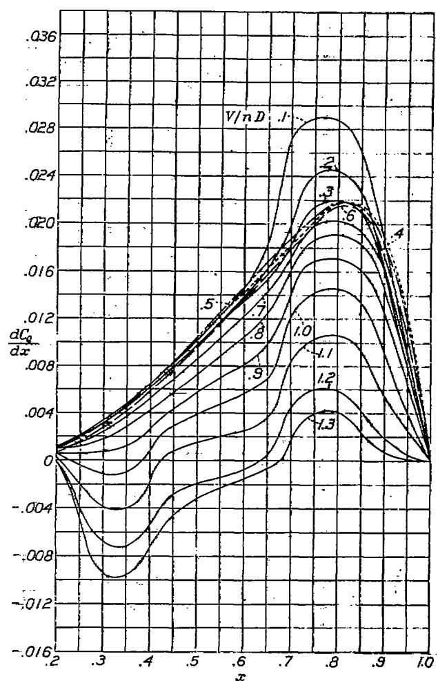
FIGURE 15.—Curves for dC_q/dx against x for propeller-hub body. \beta , 22^\circ .
