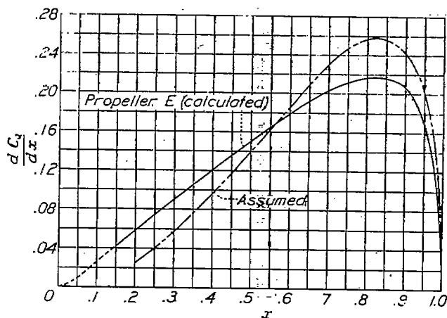
FIGURE 29.—Torque-gradient curves. \beta , 65°.
