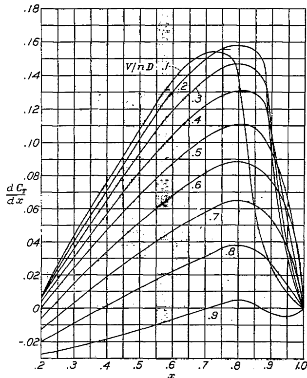
FIGURE 12.—Curves for dC_r/dx against x for propeller-hub body. \beta , 17^\circ .
