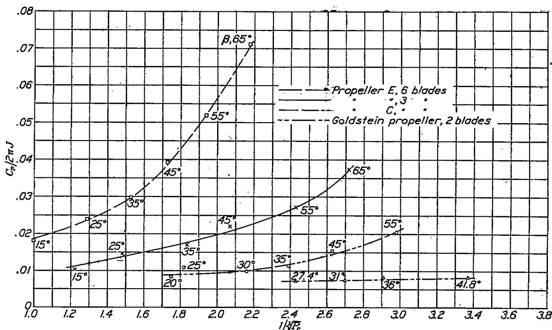
FIGURE 28.—Relationship between 1/\sqrt{P_r} and C_p/2\pi J at V/nD for peak efficiency
