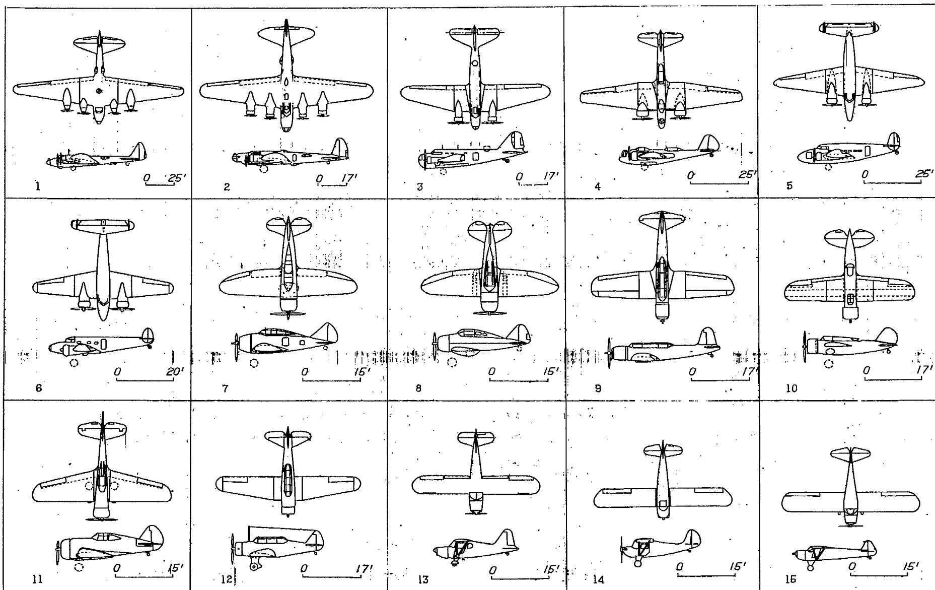
FIGURE 1.—Line drawings of airplanes tested in flight.
