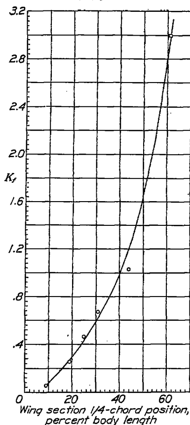
FIGURE 8.—Variation of fuselage and engine nacelle moment factor K_f with relative location of wing and body. Data taken from reference 3.
