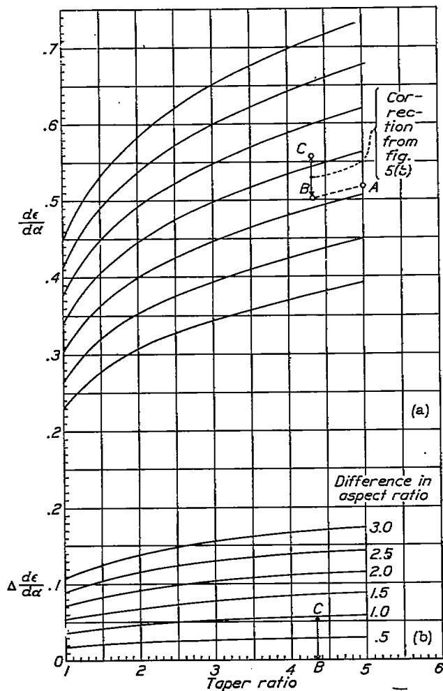
FIGURE 5.—Corrections to downwash for variations in wing aspect and taper ratios. Data taken from reference 2.
