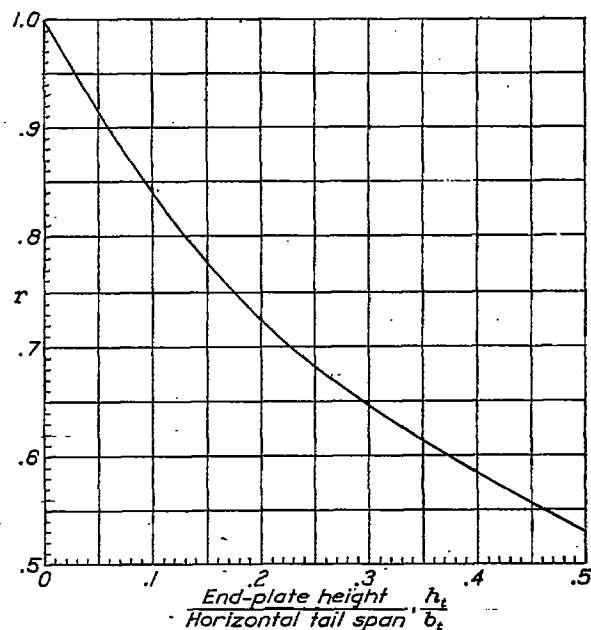
FIGURE 9.—Correction for dC_N/d\alpha_t of horizontal tail with end plates.
