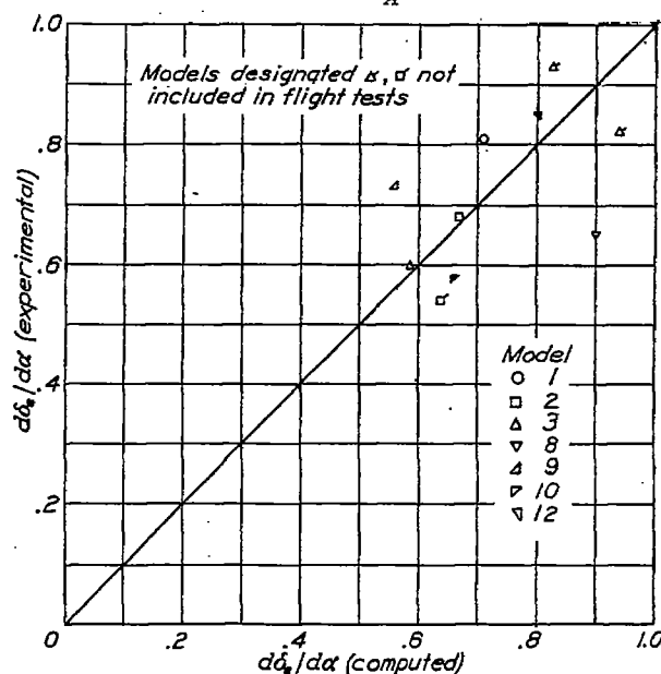
FIGURE 10.—Comparison of experimental and computed values of stability, propeller off.
