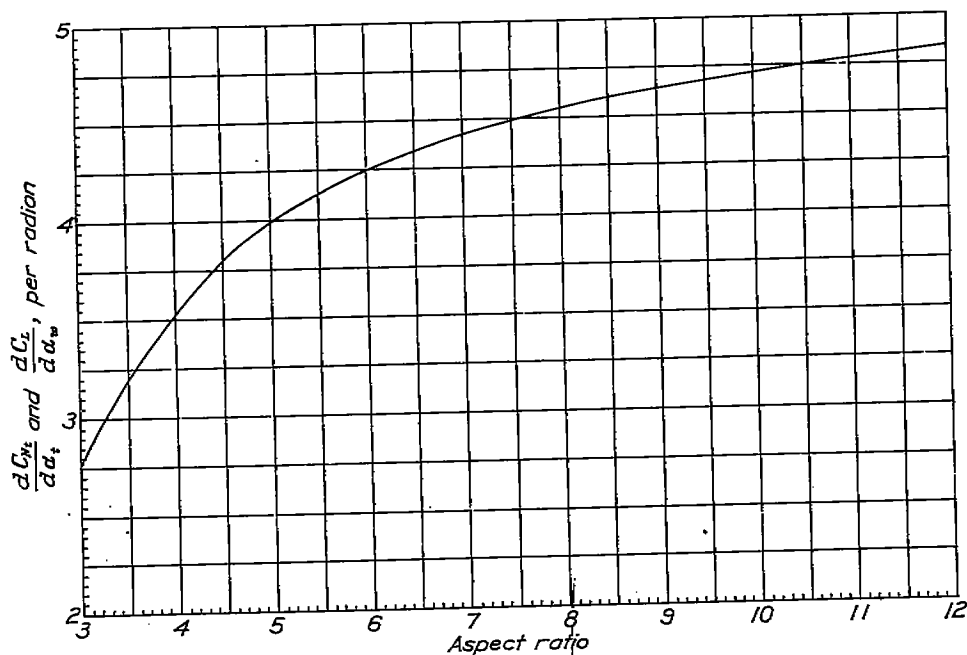
FIGURE 7.—Variation of \frac{dC_N}{d\alpha_z} and \frac{dC_L}{d\alpha_z} with aspect ratio for conventional sections. Data taken from reference 1.
