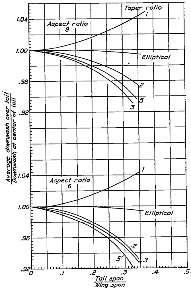
FIGURE 6.—Correction factor to convert downwash at center of horizontal tail to average downwash over tail. Data taken from reference 2.
