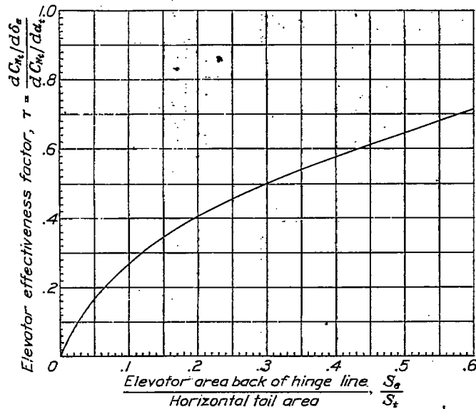
FIGURE 3.—Variation of elevator effectiveness factor \tau with ratio of elevator area back of hinge line to horizontal tail area. Data taken from reference 1.
