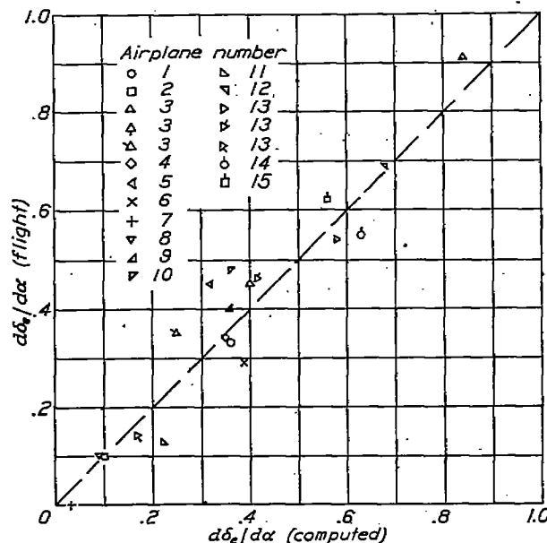
FIGURE 12.—Comparison of computed stability with flight stability as determined with idling propellers.
