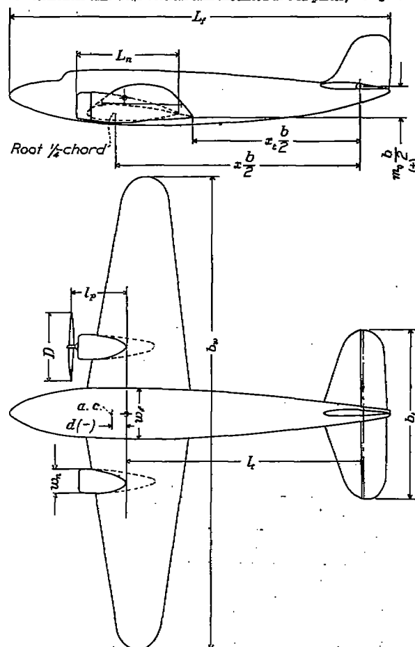
FIGURE 2.—Dimensions used in stability calculations. Distances measured at angle of zero lift.
