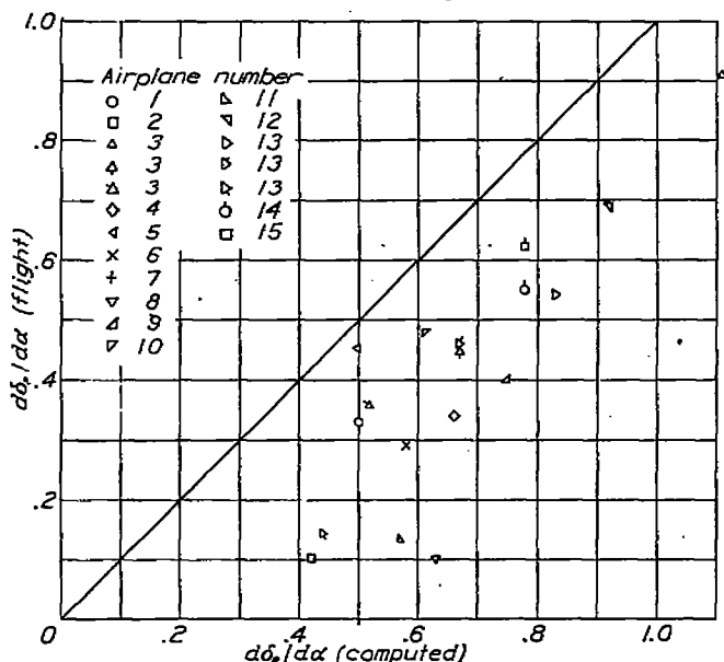
FIGURE 11.—Comparison of flight stability as determined with idling propellers with computed stability, propeller off.
