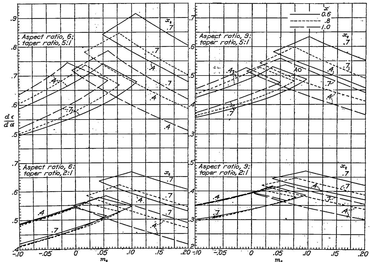
FIGURE 4.—Variation of rate of change of downwash over horizontal tail with angle of attack d\epsilon/d\alpha with location of horizontal tail m_\alpha for various wing aspect and taper ratios. Data taken from reference 2.
