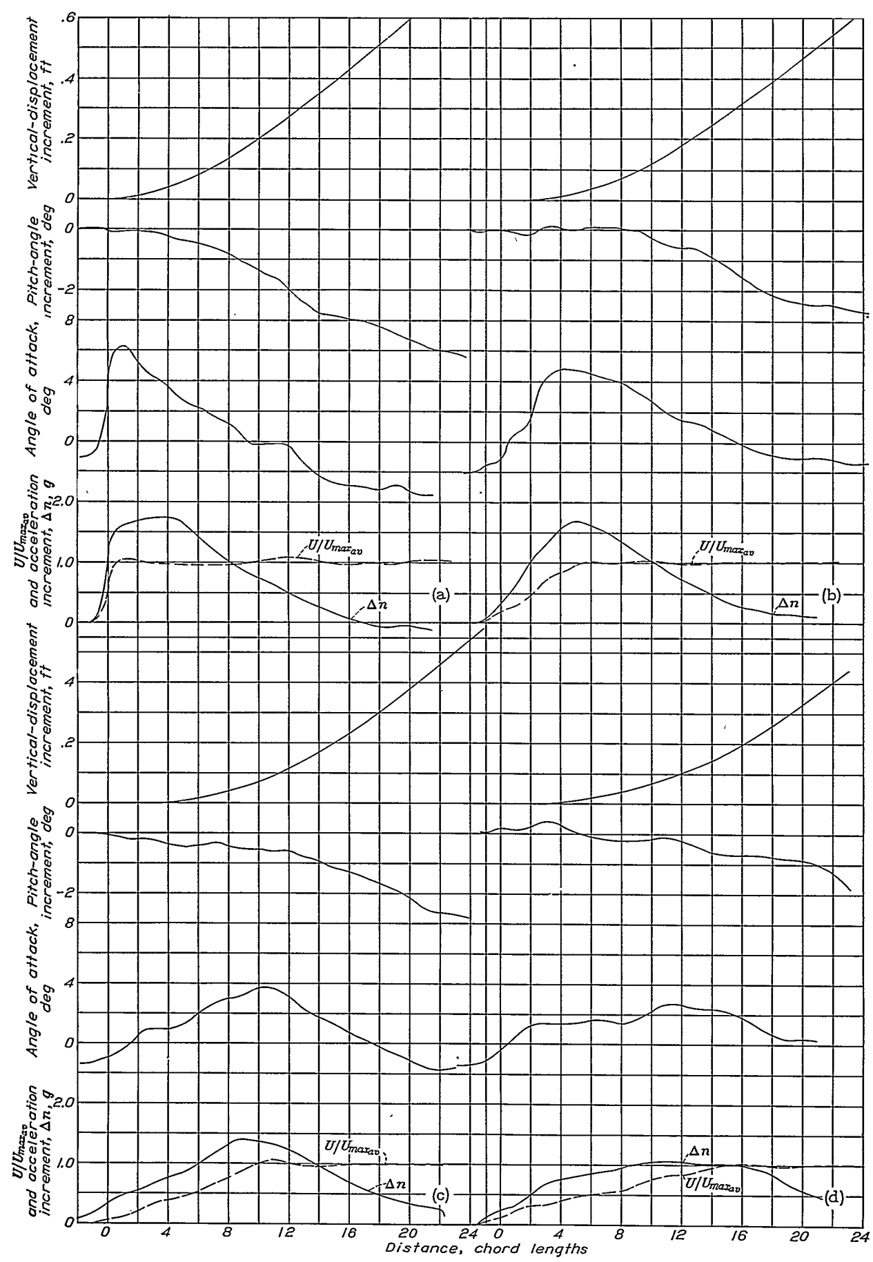
(a) Gradient distance, H , 0 feet (sharp-edge gust). (b) Gradient distance, H , 24 feet (full-scale). (c) Gradient distance, H , 51 feet (full-scale). (d) Gradient distance, H , 66 feet (full-scale).
