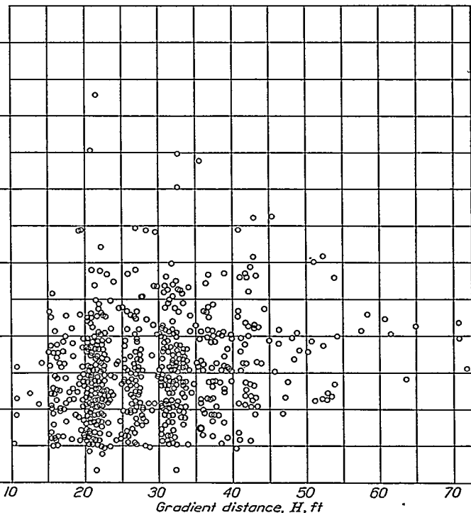
FIGURE 6.—Gust velocity U as a function of the gust-gradient distance H for regular flights.
