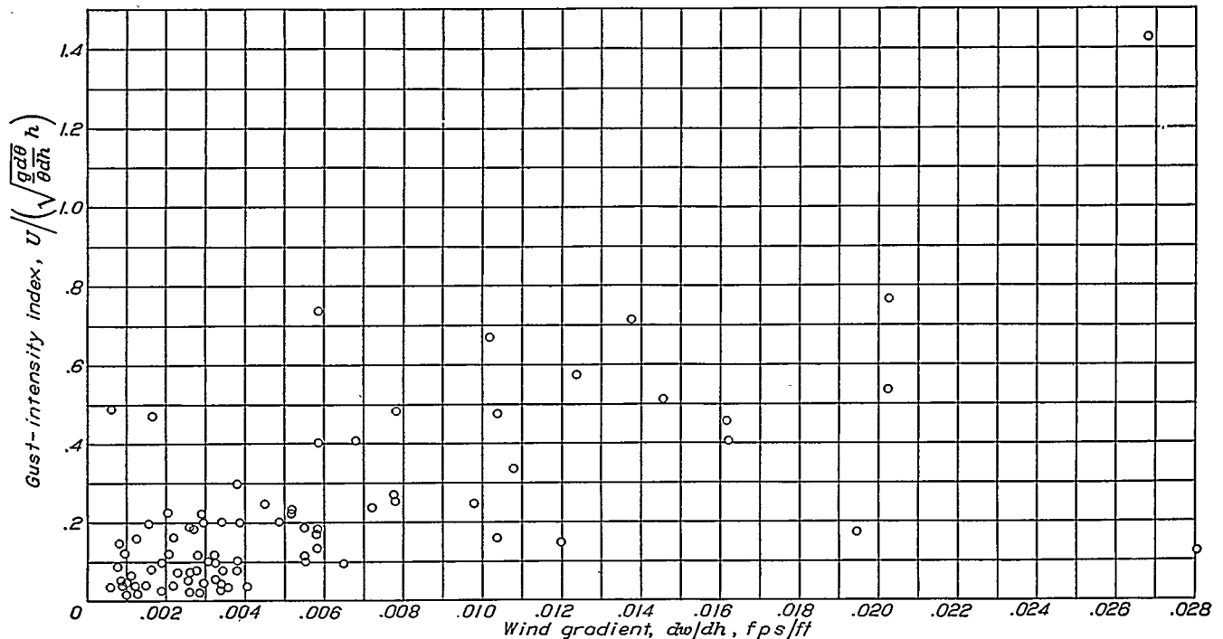
FIGURE 8.—Relation between gust-intensity index and wind gradient.
