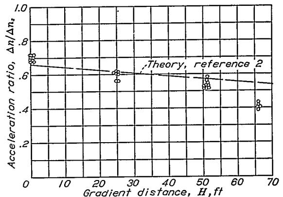
FIGURE 4.—Variation of acceleration ratio with gradient distance.
