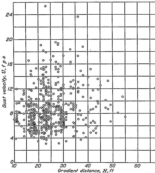
FIGURE 5.—Gust velocity U as a function of the gust-gradient distance H for preliminary flights.
