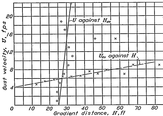
FIGURE 7.—Correlation of gust velocity and gradient distance.
