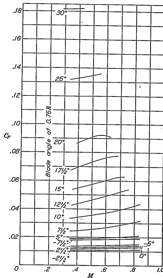
FIGURE 12.—Variation of static-power coefficient with tip-speed ratio and blade angle. Propeller 5868-R6, 3 blades.
