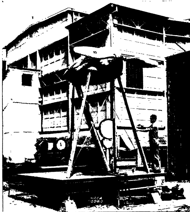
FIGURE 1.—Propeller 37-3647 mounted on test rig.
