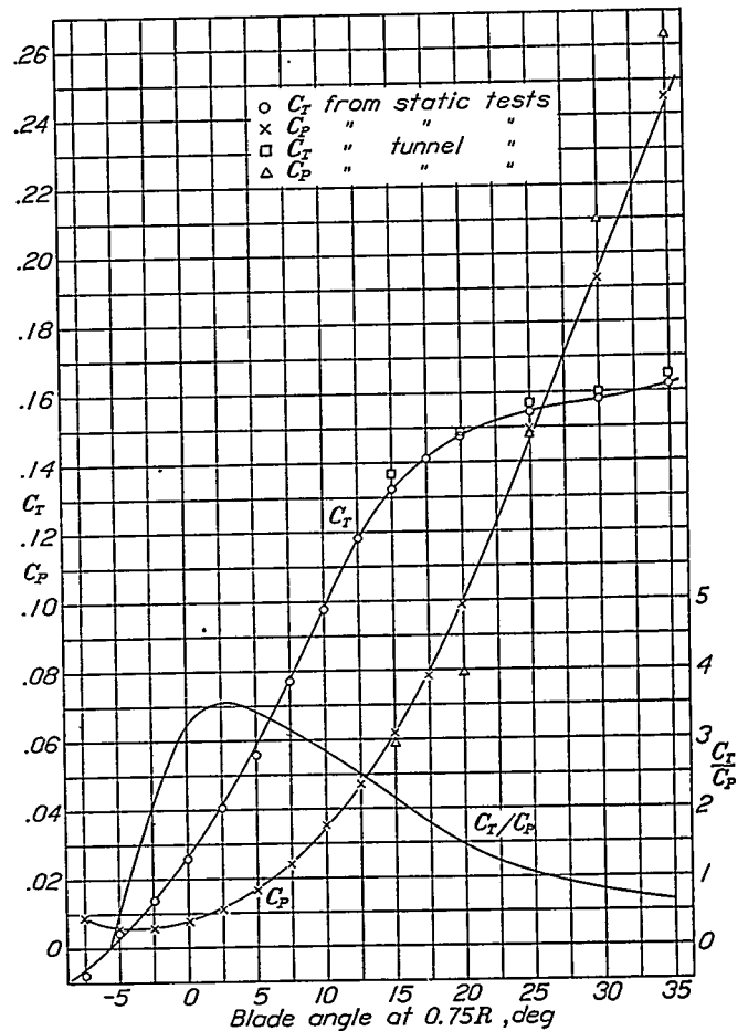
FIGURE 21.—Characteristics of 3-blade propeller 5868-9 at zero V/nD . M , 0.5.
