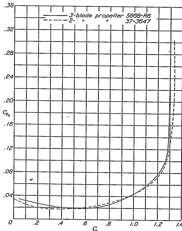
FIGURE 35.—Comparison of polars obtained from static tests of 2- and 3-blade propellers having the same solidity. M , 0.5.
