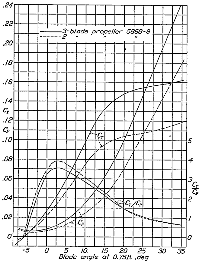
FIGURE 26.—Comparison of static aerodynamic characteristics of 2-blade and 3-blade propellers. M , 0.5.
