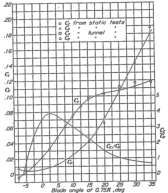
FIGURE 20.—Characteristics of 2-blade propeller 5868-9 at zero V/nD . M , 0.5.
