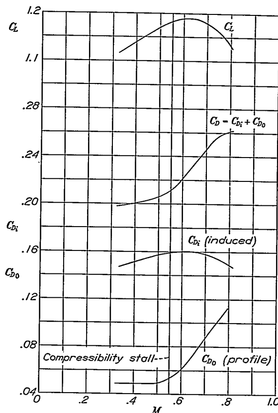
FIGURE 17.—Effect of compressibility on airfoil coefficients obtained from the static-test propeller coefficients for 2-blade propeller 5868-R6 set 15^\circ at 0.75R .
