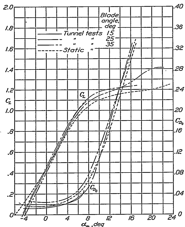
FIGURE 32.—Comparison of lift and drag coefficients obtained from wind-tunnel and static tests for 2-blade propeller 5868-9.
