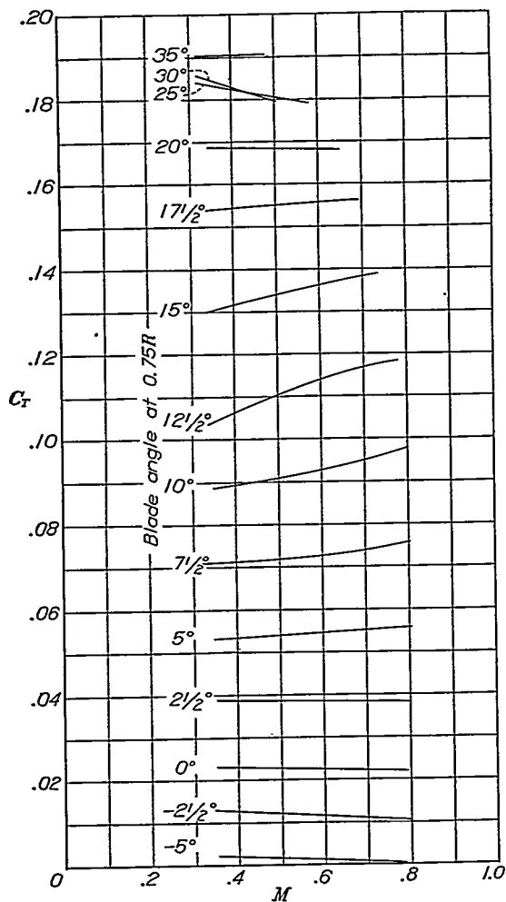
FIGURE 15.—Variation of static-thrust coefficient with tip-speed ratio and blade angle. Propeller 37-3647, 2 blades.
