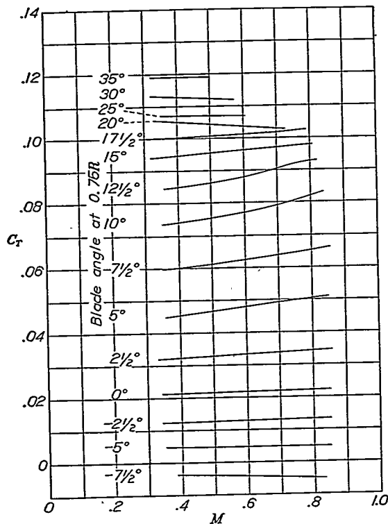
FIGURE 5.—Variation of static-thrust coefficient with tip-speed ratio and blade angle. Propeller 5868-9, 2 blades.
