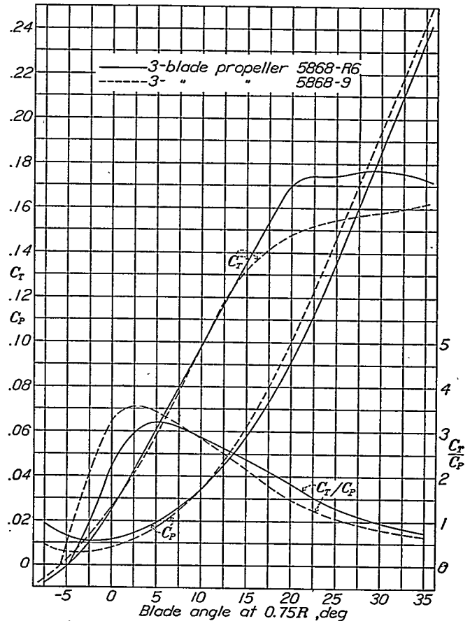
FIGURE 27.—Comparison of static aerodynamic characteristics of 3-blade propellers having Clark Y (5868-9) and R. A. F. 6 (5868-R6) airfoil sections. M , 0.5.
