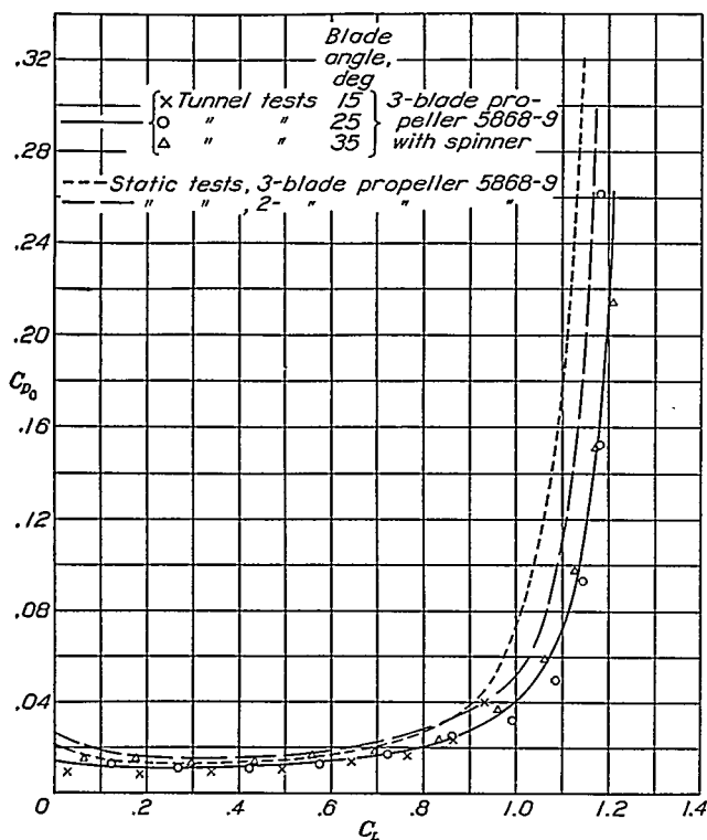
FIGURE 33.—Comparison of polars obtained from wind-tunnel and static tests of propeller 5868-9.
