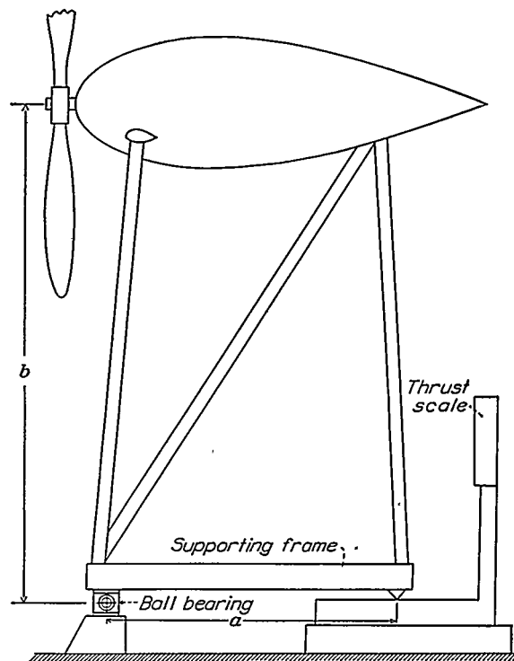
FIGURE 2.—Diagrammatic sketch showing method of measuring static thrust.
