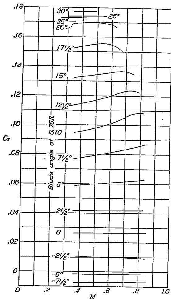
FIGURE 11.—Variation of static-thrust coefficient with tip-speed ratio and blade angle. Propeller 5868-R6, 3 blades.
