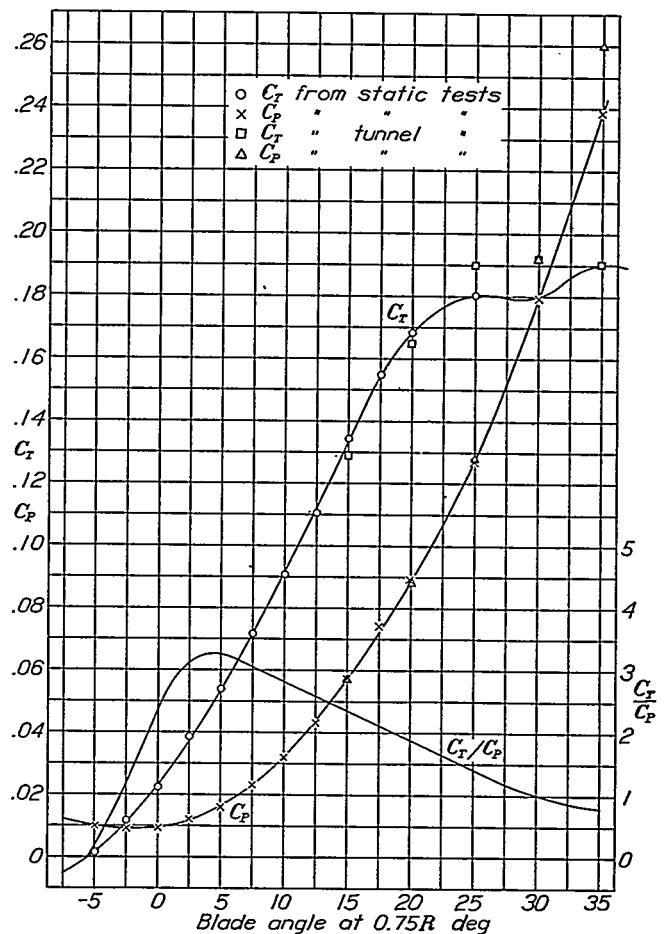
FIGURE 25.—Characteristics of 2-blade propeller 37-3647 at zero V/nD . M , 0.5.
