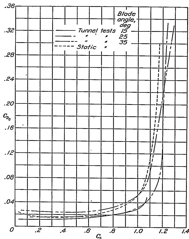
FIGURE 30.—Comparison of polars obtained from wind-tunnel tests and from static tests of 2-blade propeller 5868-9.
