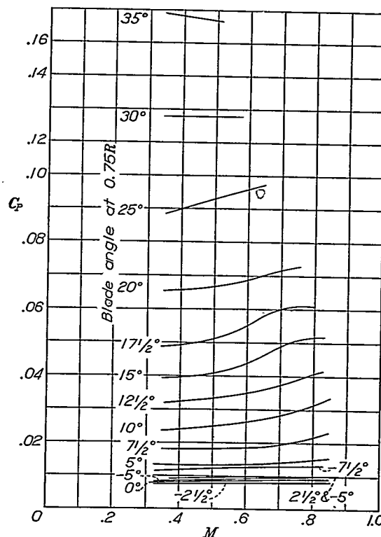
FIGURE 10.—Variation of static-power coefficient with tip-speed ratio and blade angle. Propeller 5868-R6, 2 blades.
