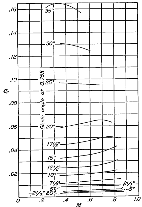
FIGURE 14.—Variation of static-power coefficient with tip-speed ratio and blade angle. Propeller 6623-B, 2 blades.
