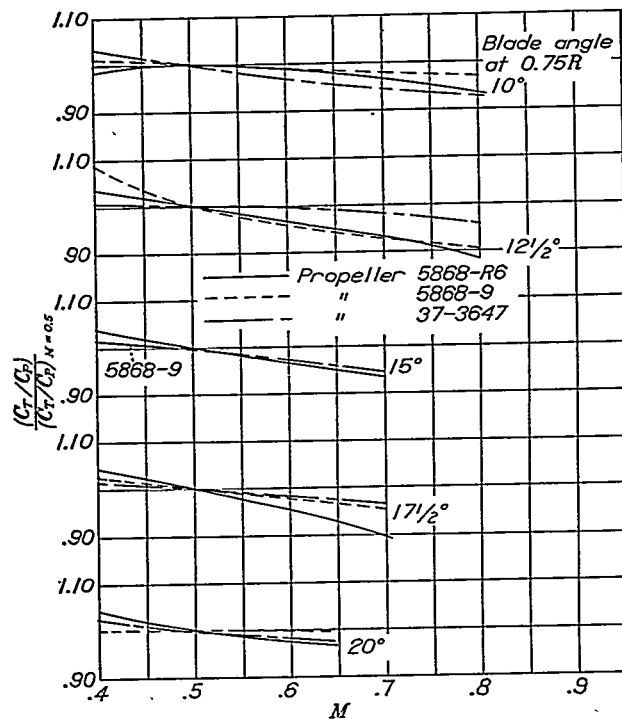
FIGURE 19.—Variation of propeller coefficients with tip-speed ratio for the 3-blade propellers and the 2-blade propeller 37-3647 having the same solidity.
