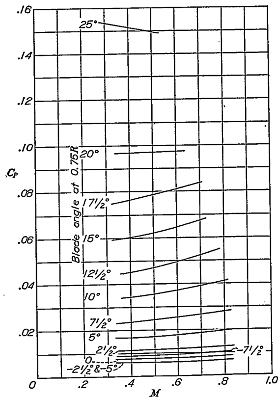
FIGURE 8.—Variation of static-power coefficient with tip-speed ratio and blade angle. Propeller 5868-9, 3 blades.
