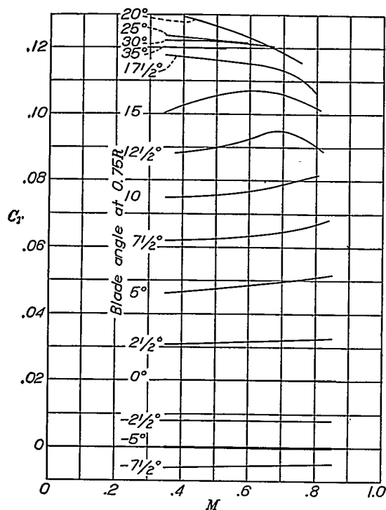
FIGURE 9.—Variation of static-thrust coefficient with tip-speed ratio and blade angle. Propeller 5868-R6, 2 blades.
