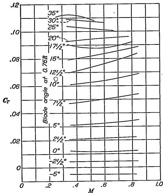
FIGURE 13.—Variation of static-thrust coefficient with tip-speed ratio and blade angle. Propeller 6623-B, 2 blades.
