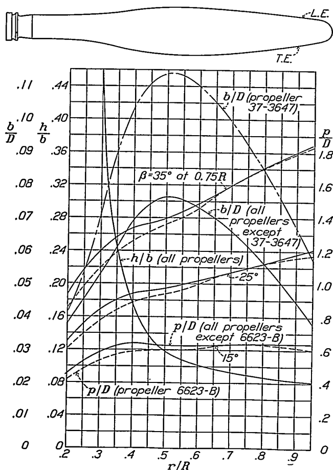
FIGURE 3.—Blade-form curves for propellers 5868-9, 5868-R6, 6623-B, and 37-3647. D , diameter; R , radius to the tip; r , station radius; b , section chord; h , section thickness; p , geometric pitch; \beta , blade angle.
