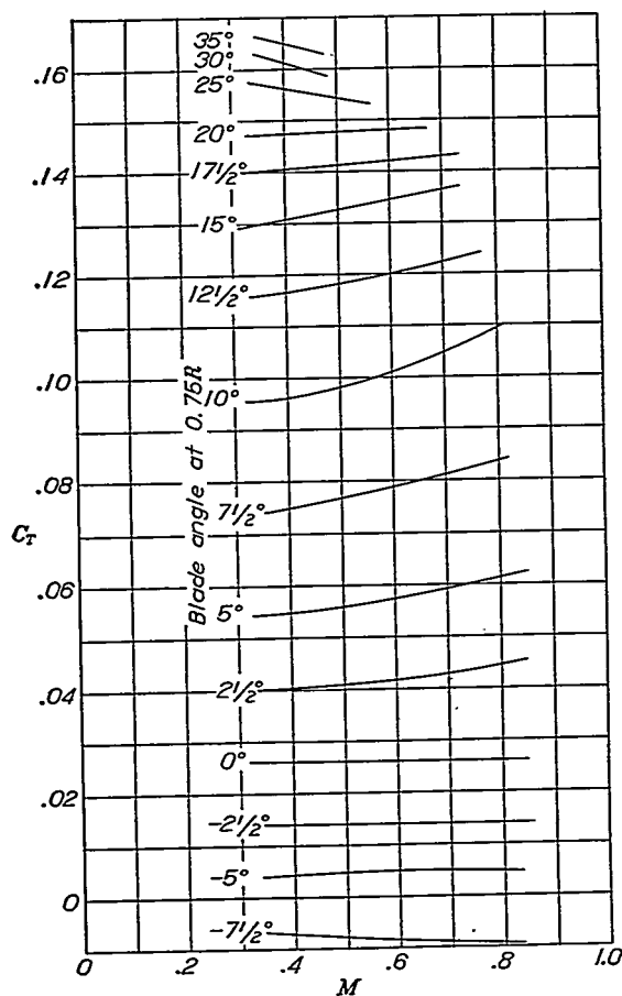
FIGURE 7.—Variation of static-thrust coefficient with tip-speed ratio and blade angle. Propeller 5868-9, 3 blades.
