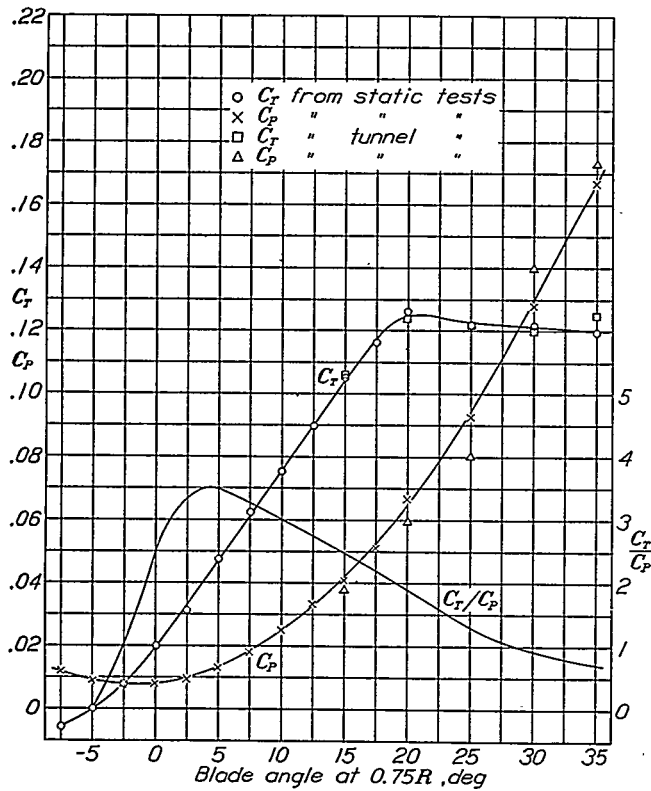
FIGURE 22.—Characteristics of 2-blade propeller 5868-R6 at zero V/nD . M , 0.5.
