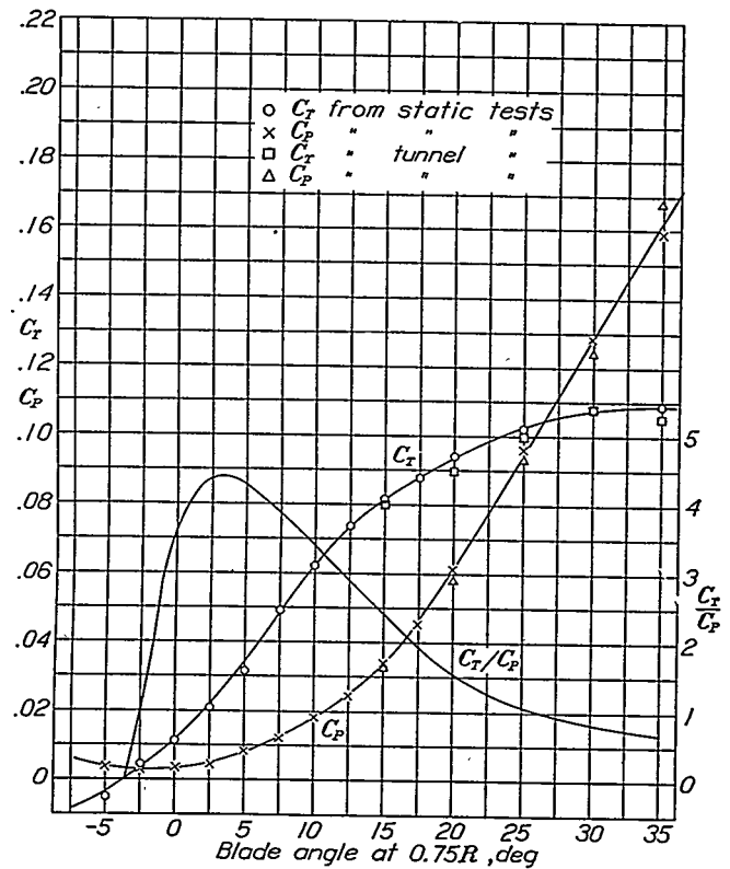
FIGURE 24.—Characteristics of 2-blade propeller 6623-B at zero V/nD . M , 0.5.
