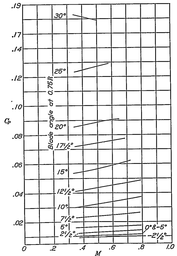
FIGURE 16.—Variation of static-power coefficient with tip-speed ratio and blade angle. Propeller 37-3647, 2 blades.
