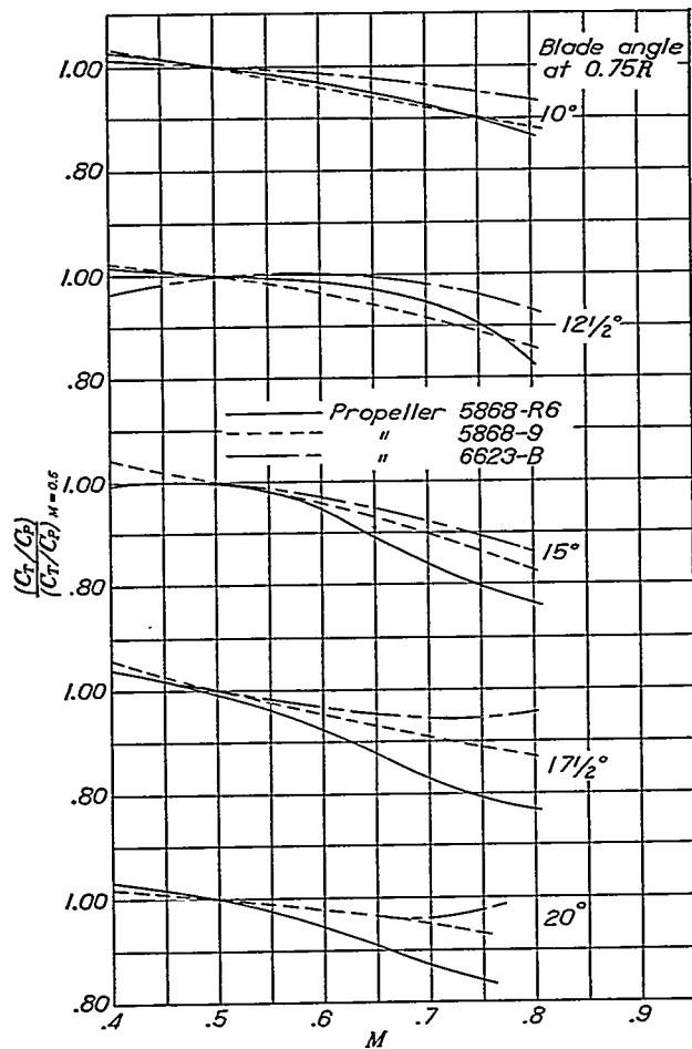
FIGURE 18.—Variation of propeller coefficients with tip-speed ratio for the 2-blade propellers.
