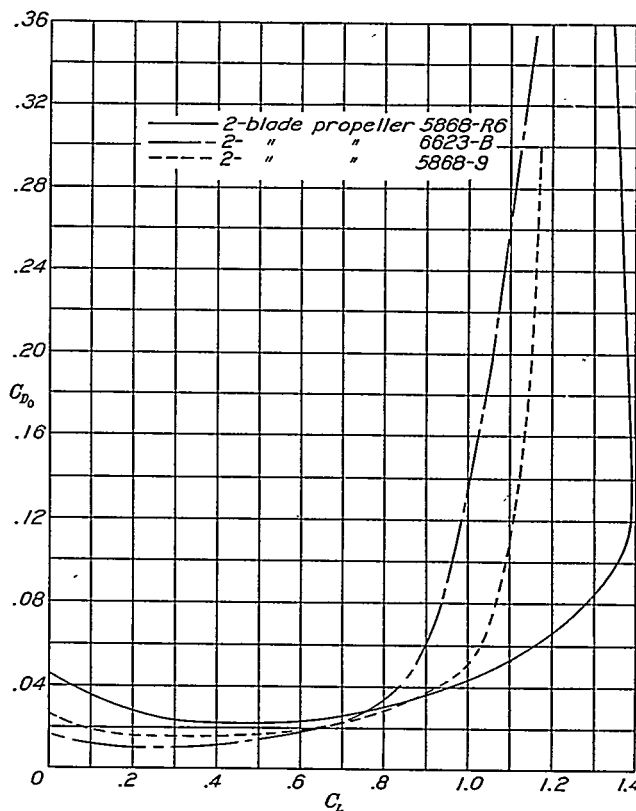
FIGURE 34.—Comparison of polars obtained from static tests of three 2-blade propellers having different airfoil sections. M , 0.5.
