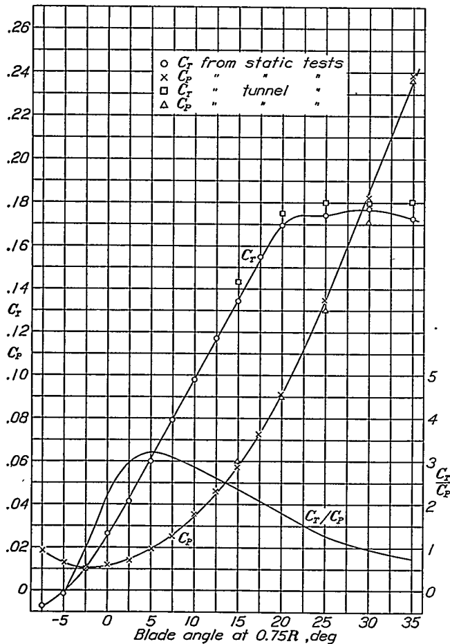
FIGURE 23.—Characteristics of 3-blade propeller 5868-R6 at zero V/nD . M , 0.5.
