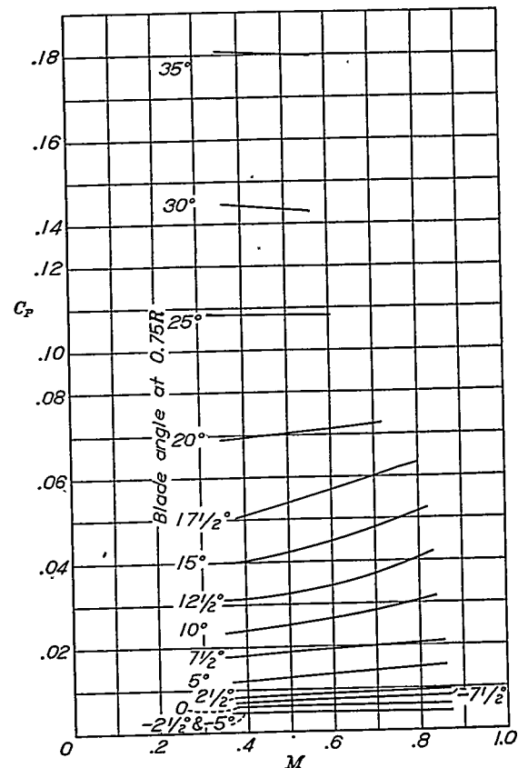
FIGURE 6.—Variation of static-power coefficient with tip-speed ratio and blade angle. Propeller 5868-9, 2 blades.
