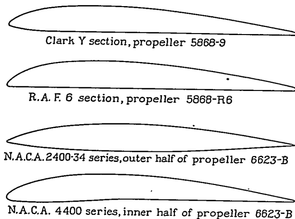
FIGURE 4.—Propeller blade sections; representative of the 0.70R station.
