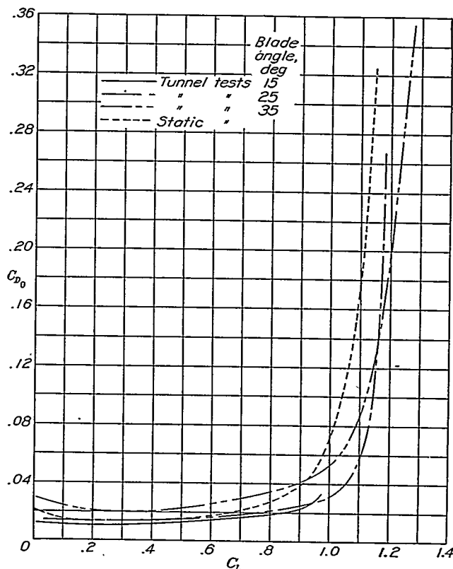
FIGURE 31.—Comparison of polars obtained from wind-tunnel tests and from static tests of 3-blade propeller 5868-9.
