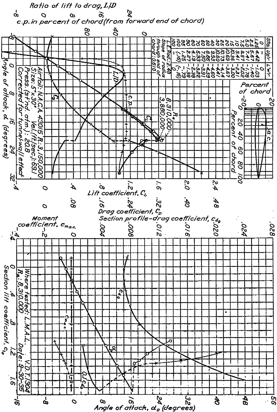
FIGURE 56.—N. A. C. A. 43015 AIRFOIL.
