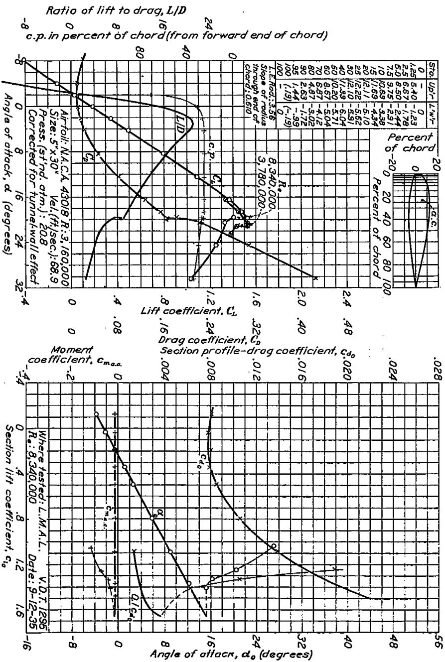
FIGURE 57.—N. A. C. A. 43018 AIRFOIL.
