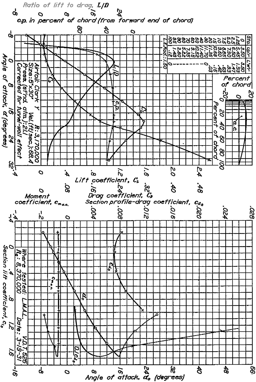
FIGURE 18.—Clark Y airfoil.
