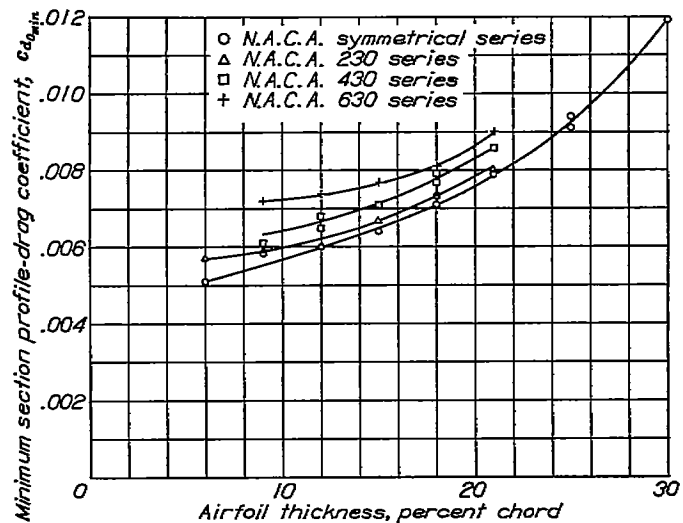
FIGURE 2.—Variation of minimum profile-drag coefficient with airfoil thickness. Effective Reynolds Number, 8,200,000.
