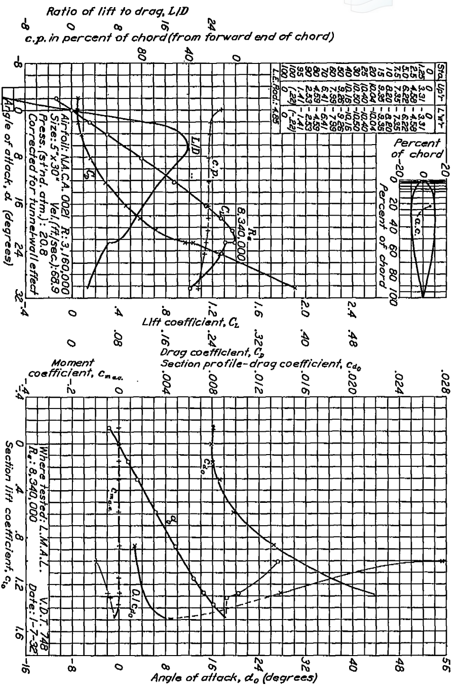
FIGURE 35.—N. A. C. A. 0021 airfoil.
