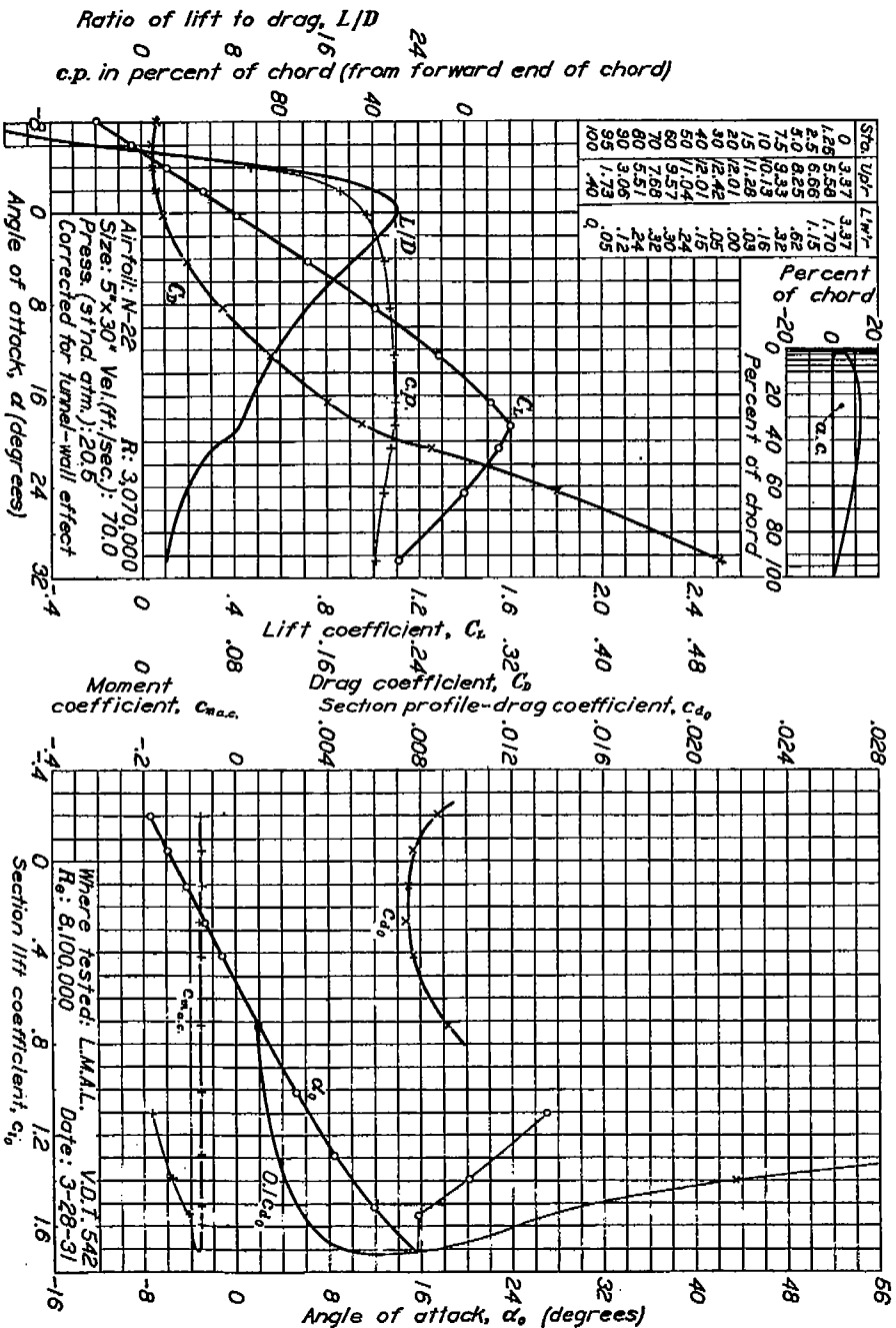
Figure 24.—N-22 airfoil.
