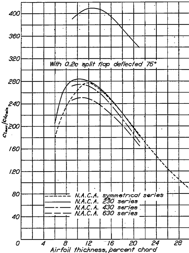
FIGURE 3.—Variation of c_{l_{max}}/c_{d_{min}} with airfoil thickness.
