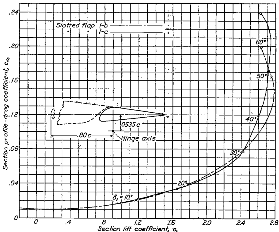
FIGURE 14.—Comparison of slotted flaps 1-b and 1-c.
