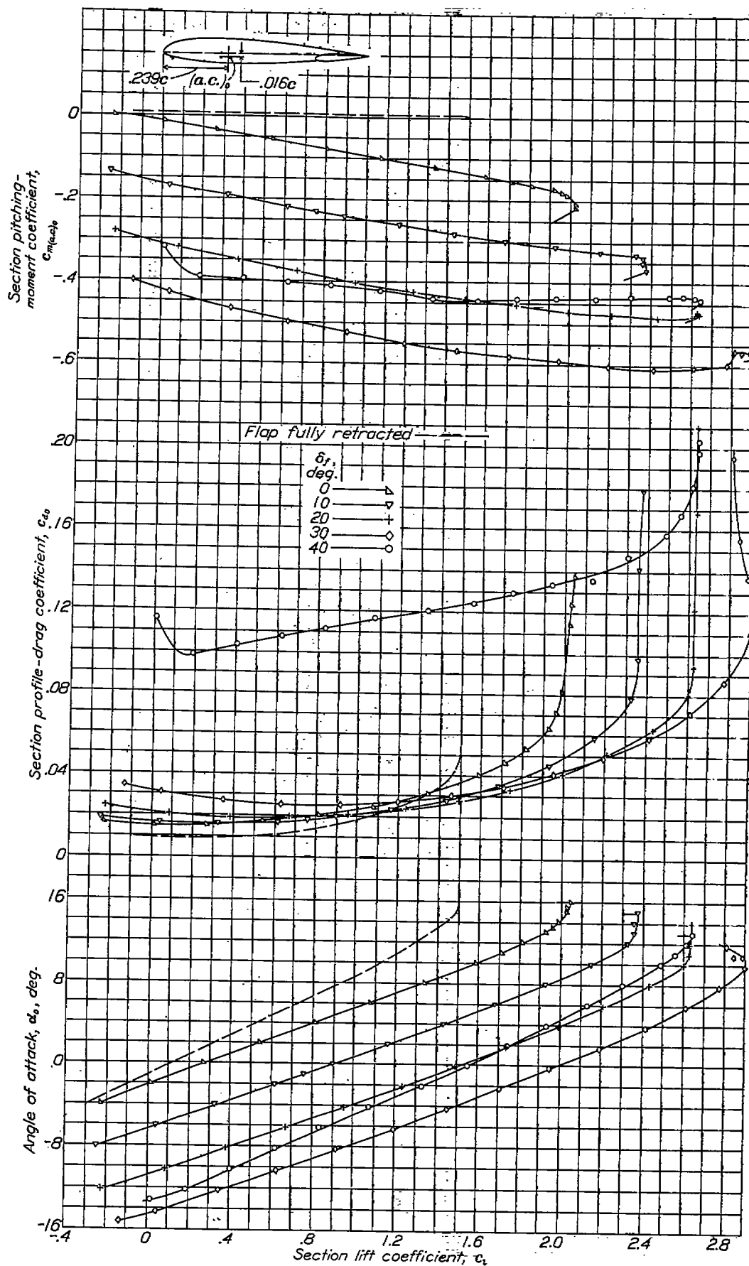
FIGURE 11.—Section aerodynamic characteristics of N. A. C. A. 23012 airfoil with a 0.2667 c_u N. A. C. A. 23012 Fowler flap.
