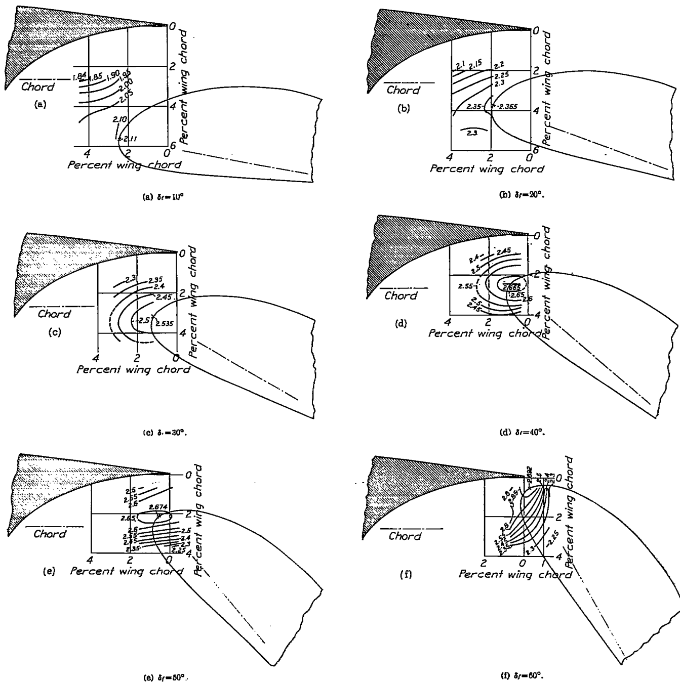
FIGURE 19.—Contours of flap location for c_{l_{max}} . Slotted flap 2-1.
