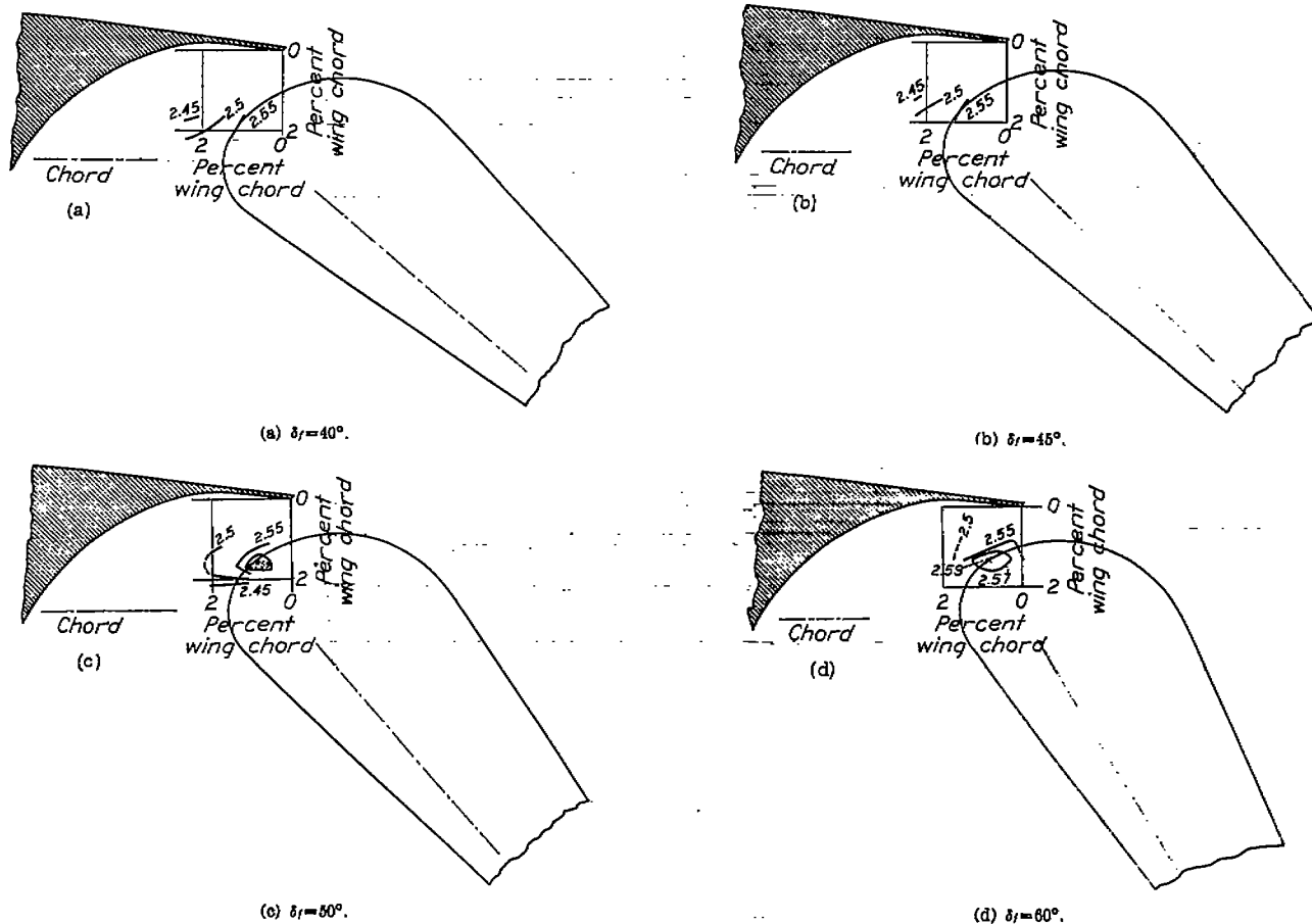
FIGURE 20.—Contours of flap location for c_{l_{max}} . Slotted flap 3-l.
