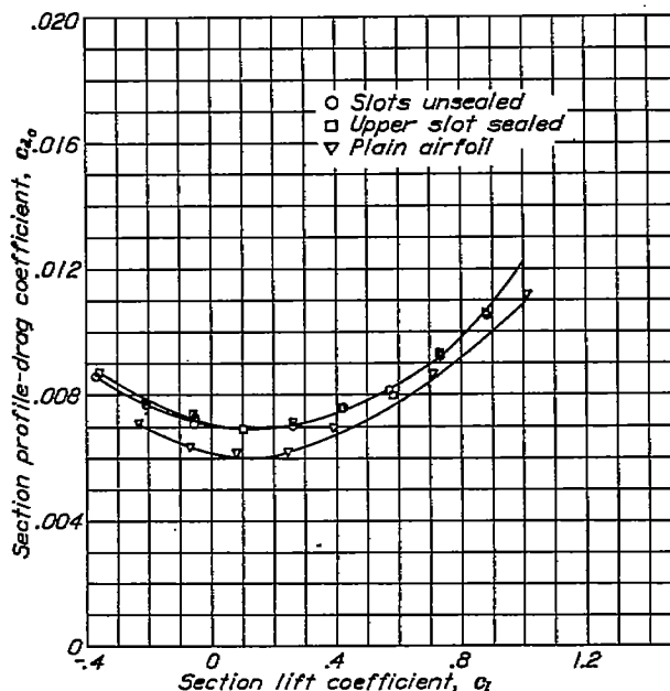
FIGURE 38.—Effect of slot opening on profile drag of N. A. C. A. 23012 airfoil with slotted flap 2-h neutral. Effective Reynolds Number, approximately 8,200,000.
