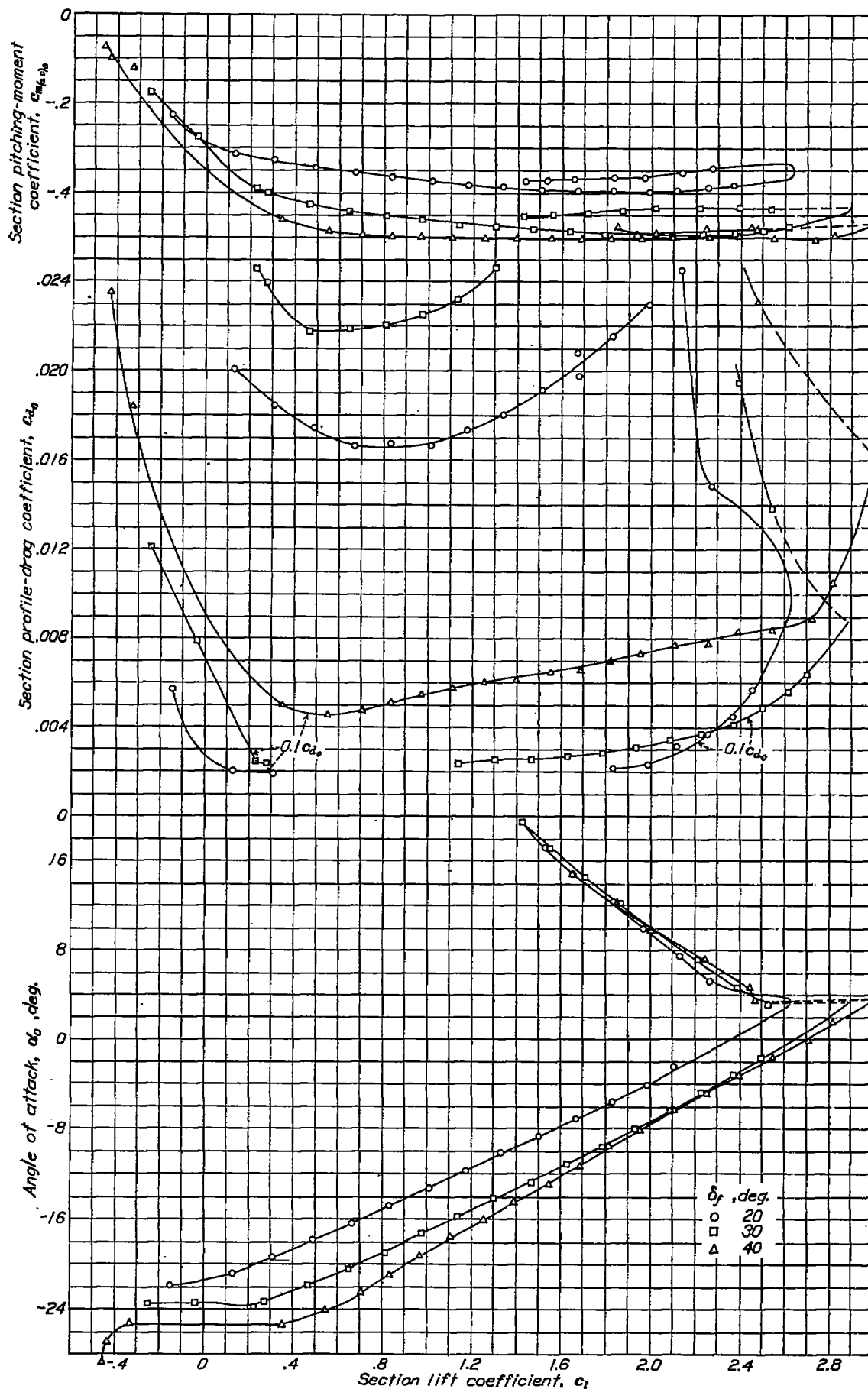
FIGURE 36.—Section aerodynamic characteristics of N. A. C. A. 23012 airfoil with 0.2586c slotted flap 2-h and the 0.60c plain flap deflected 12°. Effective Reynolds Number approximately 8,200,000.
