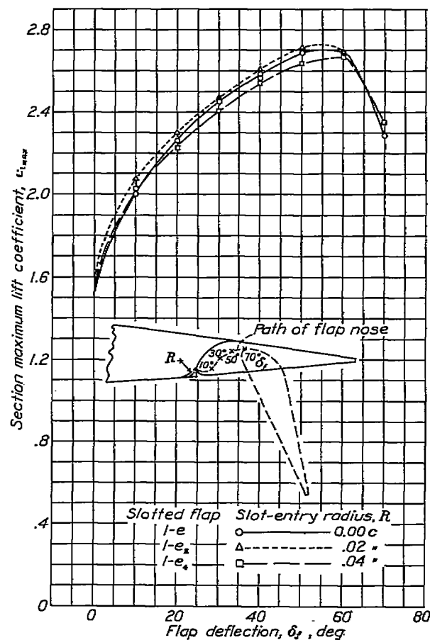
FIGURE 17.—Effect of slot-entry radius on c_{l_{max}} .
