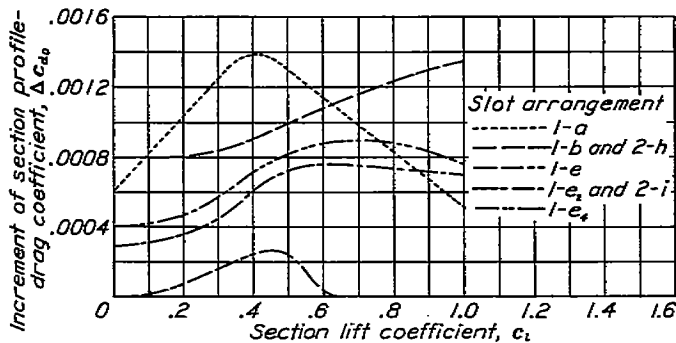
FIGURE 22.—Effect of slot openings in surface of airfoil on increments of profile drag \delta , 0°; effective Reynolds Number, 3,500,000.
