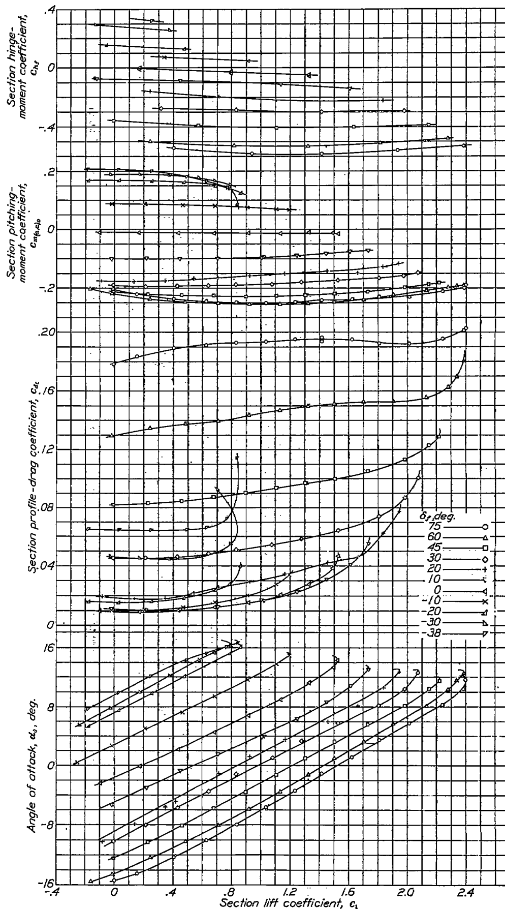
FIGURE 9.—Section aerodynamic characteristics of N. A. O. A. 23012 airfoil with a 0.20c plain flap.
