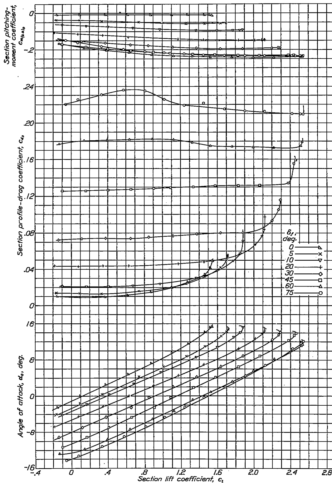
FIGURE 8.—Section aerodynamic characteristics of N. A. C. A. 23012 airfoil with a 0.20c split flap.
