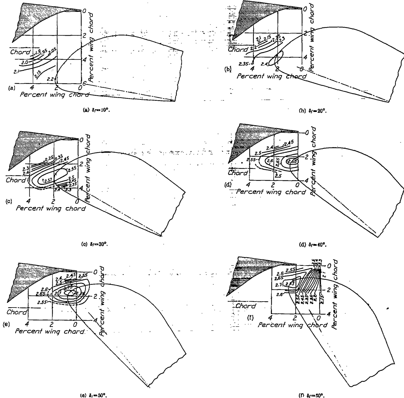
FIGURE 15.—Contours of flap location for c_{l,max} . Slotted flap 1-b.
