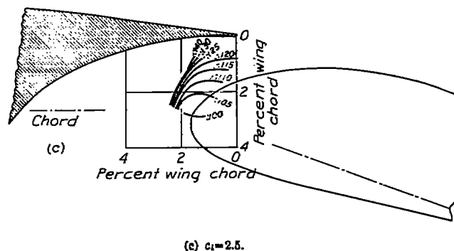
FIGURE 26.—Contours of flap location for c_{L_0} . Slotted flap 2-l.
