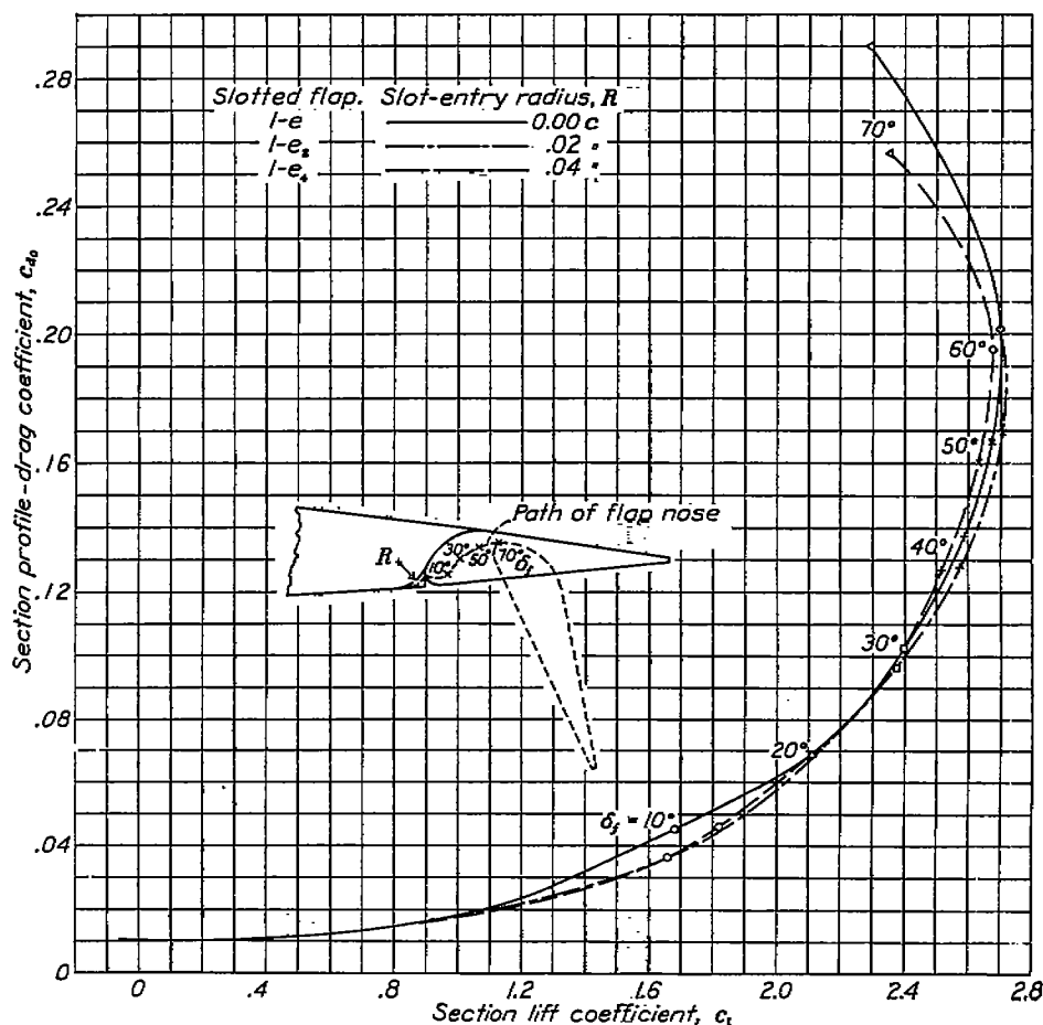
FIGURE 24.—Effect of slot-entry radius on c_{d_0} .
