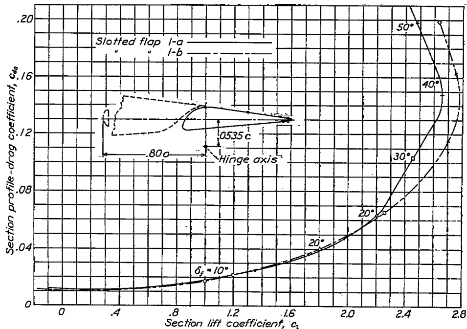
FIGURE 13.—Comparison of slotted flaps 1-a and 1-b.
