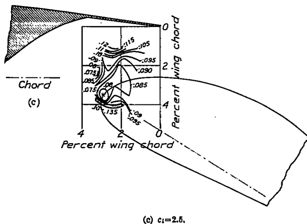
FIGURE 25.—Contours of flap location for c_{L_0} . Slotted flap 2-h.
