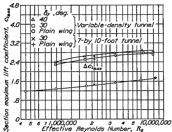
FIGURE 37.—Scale effect on c_{l,max} for N. A. C. A. 23012 airfoil with and without 0.256c slotted flap 2-h.
