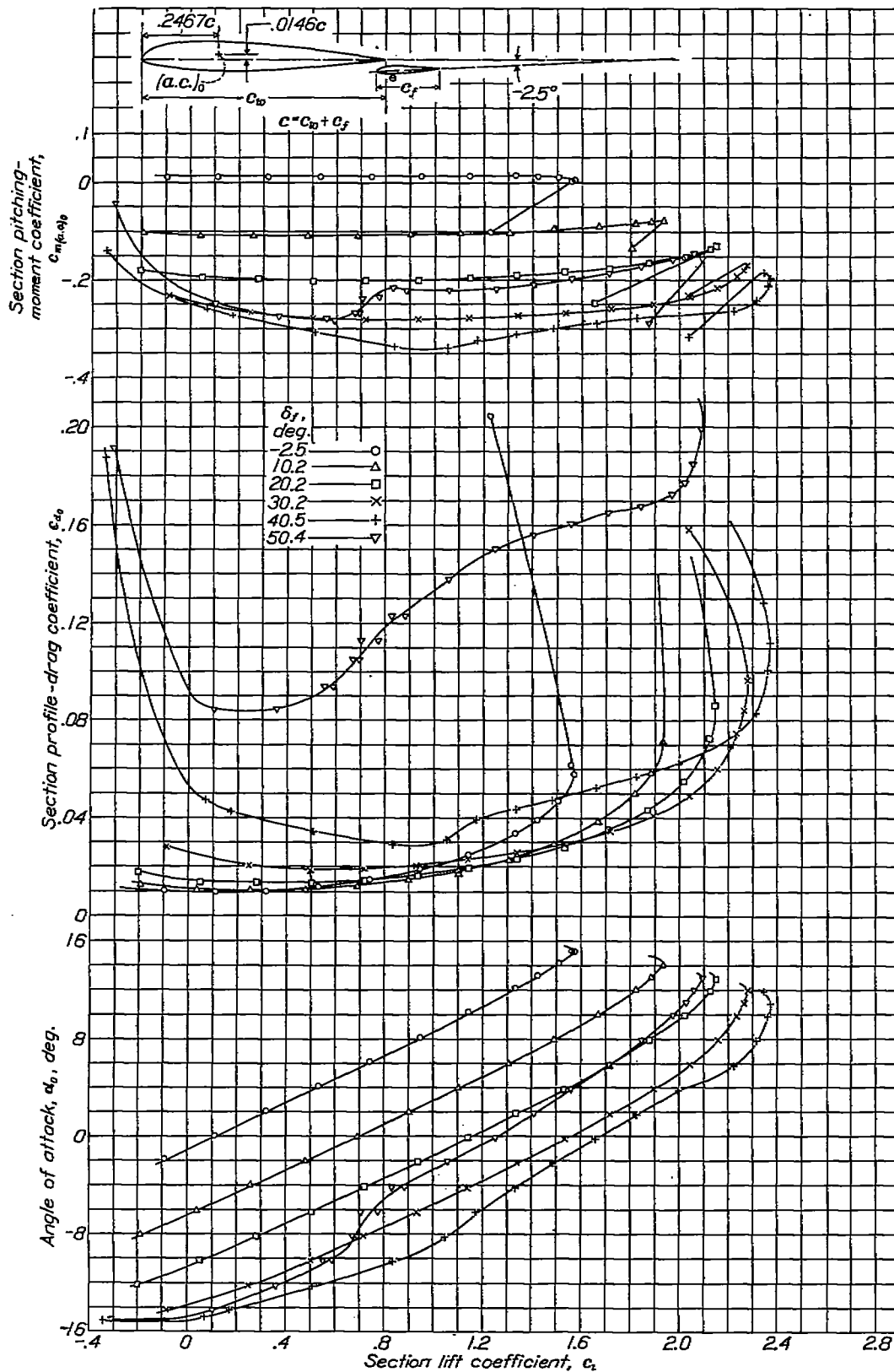
FIGURE 10.—Section aerodynamic characteristics of N. A. C. A. 23012 airfoil with a 0.2667c N. A. C. A. 23012 external-airfoil flap.
