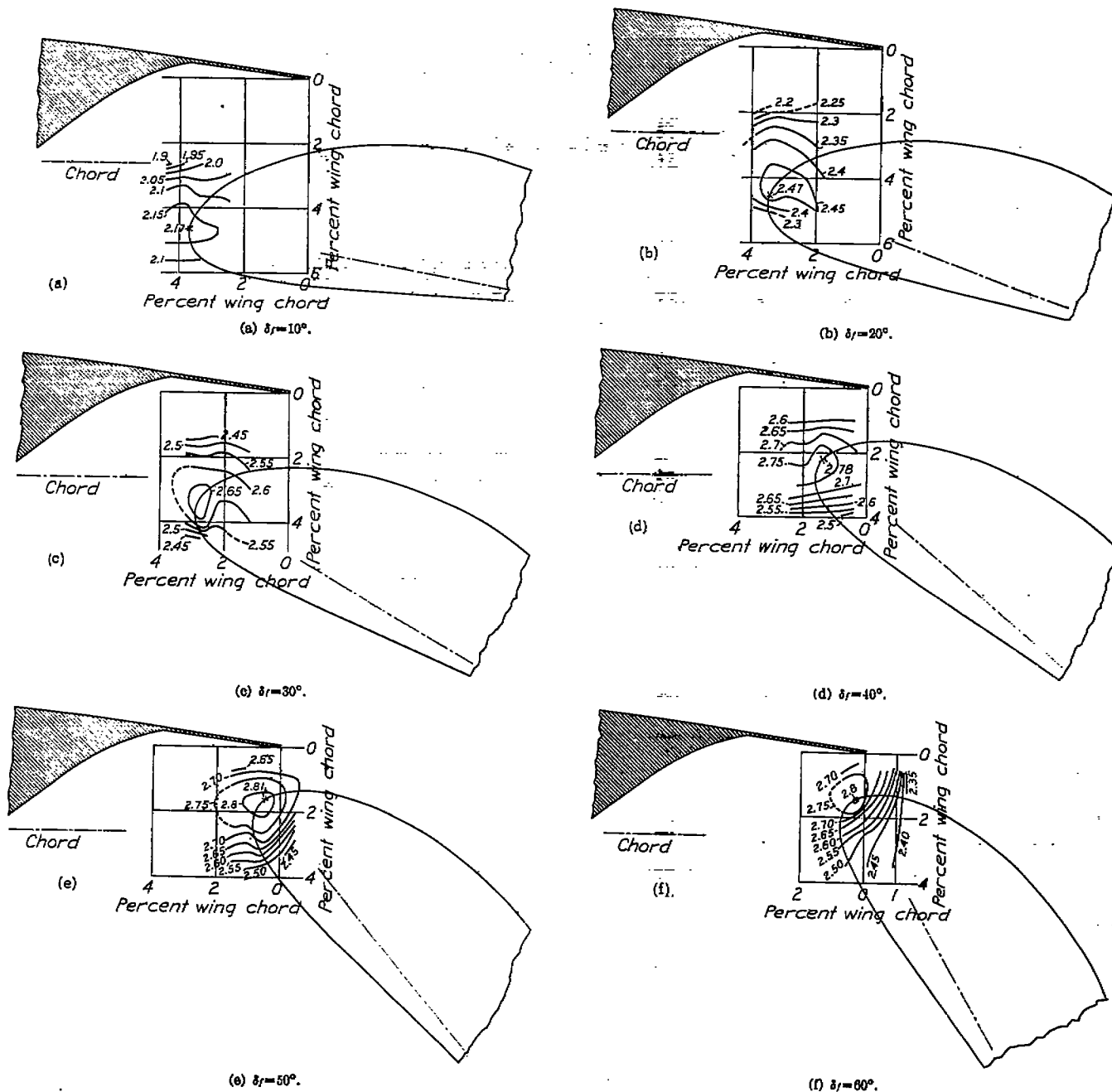
FIGURE 18.—Contours of flap location for c_{l,max} . Slotted flap 2-h.
