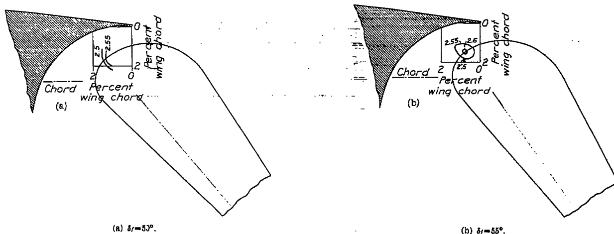
FIGURE 21.—Contours of flap location for c_{l_{max}} . Slotted flap 3-g.
