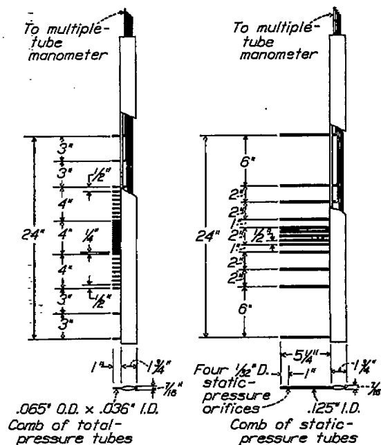
FIGURE 3.—Combs of total- and static-pressure tubes.
