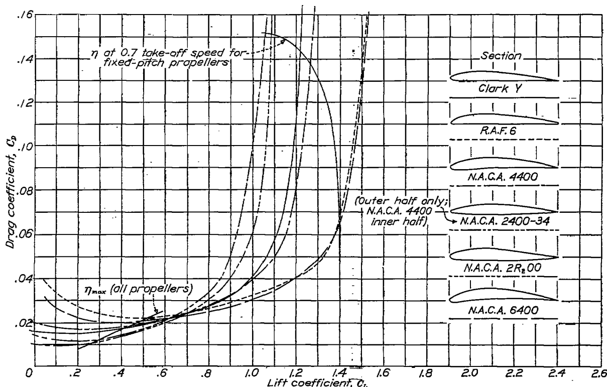
FIGURE 36.—Polar airfoil section characteristics reduced from propeller results. V/V_\infty = 0.46 (approximately); blade angle, 25° at 0.75R.
