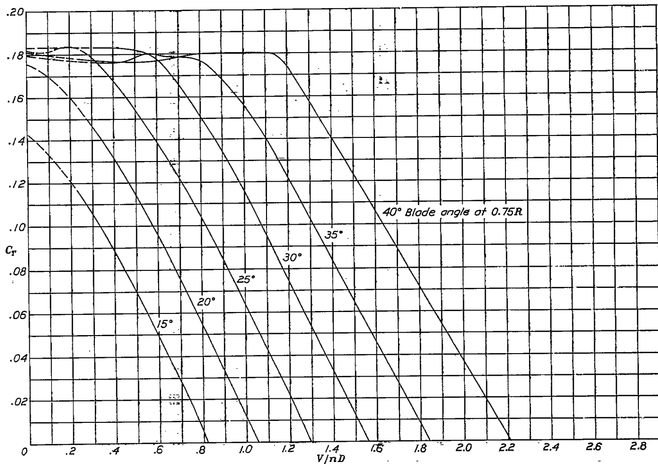
FIGURE 11.—Thrust-coefficient curves for propeller 5808-R6 (R. A. F. 6 section).
