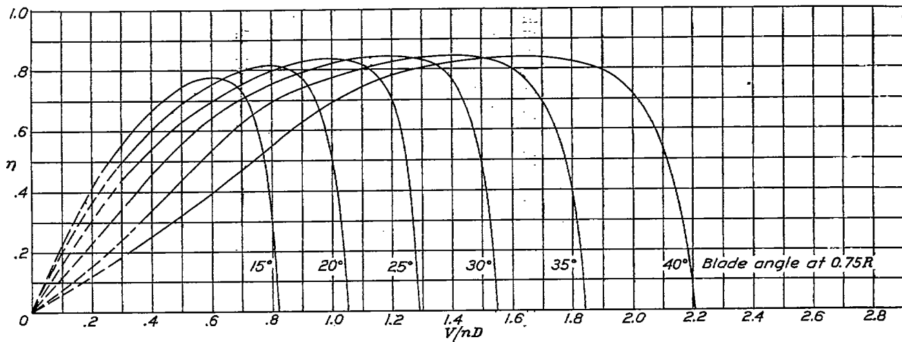
FIGURE 10.—Efficiency curves for propeller 5808-R6 (R. A. F. 6 section).
