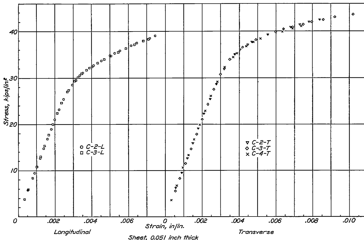
FIGURE 10.—Pack compressive tests on aluminum alloy 178T sheet.
