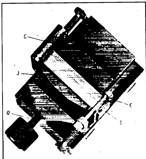
FIGURE 3.—Machining jig.
