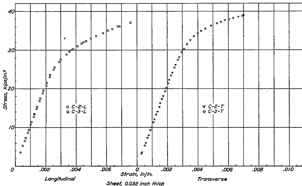
FIGURE 9.—Pack compressive tests on aluminum alloy 178T sheet.
