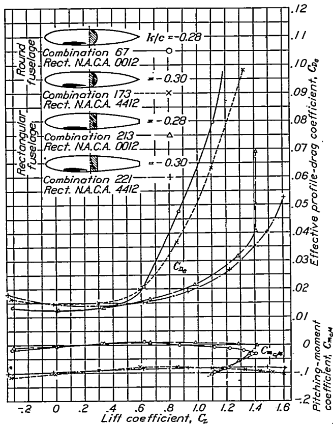
FIGURE 1.—Effect of fuselage section on wing-fuselage interference.
