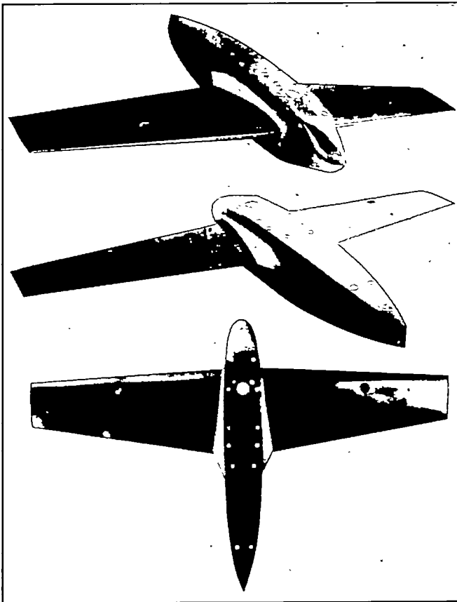
FIGURE 8.—Combination 229, showing tapered fillets.
