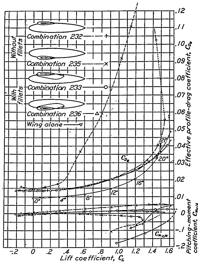
FIGURE 4.—Effect of fillets on tapered-wing, round-fuselage combinations; k/c = \pm 0.34 .
