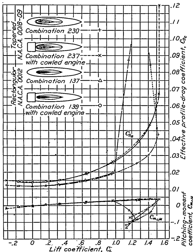
FIGURE 7.—Characteristics of cowled-engine, filleted combinations; k/c = 0 .
