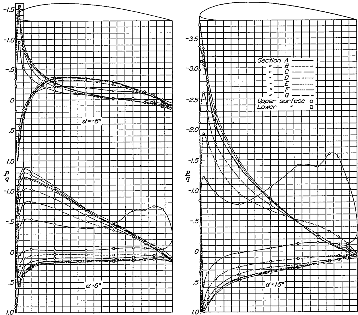
FIGURE 4.—Pressure distribution over airfoil sections at three angles of attack; \delta_1 = 0^\circ .
