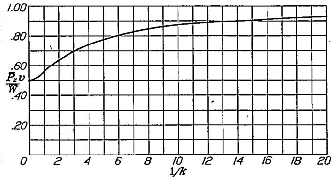
FIGURE 3.—The ratio of energy of propulsion to the energy required to maintain the oscillations \left(\frac{\bar{P}_x v}{W}\right) as a function of 1/k for the case of pure flapping.
