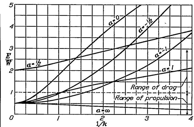
FIGURE 4.—The ratio of the energy dissipated in the wake to the energy required to maintain the oscillations (\bar{E}/W) as a function of 1/k for the case of pure angular oscillations about x=a .
