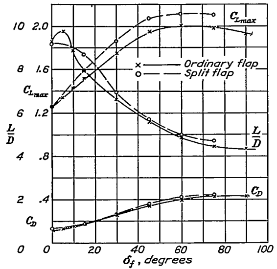
FIGURE 19.—Effect of flap deflection on maximum lift, and on lift-drag ratio and drag at maximum lift. The 0.20c full-span ordinary and split flaps on the Clark Y airfoil.
