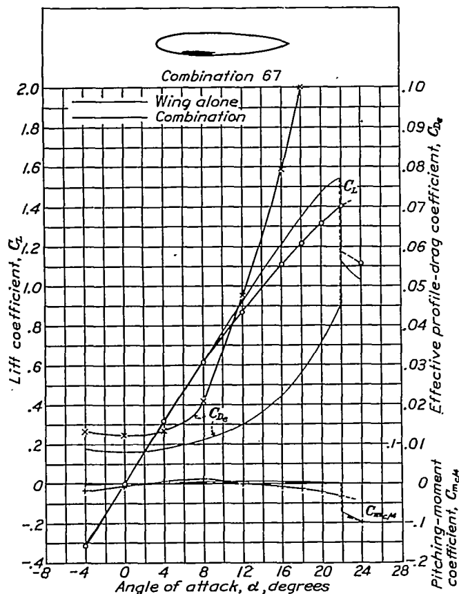
FIGURE 9.—Aerodynamic characteristics of a typical low-wing combination.
