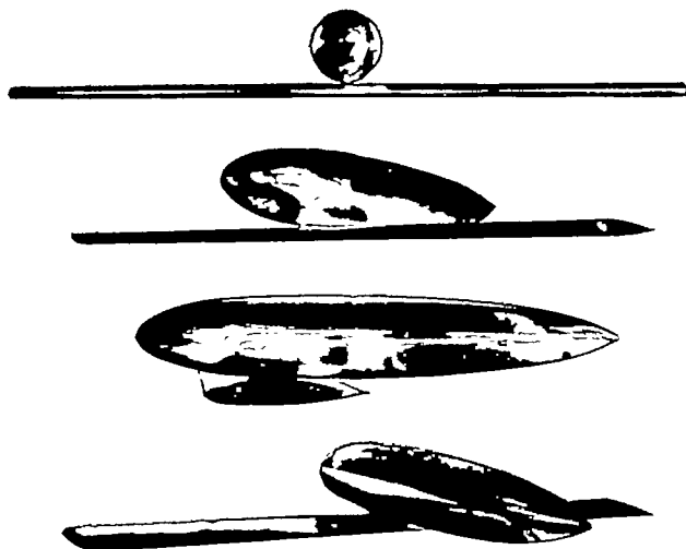
FIGURE 24.—Combination 72 (combination 24 inverted) showing poor junctions at the wing roots.
