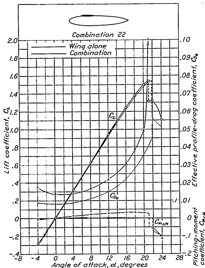
FIGURE 5.—Aerodynamic characteristics of a typical high-wing combination.
