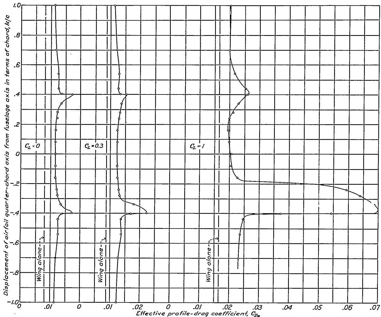
FIGURE 10.—Variation of effective profile-drag coefficient with vertical wing position. Rectangular wing of N. A. C. A. 0012 airfoil section and round fuselage; d/c=0 ; i_w=0^\circ .
