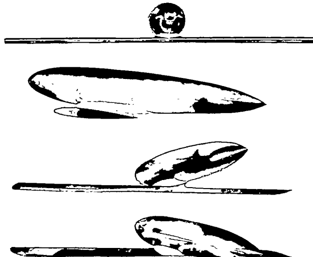
FIGURE 27.—Combination 146 (combination 143 inverted) showing small tapered fillets.
