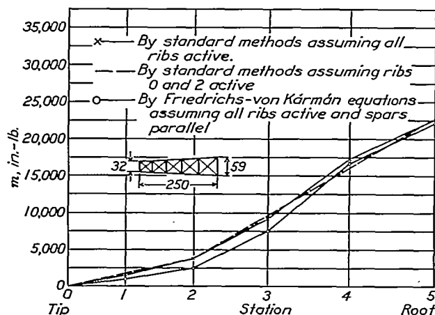
FIGURE 18.—Relief moments in XHB-3 wing frame calculated by three methods.
