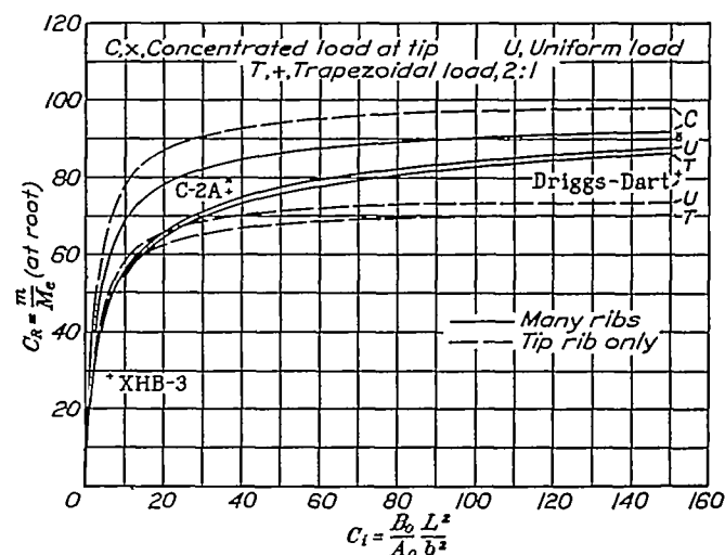
FIGURE 23.—Relief coefficient for wings with constant-section spars.
