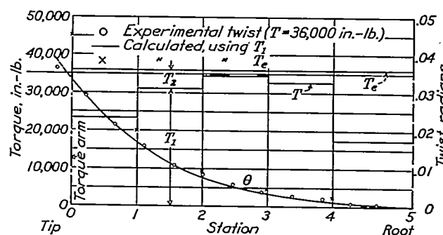
FIGURE 16.—Torque and twist in C-2A Transport wing.
