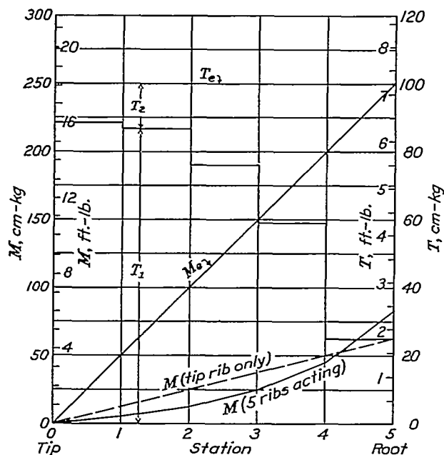
FIGURE 9.—Torque and bending moments in duralumin wing frame.
