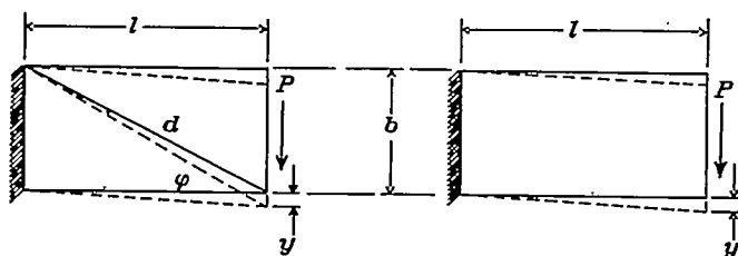
FIGURE 11.—Shear deflection of truss panel and solid sheet.
