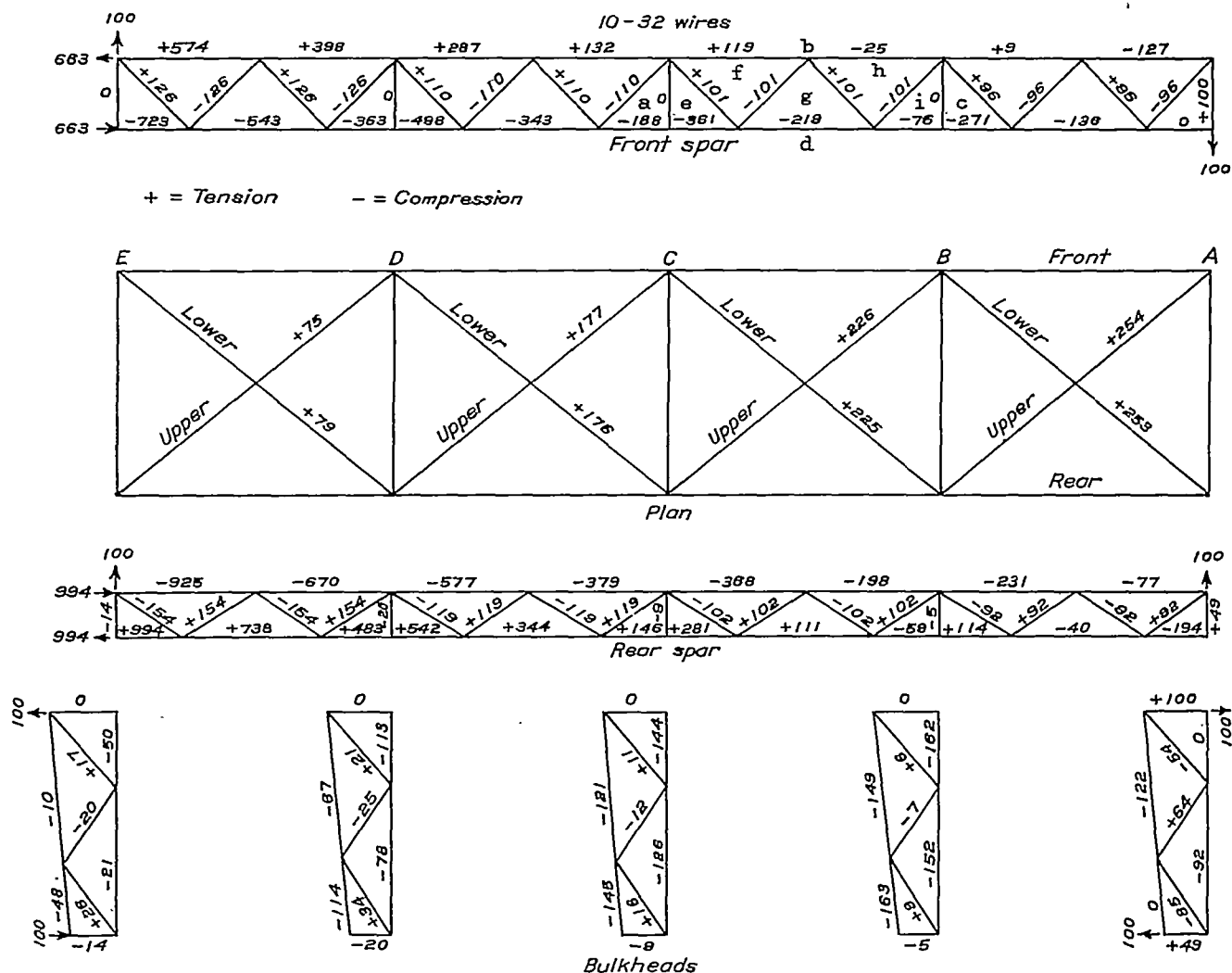
FIGURE 14.—Stress sheet for trussed wing frame (reference 9). Four-pin support; 100-lb. down on tip of front spar; 100-lb. up on tip of rear spar.
