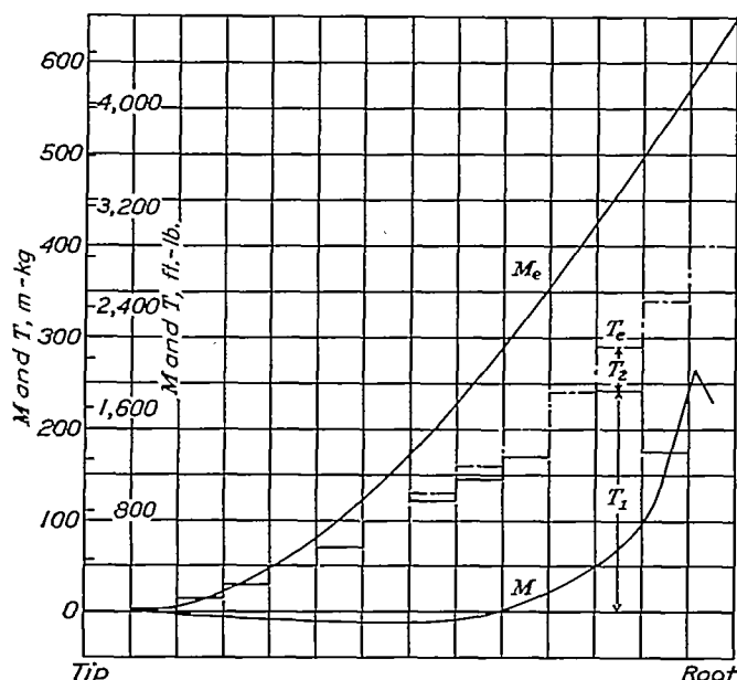
FIGURE 22.—Torque and bending moments (experimental) in plywood covered wing.
