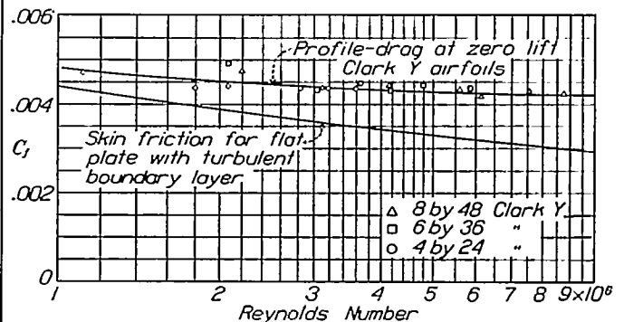
FIGURE 13.—Comparison of the Clark Y profile-drag coefficient at zero lift with the skin-friction drag coefficient for a flat plate having a completely turbulent boundary layer. C_D for airfoils based on actual surface area.
