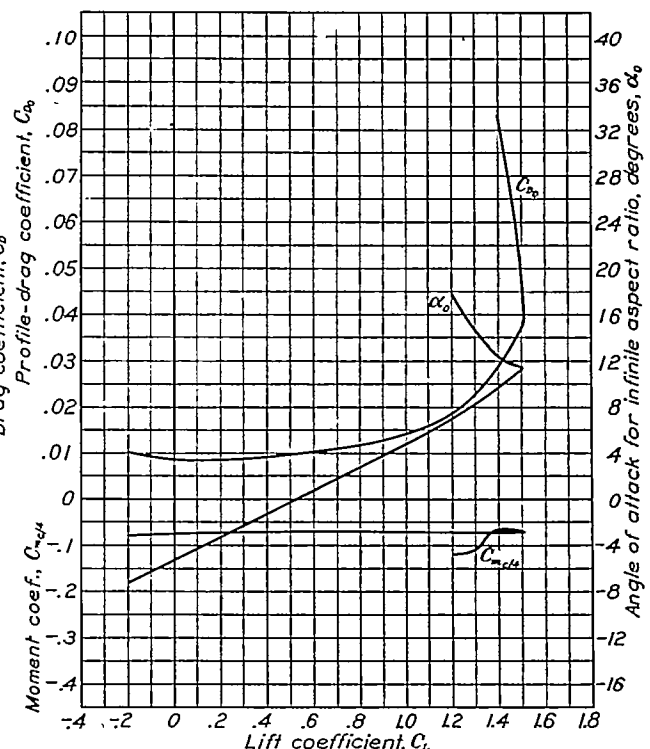
FIGURE 8.—Characteristics of the 8 by 48 Clark Y airfoil at a Reynolds Number of about 6,000,000.
