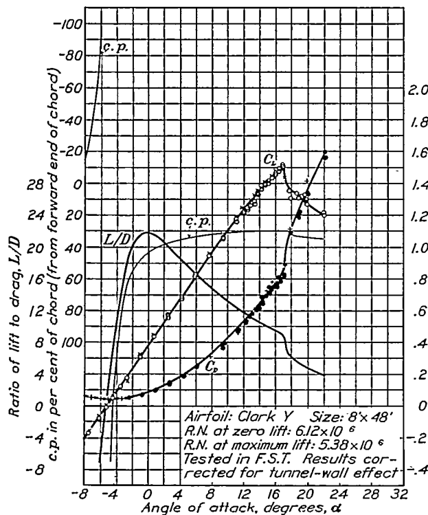
FIGURE 8.—Characteristics of the 8 by 48 Clark Y airfoil at a Reynolds Number of about 6,000,000.
