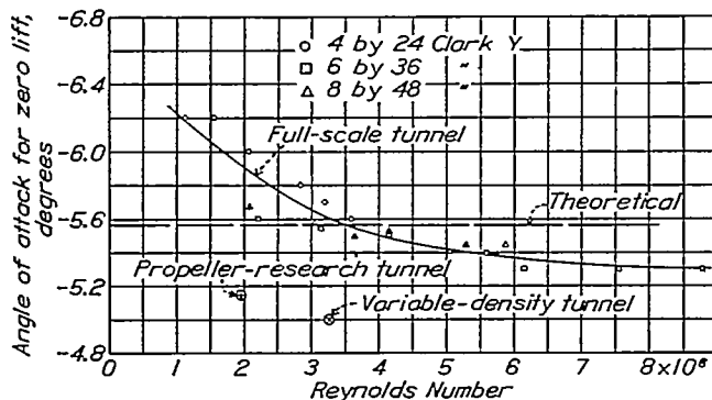
FIGURE 10.—Variation with Reynolds Number of the Clark Y angle of attack at zero lift. Propeller-research-tunnel value from reference 3. Variable-density-tunnel value from reference 4. Theoretical value from reference 5.
