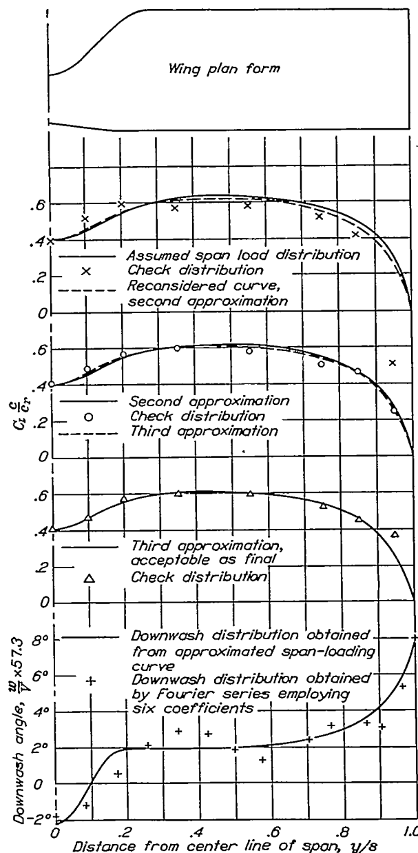
FIGURE 3.—Approximation of span load distribution for a wing with cut-out. \alpha_a = 8^\circ .
