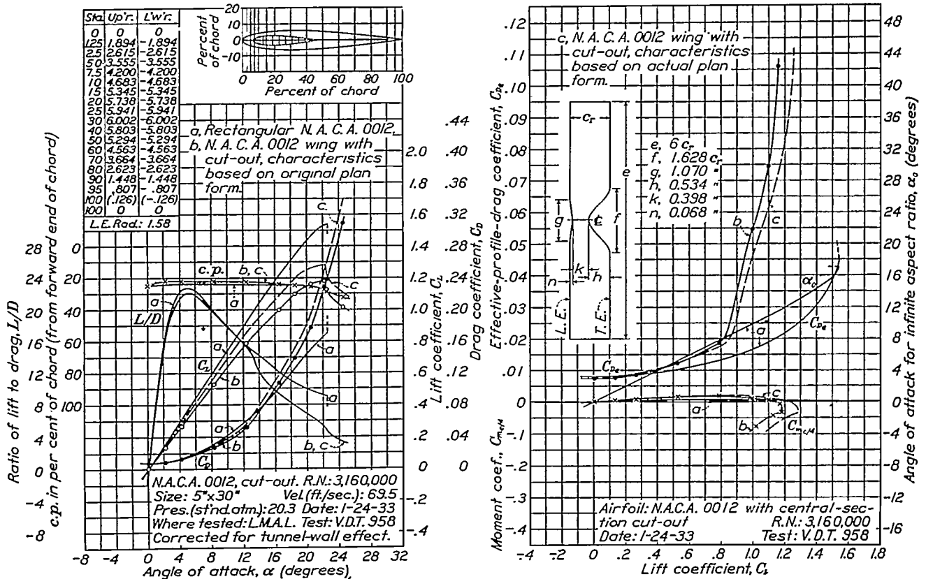
FIGURE 2.—Characteristics of a wing with central-section cut-out.
