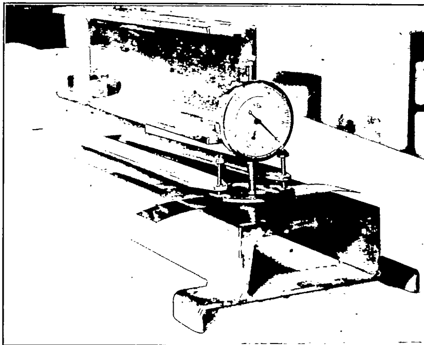
FIGURE 11.—Thickness tester.
