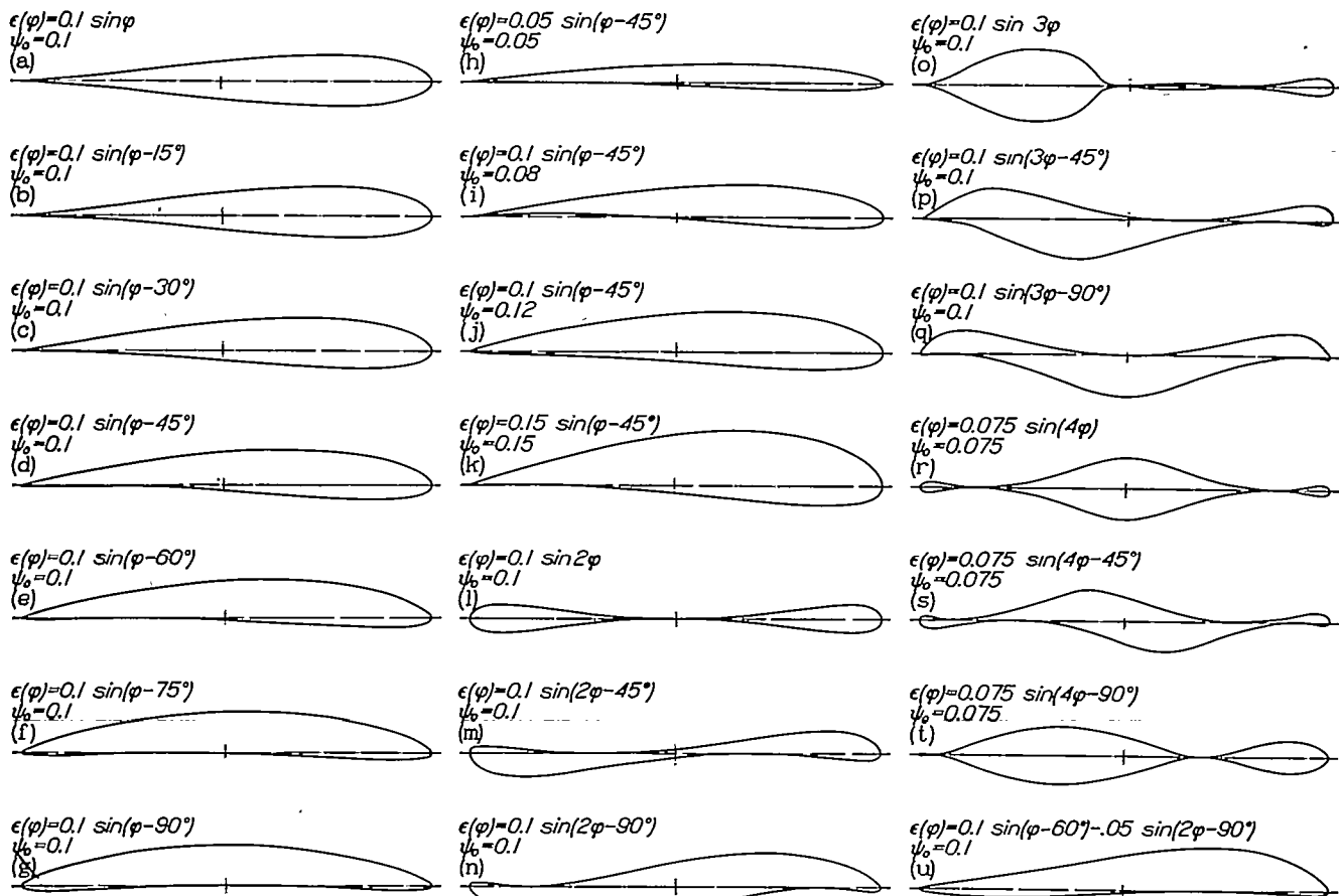
FIGURE 29.—Airfoils created by varying \epsilon(\varphi)
