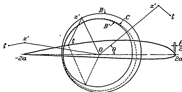
FIGURE 4.—Transformation of airfoil into a nearly circular contour
