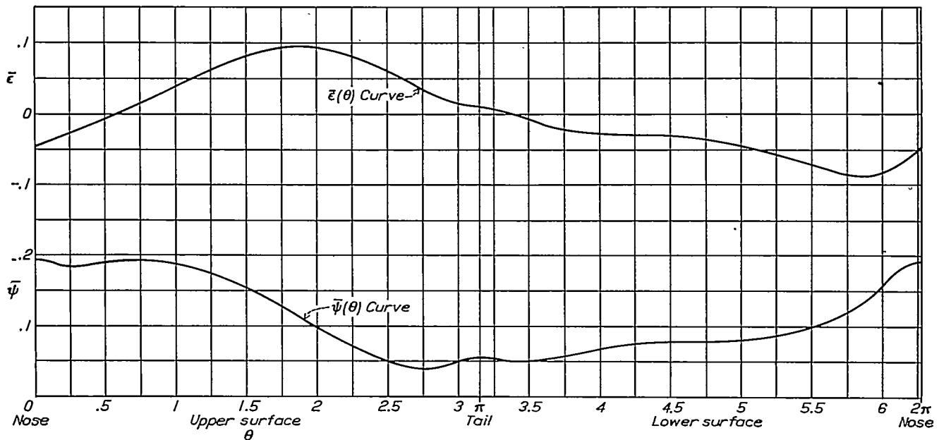
FIGURE 27.—The z(\theta) and \bar{\psi}(\theta) curves for the N. A. C. A. -M6 airfoil
