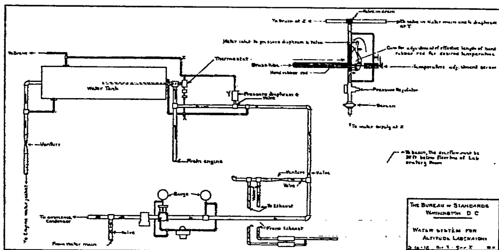
FIG. 5. Diagrammatic arrangement of circulating water piping and thermostat temperature control arrangement.
