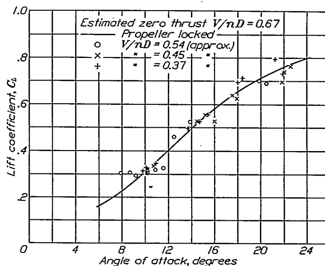
FIGURE 9.—Lift coefficient against angle of attack with varying thrust
