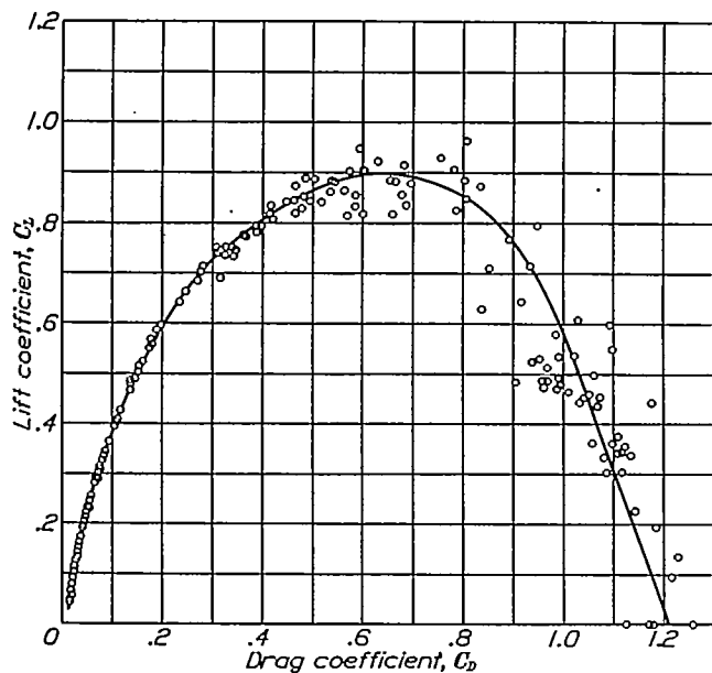
FIGURE 4.—Polar curve for PCA-3 autogiro
