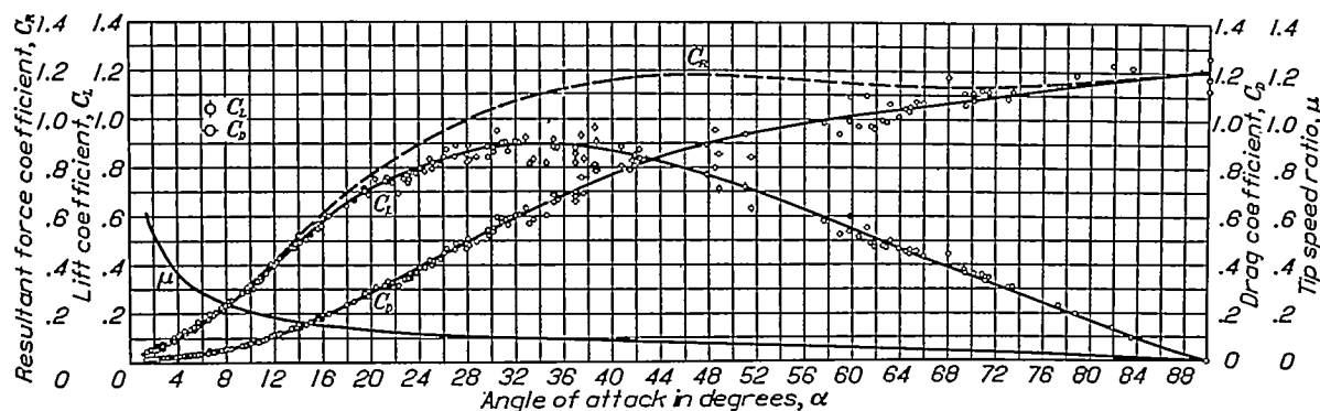
FIGURE 3.—Characteristic curves for PCA-3 autogiro
