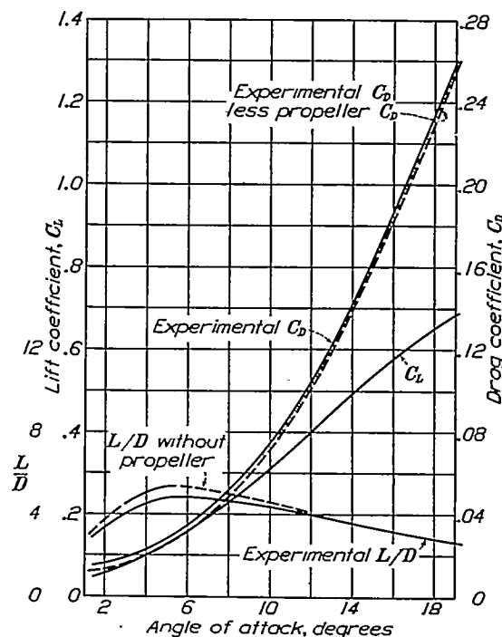
FIGURE 5.—Curves showing effect of propeller on PCA-3 autogiro characteristic curves. Estimated propeller C_D=0.003 , propeller drag= 4.98 g. (From reference 3.)
