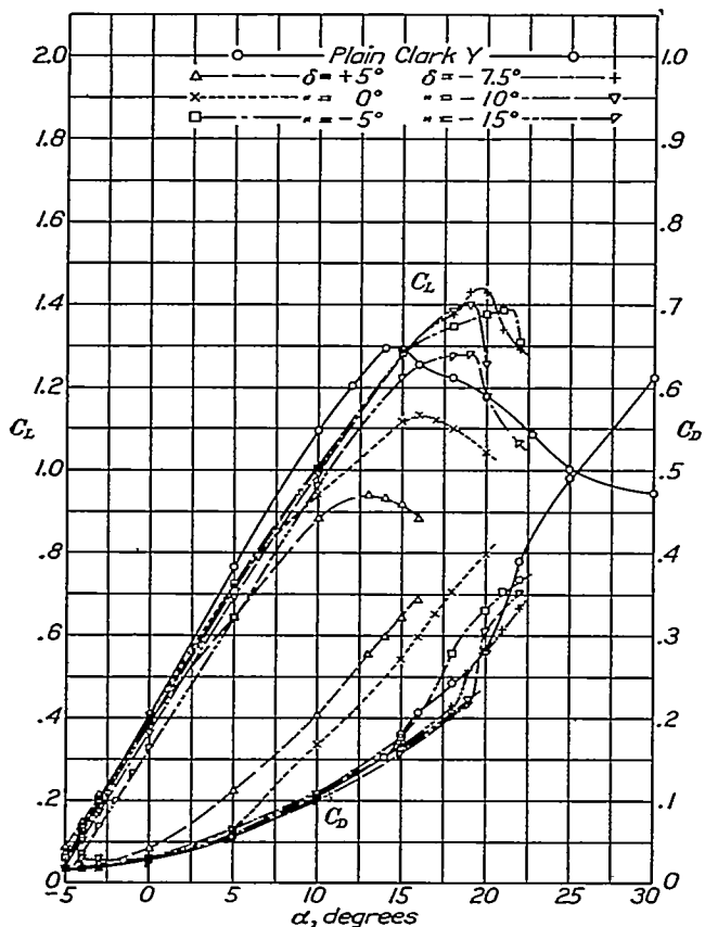
FIGURE 24.—Characteristics of combination of main and auxiliary wings with trailing edge of auxiliary 20 per cent chord behind leading edge and 19 per cent chord above chord line of main wing
