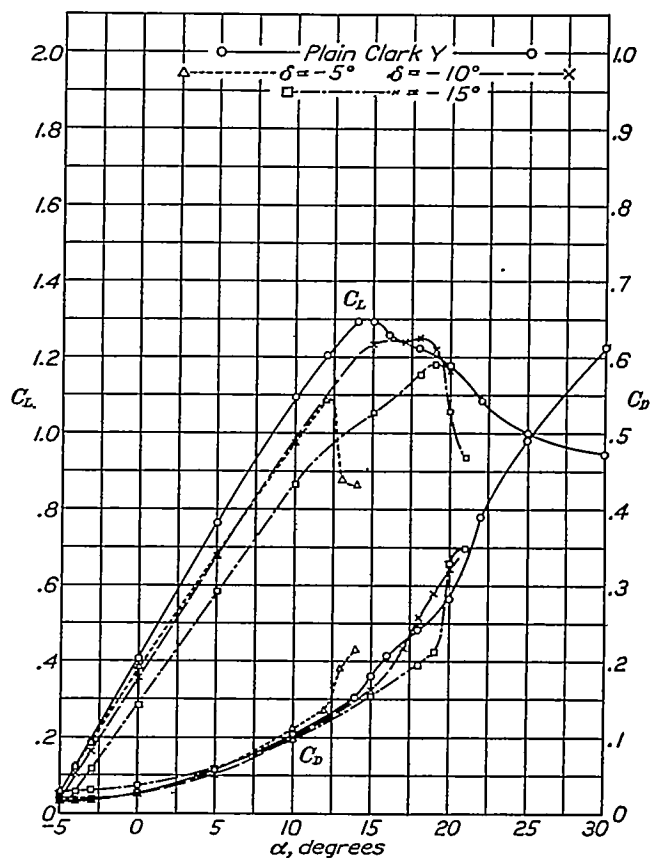
FIGURE 23.—Characteristics of combination of main and auxiliary wings with trailing edge of auxiliary 20 per cent chord behind leading edge and 14 per cent chord above chord line of main wing
