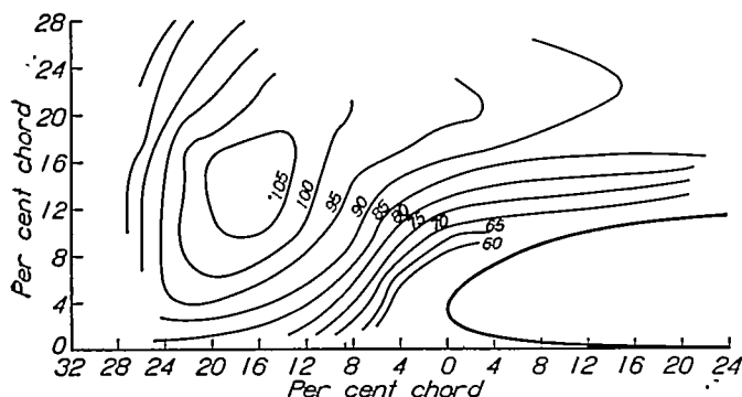
FIGURE 27.—Contours of equal values of C_{Lmax}/C_{Dmin} obtained with various settings of trailing edge of auxiliary airfoil. The value at any point represents the maximum that can be obtained with any angular position
