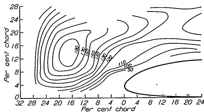
FIGURE 28.—Contours of equal values of (C_{Lmax})^2/C_{Dmin} obtained with various settings of trailing edge of auxiliary airfoil. The value at any point represents the maximum that can be obtained with any angular position
