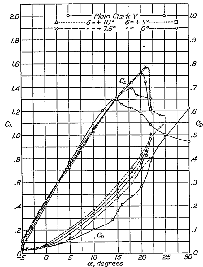
FIGURE 4.—Characteristics of combination of main and auxiliary wings with trailing edge of auxiliary 25 per cent chord ahead of leading edge and 19.5 per cent chord above chord line of main wing
