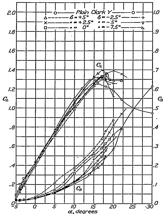
FIGURE 22.—Characteristics of combination of main and auxiliary wings with trailing edge of auxiliary 15 per cent chord behind leading edge and 28 per cent chord above chord line of main wing
