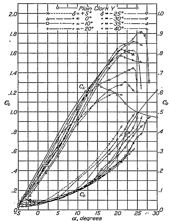
FIGURE 12.—Characteristics of combination of main and auxiliary wings with trailing edge of auxiliary 5 per cent chord ahead of leading edge and 6.5 per cent chord above chord line of main wing
