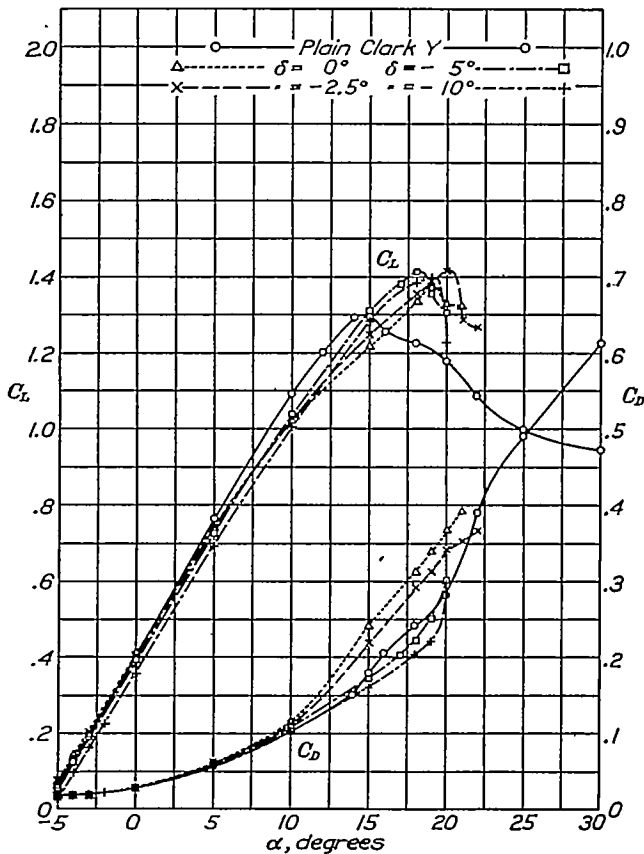
FIGURE 25.—Characteristics of combination of main and auxiliary wings with trailing edge of auxiliary 20 per cent chord behind leading edge and 24 per cent chord above chord line of main wing
