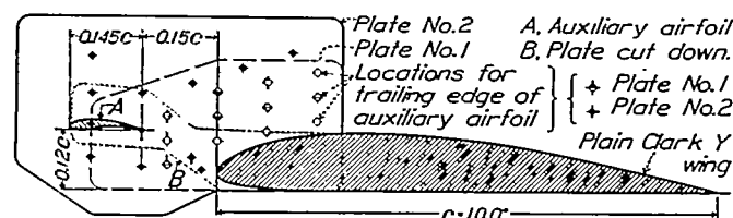
AUXILIARY ORDINATES
