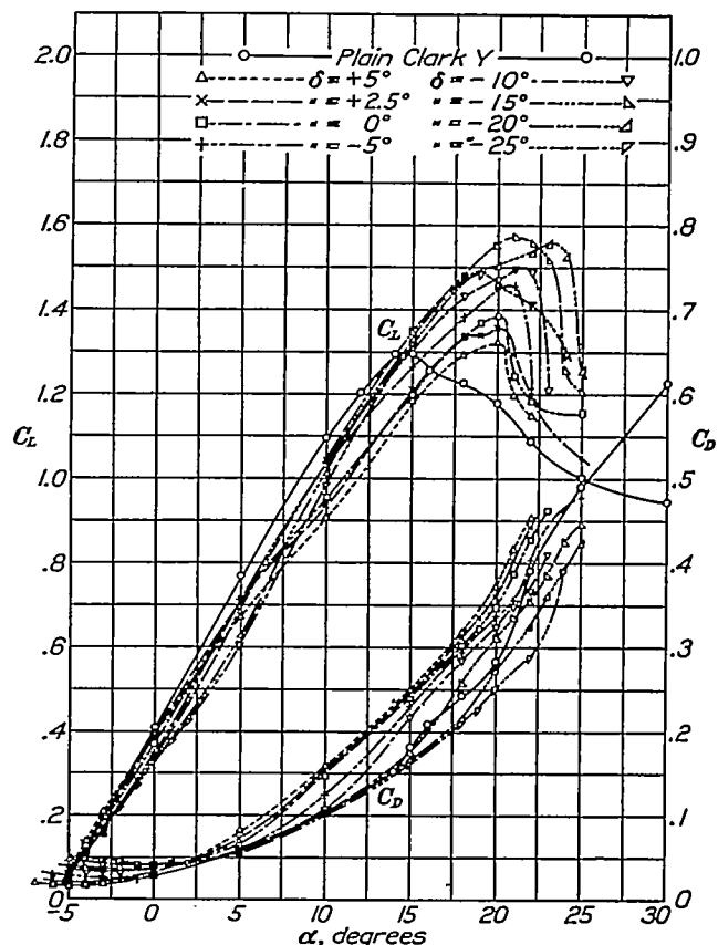
FIGURE 9.—Characteristics of combination of main and auxiliary wings with trailing edge of auxiliary 10 per cent chord ahead of leading edge and 5 per cent chord above chord line of main wing
