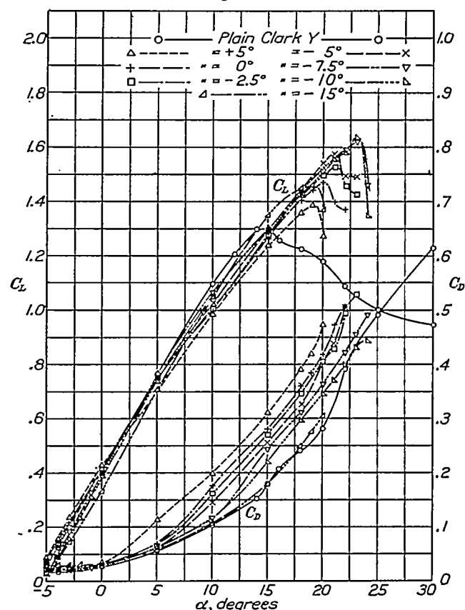
FIGURE 17.—Characteristics of combination of main and auxiliary wings with trailing edge of auxiliary 0 per cent chord ahead of leading edge and 20 per cent chord above chord line of main wing
