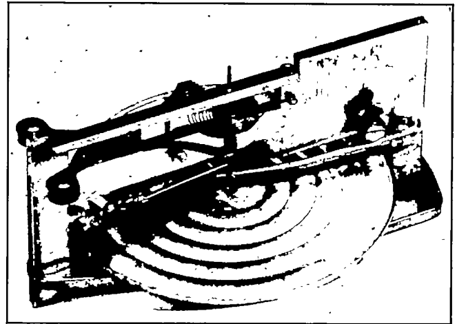
FIGURE 20.—Mechanism of a typical air-speed indicator
