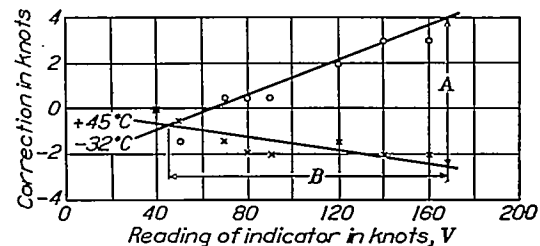
FIGURE 35.—Illustrating an instrument with an excessive change in scale errors with temperature
