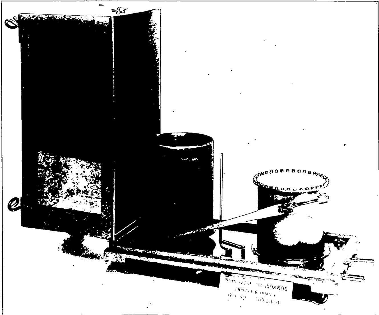
FIGURE 26.—Bureau of Standards air-speed recorder
