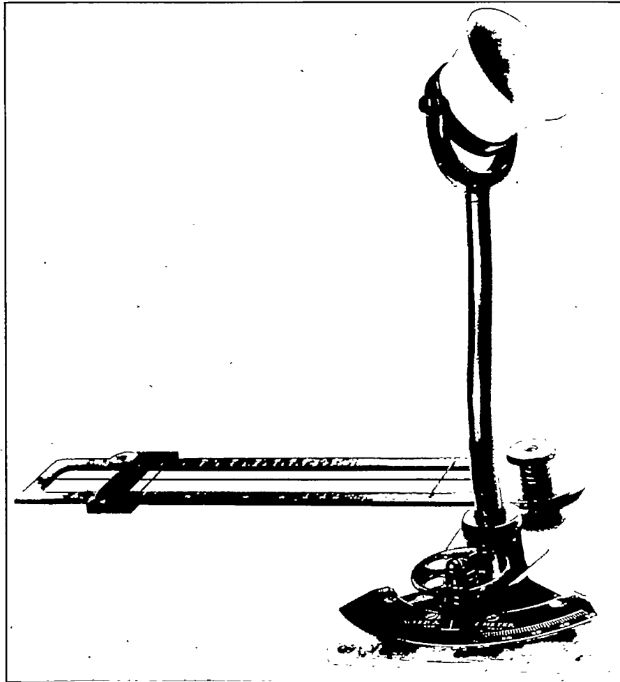
FIGURE 46.—Pionser drift and ground-speed indicator
