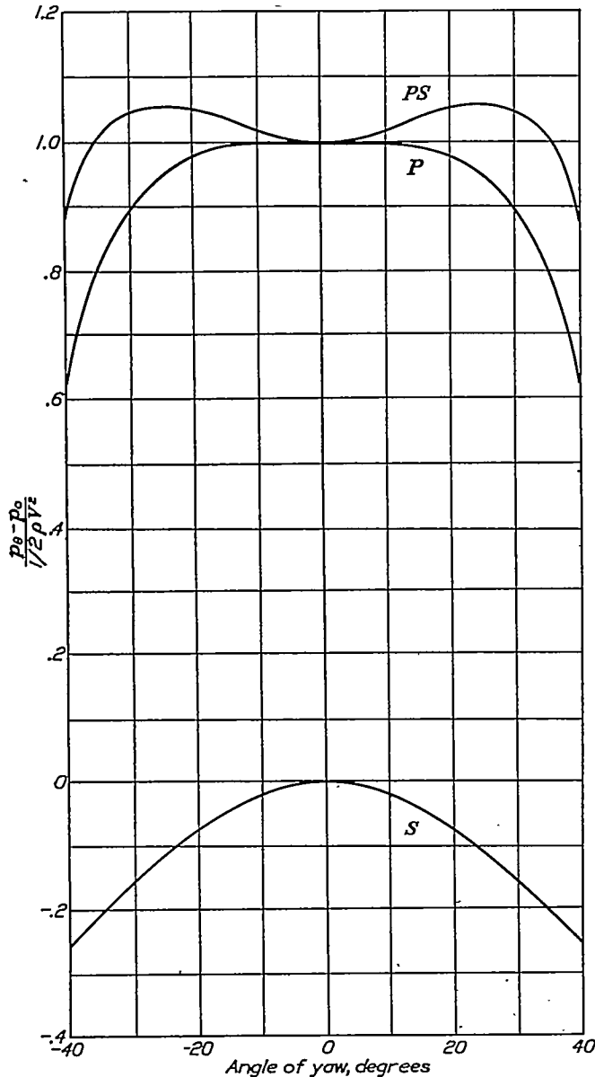
FIGURE 5.—Effect of yaw on performance of Pitot-static tube. The pressure developed is p_0 , the static pressure p_s , and the impact pressure \frac{1}{2} \rho V^2 . The curve S is for the static tube, the curve P for the Pitot tube, and the curve PS is for a combination of both
