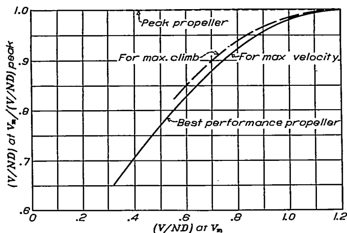
FIGURE 14a.—Comparison of propeller settings at V_{\max} for obtaining best maximum climb, best maximum velocity, and propeller set on peak efficiency
