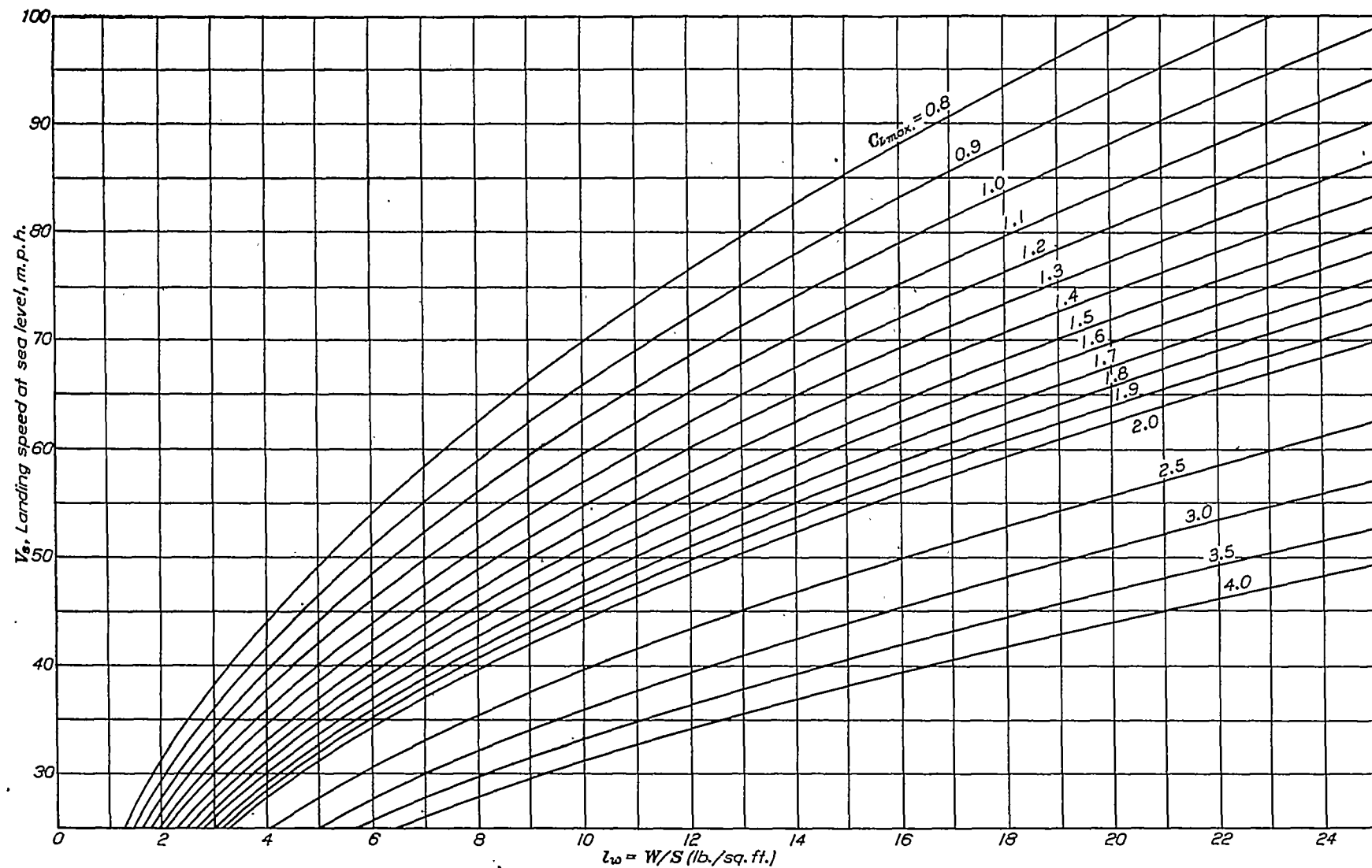
FIGURE 40.—Landing speed at sea level as a function of wing loading, l_w , and maximum lift coefficient, C_{Lmax} .
