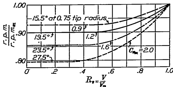
FIGURE 17.—Variation of full-throttle r. p. m. with velocity. Best performance propeller
