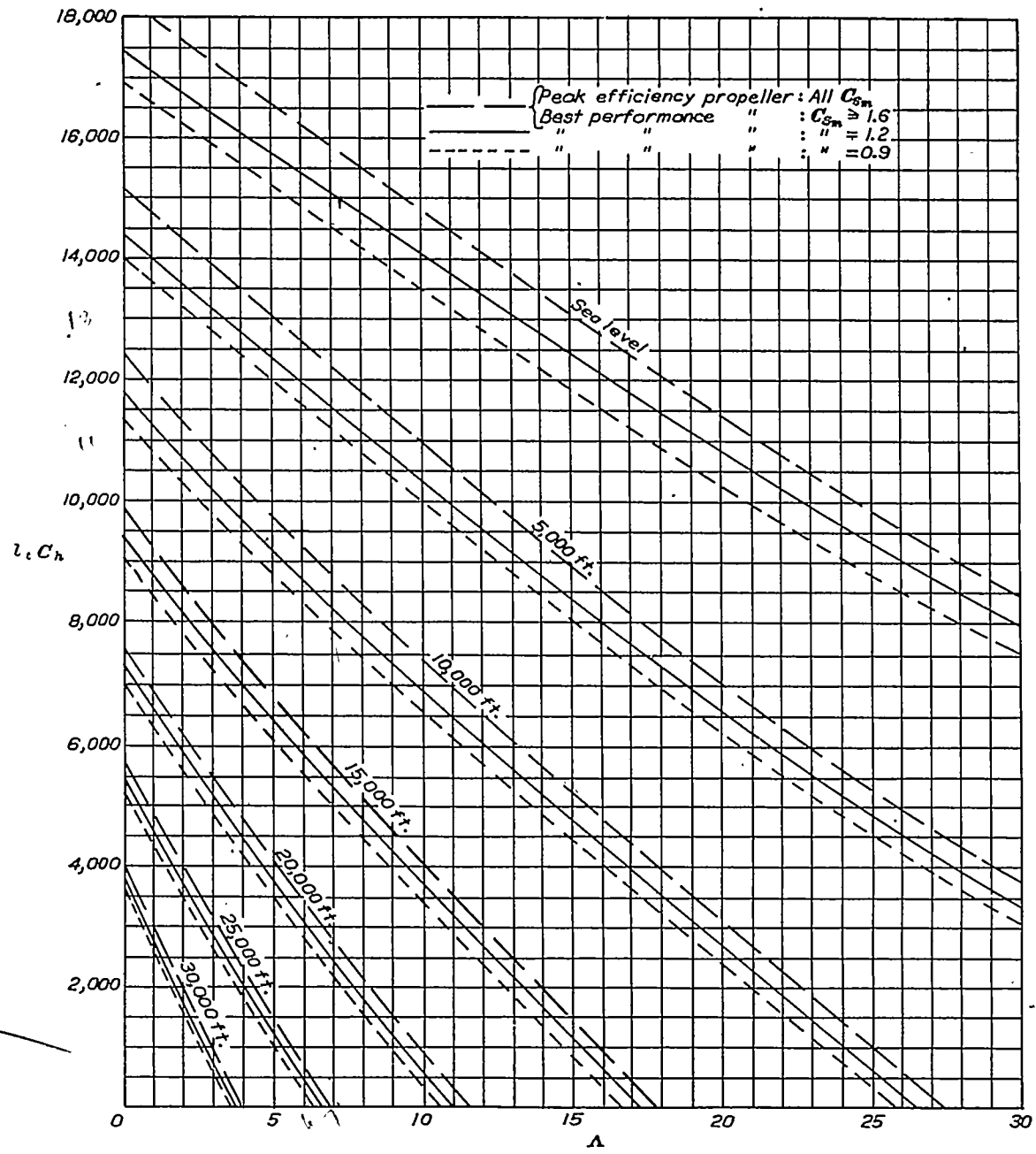
FIGURE 33.— l, C_h as a function of \Lambda , at various altitudes. C_h —maximum rate of climb in feet per minute
