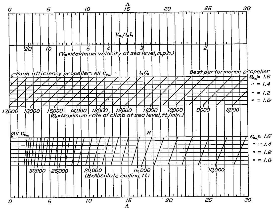
FIGURE 30.—Combination chart giving V_m / l_0 l_t , C_m , and H as functions of C_L
