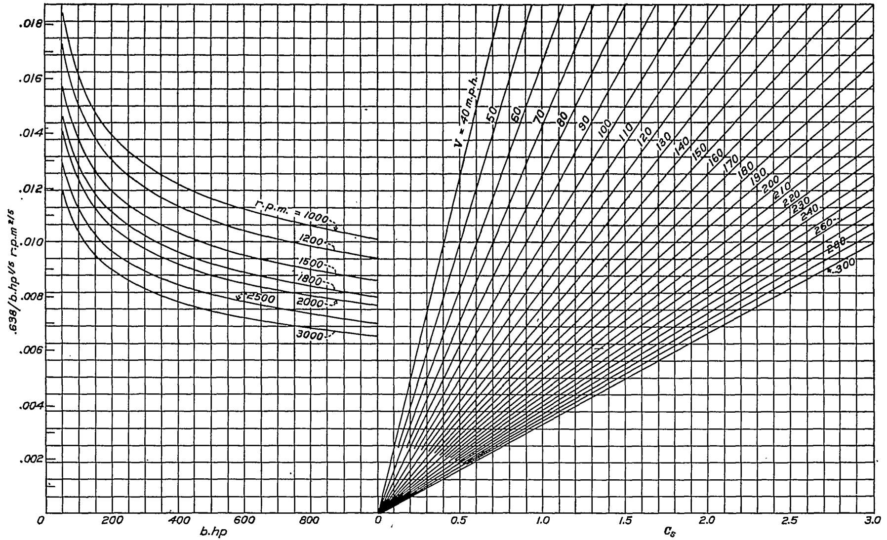
FIGURE 26.—Chart for graphical solution of C_s = \frac{.638 \text{ m. p. h.}}{b \cdot \text{hp}^{1/5} \text{ r. p. m.}^{2/5}} at sea level
