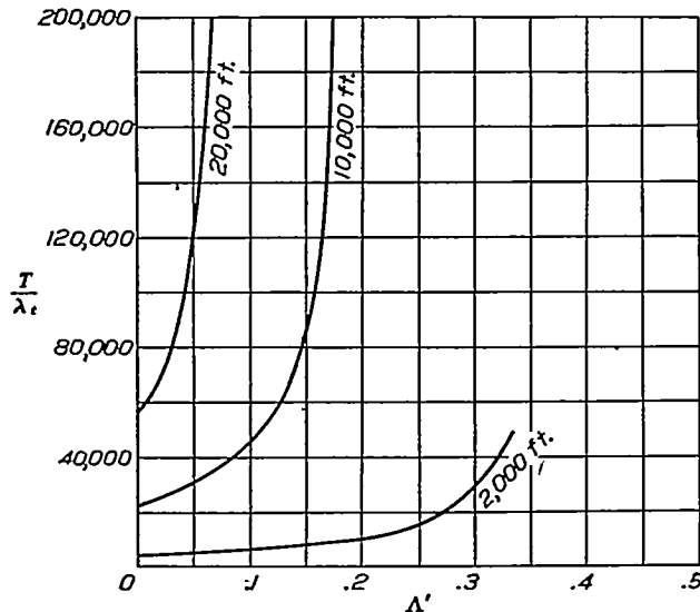
FIGURE 11.— \frac{T}{\lambda_i} as a function of \Delta' and altitude ( \sigma )
