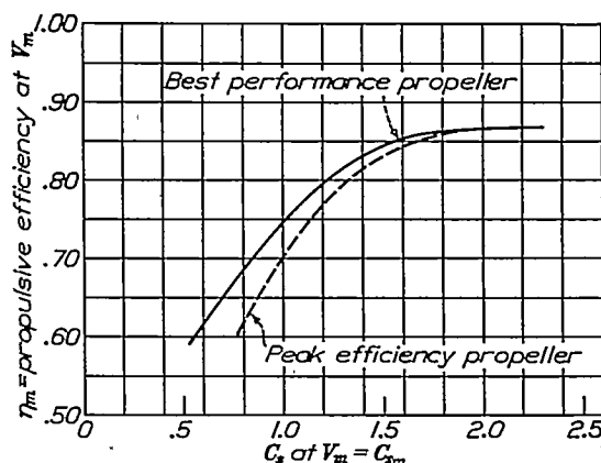
FIGURE 16b.—Propulsive efficiency at V_{max} as a function of C_s
