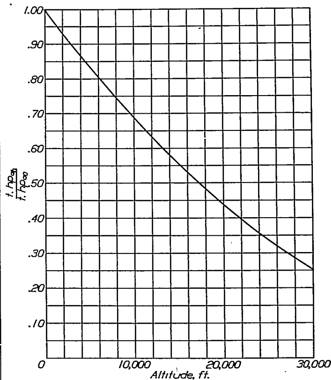
FIGURE 23.—Variation of full-throttle thrust horsepower available at constant velocity with altitude
