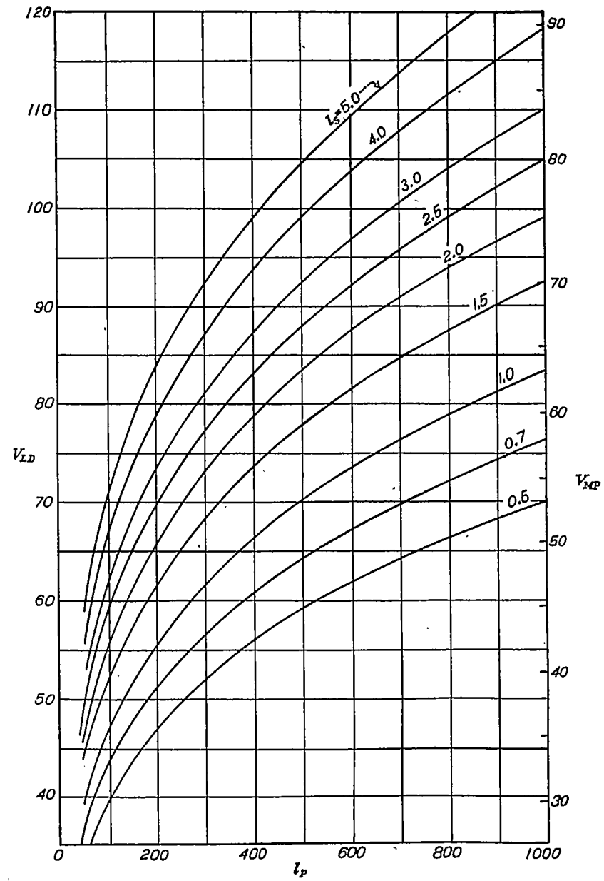
FIGURE 42.—Velocity for (\frac{L}{D})_{max} , V_{LD} , and velocity for minimum power, V_{MP} , as functions of l_p and l_i . Velocities in miles per hour
