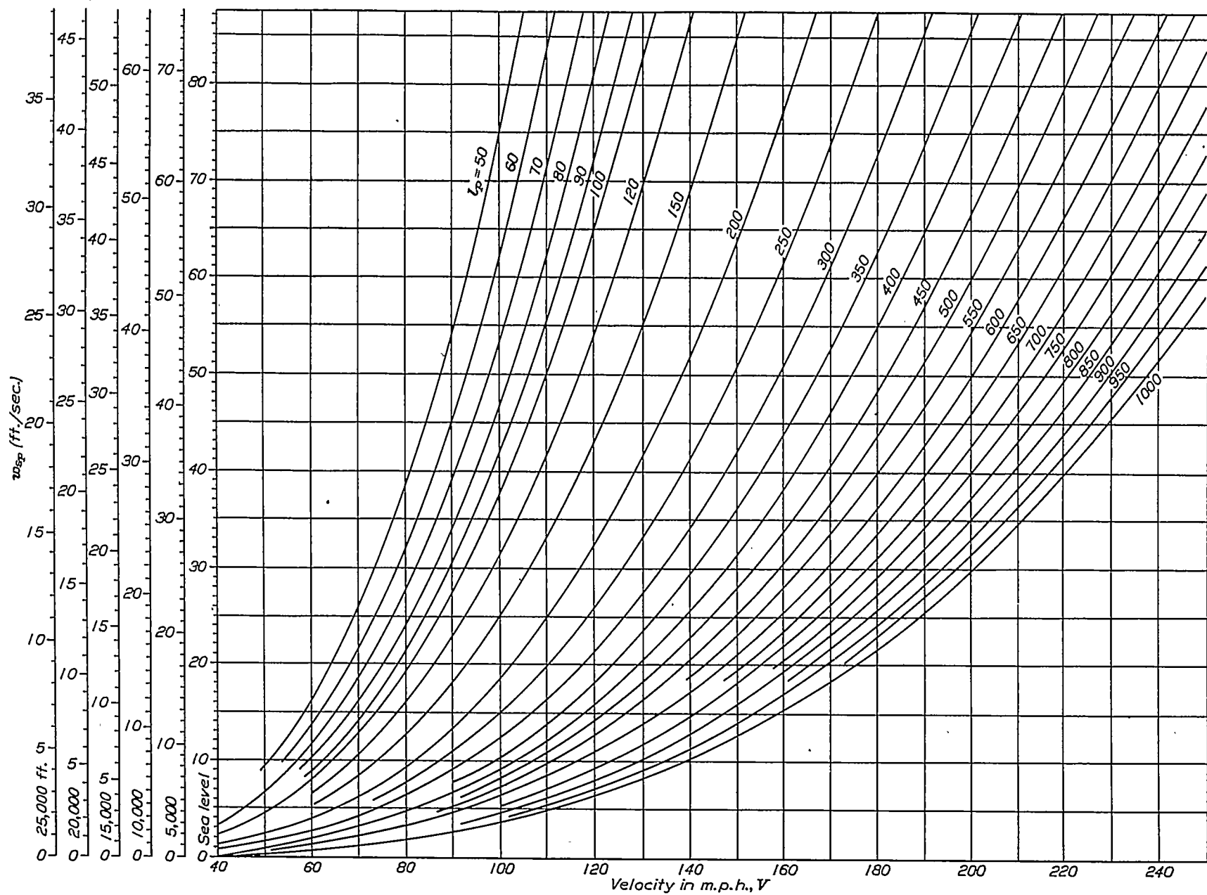
FIGURE 43.—The sinking speed w_{sp} , due to the parasite loading l_p , as a function of l_p and V , at various altitudes
