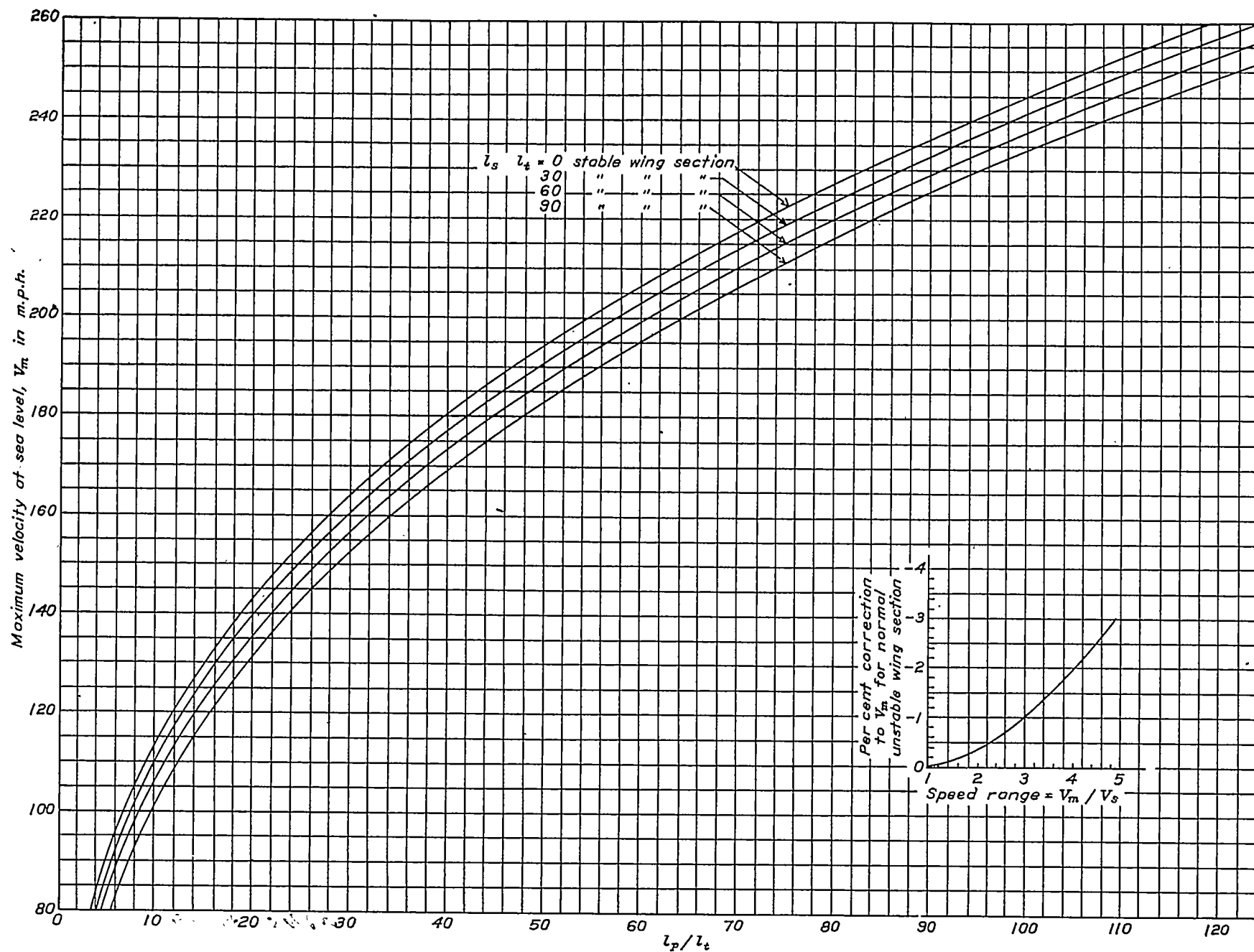
FIGURE 29.—Maximum velocity at sea level as a function of \frac{l_p}{l_t}
