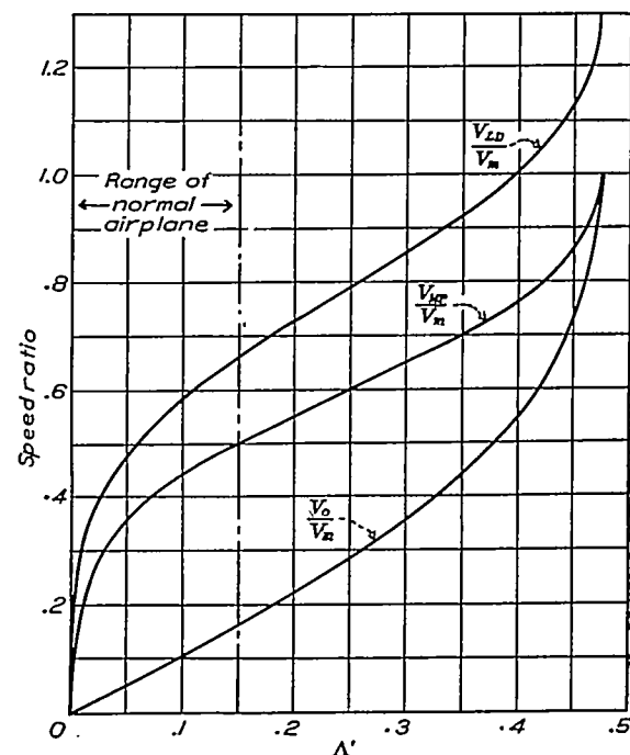
FIGURE 4.—Important speed ratios as functions of \Delta' . V_m = design maximum velocity; V_o = ideal minimum velocity; V_{MP} = velocity for minimum power required; V_{LD} = velocity for maximum \frac{L}{D} ; \frac{V_o}{V_m} = ideal speed ratio
