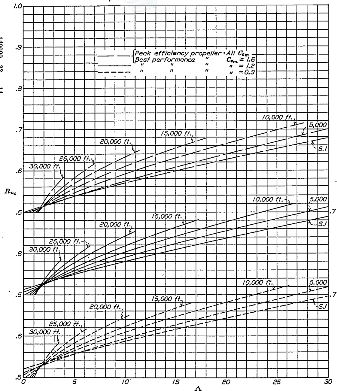
FIGURE 32.— R_{vc} = \frac{\text{velocity for maximum rate of climb}}{\text{maximum velocity at sea level}} as a function of \Lambda , at various altitudes
