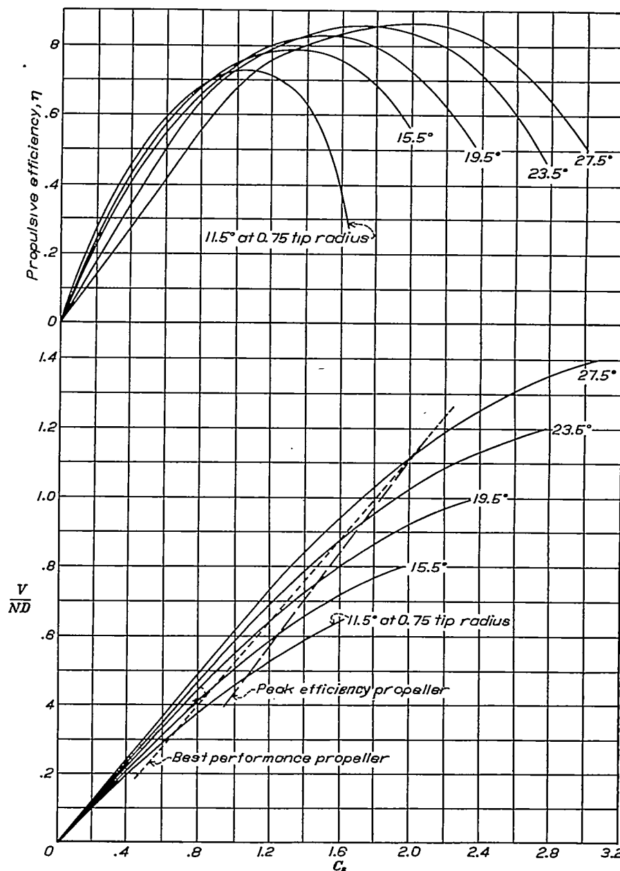
FIGURE 13.—Propeller characteristics of Navy metal propeller No. 4412. (National Advisory Committee for Aeronautics Technical Report No. 306.) Propellers set for best performance and peak efficiency are indicated
