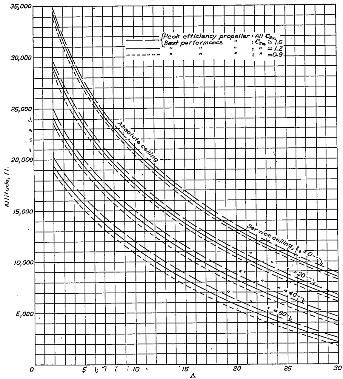
FIGURE 34.—Absolute ceiling and service ceiling as functions of \Lambda
