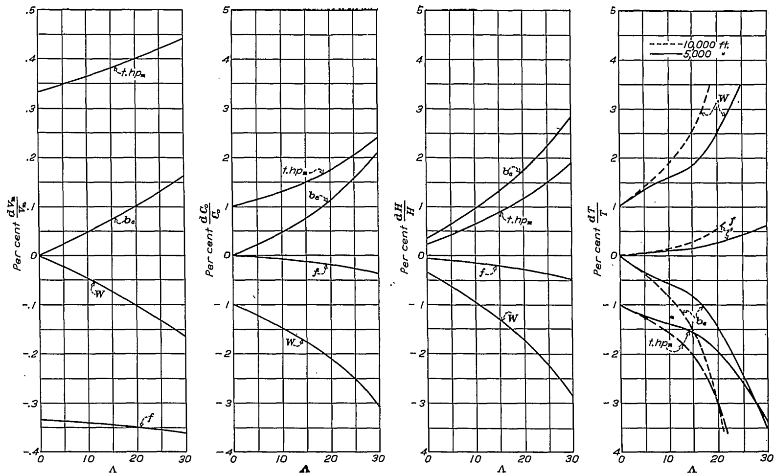
FIGURE 37.—Variation of performance with change of parameters. Charts show per cent change in performance due to 1 per cent (+1 per cent) change in parameter
