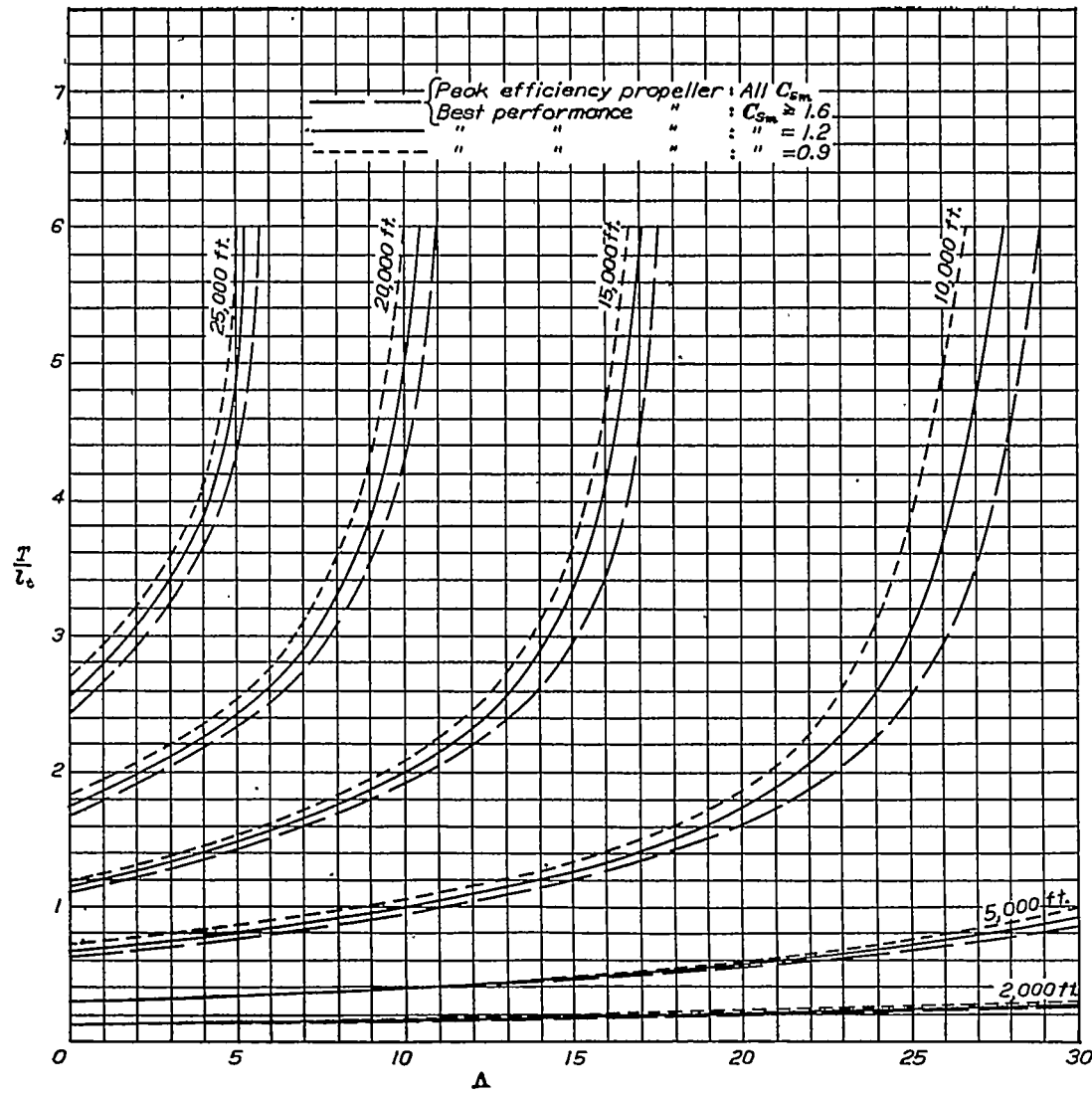
FIGURE 35.— \frac{T}{t_1} as a function of A , at various altitudes. T =minimum time required to climb to altitude (minutes)
