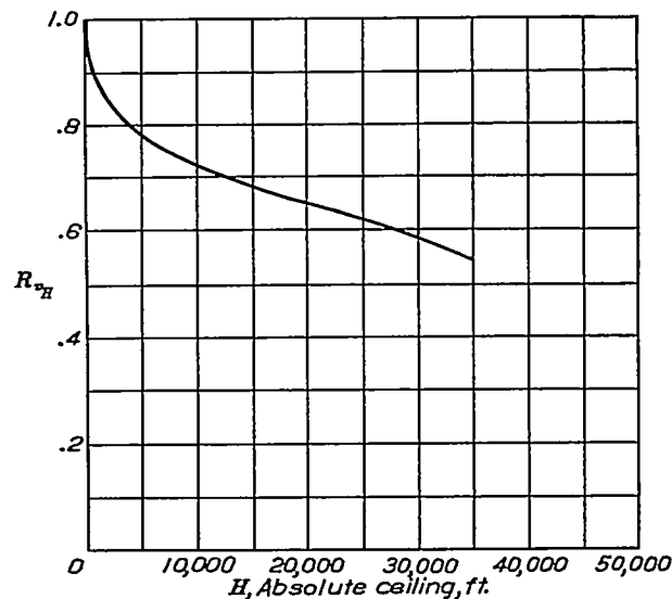
FIGURE 8.— R_{vH} as a function of absolute ceiling
