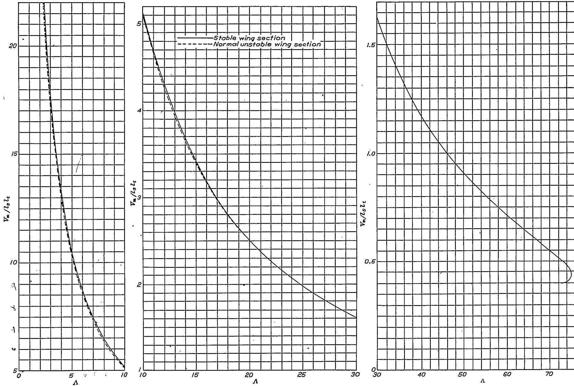
FIGURE 30. \frac{V_m}{l_s l_t} as a function of \Lambda . V_m = maximum velocity at sea level in m. p. h.
