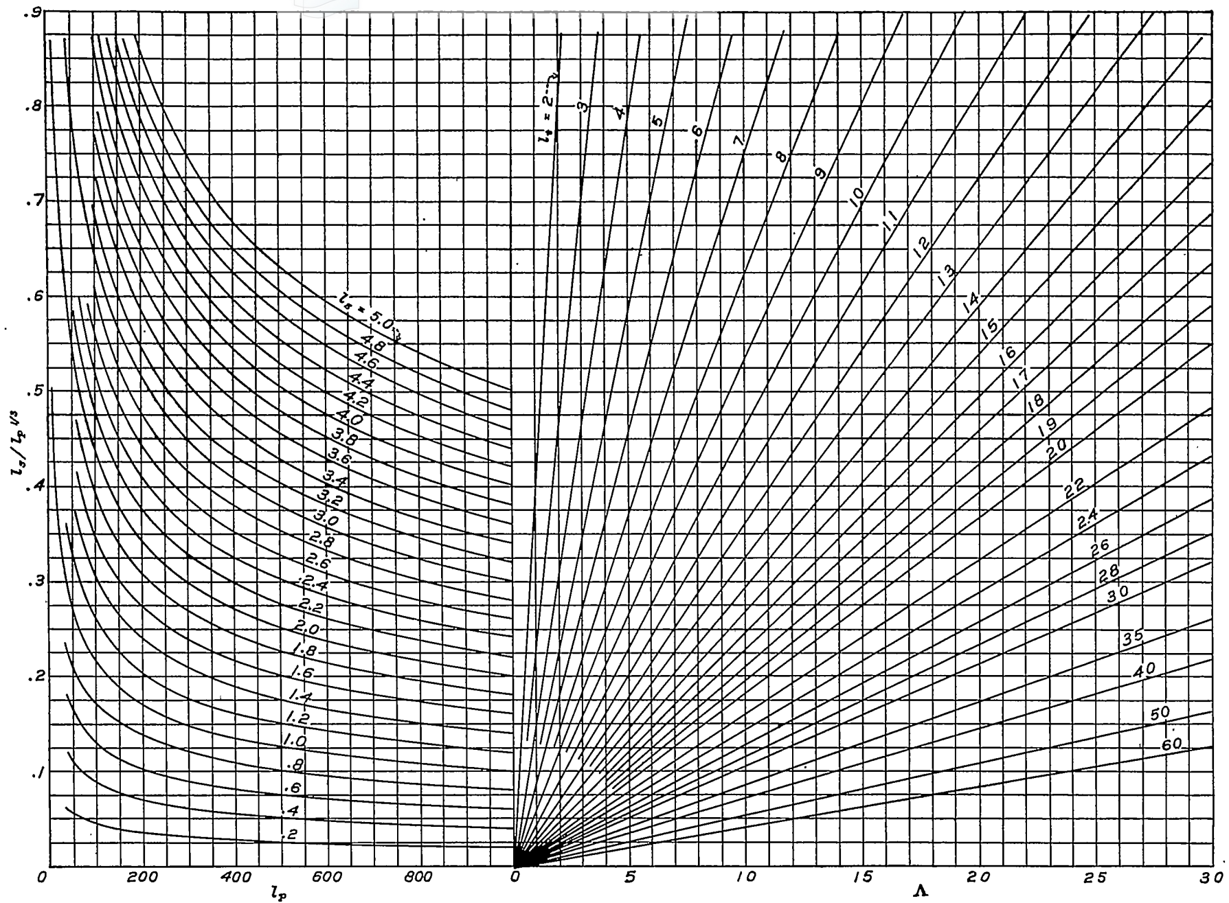
FIGURE 28.—Chart for the graphical solution of \Delta = \frac{l_t l_t^{1/2}}{l_p v}
