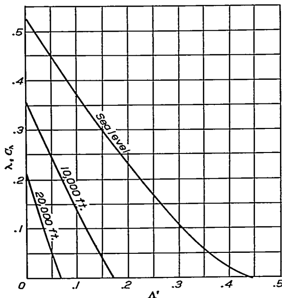
FIGURE 7.— \lambda_v C_h as a function of \Lambda' and altitude ( \sigma )
