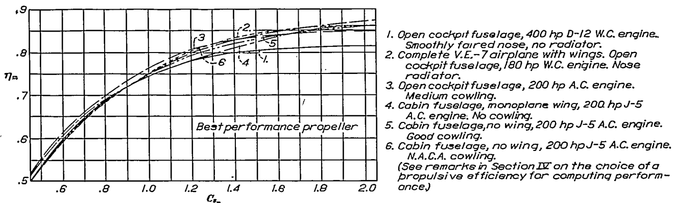
FIGURE 27.—Propulsive efficiency at V_{max} as a function of C_L for various aircraft engines and bodies. Nine-foot metal propeller. Navy No. 4412. Data from National Advisory Committee for Aeronautics. Technical Report 350
