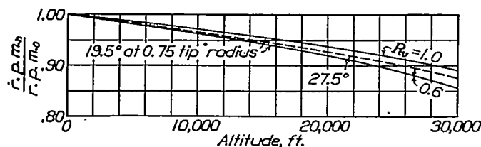
FIGURE 21.—Variation of full-throttle r. p. m. at constant velocity with altitude
