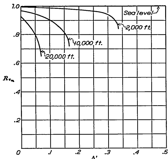
FIGURE 5.— R_{v_m} as a function of \Delta' and altitude ( \sigma )
