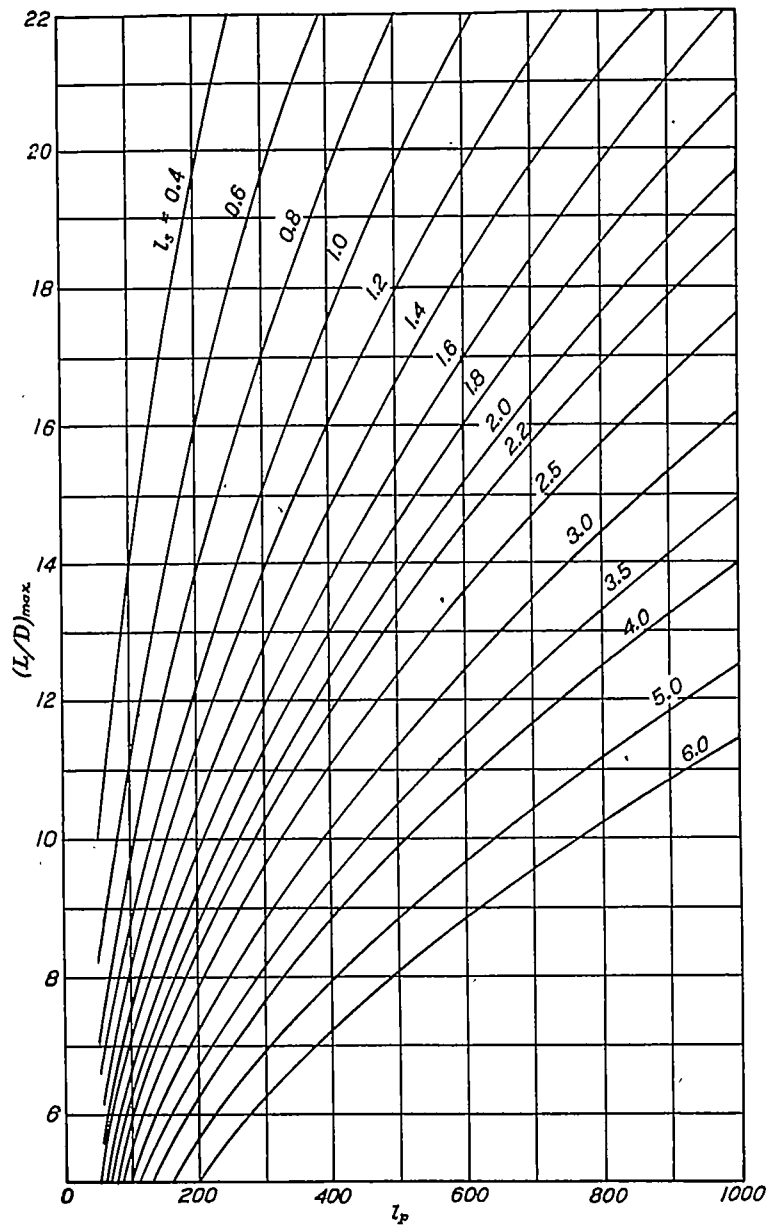
FIGURE 41.—Maximum lift/drag ratio as a function of l_p and l_i .
