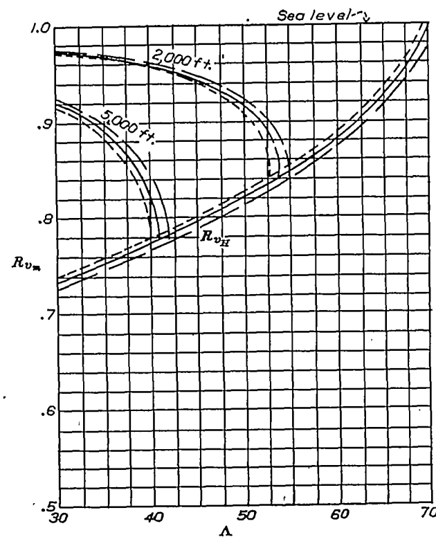
FIGURE 31.— Rv_m = \frac{\text{max. velocity at altitude}}{\text{max. velocity at sea level}} as a function of A , at various altitudes. Rv_H = \frac{\text{velocity at absolute ceiling}}{\text{max. velocity at sea level}} as a function of A
