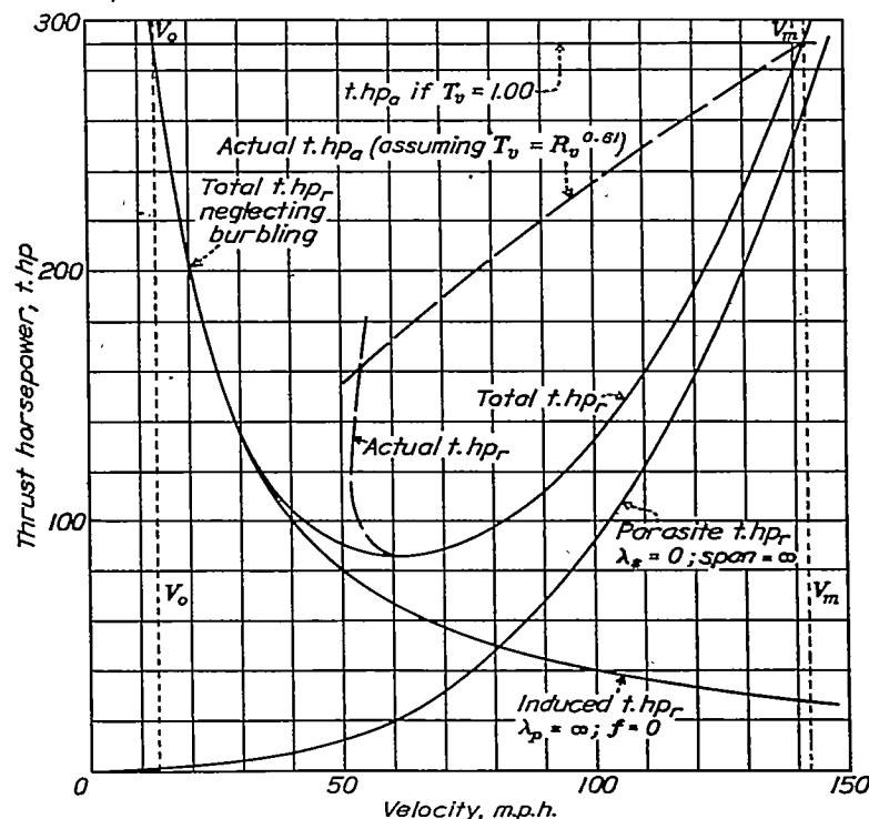
FIGURE 2.—Power curves for a normal airplane and its associated "ideal airplane." Assumed airplane characteristics: \lambda_p=250,000 ; \lambda_s=800 ; \lambda_t=0.025 ; \Delta'=0.0523 ; W=4,000 lb.; S=400 sq. ft.; C_{L_{max}}=1.45
