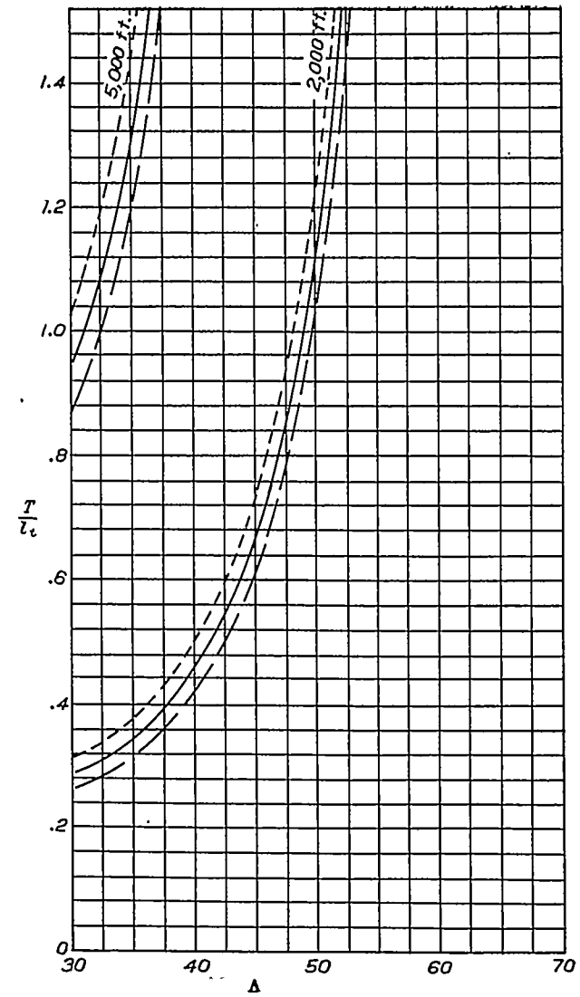
FIGURE 35.— \frac{T}{t_1} as a function of A , at various altitudes. T =minimum time required to climb to altitude (minutes)
