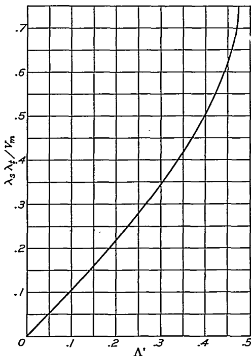
FIGURE 1. \frac{\lambda_s \lambda_t}{V_m} as a function of \Lambda' = \frac{\lambda_s \lambda_t^{3/4}}{\lambda_p^{3/4}}
