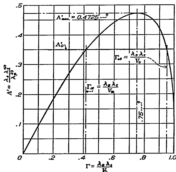
FIGURE 3.—Plot of the fourth degree relation connecting \Delta' and \Gamma
