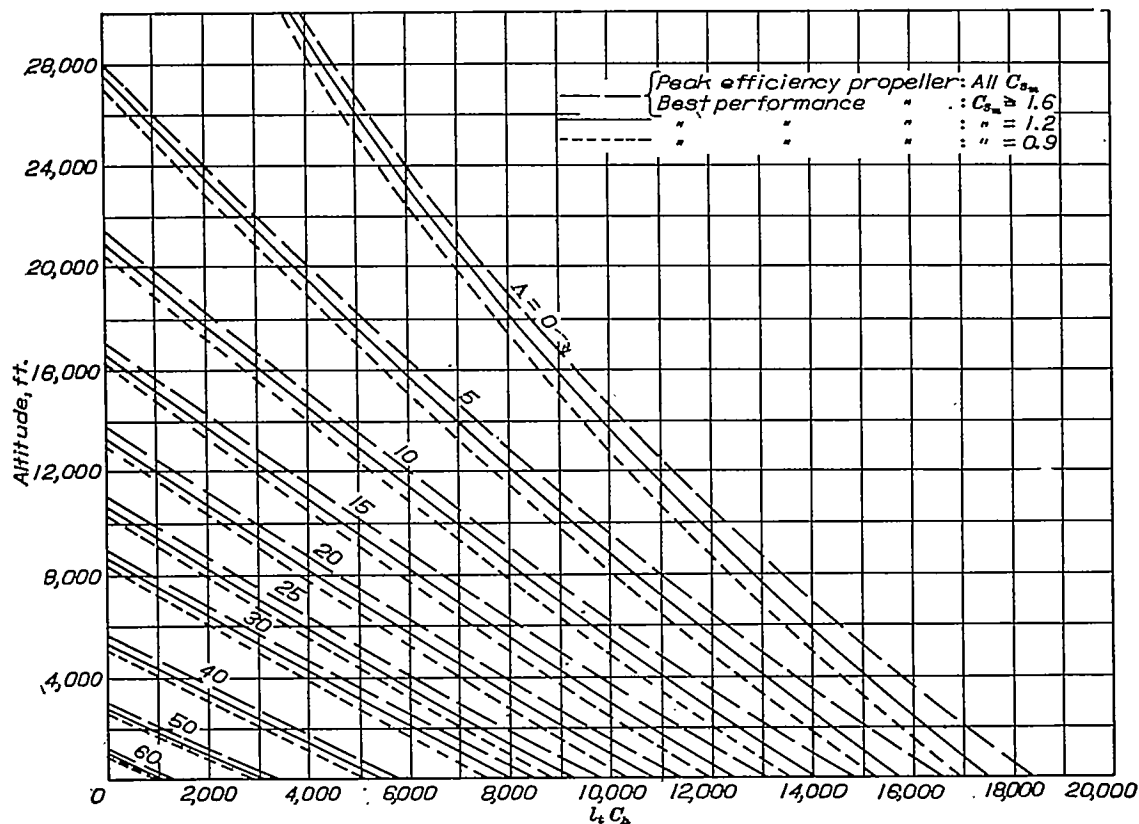
FIGURE 38.—Variation of l_t C_A with altitude for various values of A
