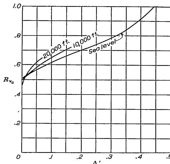
FIGURE 6.— R_{v_e} as a function of \Delta' and altitude ( \sigma )
