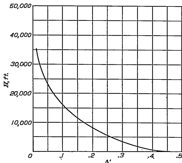
FIGURE 9.—Absolute ceiling as a function of \Lambda'
