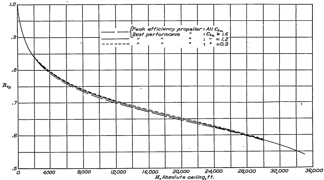
FIGURE 39.— R_{v_H} as a function of absolute ceiling. R_{v_H} = \frac{\text{velocity at absolute ceiling}}{\text{maximum velocity at sea level}}
