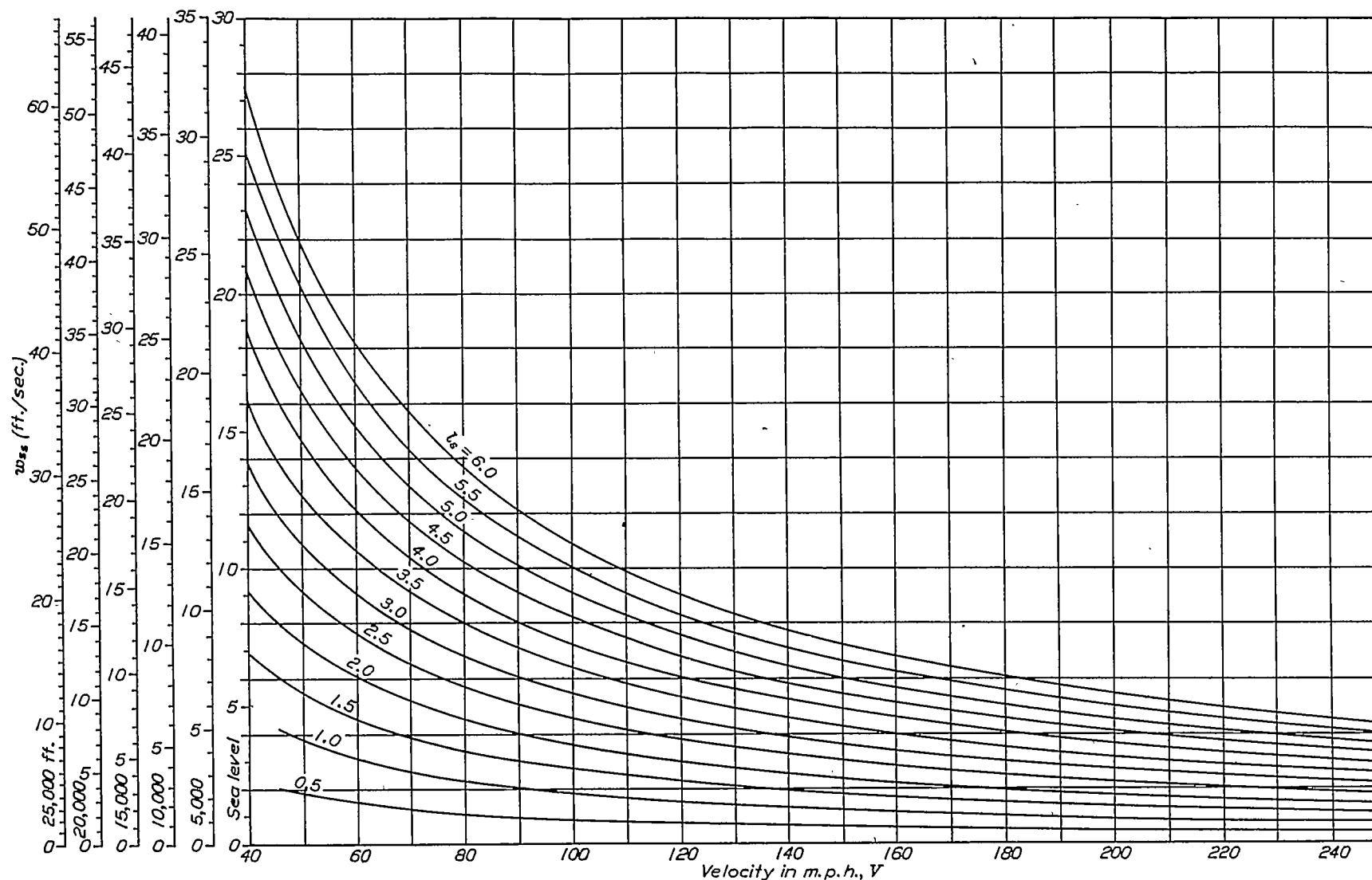
FIGURE 44.—The sinking speed w_s , due to the effective span loading l_e , as a function of l_e and V , at various altitudes
