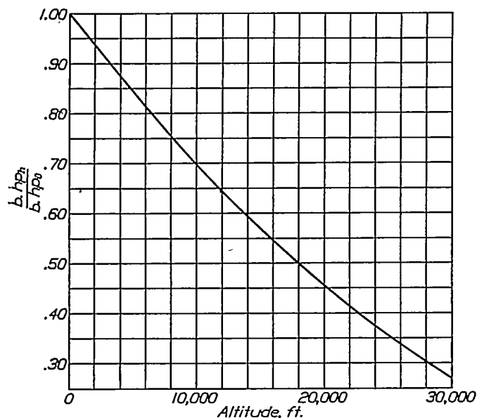
FIGURE 22.—Variation of full-throttle brake horsepower at constant r. p. m. with altitude
