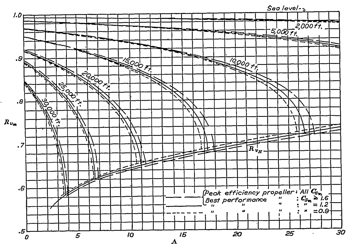
FIGURE 31.— Rv_m = \frac{\text{max. velocity at altitude}}{\text{max. velocity at sea level}} as a function of A , at various altitudes. Rv_H = \frac{\text{velocity at absolute ceiling}}{\text{max. velocity at sea level}} as a function of A
