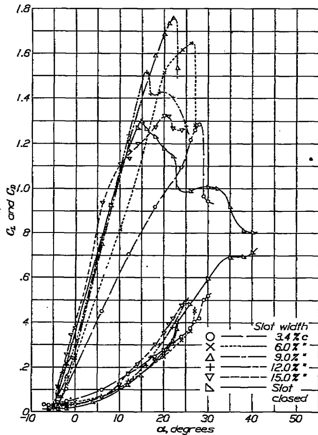
FIGURE 21.— C_L and C_D versus \alpha . Slot gap=3.5 per cent c . Slot depth=2.5 per cent c above c
