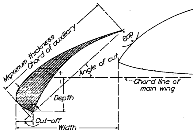
FIGURE 1.—Variable geometric factors—slotted Clark Y wing
