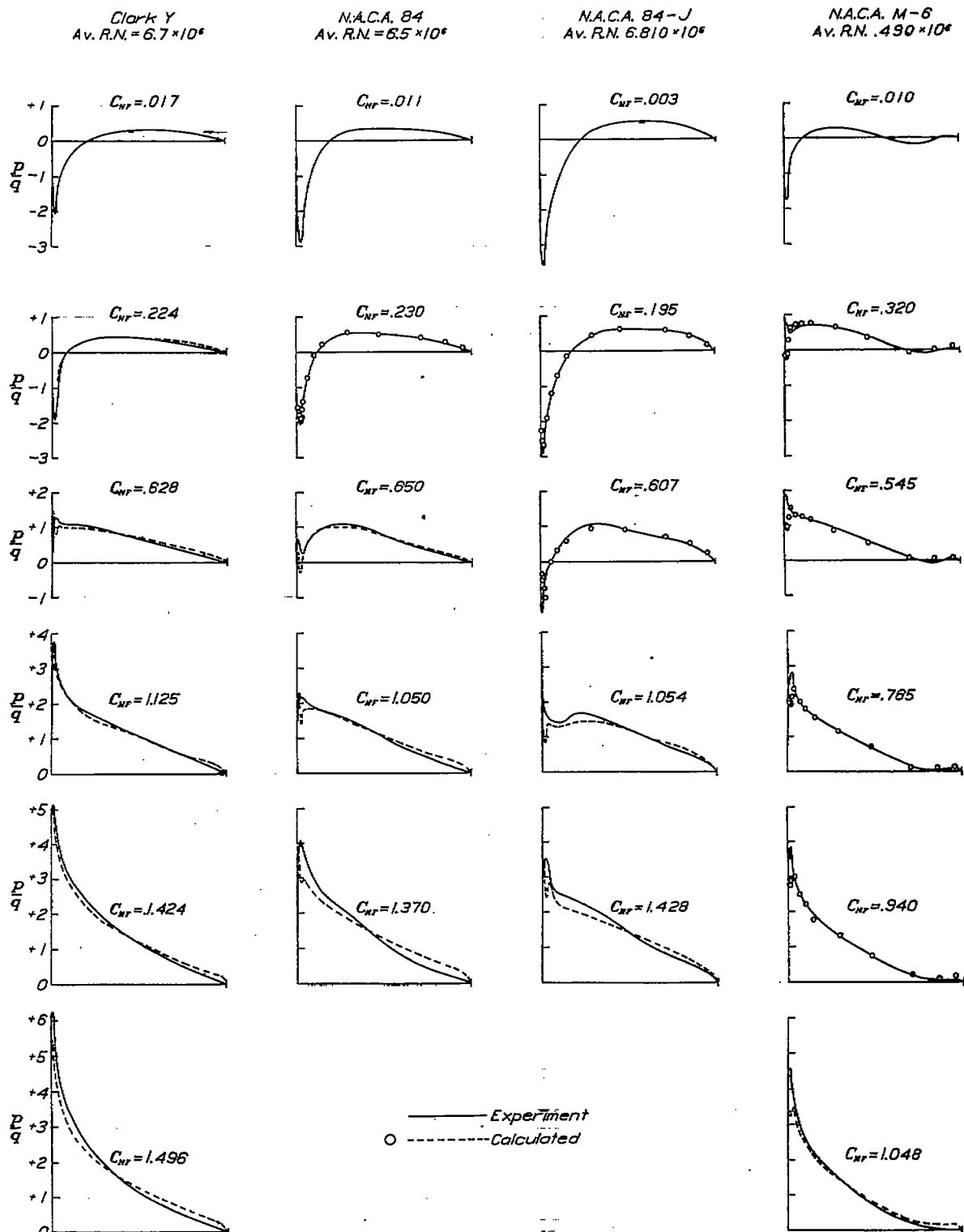
FIGURE 12.—Force distribution
