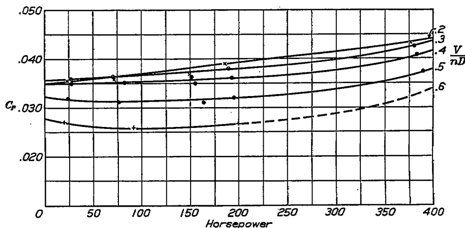
FIGURE 16.—Propeller No. 4412 ( 15^\circ at 42^\circ ), D-12 engine
