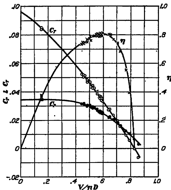
FIGURE 12.—Propeller No. 4102. Diameter 10 feet 5 inches
