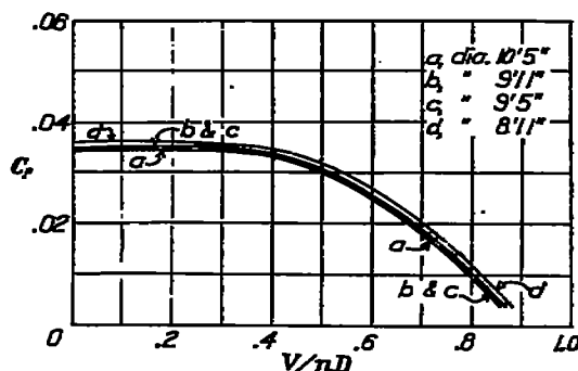
FIGURE 14.—Power coefficients
