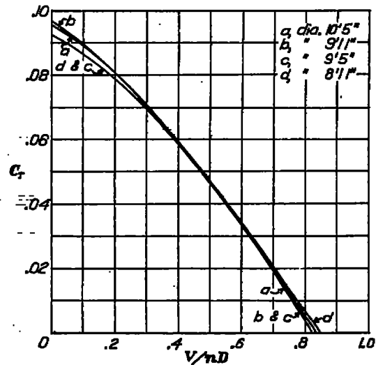
FIGURE 13.—Thrust coefficients
