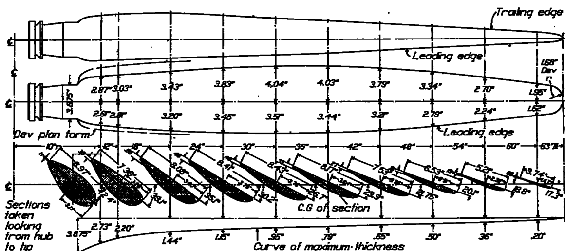
FIGURE 4.—Metal blade 10.5-foot diameter propeller. Right-hand No. 4102
