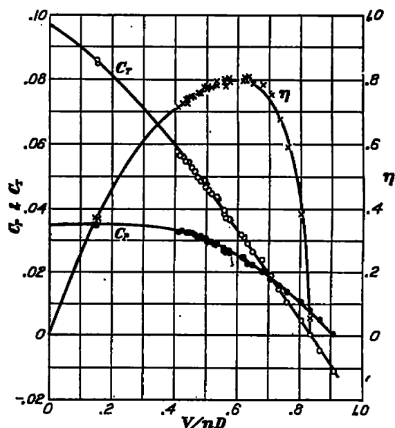
FIGURE 11.—Propeller No. 4414. Diameter 9 feet 11 inches
