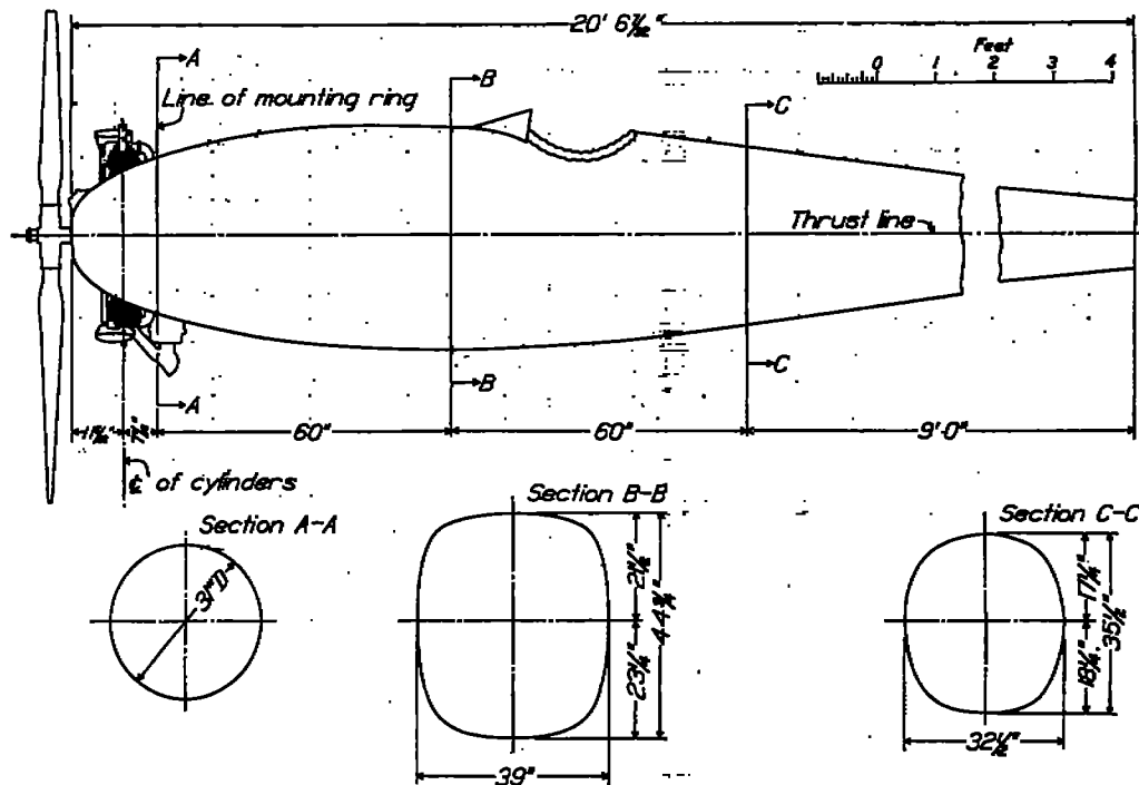
FIGURE 6.—Fuselage and engine
