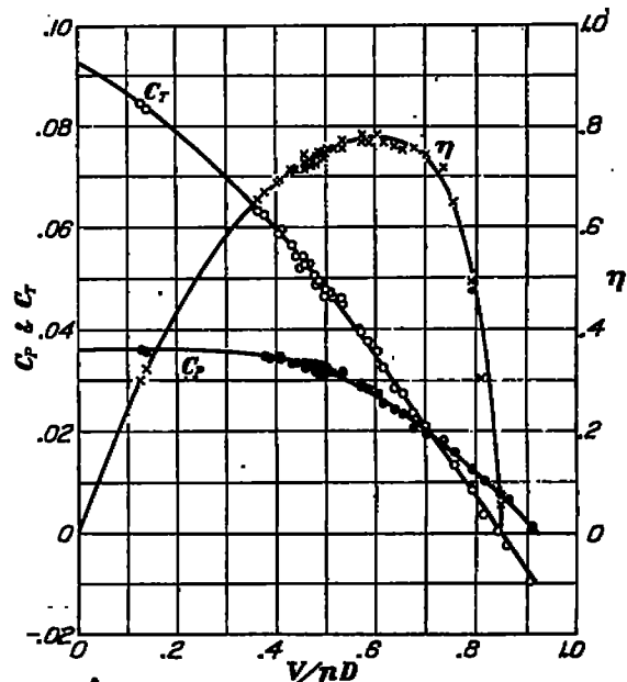
FIGURE 9.—Propeller No. 4412. Diameter 8 feet 11 inches
