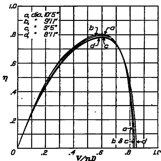
FIGURE 15.—Propulsive efficiencies
