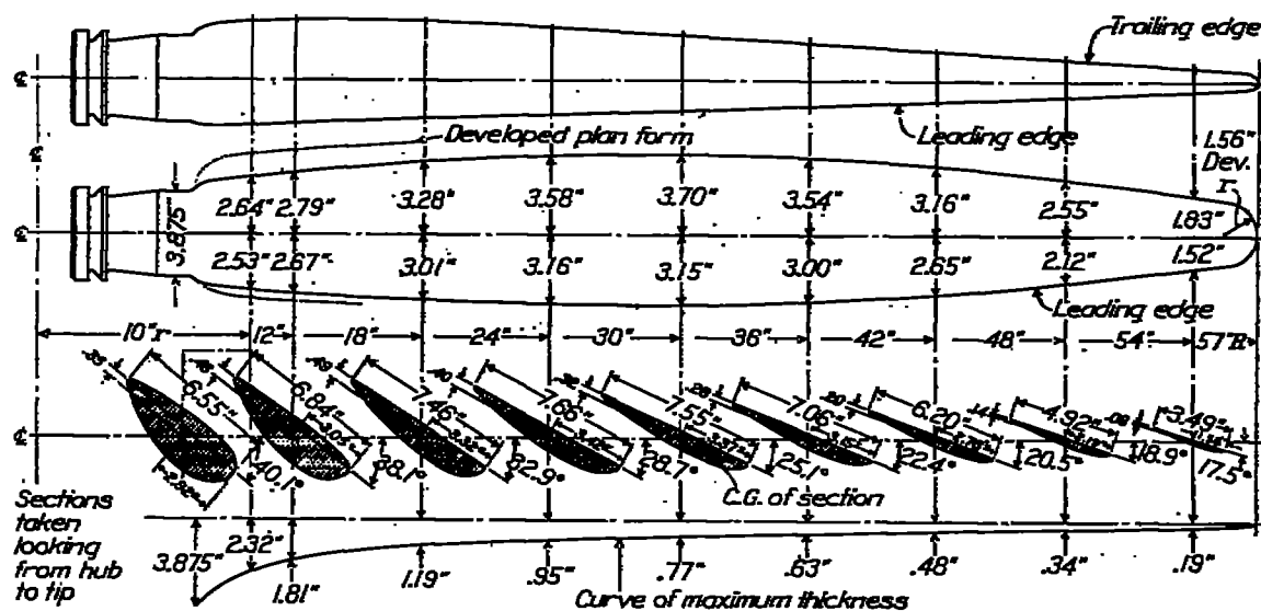
FIGURE 2.—Metal blade 9.5-foot diameter propeller. Right-hand No. 413
