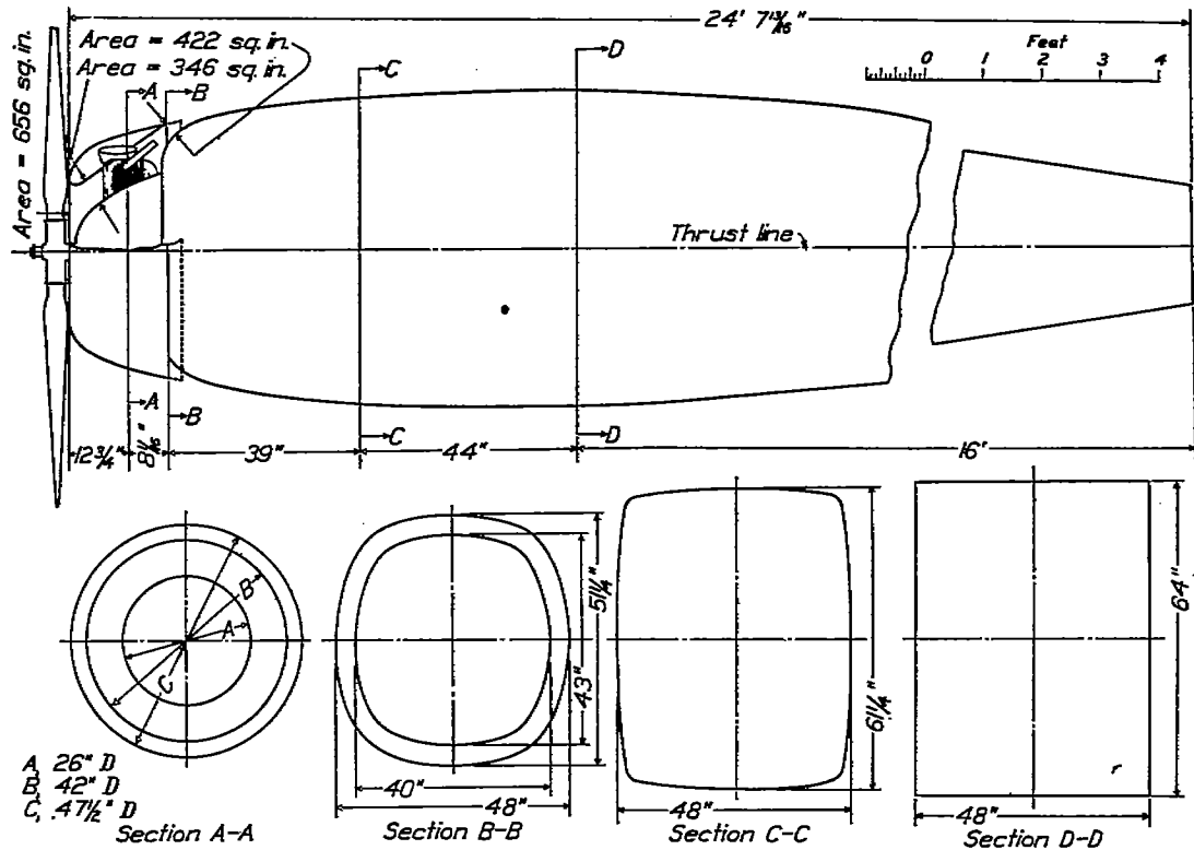
FIGURE 7.—Cowling No. 10 modified
