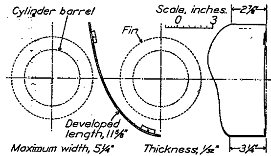
FIGURE 10.—Single deflector
