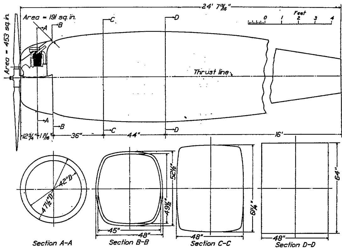
FIGURE 6.—Cowling No. 9
