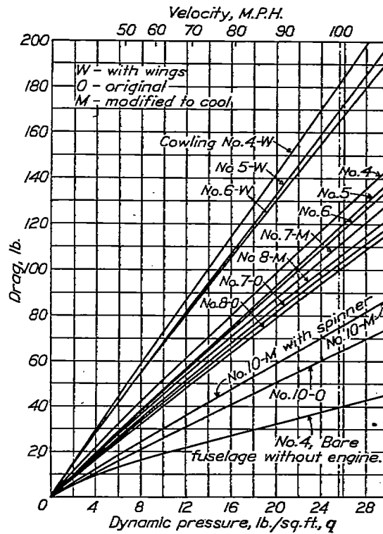
FIGURE 30.—Drag of fuselage and engine with various cowlings
