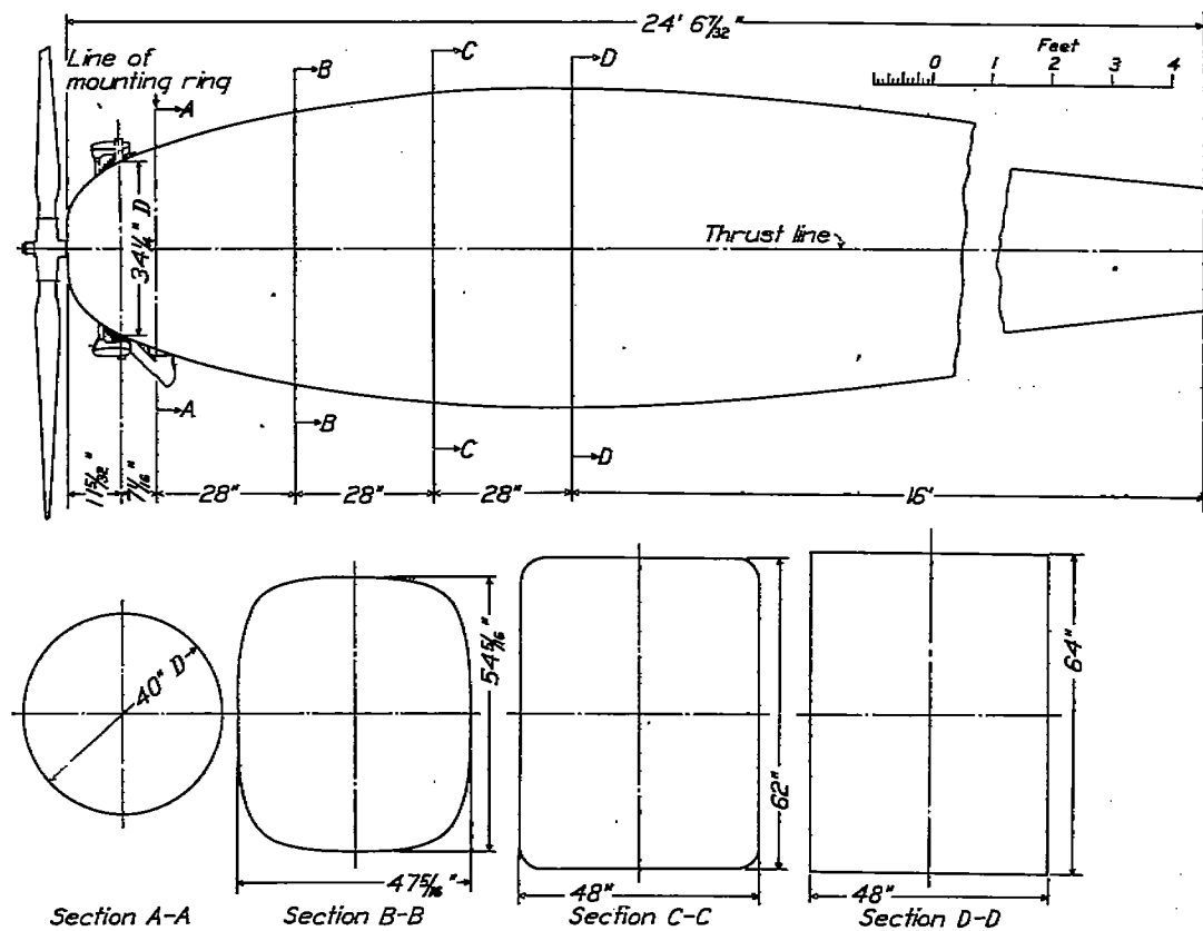
FIGURE 4.—Cowling No. 7
