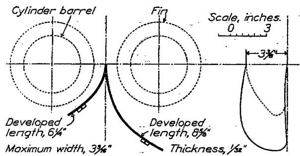
FIGURE 9.—Double deflectors
