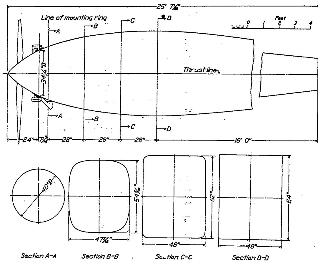
FIGURE 5.—Cowling No. 8
