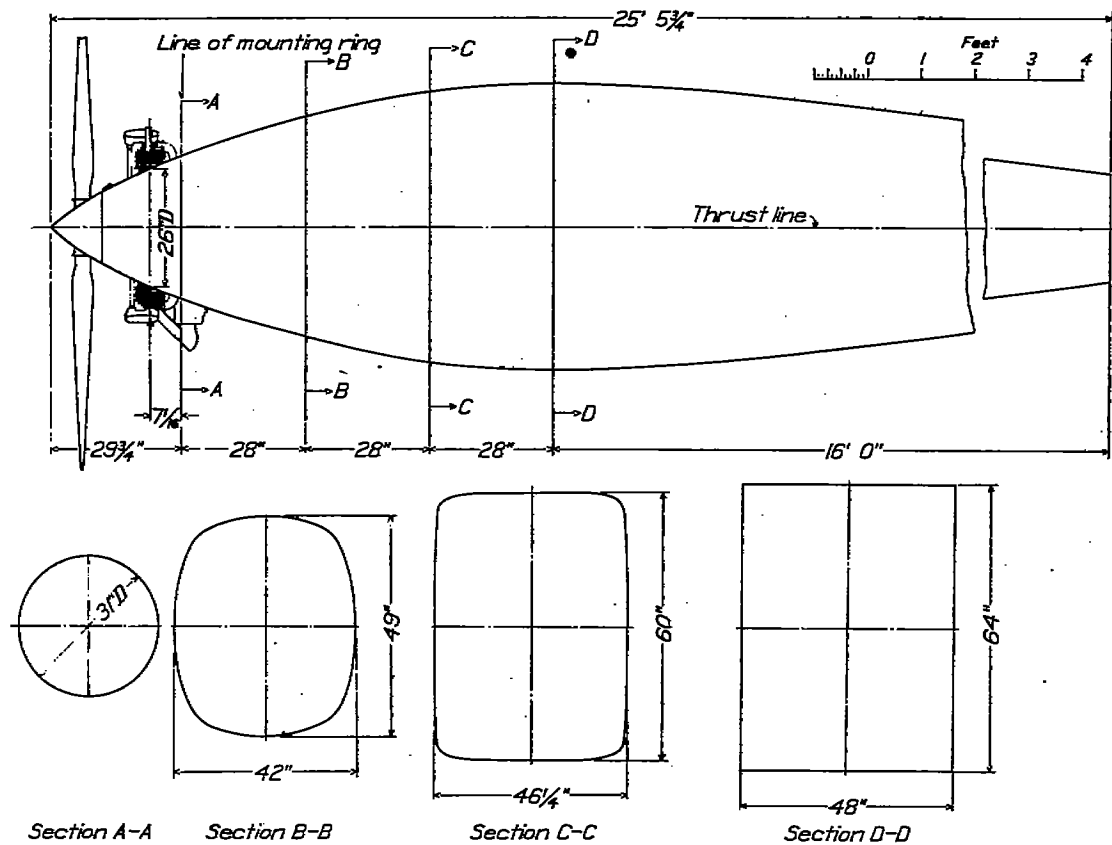
FIGURE 3.—Cowling No. 6
