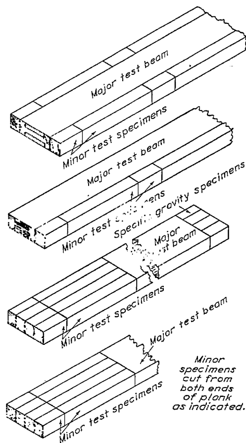
FIG. 4.—Matching diagrams.
