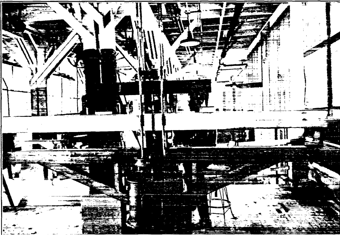
FIG. 5.—Two-point loading test.
