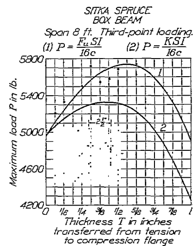
FIG. 7.—Influence of unequal flange depth on strength of box beams.
