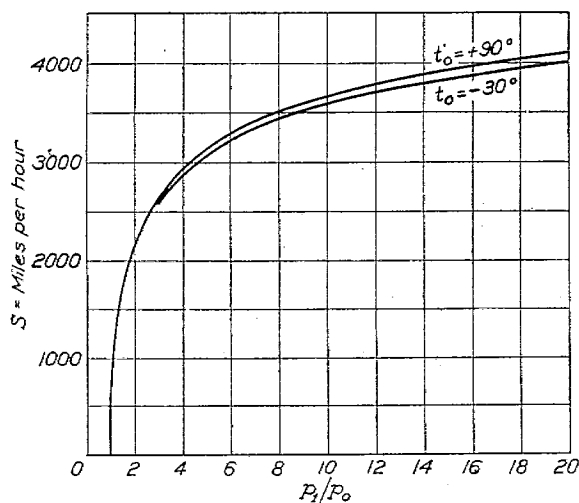
FIG. 4 (Table 5).—Jet speed, S .
