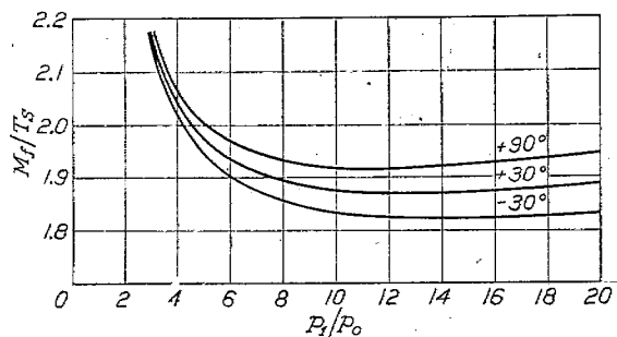
FIG. 6 (Table 7).—Lbs. fuel per hour for static thrust of 1 lb. = M_1/T_s .
