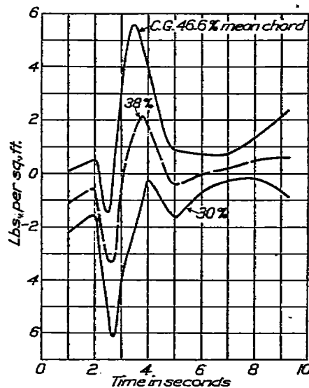
FIG. 32.—Effect of change of C. G. on tail loading.
