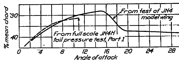
FIG. 30.—Center of pressure travel on wings.
