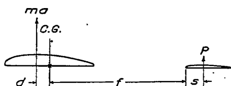
FIG. 29.—Forces acting on an airplane.
