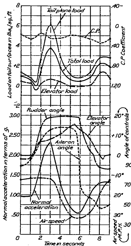
FIG. 25.—Slow flattening out of a dive and turn.
