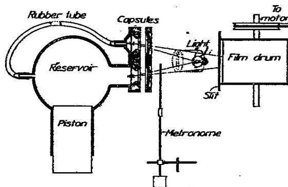
FIG. 15.—Apparatus for measuring the error in pressure reading through small tubes.
