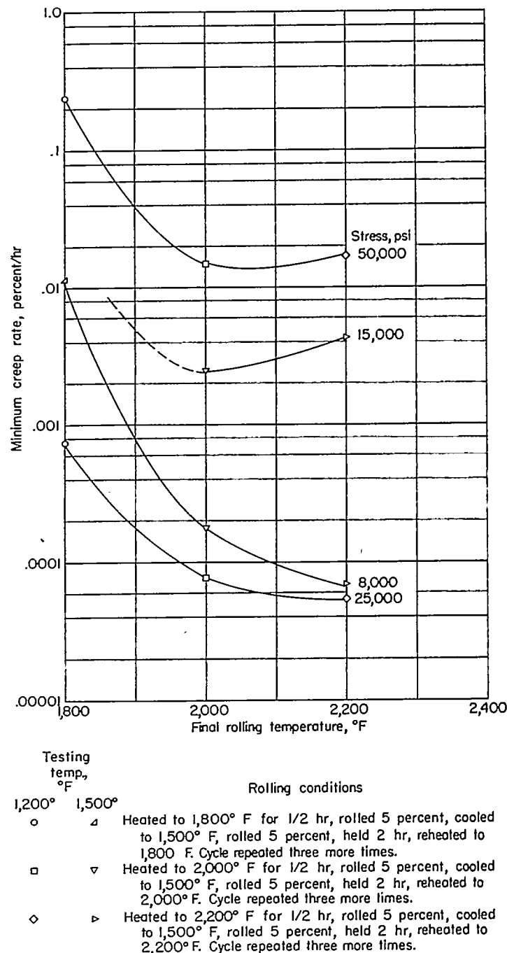
FIGURE 20.—Effect of cyclic rolling on minimum creep rates at 1,200° and 1,500° F for indicated initial stresses.
