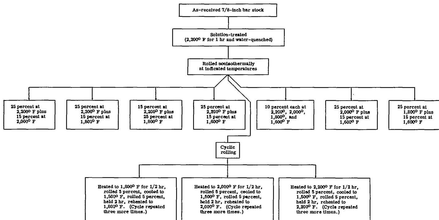
FIGURE 1.—Flow sheet of rolling program. Reductions were made in open passes unless otherwise indicated.
