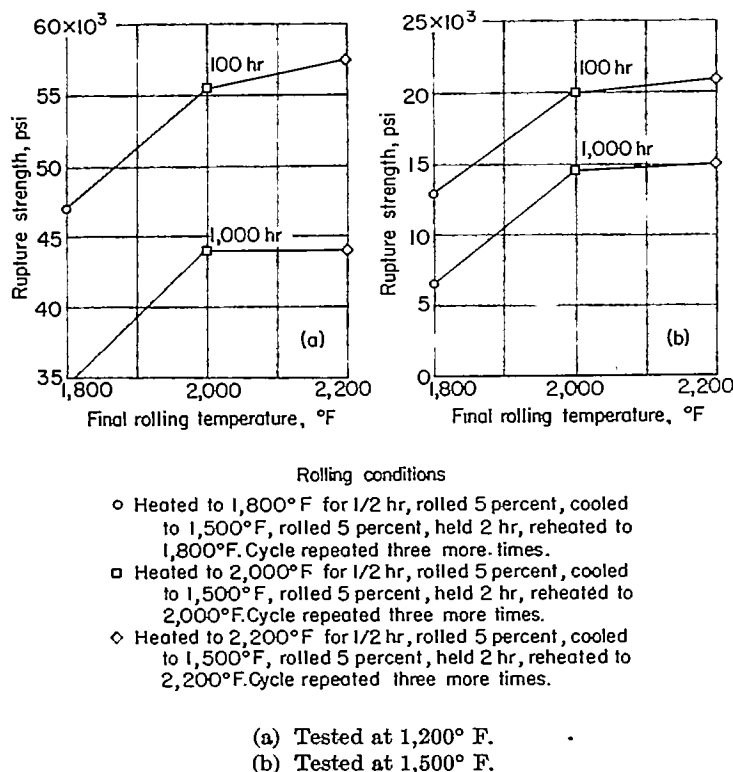
FIGURE 19.—Effect of cyclic rolling on the 100- and 1,000-hour rupture strengths at 1,200° and 1,500° F.
