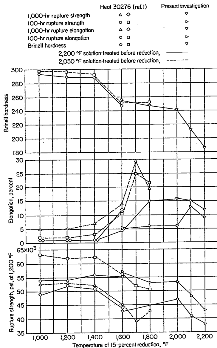
FIGURE 26.—Comparison of 1,200° F rupture strengths, rupture elongations, and Brinell hardnesses after 15-percent reduction at various temperatures for this investigation and another heat of same alloy (heat 30276, ref. 1).
