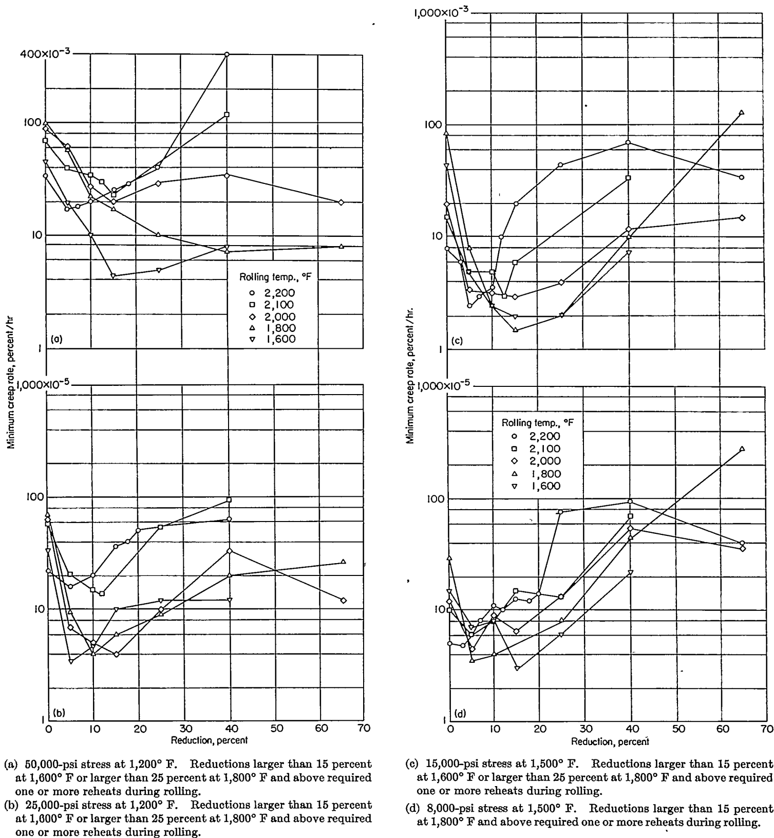
FIGURE 7.—Influence of isothermal reductions at indicated rolling temperature on as-rolled minimum creep rates in 1,000 hours for various stresses at 1,200° and 1,500° F.
