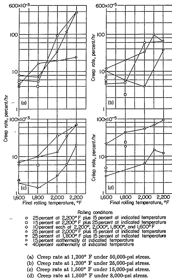
FIGURE 16.—Effect of rolling temperature on creep rate at 1,200° and 1,500° F for various amounts and methods of deformation.
