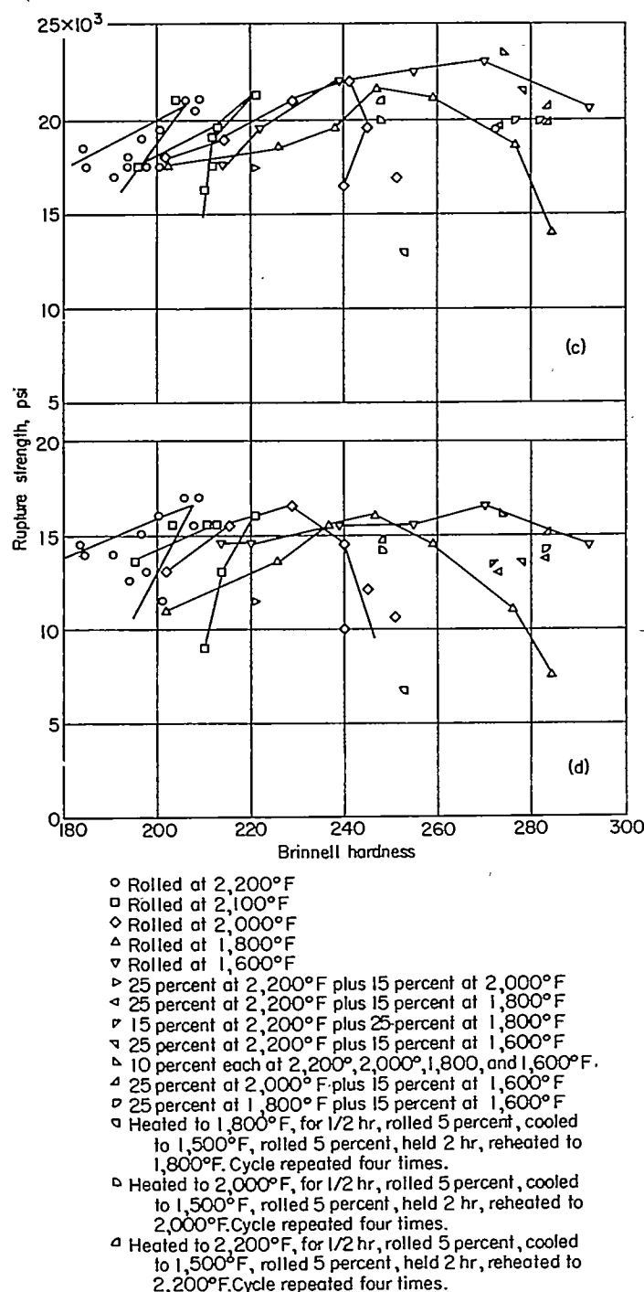
(c) 100-hour rupture strengths at 1,500° F. (d) 1,000-hour rupture strengths at 1,500° F.
