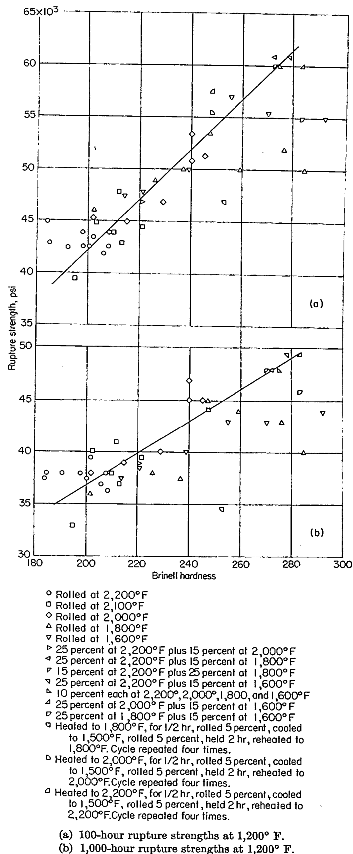
FIGURE 24.—Correlation of 100- and 1,000-hour rupture strengths at 1,200° F and 1,500° F with as-rolled Brinell hardness.
