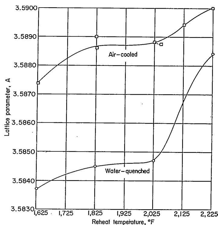
FIGURE 13.—Influence of cooling rate from reheat temperature on lattice parameter. Specimens solution-treated at 2,200° F for 1 hour, water-quenched, reheated to indicated reheat temperature for ¼ hour, and cooled as indicated.
