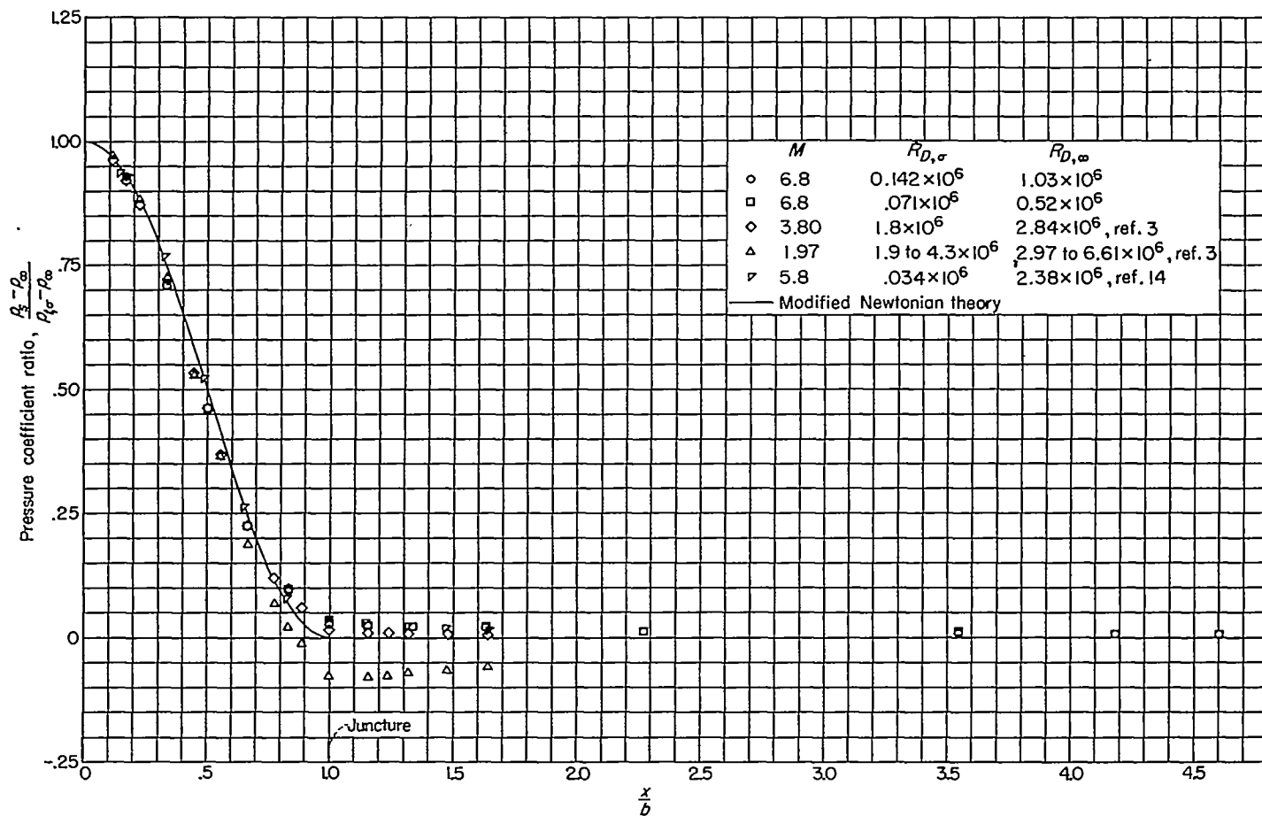
FIGURE 5.—Longitudinal pressure-coefficient distribution.
