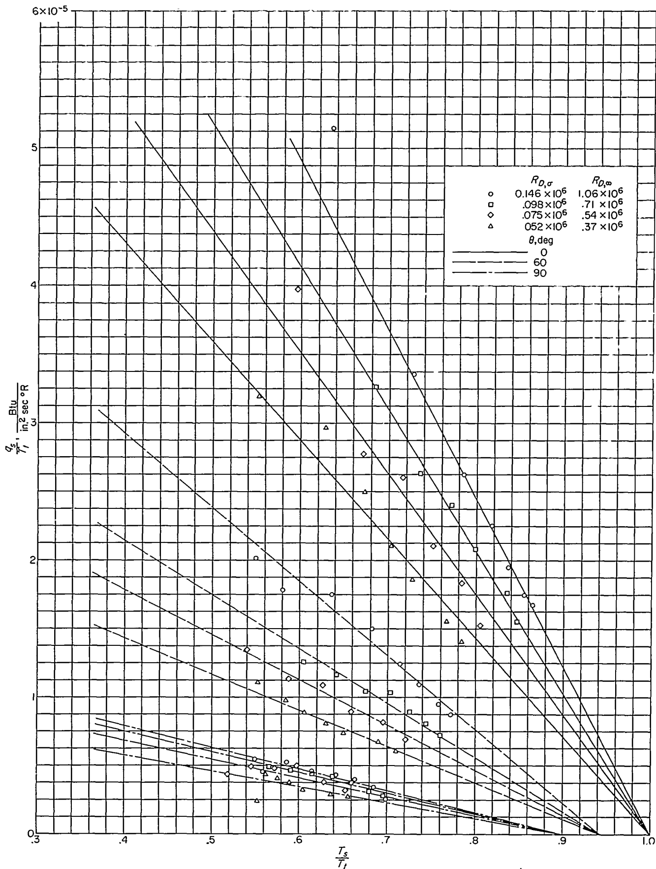
FIGURE 4.—Heat-transfer rate plotted against surface temperature for various angles of \theta on the 3.025-inch-diameter heat-transfer model.
