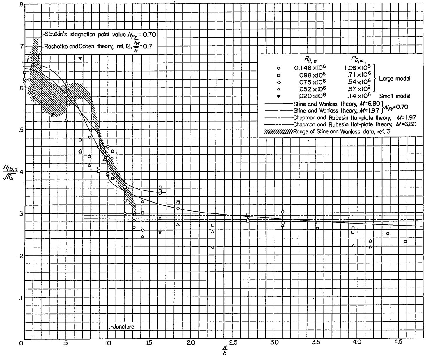
FIGURE 11.—Variation of the local heat-transfer parameter along the surface.
