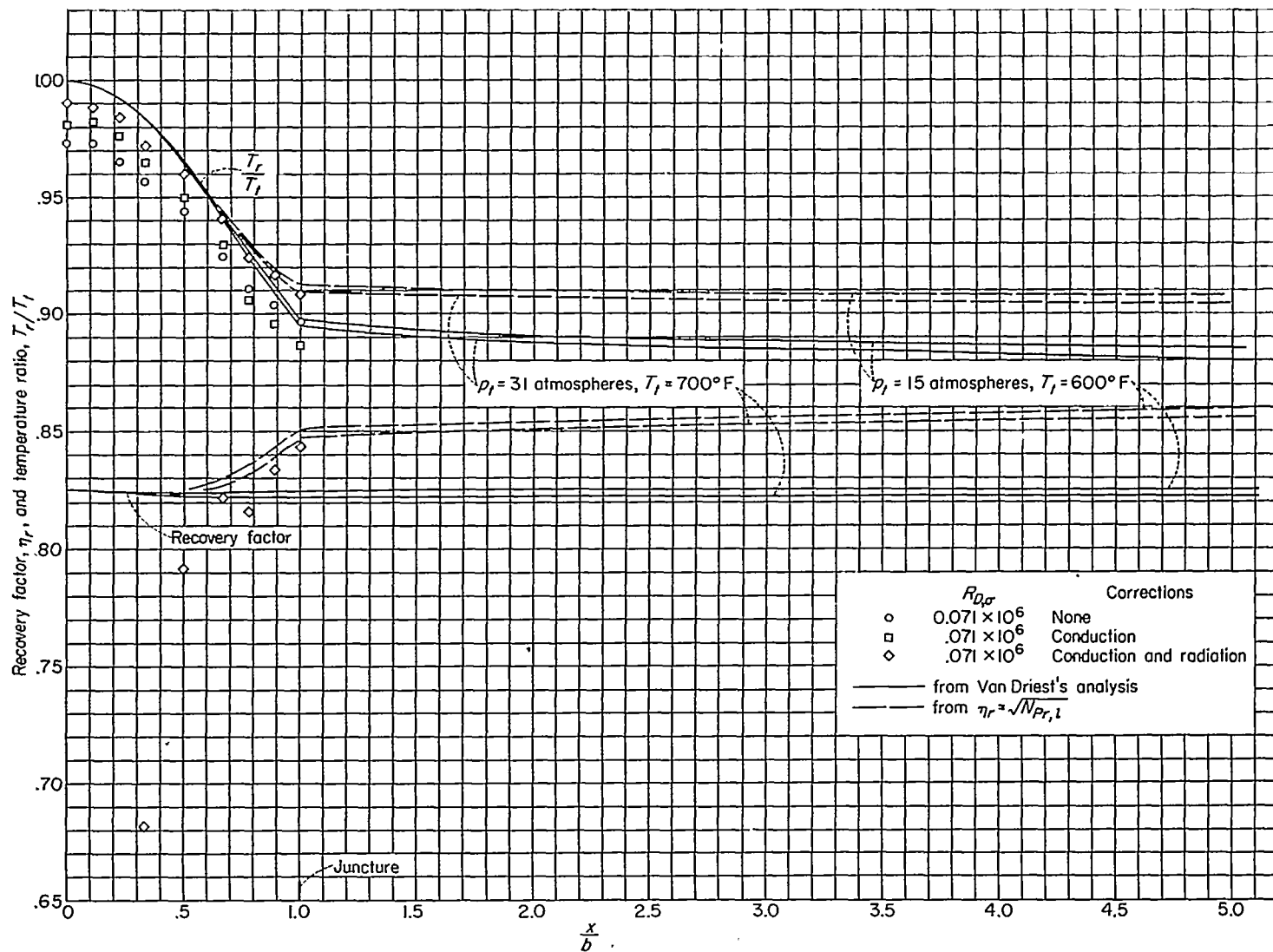
FIGURE 9.—Variation of the surface temperature ratio and recovery factor along the surface.
