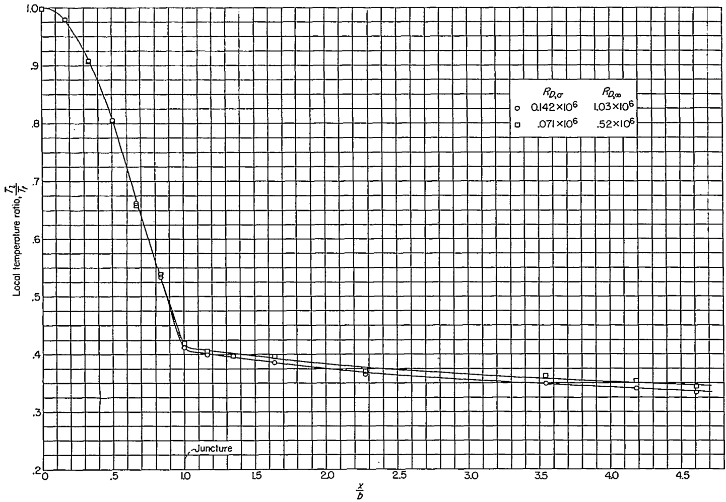
FIGURE 8.—Variation of the local temperature ratio (outside the boundary layer) along the surface.
