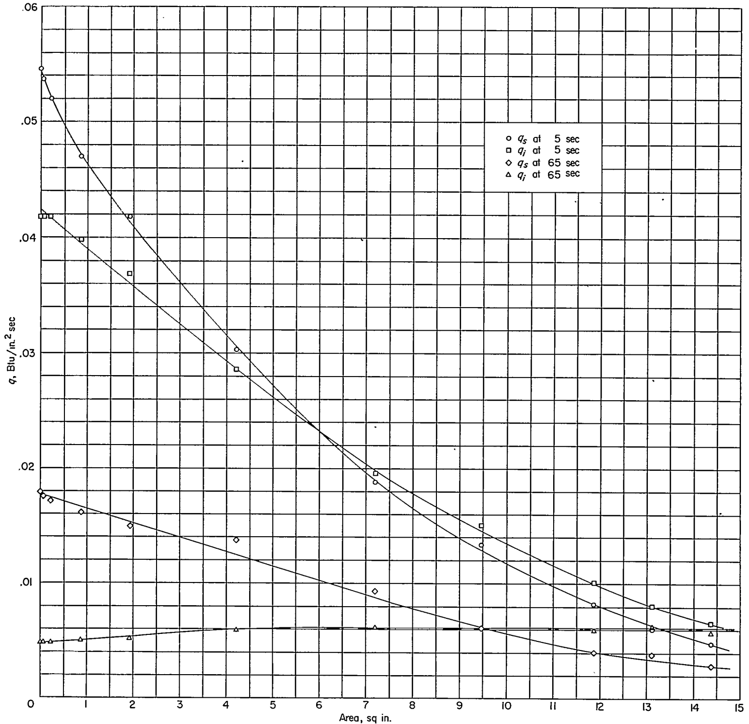
FIGURE 3.—Heat transfer to the hemisphere of the 3.025-inch-diameter heat-transfer model both with and without the conduction correction.
