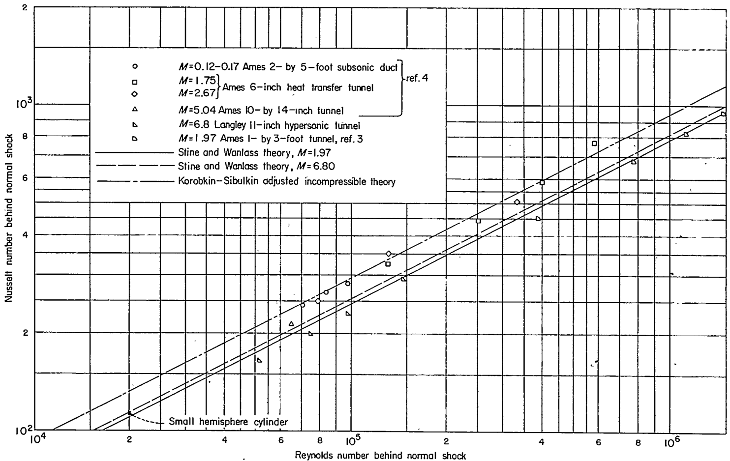
FIGURE 15.—Average heat transfer on the hemisphere plotted against Reynolds number for conditions behind a normal shock.
