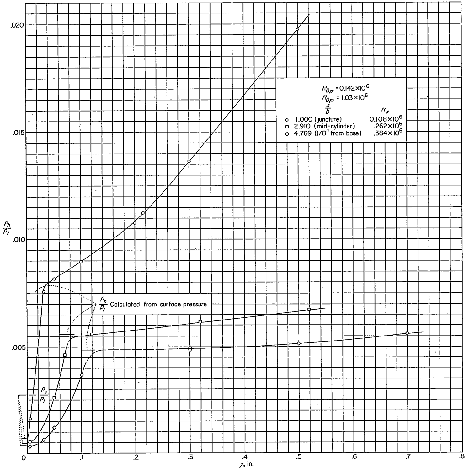
FIGURE 6.—Pitot pressure surveys of flow near the surface of the cylinder.
