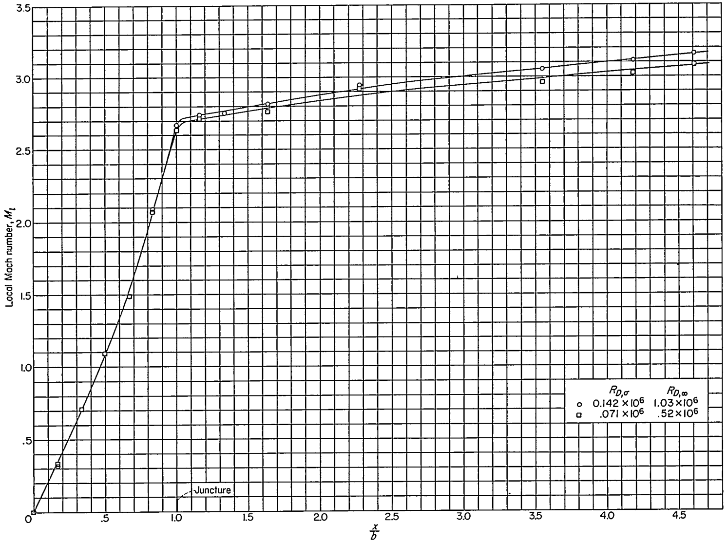
FIGURE 7.—Variation of local Mach number (outside the boundary layer) along the surface.
