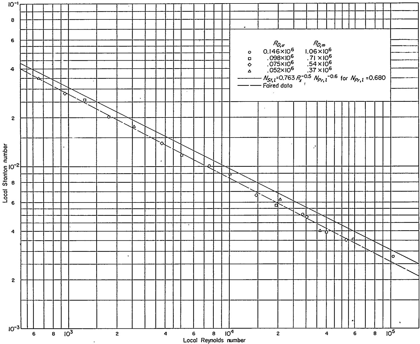
FIGURE 14.—Variation of the local Stanton number with the local Reynolds number for values of \theta from 0^\circ to 45^\circ .
