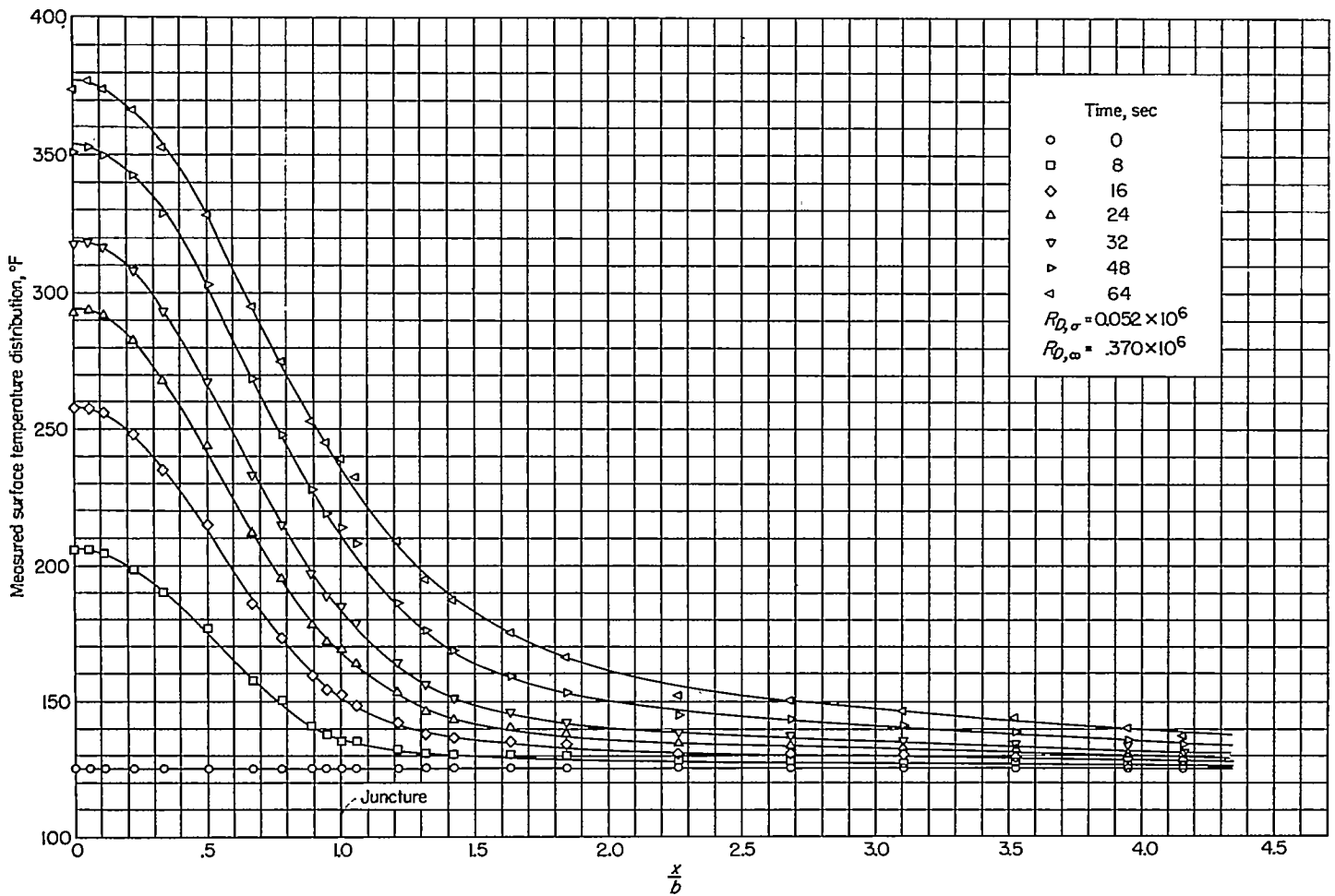
FIGURE 10.—Typical surface temperature distribution on 3.025-inch-diameter heat-transfer model at various times during a test.
