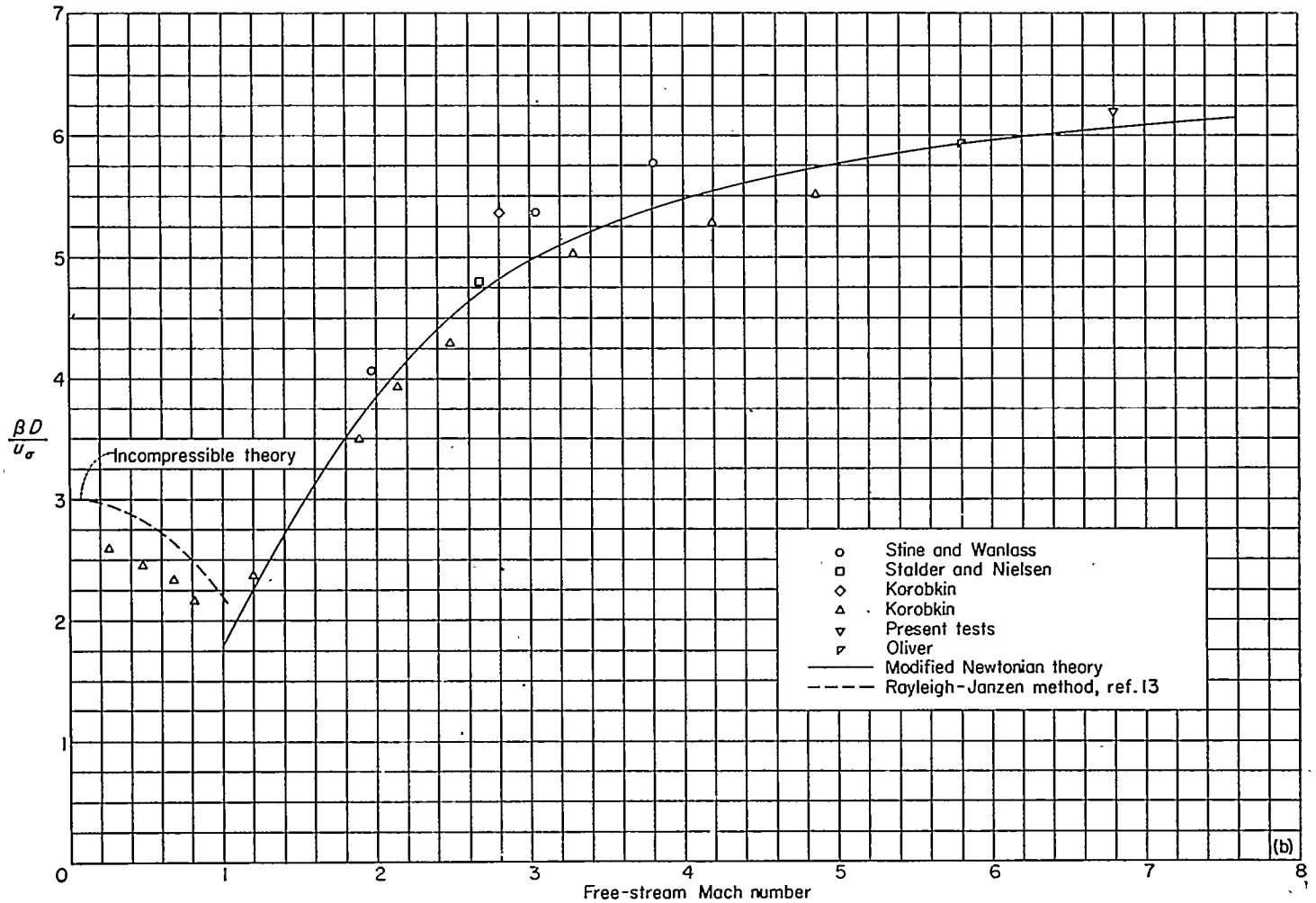
(a) Nondimensional local flow velocity along the surface.
