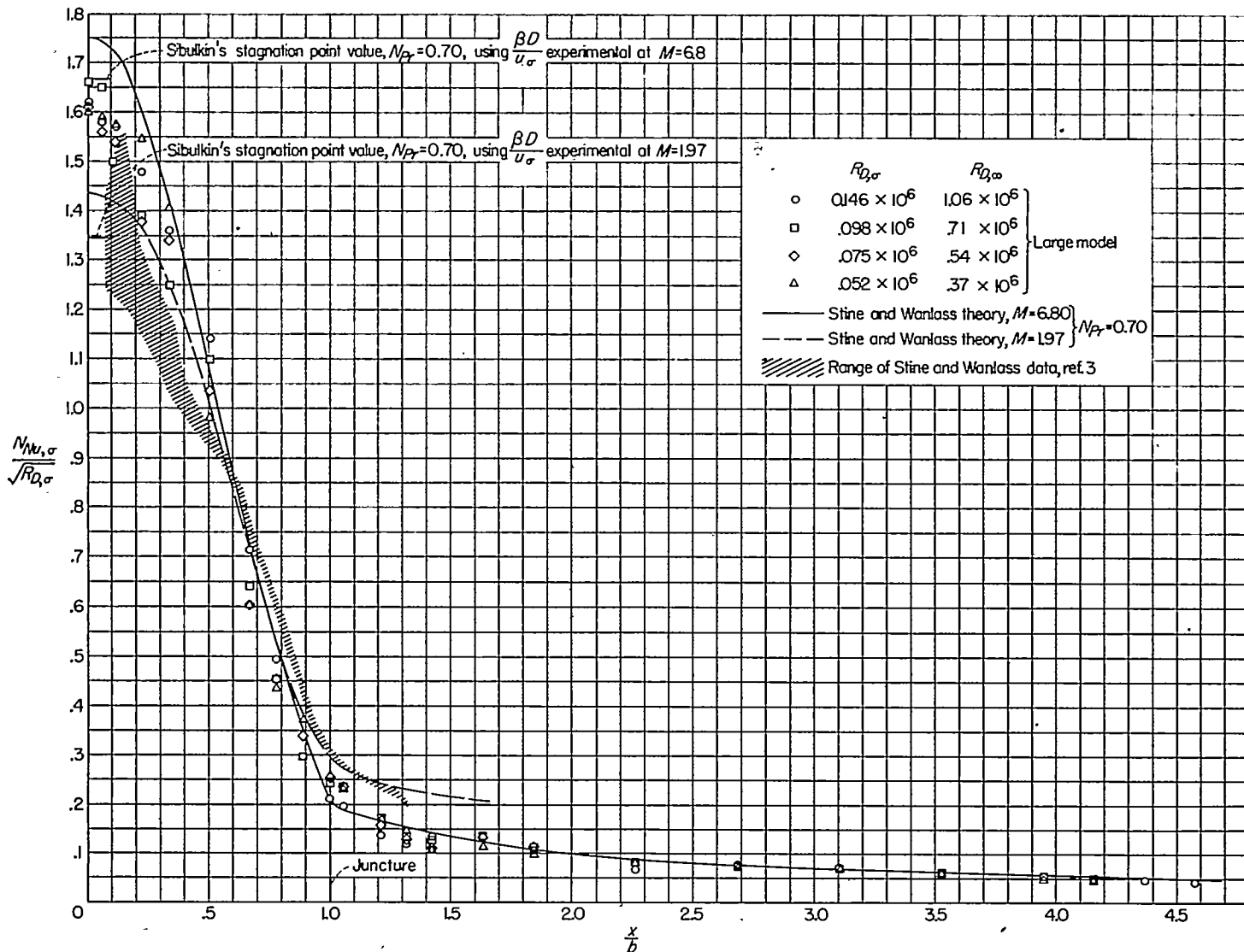
FIGURE 12.—Variation of the heat-transfer parameter (based on diameter and conditions behind the normal shock) along the surface.
